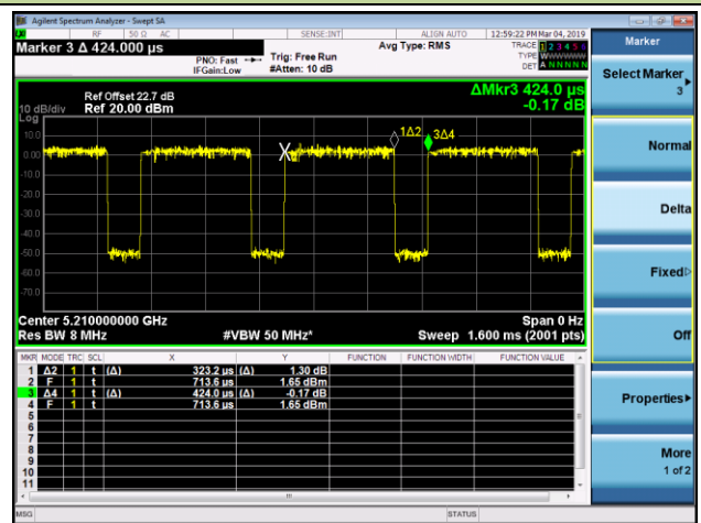
802.11ac-VHT80 (T = 424.0us)
