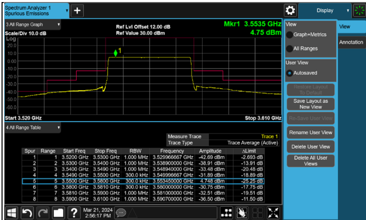
CH 637668 (3565.02 MHz)
