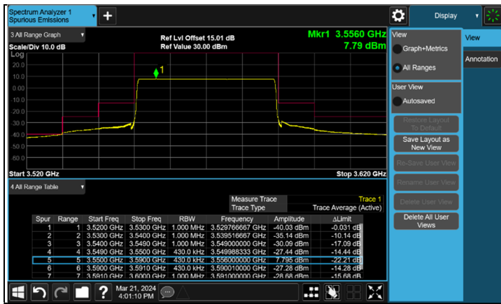
CH 638000 (3570 MHz)
