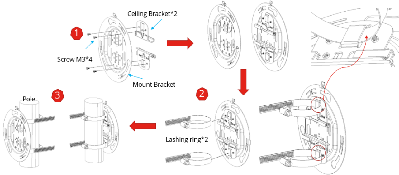
Figure 9. Pole Mount Overview
