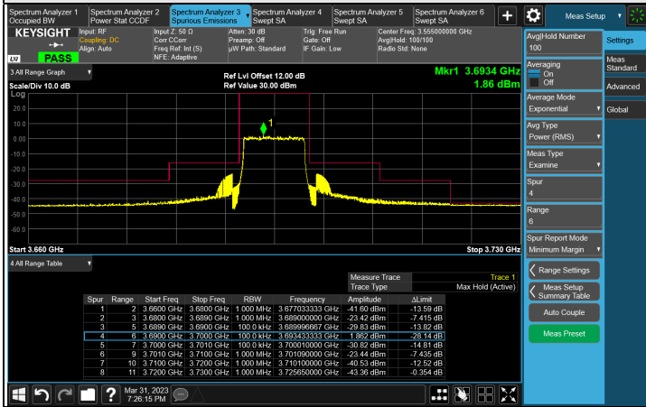
CH 646333 (3694.98 MHz)
