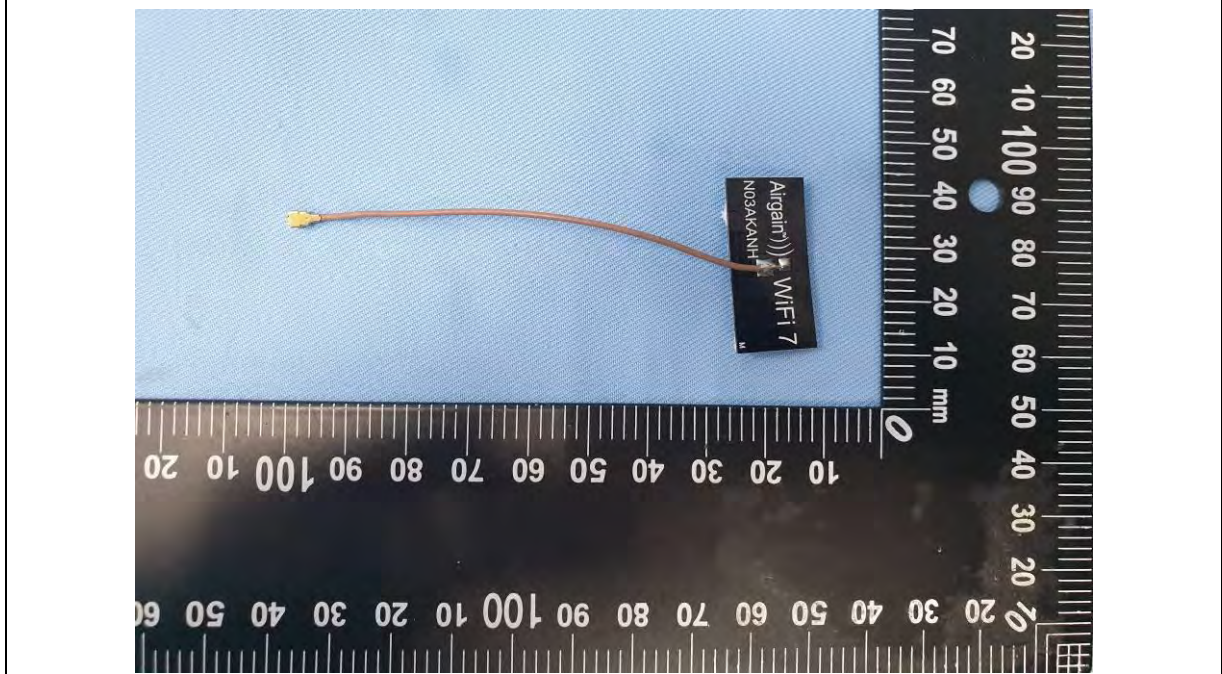
EUT Photo (28)
