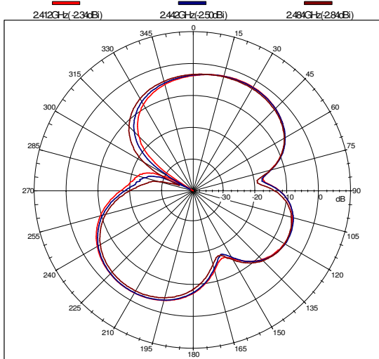
Far-field amplitude of S-ant2-H.nsi
