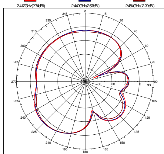
Far-field amplitude of L-ant2-H.nsi
