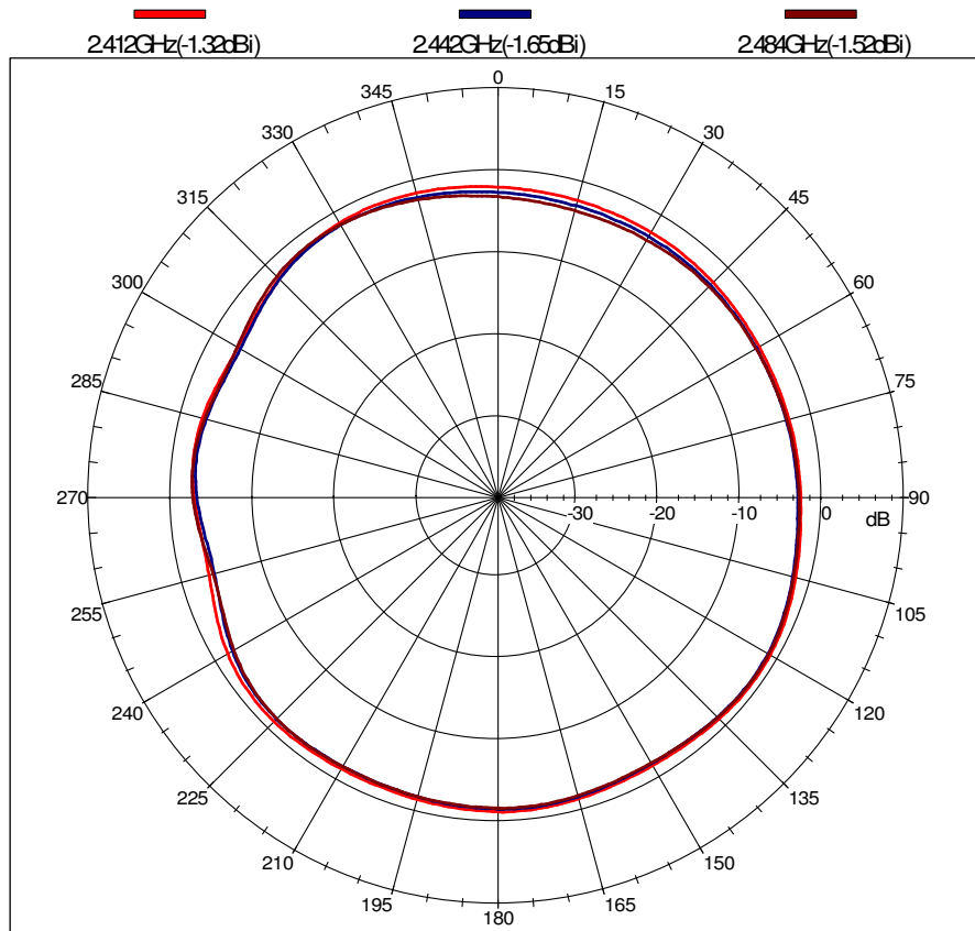
Far-field amplitude of L-11bg-H plane.nsi
