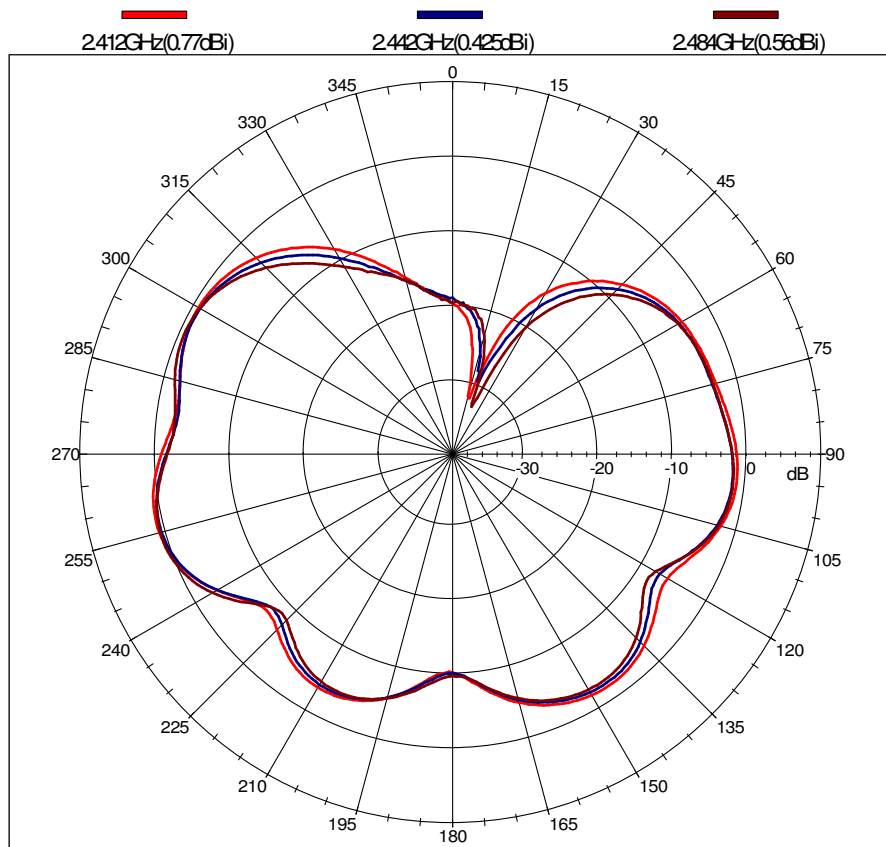
Far-field amplitude of L-11bg-E plane.nsi
