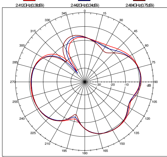
Far-field amplitude of L-ant-H.nsi
