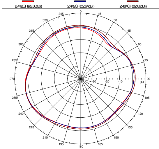
Far-field amplitude of S-ant-V.nsi
