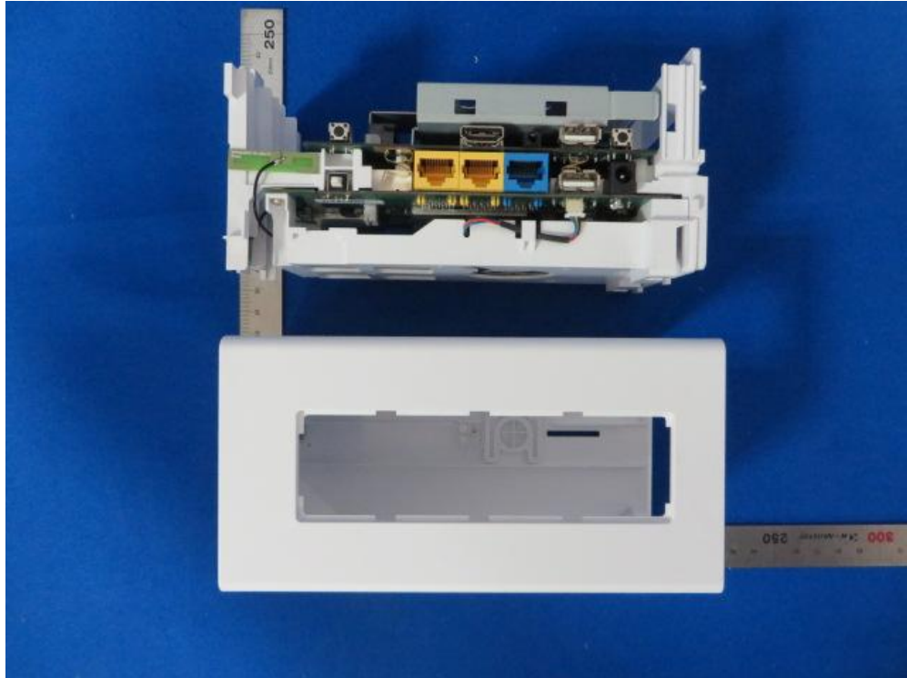
(8) EUT Photo (WHD0110(RoHS))
