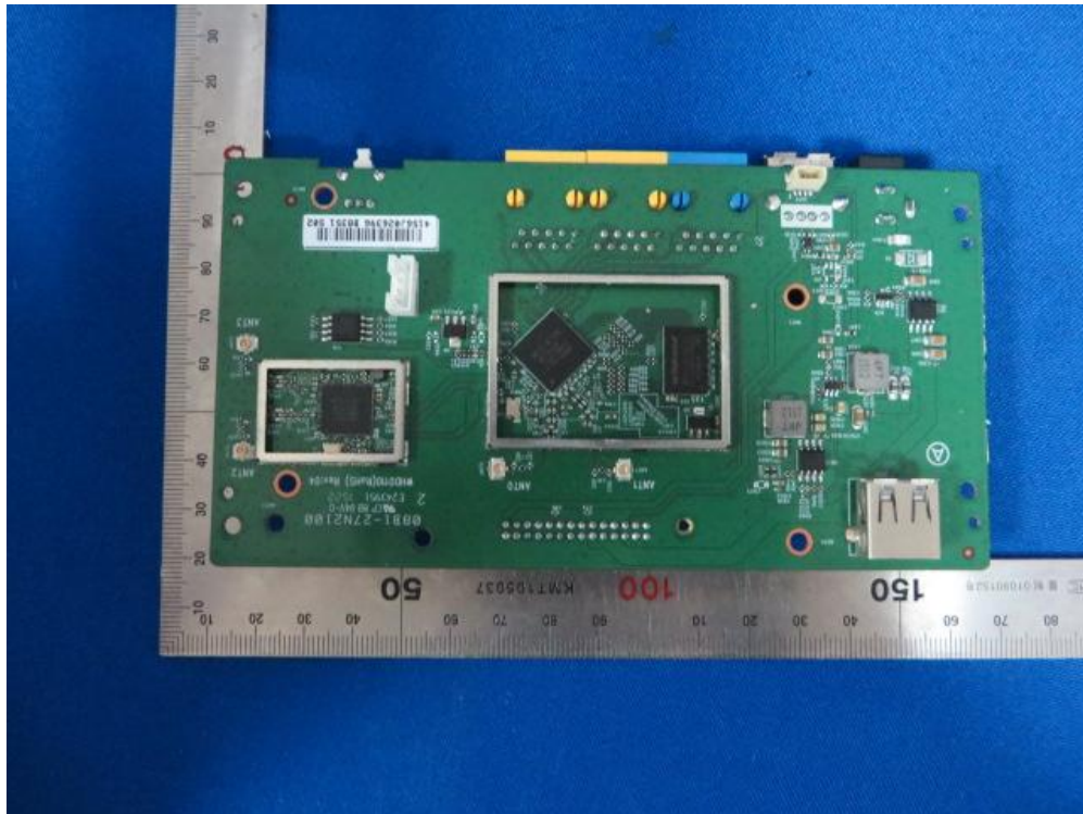
(47) EUT Photo (WHD0111(RoHS))
