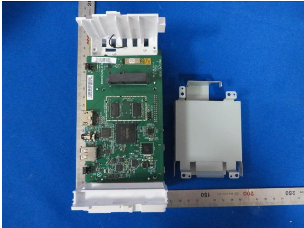
(17) EUT Photo (WHD0110(RoHS))
