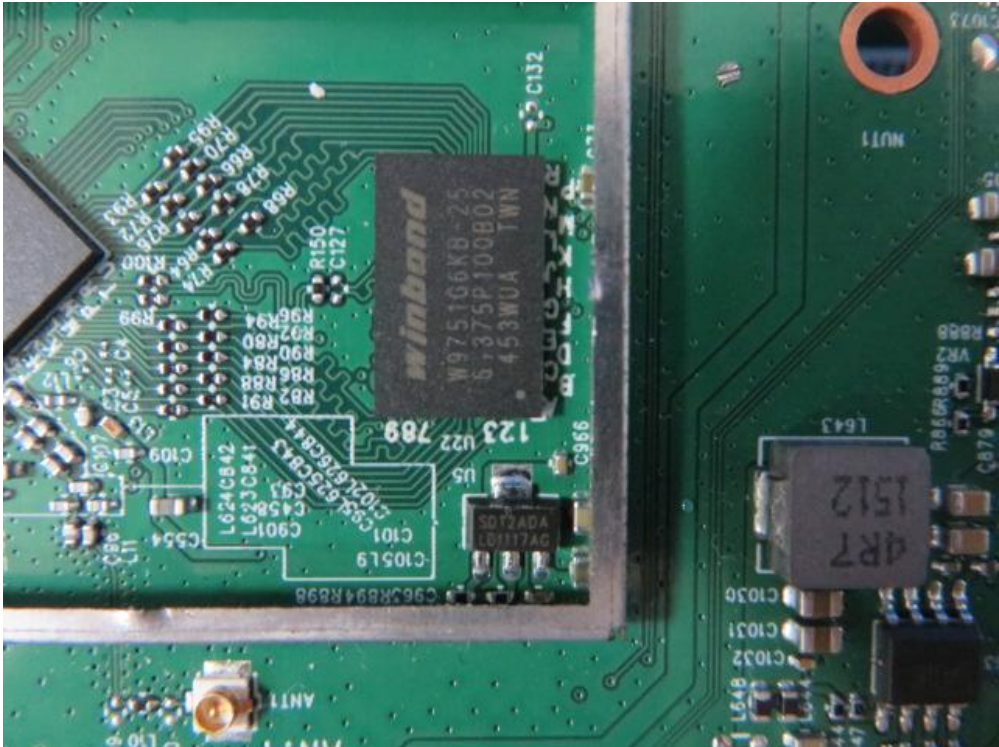
(32) EUT Photo (WHD0110(RoHS))
