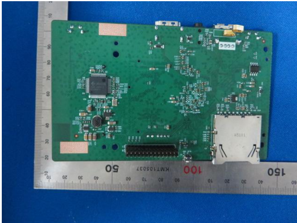
(43) EUT Photo (WHD0111(RoHS))
