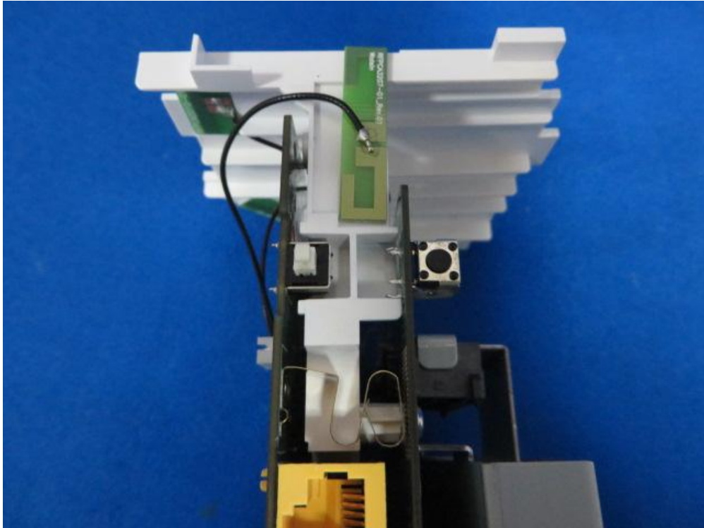
(16) EUT Photo (WHD0110(RoHS))
