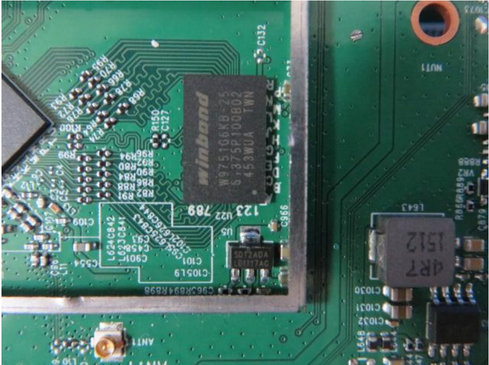
(51) EUT Photo (WHD0111(RoHS))
