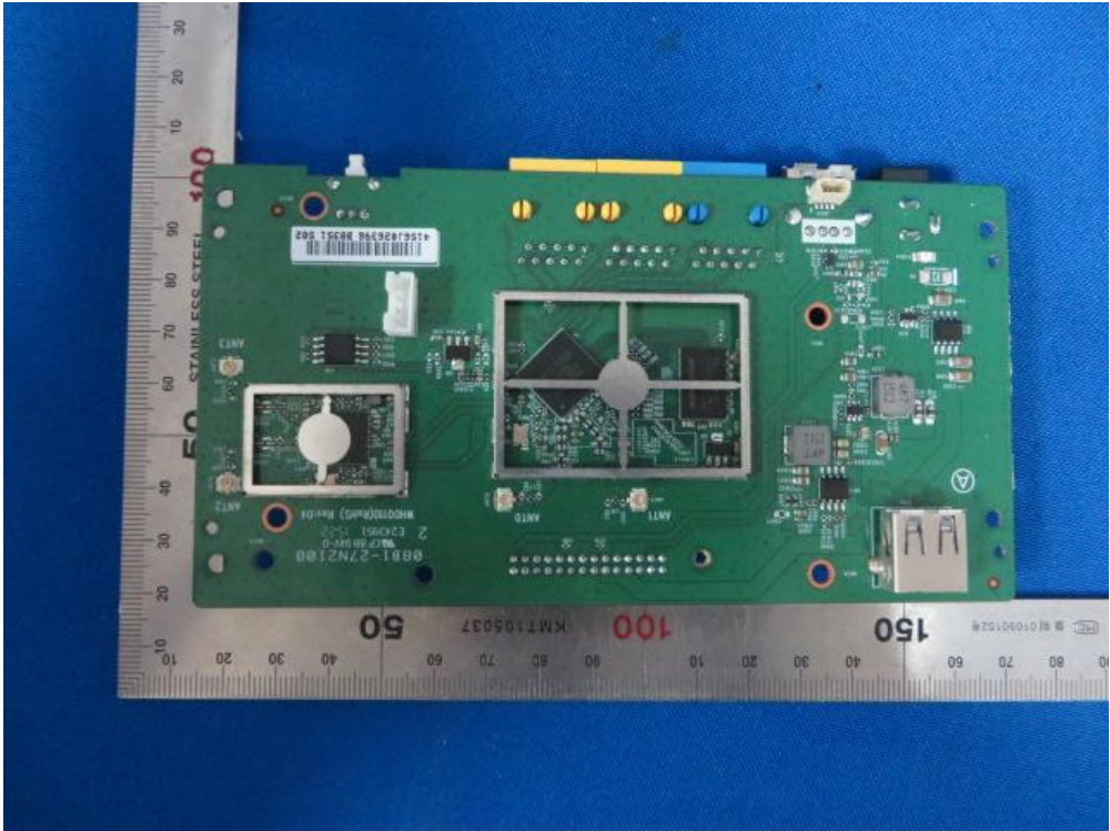
(46) EUT Photo (WHD0111(RoHS))
