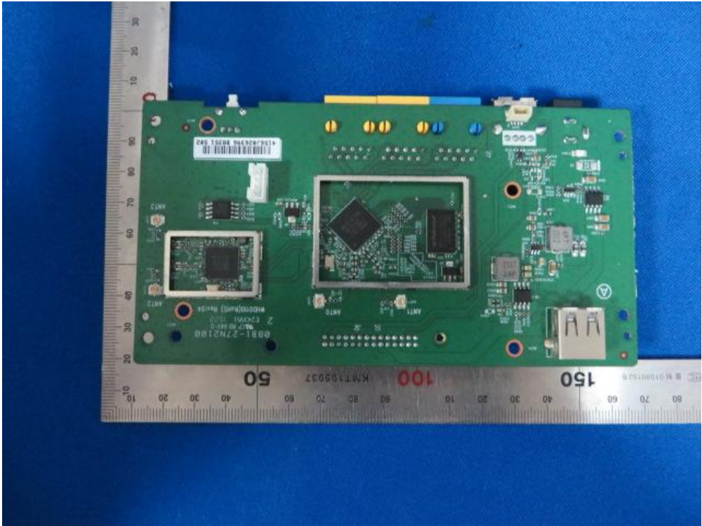
(28) EUT Photo (WHD0110(RoHS))
