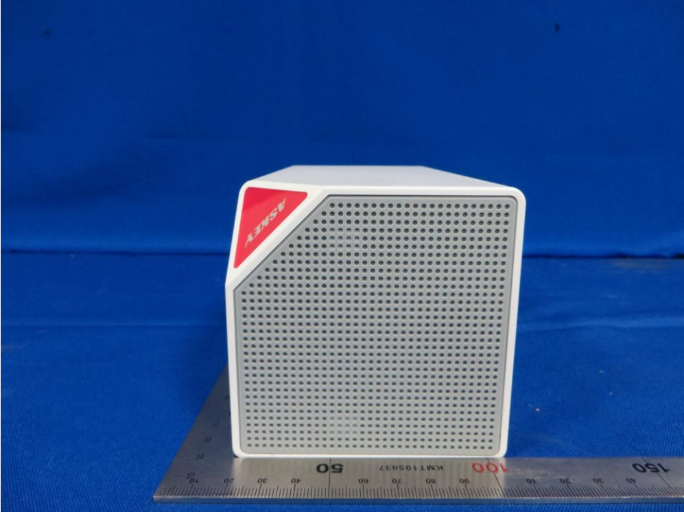
(12) EUT Photo (WHD0111(RoHS))
