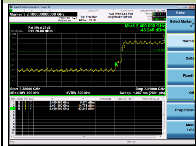
Channel 00 (2402MHz)
