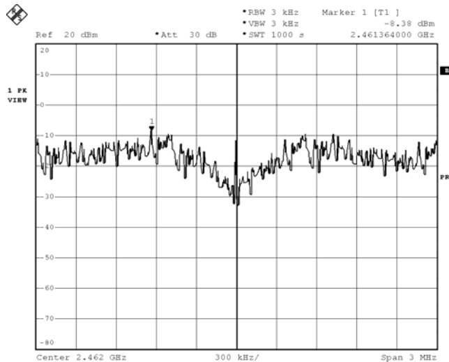
Figure Channel 11: 11Mbps
