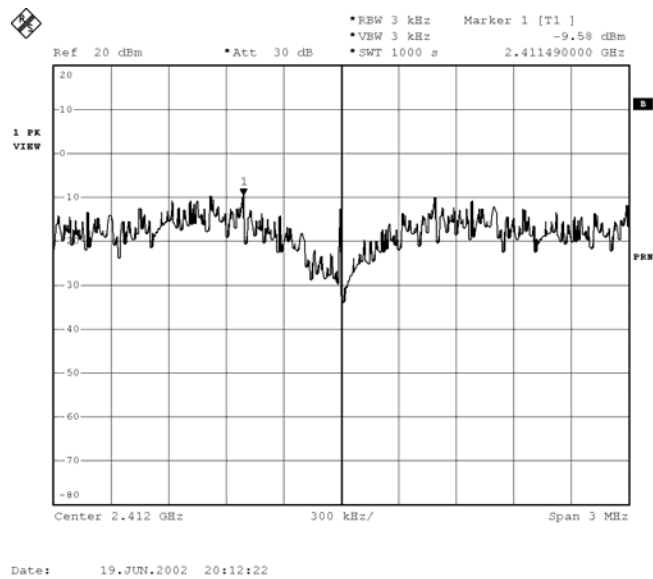
Figure Channel 1: 11Mbps
