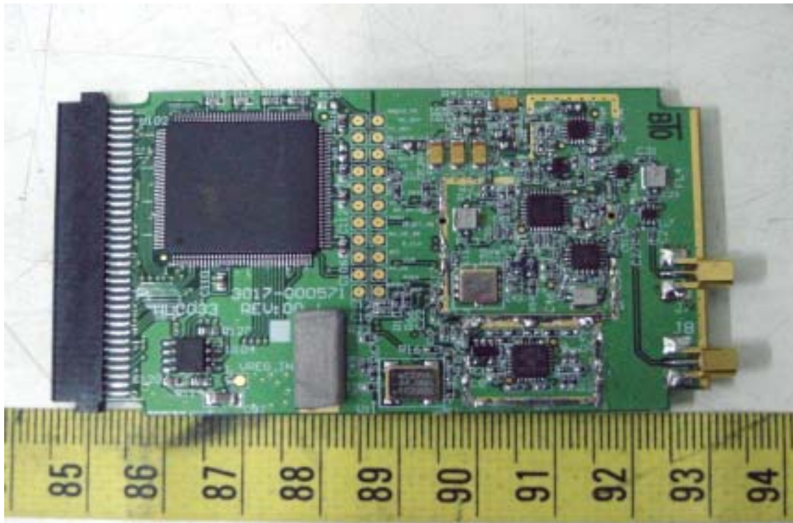
Component View of RF Module
