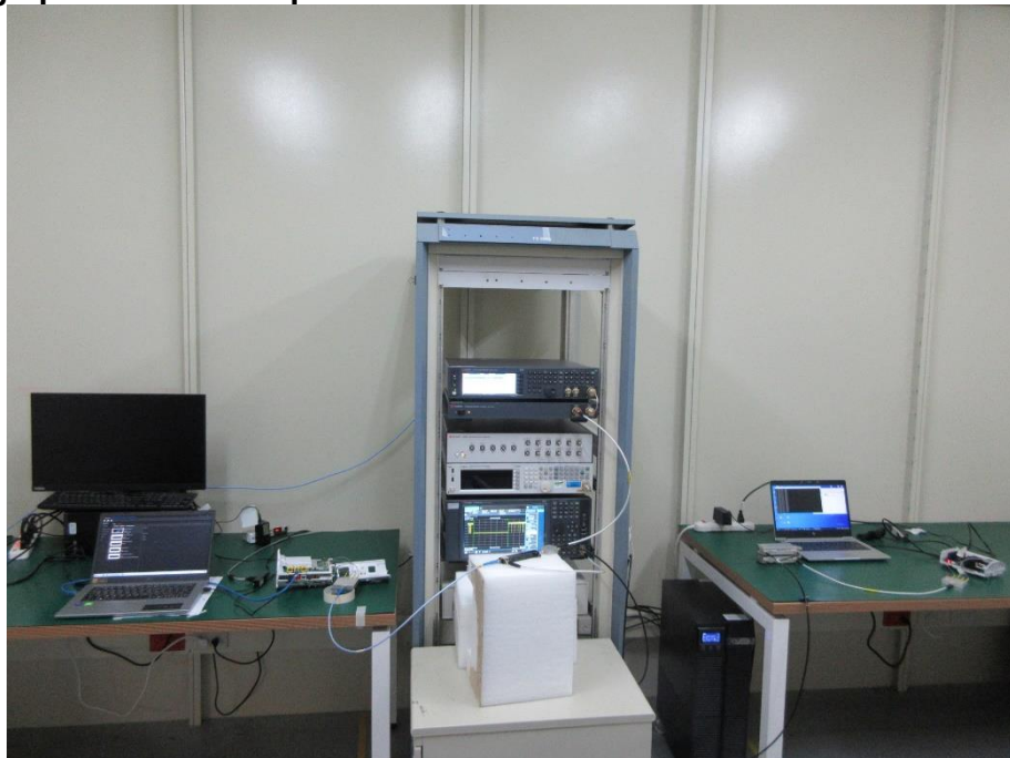
Photograph 10: Test Setup for CBP
