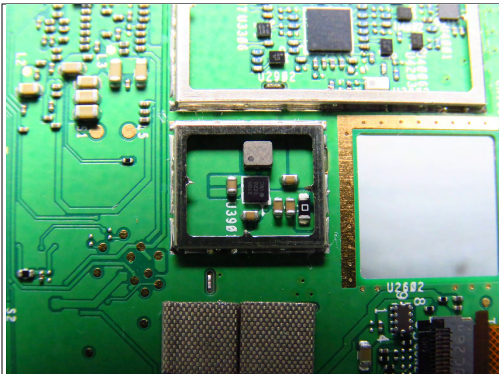
Chip: WCN3660B
