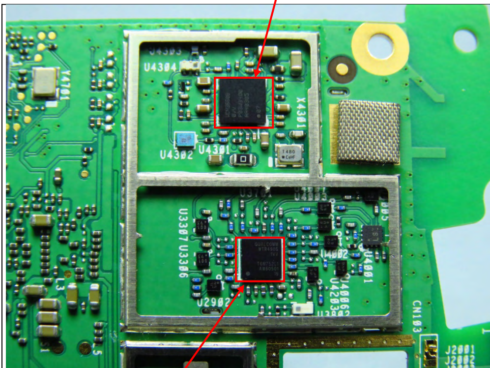
Chip: WTR4905
