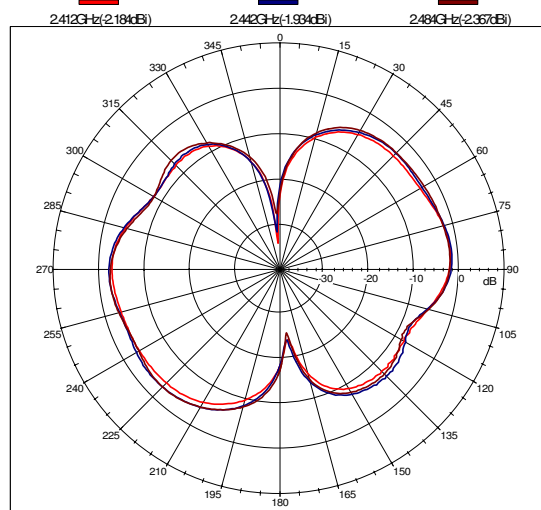
Far-field amplitude of S-ant1-H.nsi
