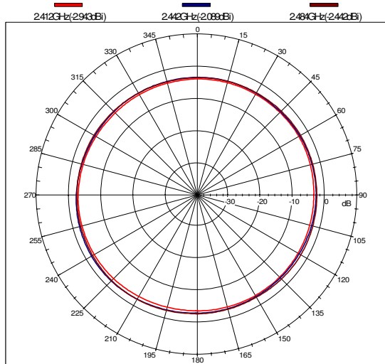
Far-field amplitude of S-ant1-V.nsi
