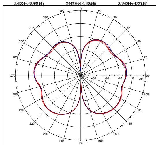
Far-field amplitude of S-ant2-H.nsi
