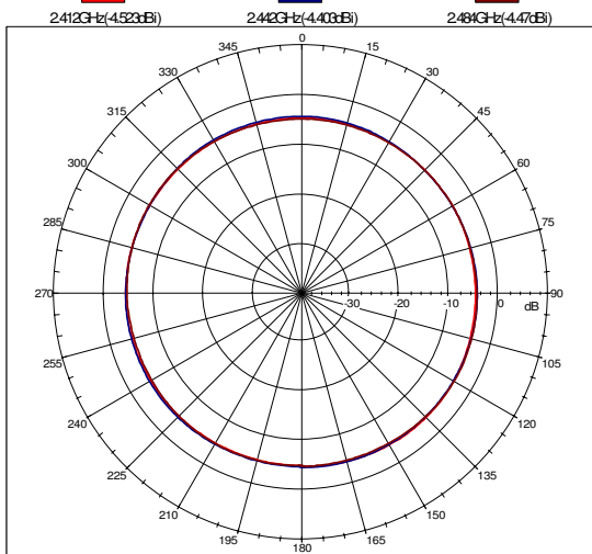
Far-field amplitude of S-ant2-V.nsi
