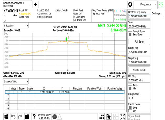
802.11a_20MHz_Chain3_5745MHz
