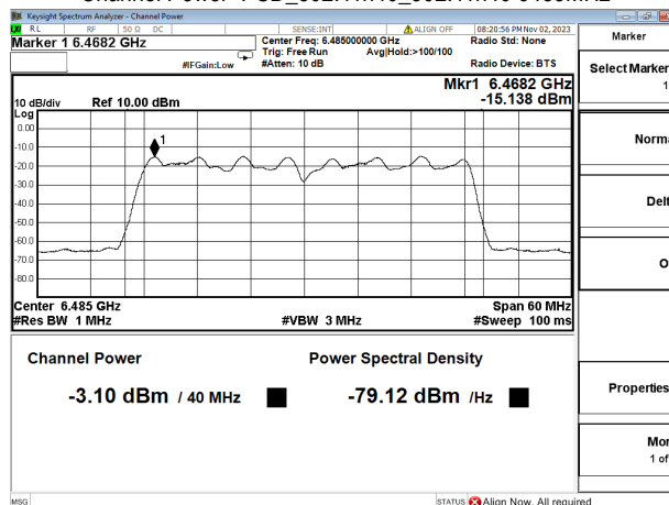
Channel Power+PSD_802.11n40_802.11n40 6485MHz
