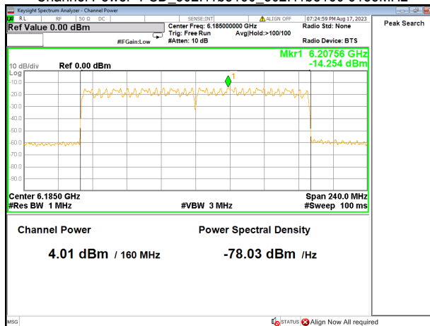
Channel Power+PSD_802.11be160_802.11be160 6185MHz
