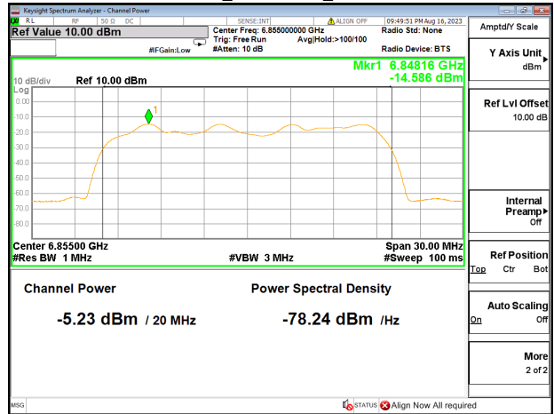
Channel Power+PSD_802.11be20_802.11be20_6855MHz
