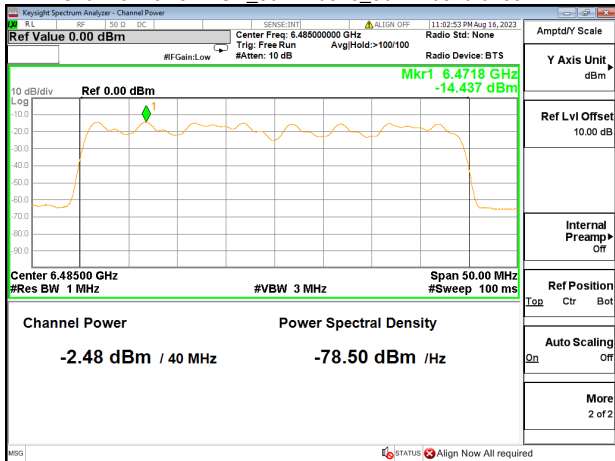
Channel Power+PSD_802.11be40_802.11be40_6485MHz
