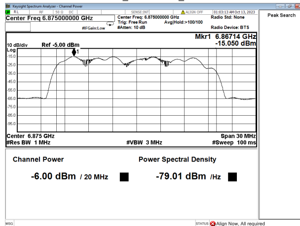
Channel Power+PSD_802.11be20_802.11be20 6875MHz
