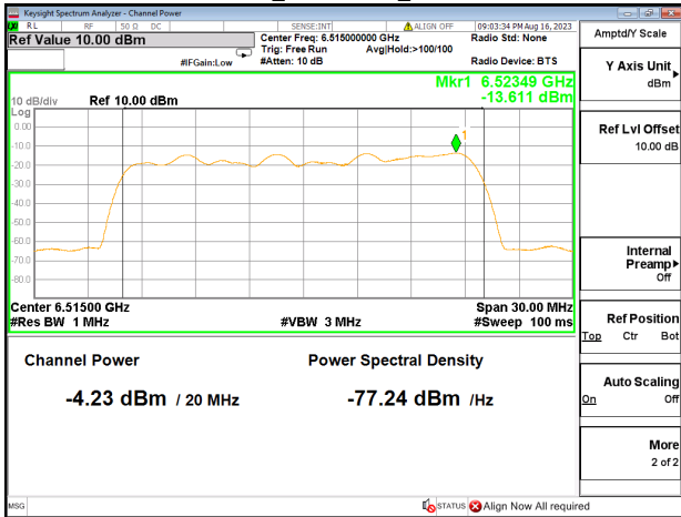
Channel Power+PSD_802.11be20_802.11be20_6515MHz
