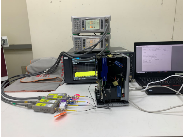
Part_15.407_5G_CDD_Conducted_Setup
