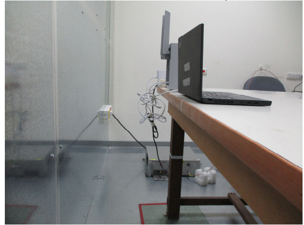
Part_15.407_6E_Conduction_Setup
