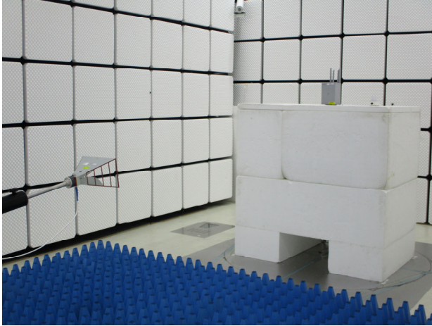
Part_15.247_2.4G_Beamforming_Radiated_Setup
