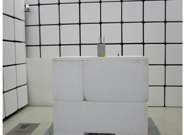
Part_15.407_6E_CDD_Radiated_Setup
