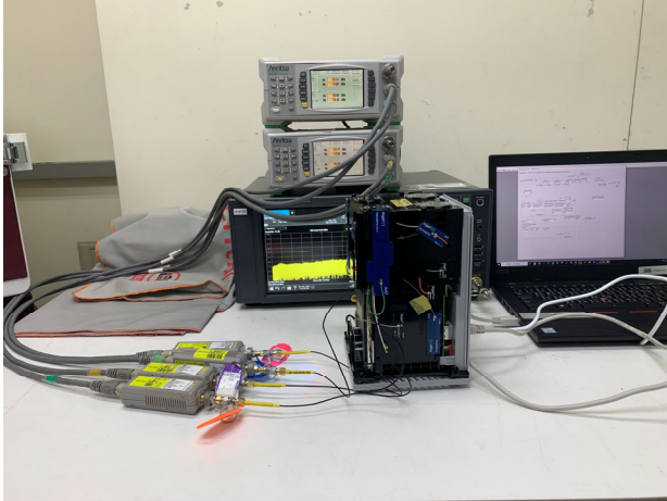
Part_15.407_5G_Normal_DFS_Master_Setup
