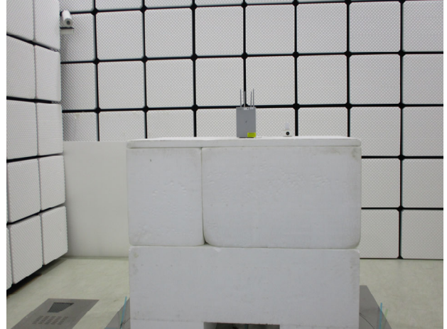
Part_15.407_6E_CDD_Radiated_Setup
