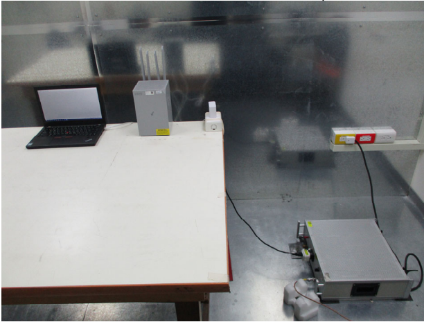
Part_15.247_2.4G_Conduction_Setup
