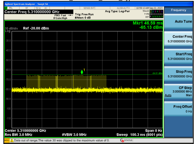
EHT40_5310MHz_Radar_Type 1-B
