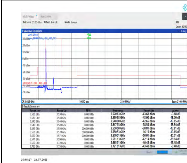
1-N48-PC3-30-20-L-4-CP-QPSK-Edge_1RB_Left-1@0-Ant3-1--PASS-see graph
