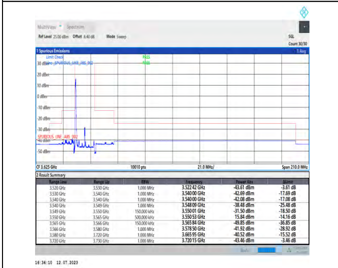
1-N48-PC3-30-15-L-4-CP-QPSK-Edge_1RB_Left-1@0-Ant3-1--PASS-see graph
