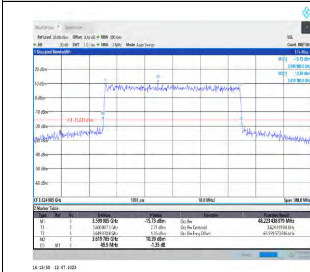
1-N48-PC3-30-50-M-7-CP-16QAM-Outer_Full-133@ 0-Ant3-48.223-49.900-≤50-PASS
