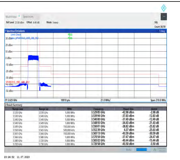
1-N48-PC3-30-15-L-3-DFT-PI2BPSK-Outer_Full-36@0Ant3-1--PASS-see graph
