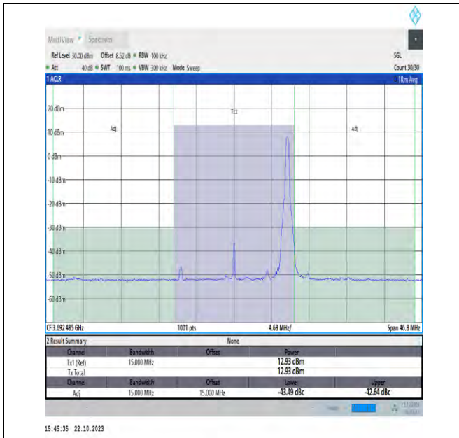
NTV_N48_PC3_30_15_H_TID17_#1_-15_15
