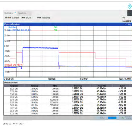
1-N48-PC3-30-60-L-3-DFT-PI2BPSK-Outer_Full-16 2@0-Ant3-1--PASS-see graph
