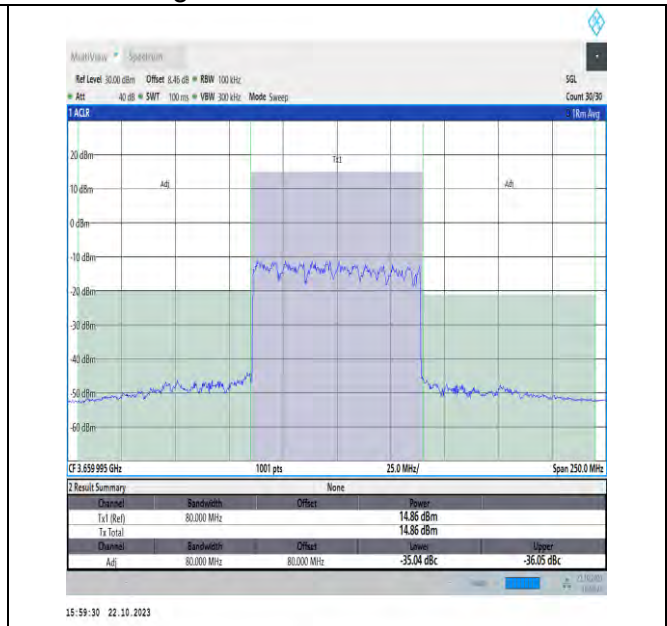
NTV_N48_PC3_30_80_H_TID1_#1_-80_80
