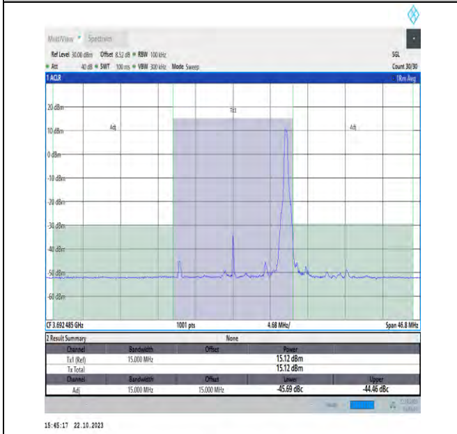
NTV_N48_PC3_30_15_H_TID3_#1_-15_15
