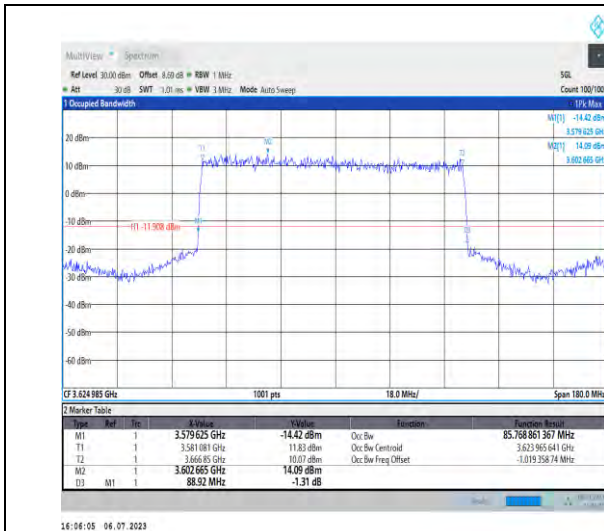
1-N48-PC3-30-90-M-2-DFT-PI2BPSK-Outer_Full-24 @0-Ant3-85.769-88.920-≤90-PASS
