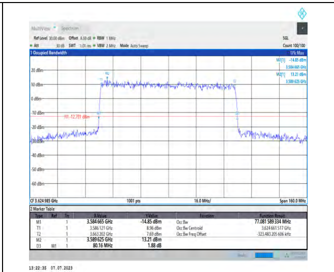
1-N48-PC3-30-80-M-4-DFT-64QAM-Outer_Full-100 @0-Ant3-77.082-80.160-≤80-PASS
