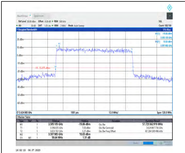
1-N48-PC3-30-60-M-8-CP-64QAM-Outer_Full-162 @0-Ant3-57.726-59.640-≤60-PASS
