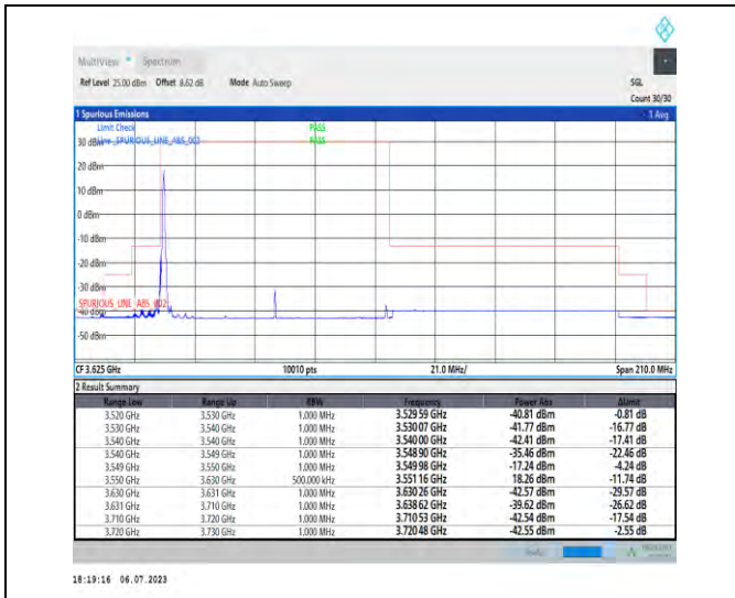
1-N48-PC3-30-80-L-1-DFT-PI2BPSK-Edge_1RB_Left -1@0-Ant3-1--PASS-see graph
