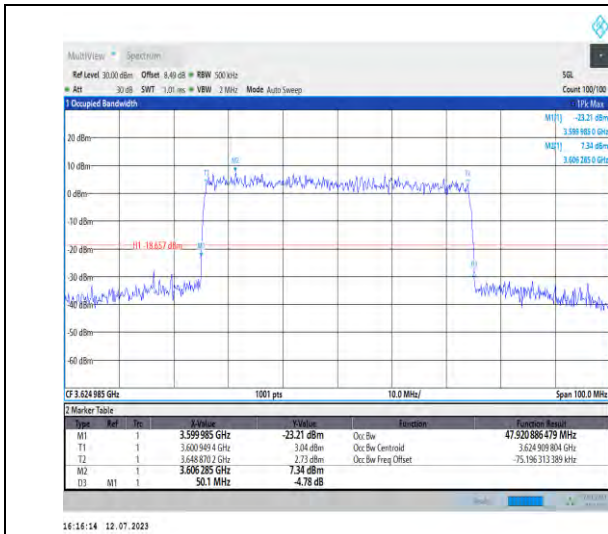
1-N48-PC3-30-50-M-9-CP-256QAM-Outer_Full-133 @0-Ant3-47.921-50.100-≤50-PASS
