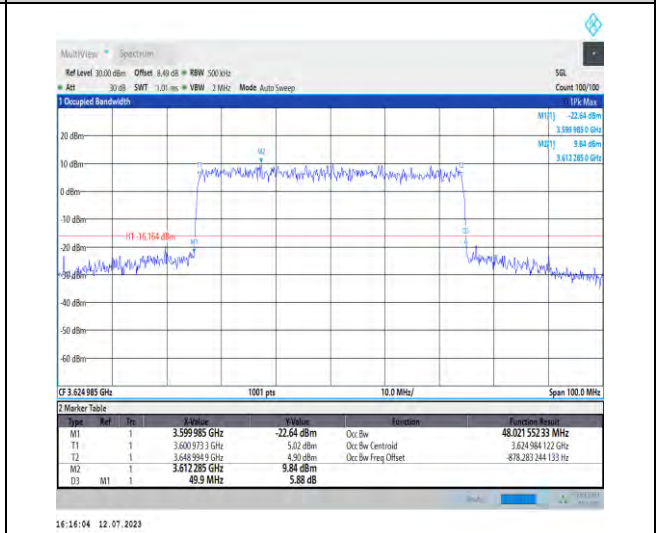
1-N48-PC3-30-50-M-8-CP-64QAM-Outer_Full-133 @0-Ant3-48.022-49.900-≤50-PASS
