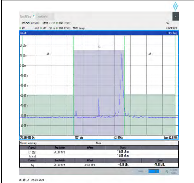
NTNV_N48_PC3_30_20_H_TID3_#1_-20_20
