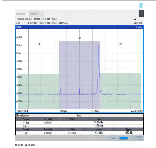
NTV_N48_PC3_30_40_H_TID3_#1_-40_40
