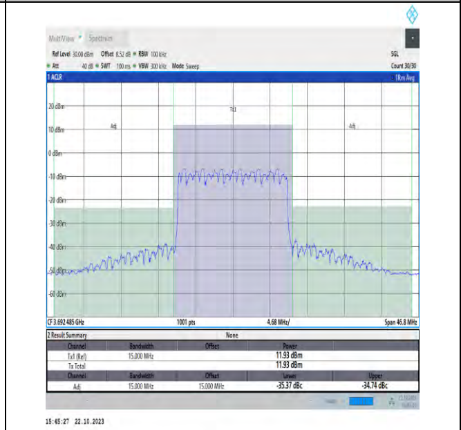
NTV_N48_PC3_30_15_H_TID16_#1_-15_15
