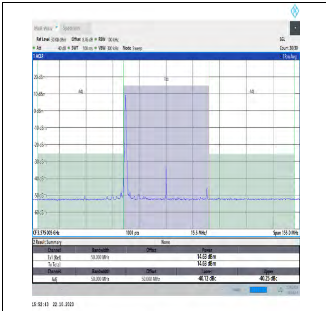
NTNV_N48_PC3_30_50_L_TID17_#1_-50_50
