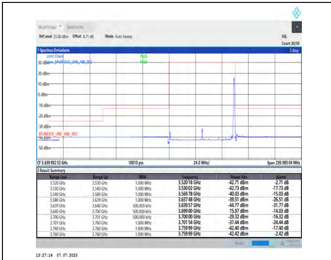
1-N48-PC3-30-60-H-2-DFT-PI2BPSK-Edge_1RB_Right t-1@161-Ant3-1--PASS-see graph
