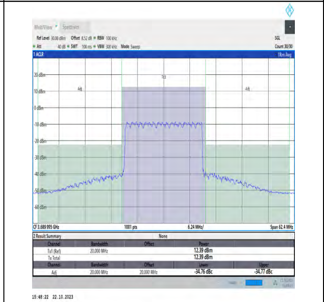
NTNV_N48_PC3_30_20_H_TID16_#1_-20_20
