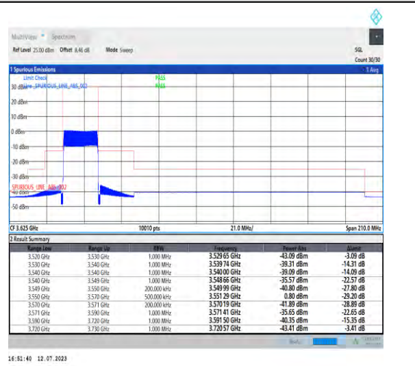
1-N48-PC3-30-20-L-6-CP-QPSK-Outer_Full-51@0-Ant3-1--PASS-see graph
