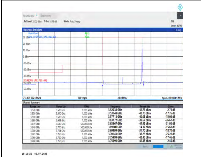
1-N48-PC3-30-60-H-5-CP-QPSK-Edge_1RB_Right-1 @161-Ant3-1--PASS-see graph
