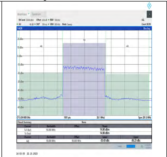
NTV_N48_PC3_30_90_H_TID1_#1_90_90
