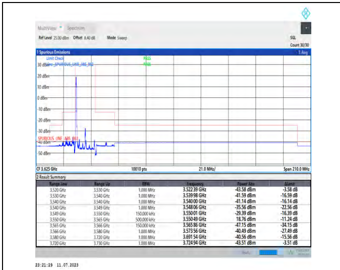
1-N48-PC3-30-15-L-1-DFT-PI2BPSK-Edge_1RB_Left-1@0-Ant3-1--PASS-see graph
