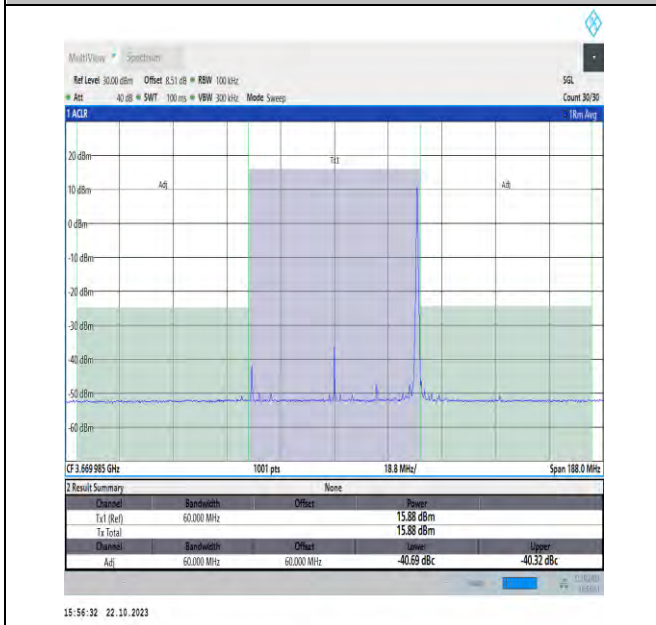
NTNV_N48_PC3_30_60_H_TID3_#1_-60_60
