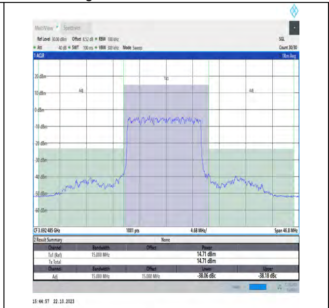
NTV_N48_PC3_30_15_H_TID1_#1_-15_15
