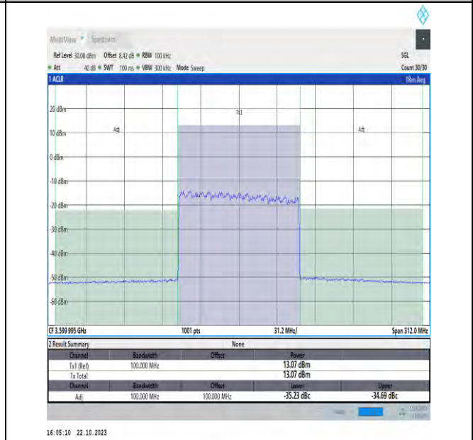
NTNV_N48_PC3_30_100_L_TID16_#1_-100_100
