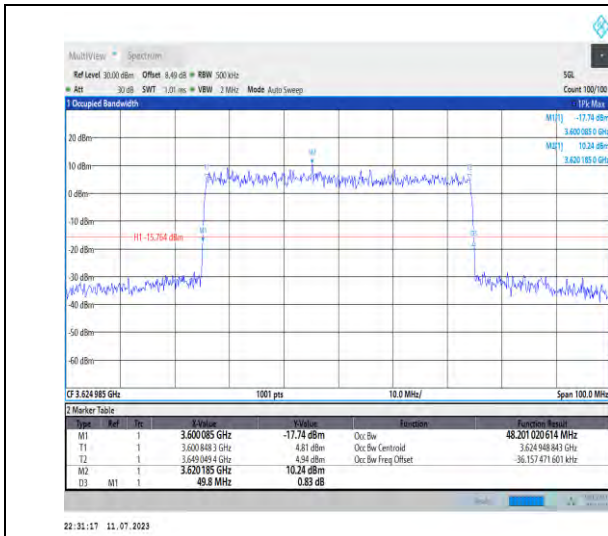
1-N48-PC3-30-50-M-5-DFT-256QAM-Outer_Full-128 @0-Ant3-48.201-49.800-≤50-PASS
