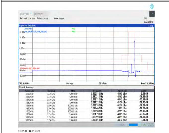
1-N48-PC3-30-10-H-5-CP-QPSK-Edge_1RB_Right-1@23-Ant3-1--PASS-see graph
