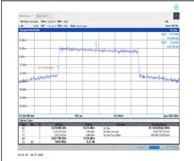
1-N48-PC3-30-100-M-7-CP-16QAM-Outer_Full-273 @0-Ant3-97.127-100.800-≤100-PASS
