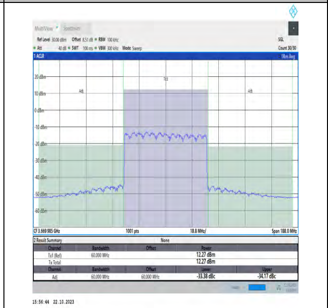
NTNV_N48_PC3_30_60_H_TID16_#1_-60_60
