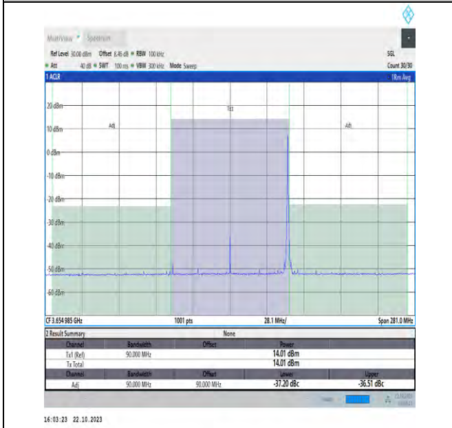
NTV_N48_PC3_30_90_H_TID3_#1_90_90
