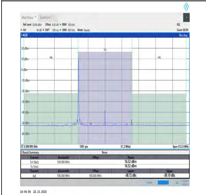
NTNV_N48_PC3_30_100_L_TID2_#1_-100_100
