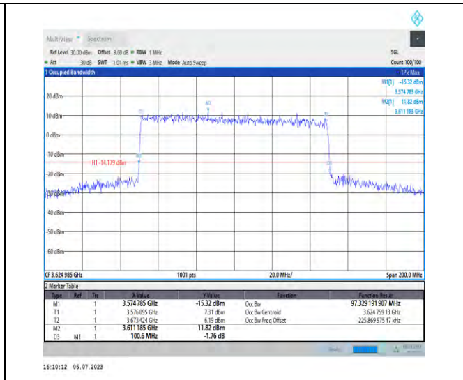
1-N48-PC3-30-100-M-6-CP-QPSK-Outer_Full-273@ 0-Ant3-97.329-100.600-≤100-PASS
