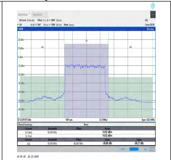
NTV_N48_PC3_30_40_H_TID1_#1_-40_40
