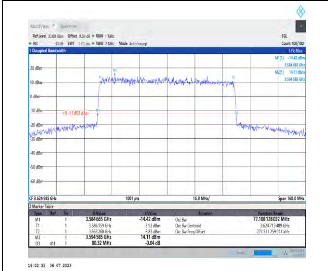
1-N48-PC3-30-80-M-1-DFT-QPSK-Outer_Full-100 @0-Ant3-77.108-80.320-≤80-PASS
