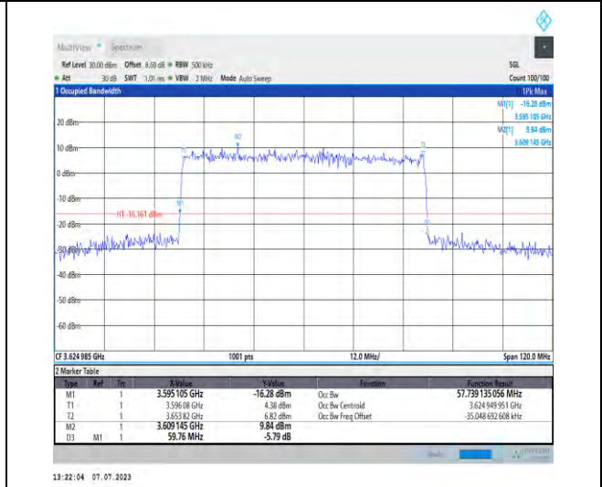
1-N48-PC3-30-60-M-3-DFT-16QAM-Outer_Full-162 @0-Ant3-57.739-59.760-≤60-PASS
