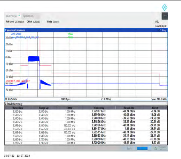
1-N48-PC3-30-15-L-6-CP-QPSK-Outer_Full-38@0-Ant3-1--PASS-see graph
