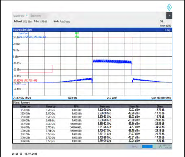
1-N48-PC3-30-60-H-6-CP-QPSK-Outer_Full-162 @0-Ant3-1--PASS-see graph
