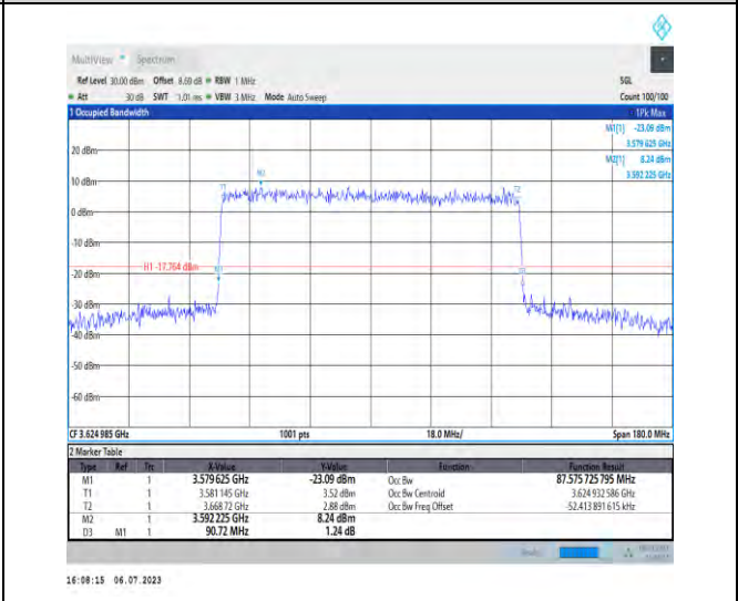
1-N48-PC3-30-90-M-9-CP-256QAM-Outer_Full-245 @0-Ant3-87.576-90.720-≤90-PASS
