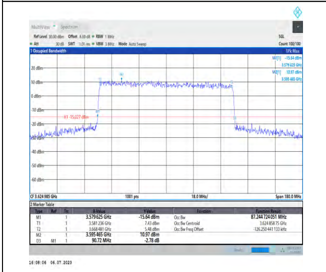
1-N48-PC3-30-90-M-8-CP-64QAM-Outer_Full-245 @0-Ant3-87.245-90.720-≤90-PASS
