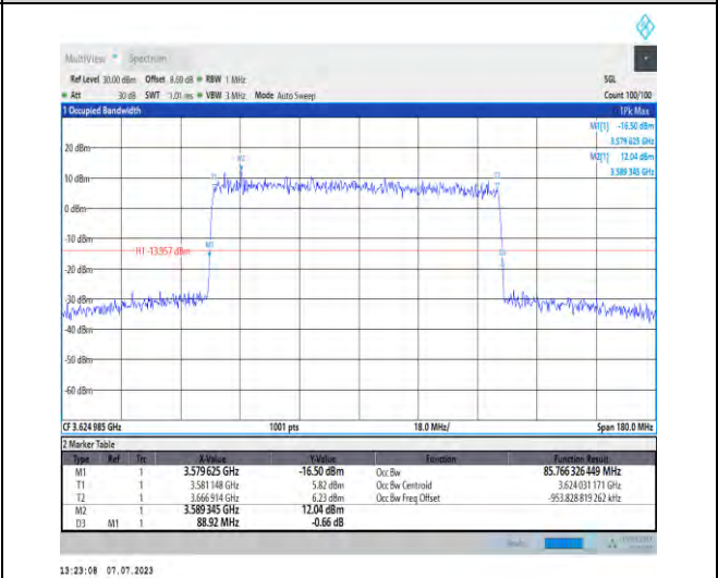
1-N48-PC3-30-90-M-5-DFT-256QAM-Outer_Full-240 @0-Ant3-85.766-88.920-≤90-PASS
