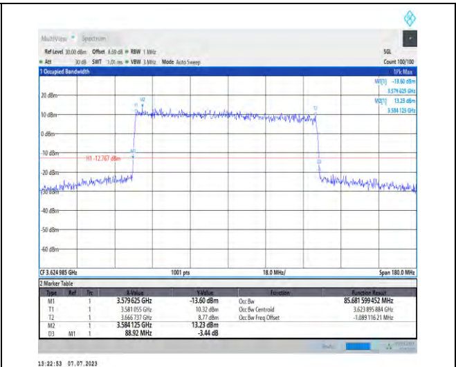
1-N48-PC3-30-90-M-3-DFT-16QAM-Outer_Full-240 @0-Ant3-85.682-88.920-≤90-PASS
