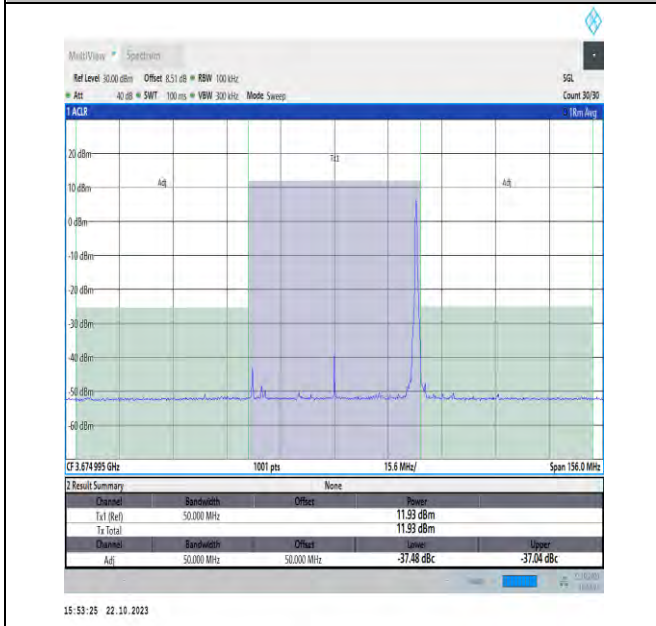
NTVN_N48_PC3_30_50_H_TID3_#1_-50_50
