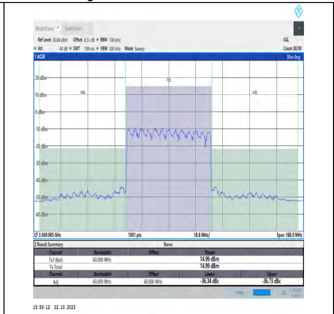
NTNV_N48_PC3_30_60_H_TID1_#1_-60_60
