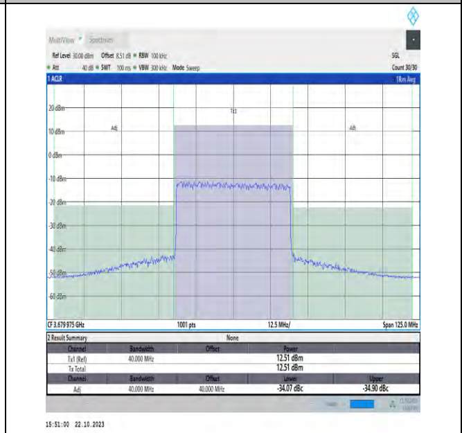
NTV_N48_PC3_30_40_H_TID16_#1_-40_40
