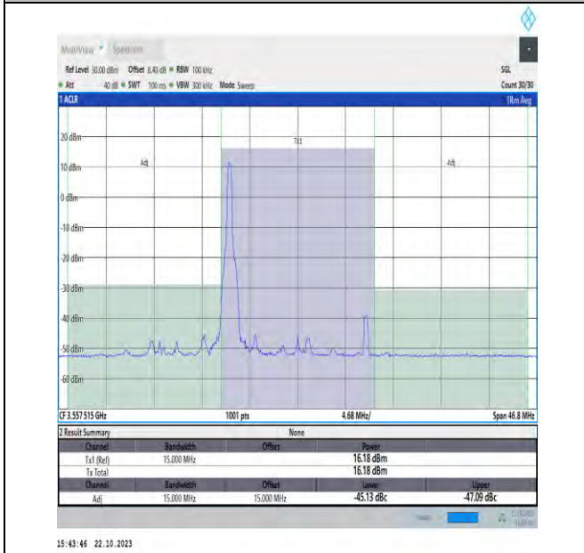
NTV_N48_PC3_30_15_L_TID2_#1_-15_15
