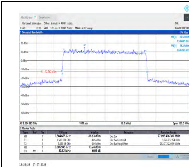
1-N48-PC3-30-80-M-3-DFT-16QAM-Outer_Full-100 @0-Ant3-77.096-80.320-≤80-PASS
