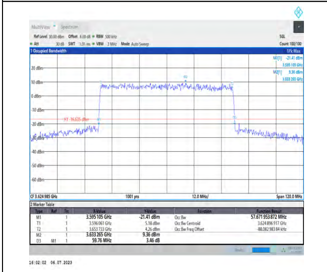
1-N48-PC3-30-60-M-6-CP-QPSK-Outer_Full-162@0 -Ant3-57.672-59.760-≤60-PASS
