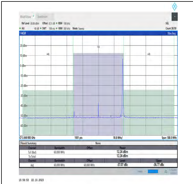
NTNV_N48_PC3_30_60_H_TID18_#1_-60_60
