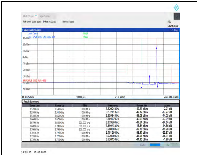
1-N48-PC3-30-20-H-2-DFT-PI2BPSK-Edge_1RB_Right-t-1@50-Ant3-1--PASS-see graph
