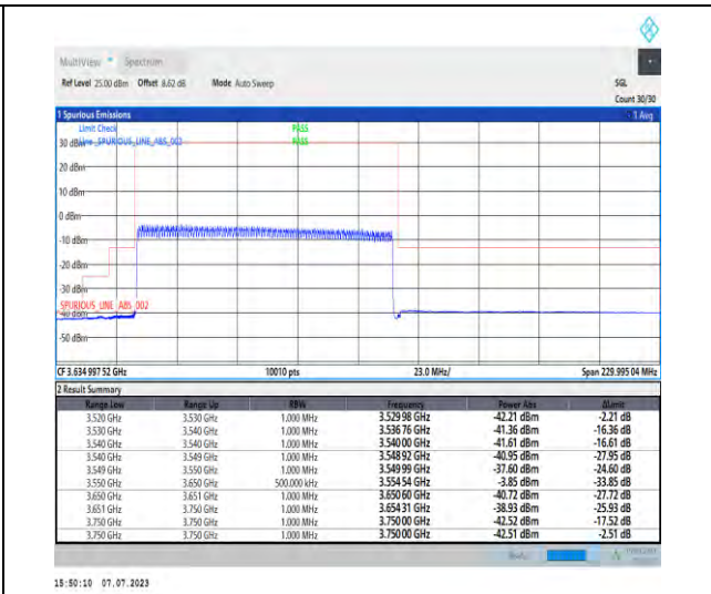
1-N48-PC3-30-100-L-3-DFT-PI2BPSK-Outer_Full-5 1@0-Ant3-1--PASS-see graph
