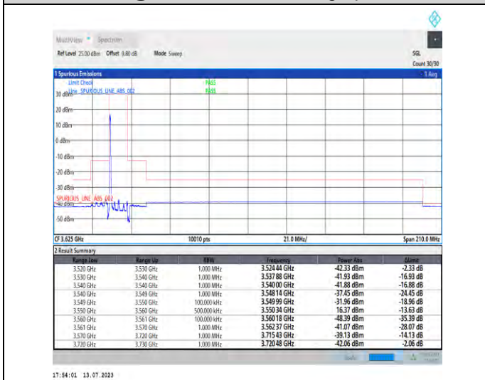
1-N48-PC3-30-10-L-4-CP-QPSK-Edge_1RB_Left-1@0-Ant3-1--PASS-see graph
