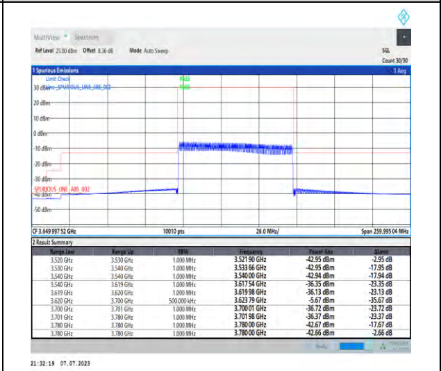
1-N48-PC3-30-80-H-6-CP-QPSK-Outer_Full-217@0-Ant3-1--PASS-see graph
