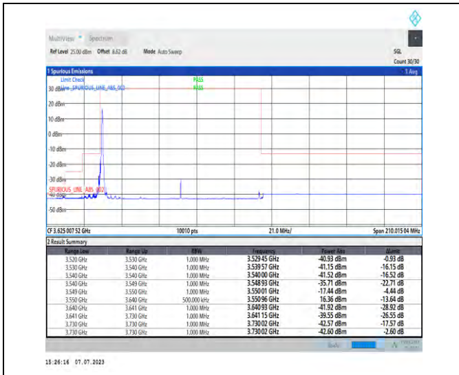
1-N48-PC3-30-90-L-1-DFT-PI2BPSK-Edge_1RB_Left -1@0-Ant3-1--PASS-see graph
