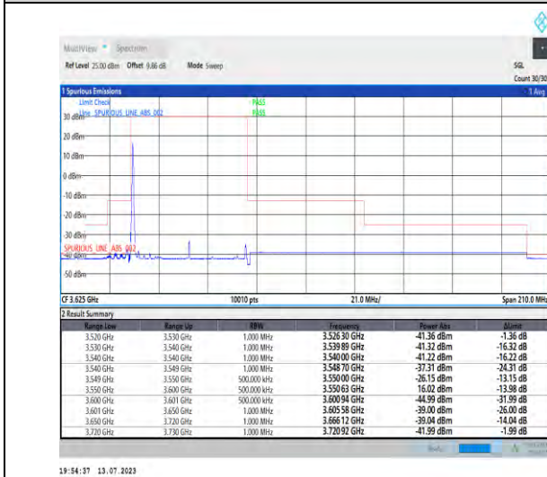
1-N48-PC3-30-50-L-4-CP-QPSK-Edge_1RB_Left-1@ 0-Ant3-1--PASS-see graph
