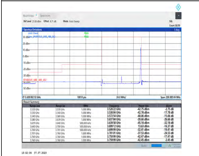
1-N48-PC3-30-60-H-5-CP-QPSK-Edge_1RB_Right-1@161-Ant3-1--PASS-see graph
