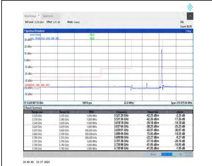
1-N48-PC3-30-40-H-5-CP-QPSK-Edge_1RB_Right-1 @105-Ant3-1--PASS-see graph
