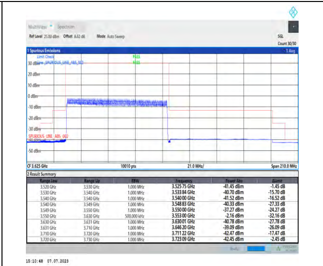
1-N48-PC3-30-80-L-3-DFT-PI2BPSK-Outer_Full-10 0@0-Ant3-1--PASS-see graph
