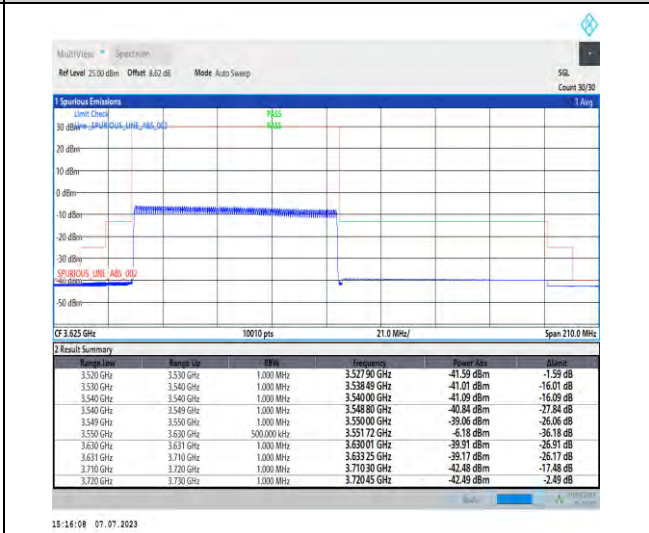
1-N48-PC3-30-80-L-6-CP-QPSK-Outer_Full-217@ 0-Ant3-1--PASS-see graph
