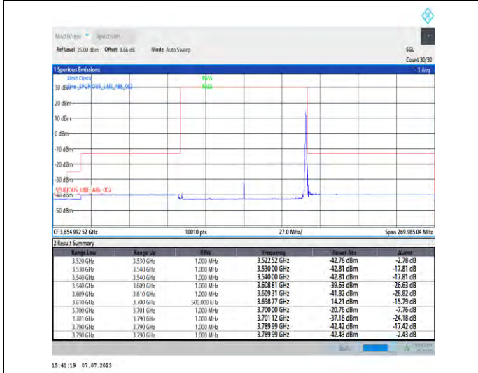
1-N48-PC3-30-90-H-5-CP-QPSK-Edge_1RB_Right-1@244-Ant3-1--PASS-see graph
