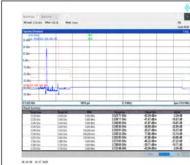
1-N48-PC3-30-15-L-1-DFT-PI2BPSK-Edge_1RB_Left-1@0-Ant3-1--PASS-see graph
