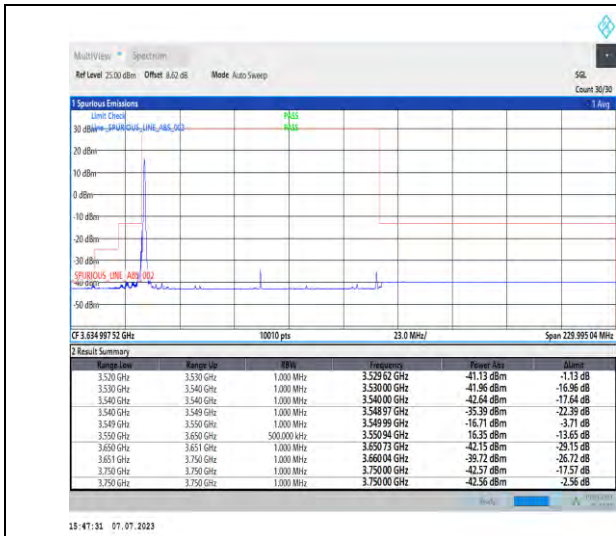
1-N48-PC3-30-100-L-1-DFT-PI2BPSK-Edge_1RB_Lef t-1@0-Ant3-1--PASS-see graph
