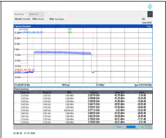
1-N48-PC3-30-90-L-3-DFT-PI2BPSK-Outer_Full-24 0@0-Ant3-1--PASS-see graph
