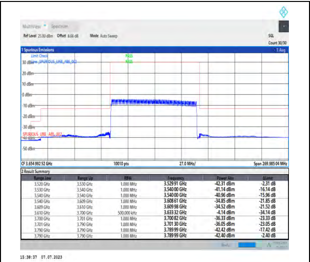
1-N48-PC3-30-90-H-3-DFT-PI2BPSK-Outer_Full-240@0-Ant3-1--PASS-see graph
