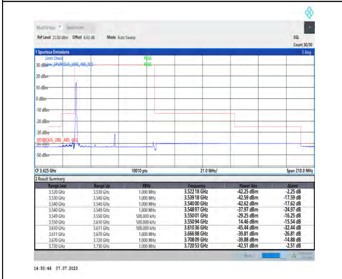
1-N48-PC3-30-60-L-4-CP-QPSK-Edge_1RB_Left-1@ 0-Ant3-1--PASS-see graph
