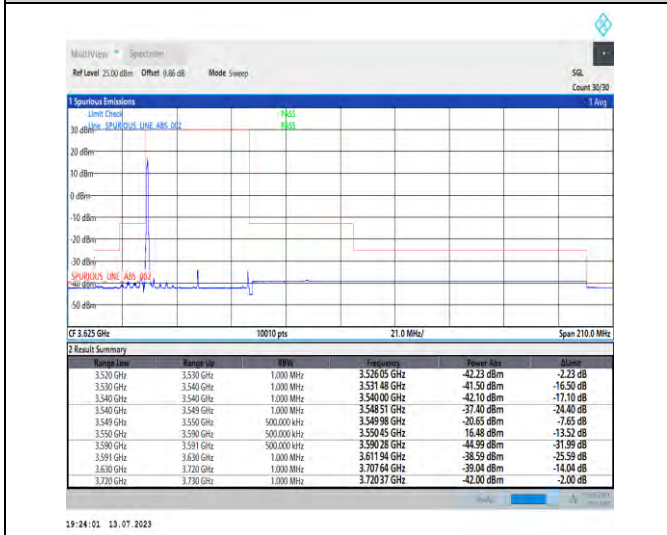
1-N48-PC3-30-40-L-4-CP-QPSK-Edge_1RB_Left-1@ 0-Ant3-1--PASS-see graph
