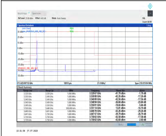
1-N48-PC3-30-90-L-4-CP-QPSK-Edge_1RB_Left-1@ 0-Ant3-1--PASS-see graph
