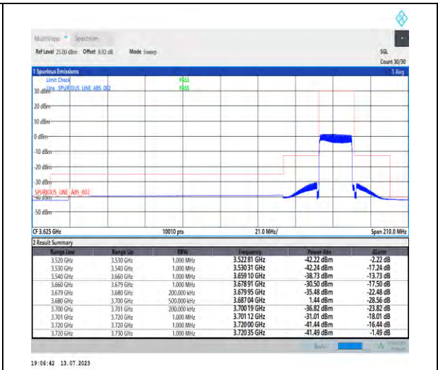
1-N48-PC3-30-20-H-3-DFT-PI2BPSK-Outer_Full-50@0-Ant3-1--PASS-see graph
