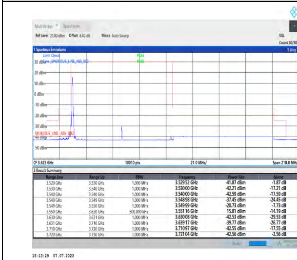
1-N48-PC3-30-80-L-4-CP-QPSK-Edge_1RB_Left-1@ 0-Ant3-1--PASS-see graph
