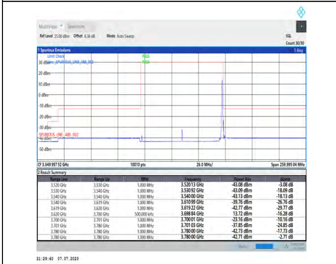
1-N48-PC3-30-80-H-5-CP-QPSK-Edge_1RB_Right-1@216-Ant3-1--PASS-see graph
