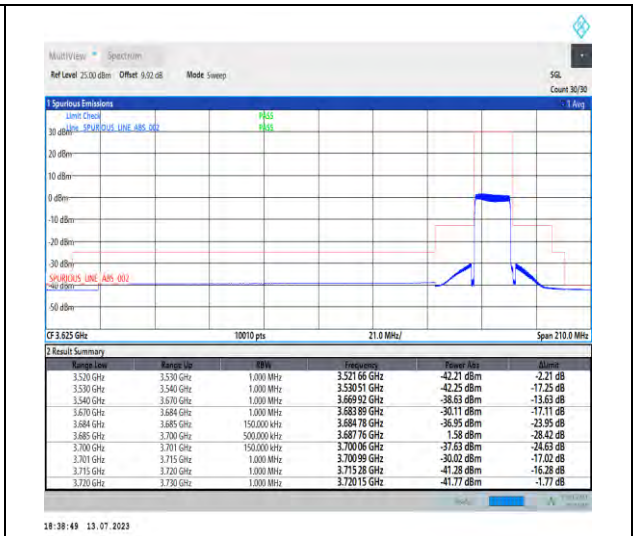
1-N48-PC3-30-15-H-3-DFT-PI2BPSK-Outer_Full-36@0Ant3-1--PASS-see graph
