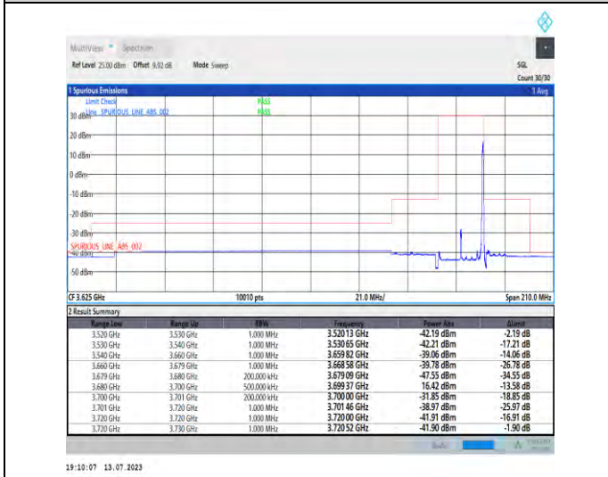
1-N48-PC3-30-20-H-5-CP-QPSK-Edge_1RB_Right-1@50-Ant3-1--PASS-see graph
