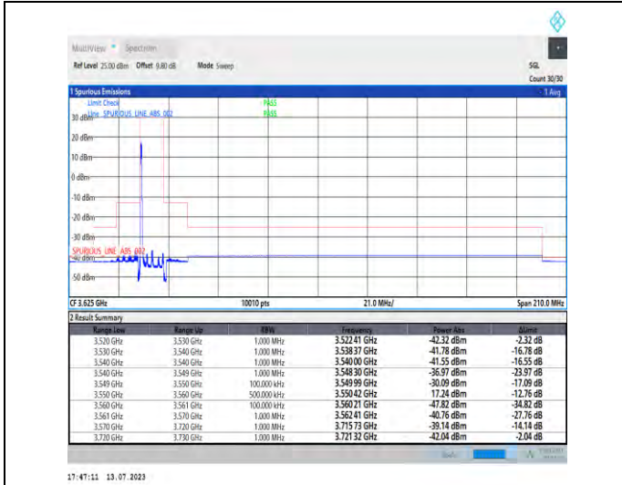
1-N48-PC3-30-10-L-1-DFT-PI2BPSK-Edge_1RB_Left-1@0-Ant3-1--PASS-see graph
