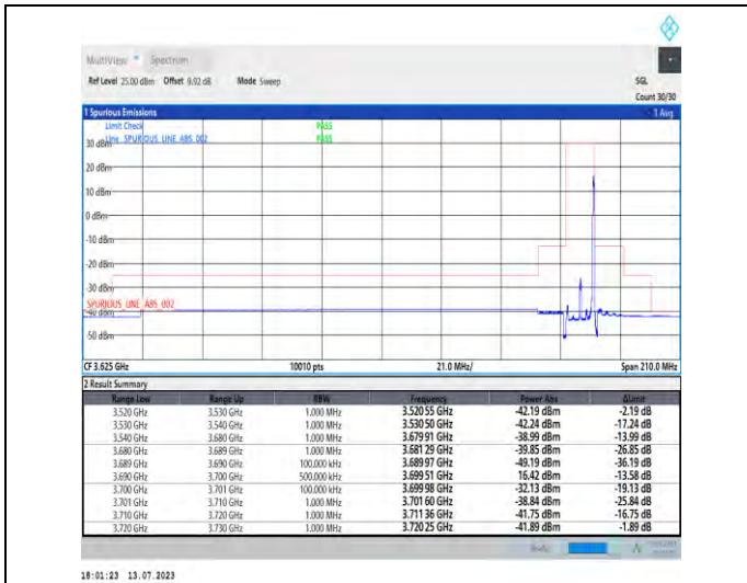
1-N48-PC3-30-10-H-2-DFT-PI2BPSK-Edge_1RB_Right-t-1@23-Ant3-1--PASS-see graph
