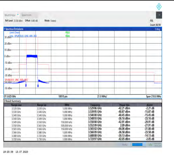
1-N48-PC3-30-15-L-6-CP-QPSK-Outer_Full-38@0-Ant3-1--PASS-see graph
