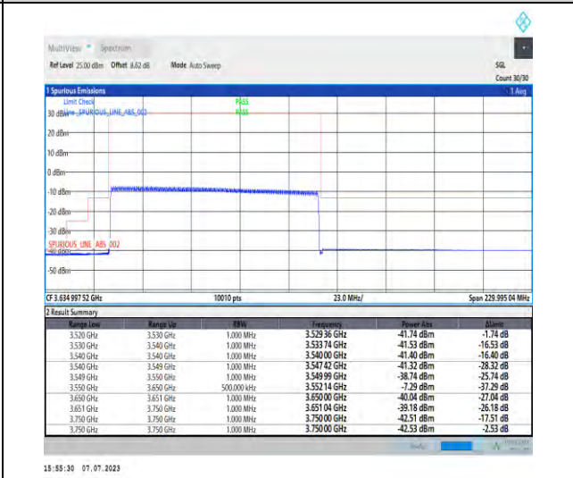
1-N48-PC3-30-100-L-6-CP-QPSK-Outer_Full-273 @0-Ant3-1--PASS-see graph
