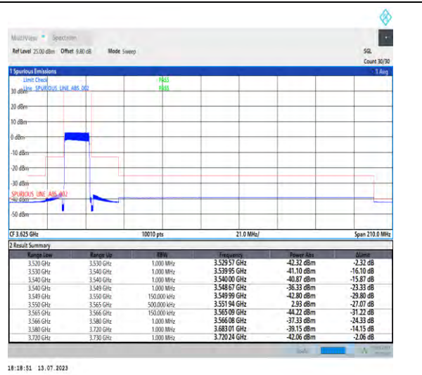
1-N48-PC3-30-15-L-3-DFT-PI2BPSK-Outer_Full-36@0Ant3-1--PASS-see graph
