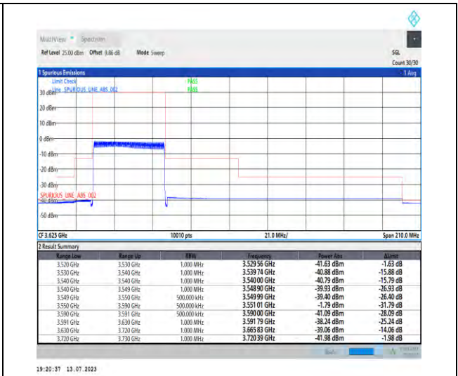
1-N48-PC3-30-40-L-3-DFT-PI2BPSK-Outer_Full-10 0@0-Ant3-1--PASS-see graph
