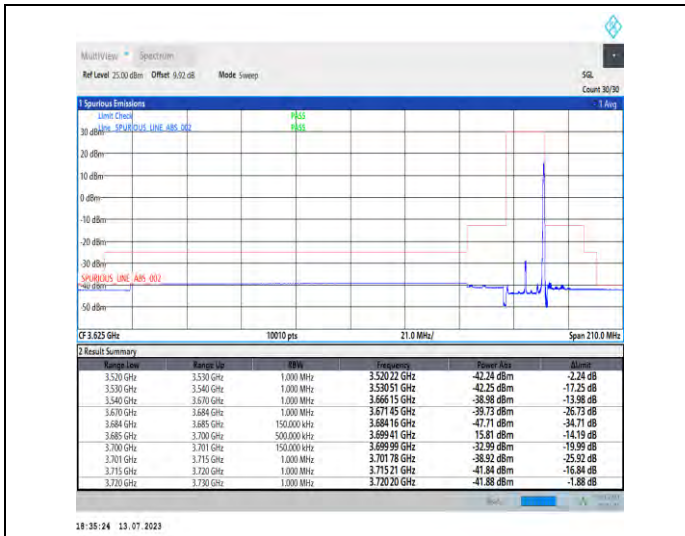
1-N48-PC3-30-15-H-2-DFT-PI2BPSK-Edge_1RB_Right -1@37-Ant3-1--PASS-see graph
