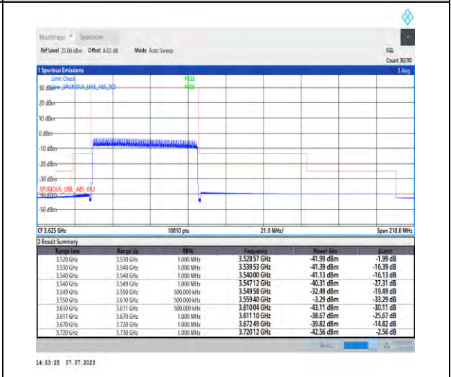
1-N48-PC3-30-60-L-6-CP-QPSK-Outer_Full-162@0 -Ant3-1--PASS-see graph
