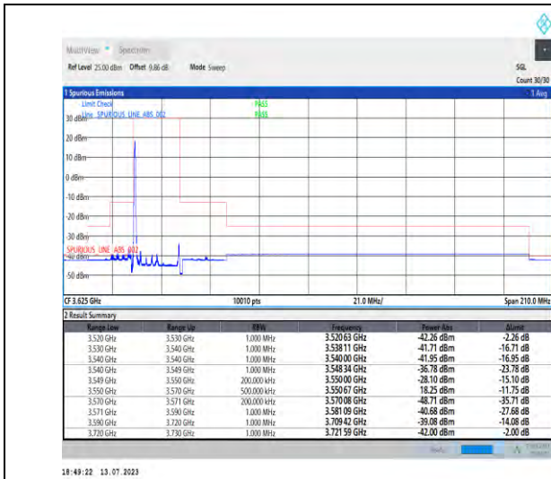
1-N48-PC3-30-20-L-1-DFT-PI2BPSK-Edge_1RB_Left-1@0-Ant3-1--PASS-see graph
