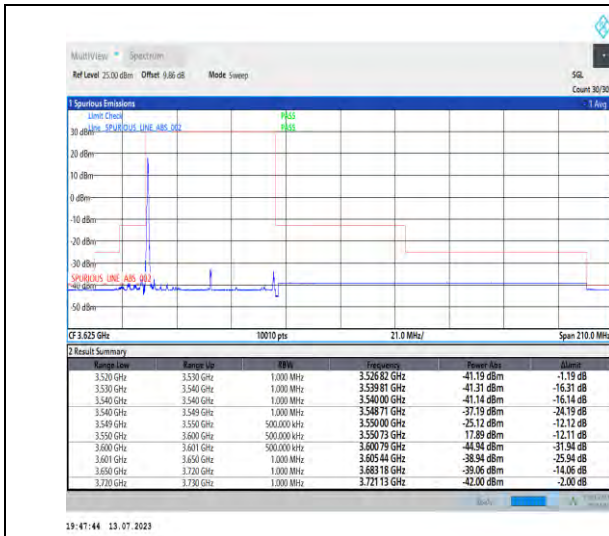
1-N48-PC3-30-50-L-1-DFT-PI2BPSK-Edge_1RB_Left -1@0-Ant3-1--PASS-see graph
