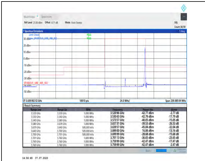
1-N48-PC3-30-60-H-2-DFT-PI2BPSK-Edge_1RB_Right-t-1@161-Ant3-1--PASS-see graph
