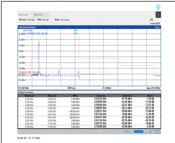
1-N48-PC3-30-60-L-1-DFT-PI2BPSK-Edge_1RB_Left -1@0-Ant3-1--PASS-see graph
