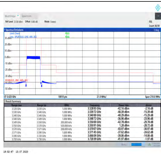
1-N48-PC3-30-20-L-3-DFT-PI2BPSK-Outer_Full-50@0-Ant3-1--PASS-see graph
