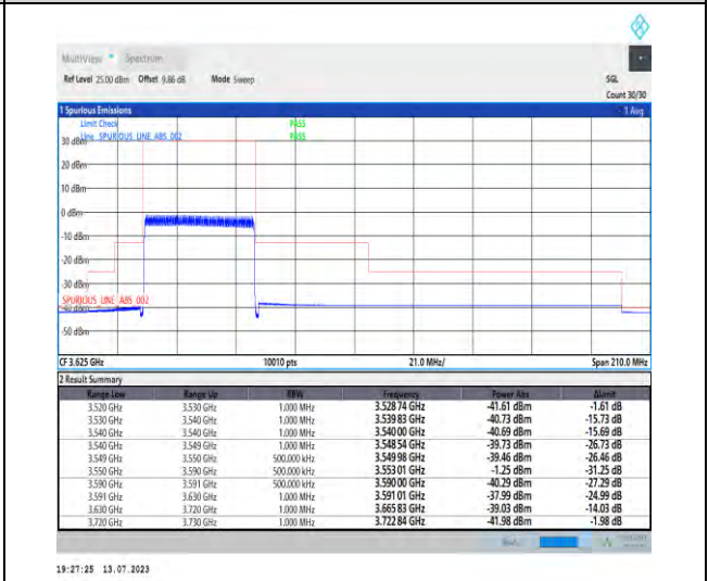
1-N48-PC3-30-40-L-6-CP-QPSK-Outer_Full-106@0 -Ant3-1--PASS-see graph
