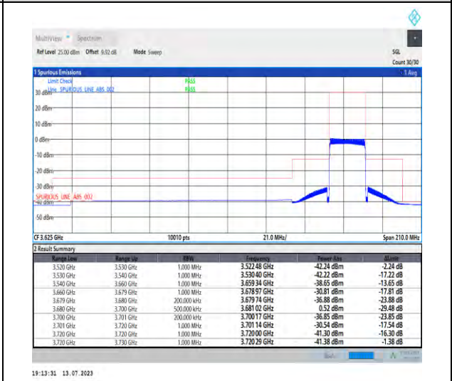
1-N48-PC3-30-20-H-6-CP-QPSK-Outer_Full-51@0-Ant3-1--PASS-see graph
