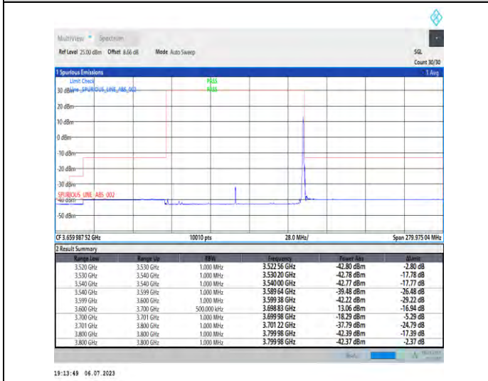
1-N48-PC3-30-100-H-5-CP-QPSK-Edge_1RB_Right-1 @272-Ant3-1--PASS-see graph
