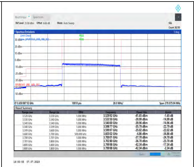
1-N48-PC3-30-100-H-3-DFT-PI2BPSK-Outer_Full -51@0-Ant3-1--PASS-see graph
