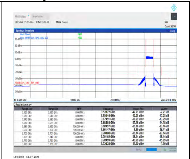
1-N48-PC3-30-10-H-3-DFT-PI2BPSK-Outer_Full-2-4@0-Ant3-1--PASS-see graph
