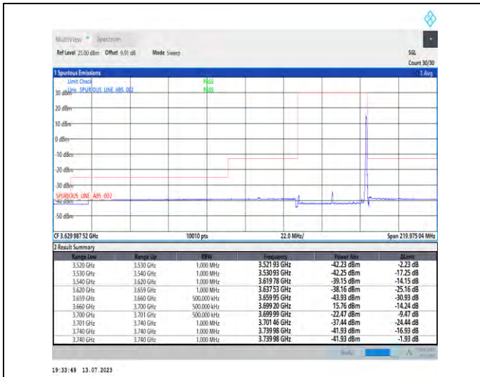
1-N48-PC3-30-40-H-2-DFT-PI2BPSK-Edge_1RB_Right t-1@105-Ant3-1--PASS-see graph
