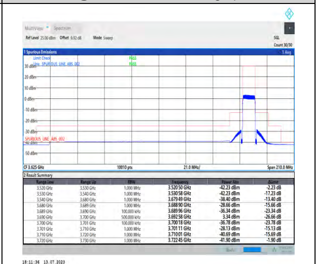
1-N48-PC3-30-10-H-6-CP-QPSK-Outer_Full-24@0-Ant3-1--PASS-see graph
