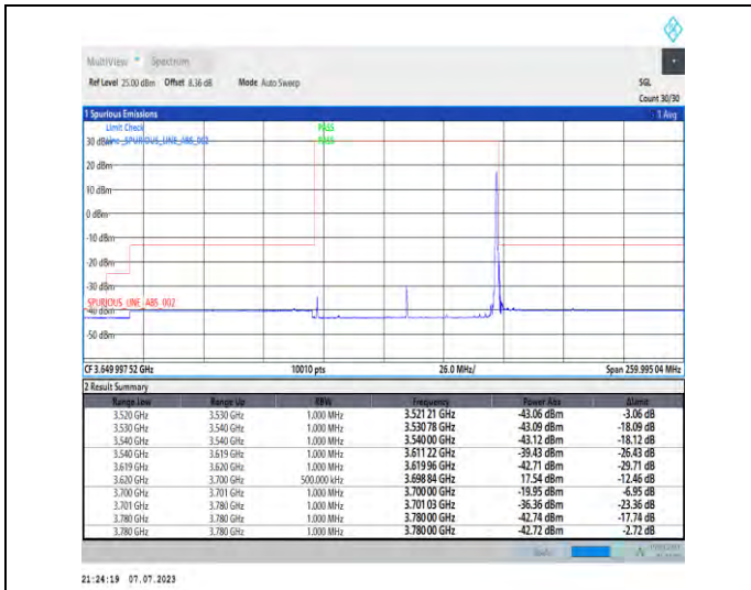
1-N48-PC3-30-80-H-2-DFT-PI2BPSK-Edge_1RB_Right-t-1@216-Ant3-1--PASS-see graph
