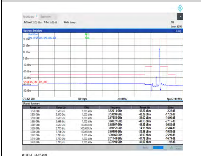
1-N48-PC3-30-10-H-5-CP-QPSK-Edge_1RB_Right-1@23-Ant3-1--PASS-see graph
