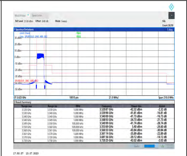
1-N48-PC3-30-10-L-3-DFT-PI2BPSK-Outer_Full-24@0-Ant3-1--PASS-see graph
