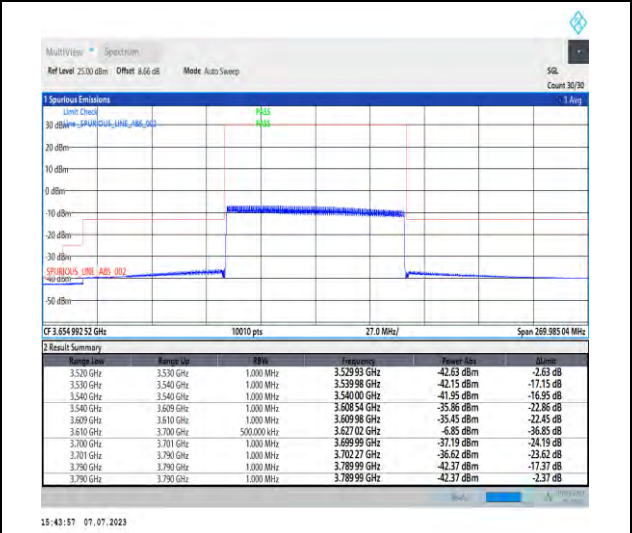
1-N48-PC3-30-90-H-6-CP-QPSK-Outer_Full-245@0-Ant3-1--PASS-see graph
