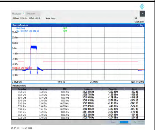
1-N48-PC3-30-10-L-6-CP-QPSK-Outer_Full-24@0-Ant3-1--PASS-see graph
