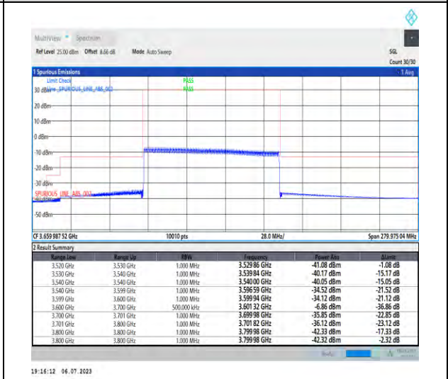
1-N48-PC3-30-100-H-6-CP-QPSK-Outer_Full-273 @0-Ant3-1--PASS-see graph
