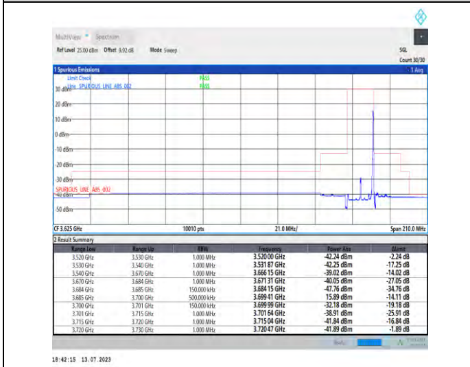
1-N48-PC3-30-15-H-5-CP-QPSK-Edge_1RB_Right-1@37-Ant3-1--PASS-see graph
