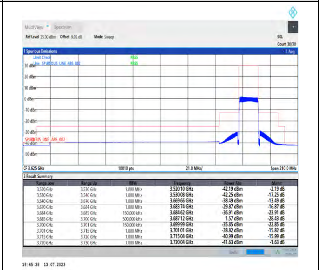
1-N48-PC3-30-15-H-6-CP-QPSK-Outer_Full-38@0-Ant3-1--PASS-see graph
