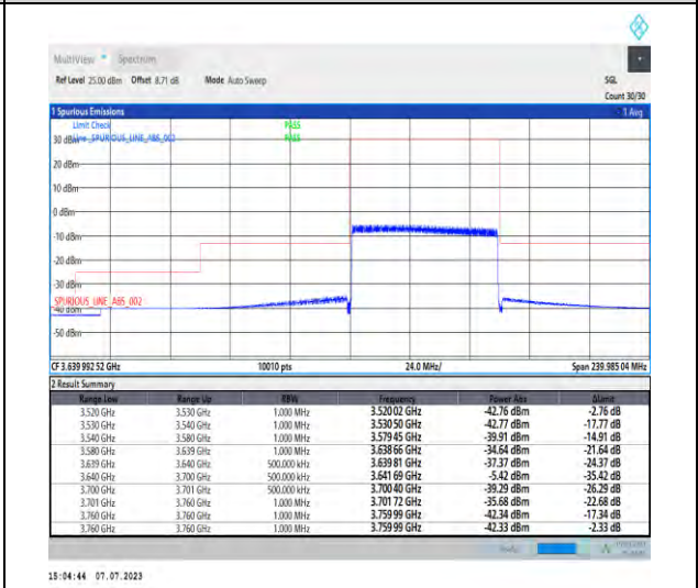
1-N48-PC3-30-60-H-6-CP-QPSK-Outer_Full-162@0-Ant3-1--PASS-see graph
