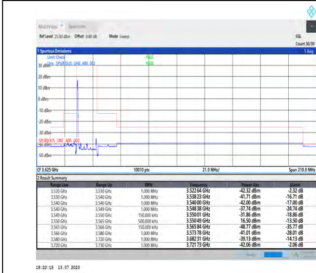
1-N48-PC3-30-15-L-4-CP-QPSK-Edge_1RB_Left-1@0-Ant3-1--PASS-see graph
