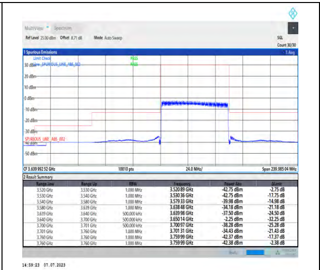
1-N48-PC3-30-60-H-3-DFT-PI2BPSK-Outer_Full-62@0-Ant3-1--PASS-see graph
