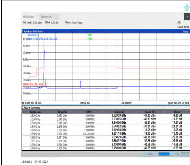
1-N48-PC3-30-100-L-4-CP-QPSK-Edge_1RB_Left-1 @0-Ant3-1--PASS-see graph
