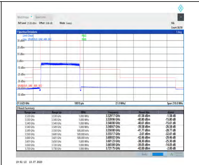
1-N48-PC3-30-50-L-3-DFT-PI2BPSK-Outer_Full-12 8@0-Ant3-1--PASS-see graph
