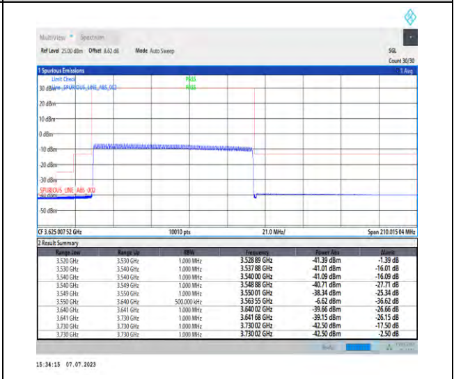
1-N48-PC3-30-90-L-6-CP-QPSK-Outer_Full-245@ 0-Ant3-1--PASS-see graph
