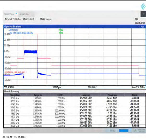
1-N48-PC3-30-20-L-6-CP-QPSK-Outer_Full-51@0-Ant3-1--PASS-see graph
