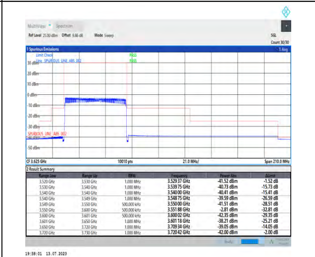
1-N48-PC3-30-50-L-6-CP-QPSK-Outer_Full-133@0 -Ant3-1--PASS-see graph
