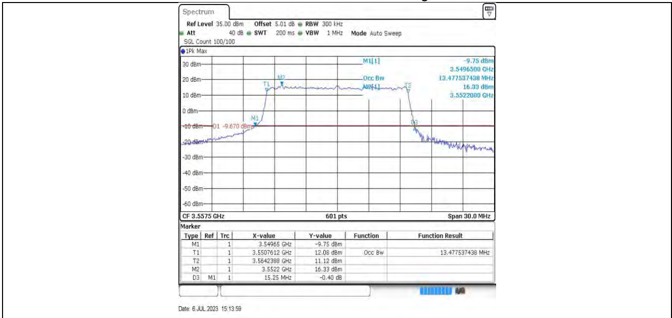
15MHz-55315 64QAM
