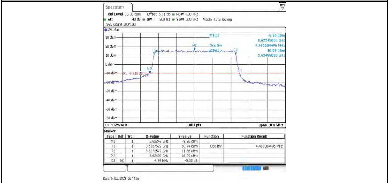
5MHz-55990 QPSK
