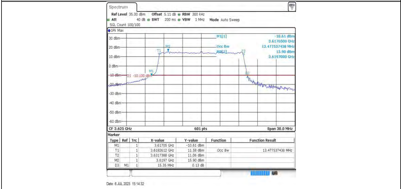
15MHz-55990 64QAM
