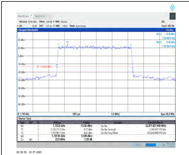
1-N66-PC3-15-25-M-1-DFT-QPSK-Outer_Full-128@ 0-Ant3-22.872-23.900-≤25-PASS
