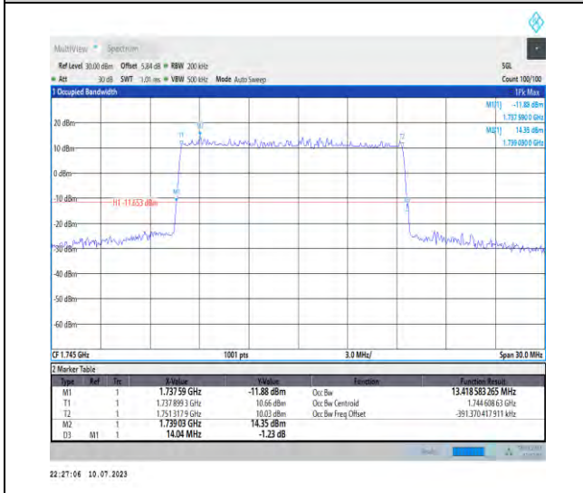
1-N66-PC3-15-15-M-1-DFT-QPSK-Outer_Full-75@ 0-Ant3-13.419-14.040≤15-PASS
