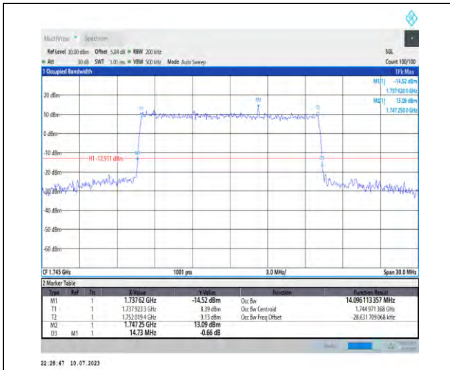
1-N66-PC3-15-15-M-7-CP-16QAM-Outer_Full-79@0 -Ant3-14.096-14.730-≤15-PASS
