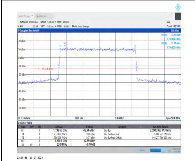
1-N66-PC3-15-25-M-3-DFT-16QAM-Outer_Full-128 @0-Ant3-22.906-23.800-≤25-PASS
