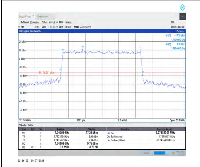
1-N66-PC3-15-10-M-6-CP-QPSK-Outer_Full-52@0- Ant3-9.274-9.800-≤10-PASS
