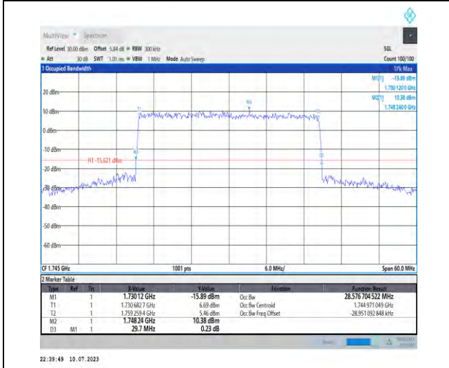
1-N66-PC3-15-30-M-6-CP-QPSK-Outer_Full-160@0 -Ant3-28.577-29.700-≤30-PASS
