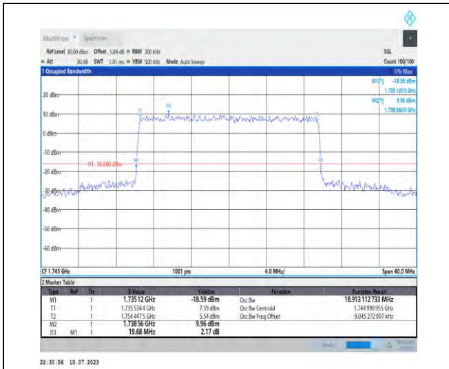
1-N66-PC3-15-20-M-6-CP-QPSK-Outer_Full-106@0 -Ant3-18.913-19.680-≤20-PASS
