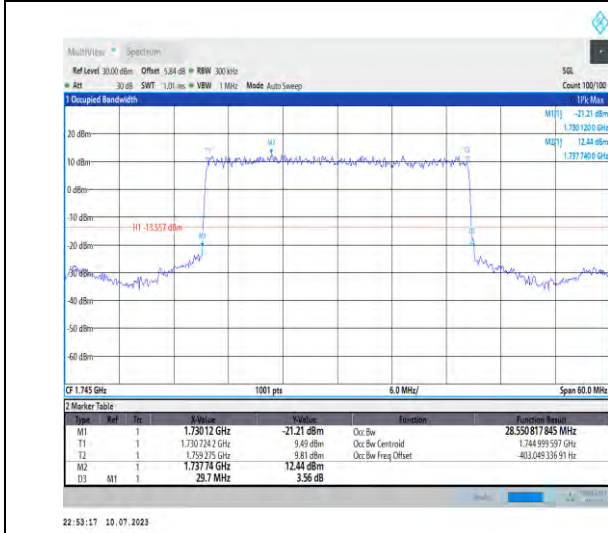
1-N66-PC3-15-30-M-2-DFT-PI2BPSK-Outer_Full-160 @0-Ant3-28.551-29.700-≤30-PASS
