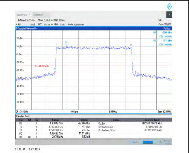
1-N66-PC3-15-30-M-7-CP-16QAM-Outer_Full-160@0 -Ant3-28.552-29.760-≤30-PASS
