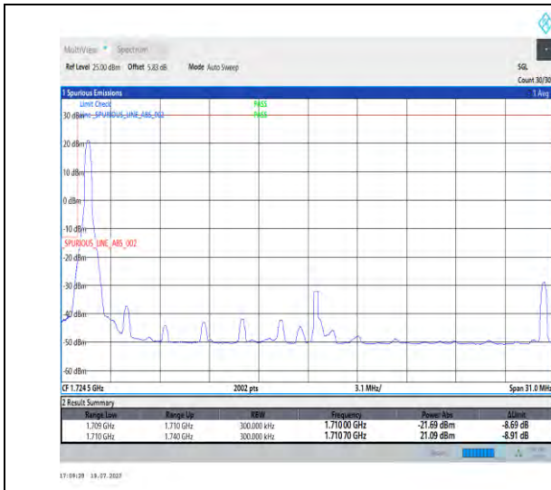
1-N66-PC3-15-30-L-1-DFT-PI2BPSK-Edge_1RB_Left-1@0-Ant3-1-seegraph-PASS-see graph
