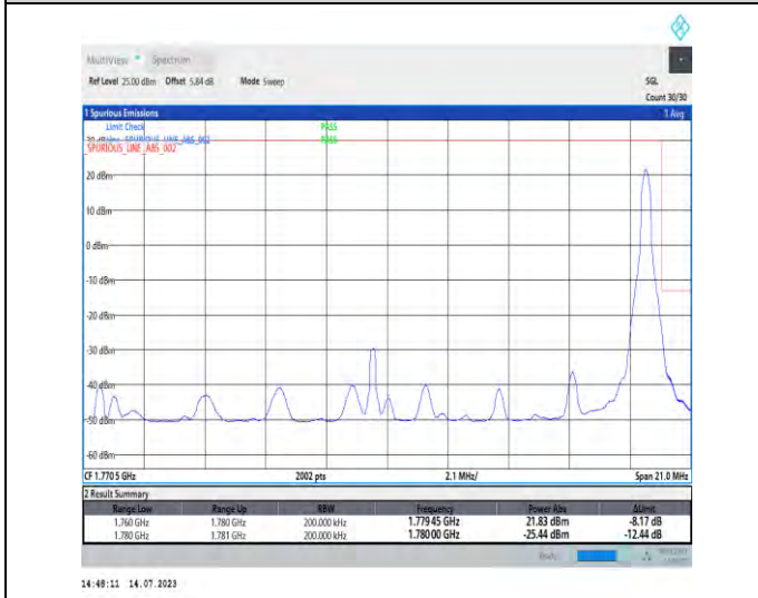
1-N66-PC3-15-20-H-5-CP-QPSK-Edge_1RB_Right-1@105-Ant3-1-seegraph-PASS-see graph
