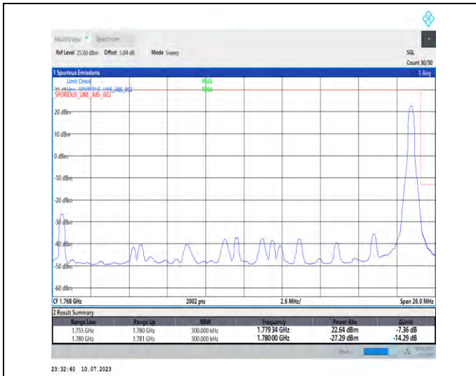
1-N66-PC3-15-25-H-2-DFT-PI2BPSK-Edge_1RB_Right-t-1@132-Ant3-1-seegraph-PASS-see graph
