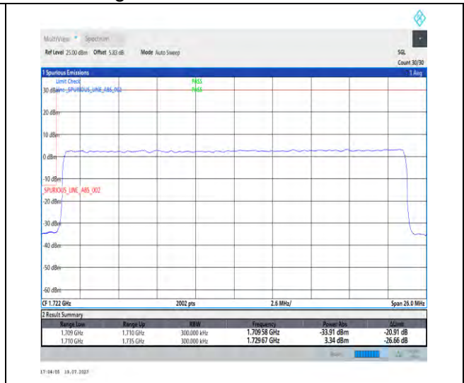
1-N66-PC3-15-25-L-3-DFT-PI2BPSK-Outer_Full-128@0-Ant3-1-seegraph-PASS-see graph
