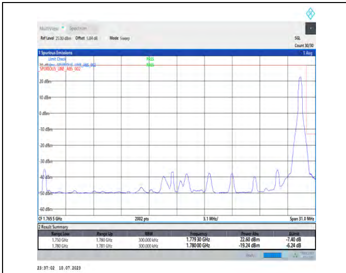
1-N66-PC3-15-30-H-2-DFT-PI2BPSK-Edge_1RB_Right-t-1@159-Ant3-1-seegraph-PASS-see graph
