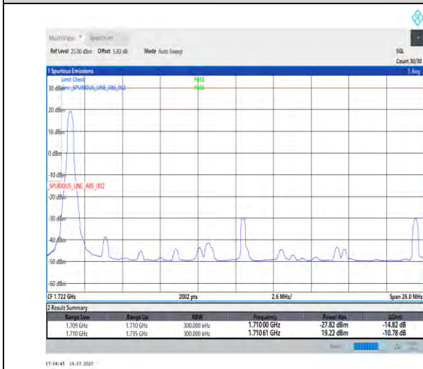
1-N66-PC3-15-25-L-4-CP-QPSK-Edge_1RB_Left-1@0-Ant3-1-seegraph-PASS-see graph
