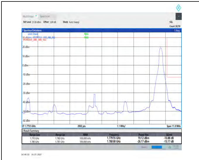
1-N66-PC3-15-10-H-2-DFT-PI2BPSK-Edge_1RB_Right-t-1@51-Ant3-1-seegraph-PASS-see graph
