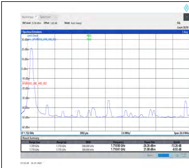
1-N66-PC3-15-25-L-1-DFT-PI2BPSK-Edge_1RB_Left-1@0-Ant3-1-seegraph-PASS-see graph
