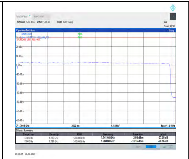
1-N66-PC3-15-40-H-3-DFT-PI2BPSK-Outer_Full-216@0-Ant3-1-seegraph-PASS-see graph
