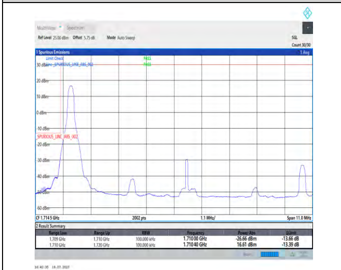
1-N66-PC3-15-10-L-4-CP-QPSK-Edge_1RB_Left-1@0-Ant3-1-seegraph-PASS-see graph
