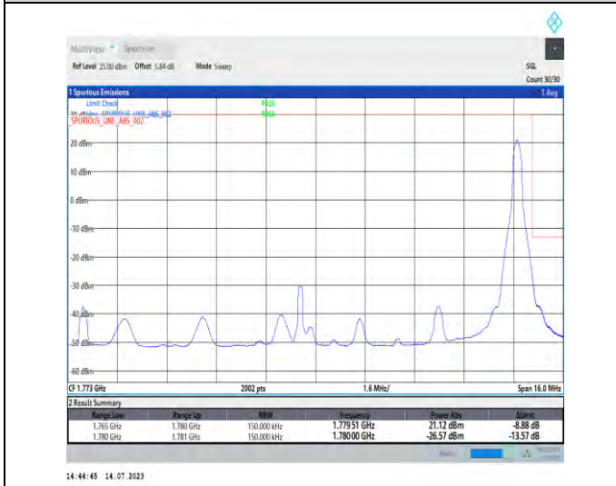
1-N66-PC3-15-15-H-5-CP-QPSK-Edge_1RB_Right-1@78-Ant3-1-seegraph-PASS-see graph
