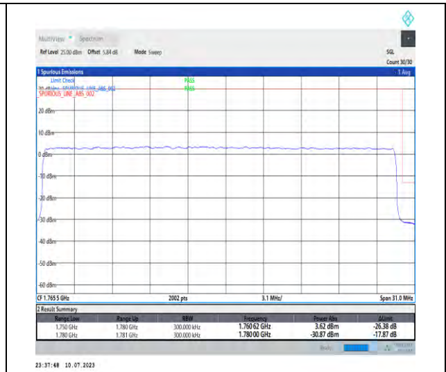
1-N66-PC3-15-30-H-3-DFT-PI2BPSK-Outer_Full-160@0-Ant3-1-seegraph-PASS-see graph
