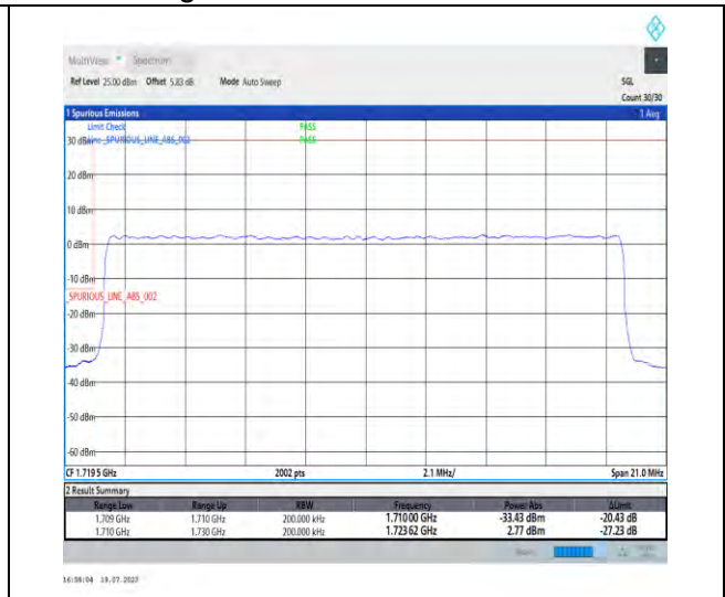
1-N66-PC3-15-20-L-3-DFT-PI2BPSK-Outer_Full-100@0-Ant3-1-seegraph-PASS-see graph
