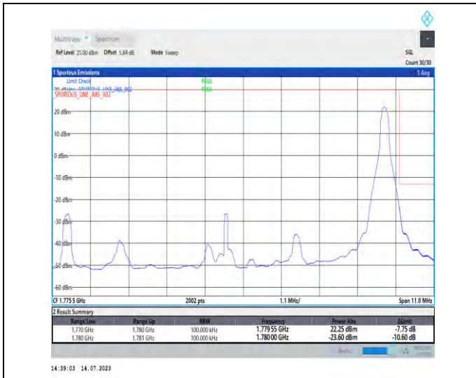
1-N66-PC3-15-10-H-2-DFT-PI2BPSK-Edge_1RB_Right-t-1@51-Ant3-1-seegraph-PASS-see graph
