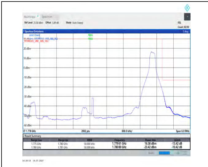
1-N66-PC3-15-5-H-2-DFT-PI2BPSK-Edge_1RB_Right-1@24-Ant3-1-seegraph-PASS-see graph
