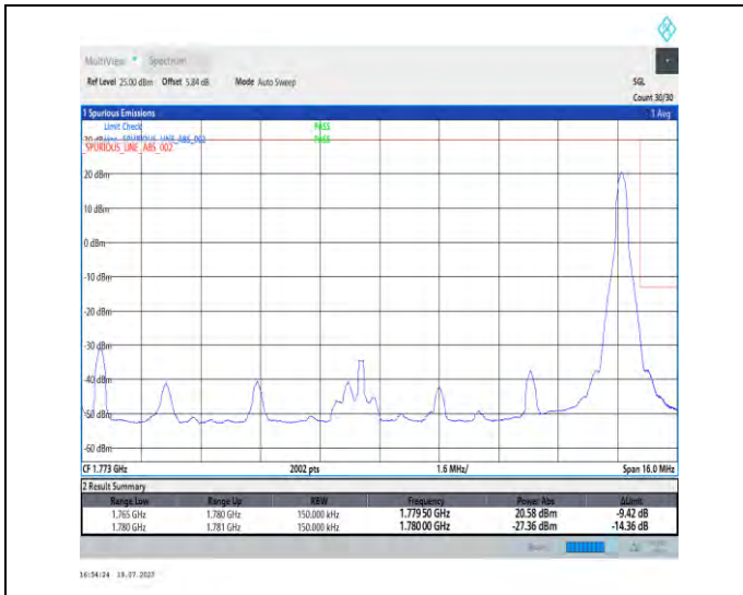
1-N66-PC3-15-15-H-2-DFT-PI2BPSK-Edge_1RB_Right-t1@78-Ant3-1-seegraph-PASS-see graph
