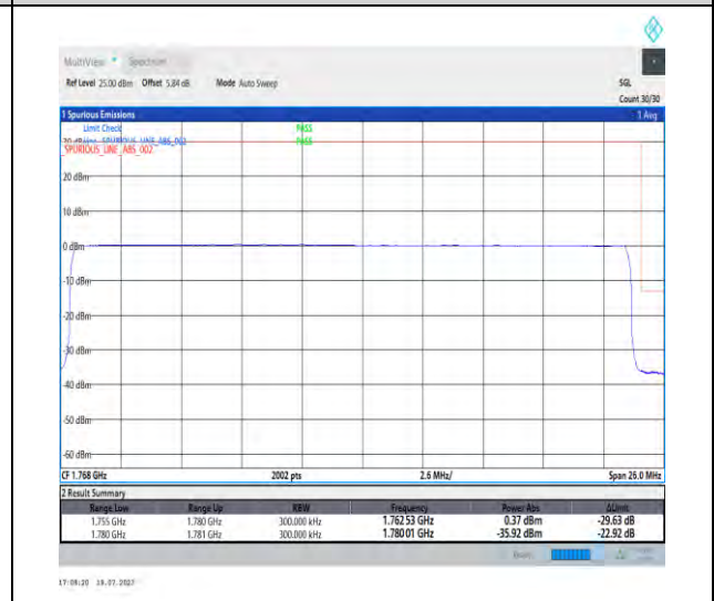
1-N66-PC3-15-25-H-6-CP-QPSK-Outer_Full-133@0-Ant3-1-seegraph-PASS-see graph
