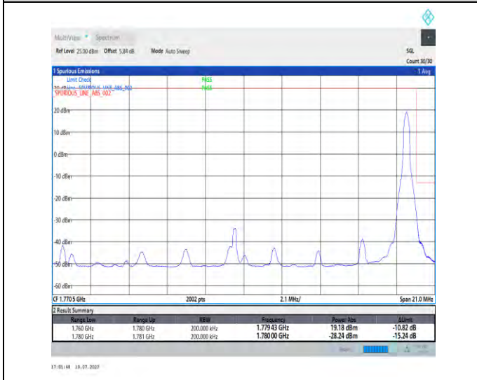
1-N66-PC3-15-20-H-5-CP-QPSK-Edge_1RB_Right-1@105-Ant3-1-seegraph-PASS-see graph
