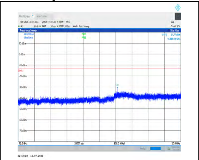
1-N66-PC3-15-40-H-1-DFT-PI2BPSK-Inner_1RB_Lef t-1@1-12000-20000-Ant3-16888.40--31.77--13-PASS
