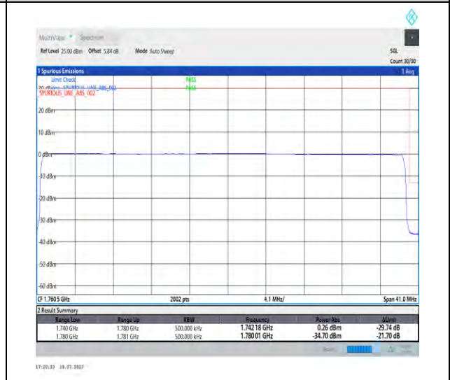
1-N66-PC3-15-40-H-6-CP-QPSK-Outer_Full-216@0-Ant3-1-seegraph-PASS-see graph
