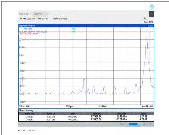
1-N66-PC3-15-30-H-2-DFT-PI2BPSK-Edge_1RB_Right-t-1@159-Ant3-1-seegraph-PASS-see graph
