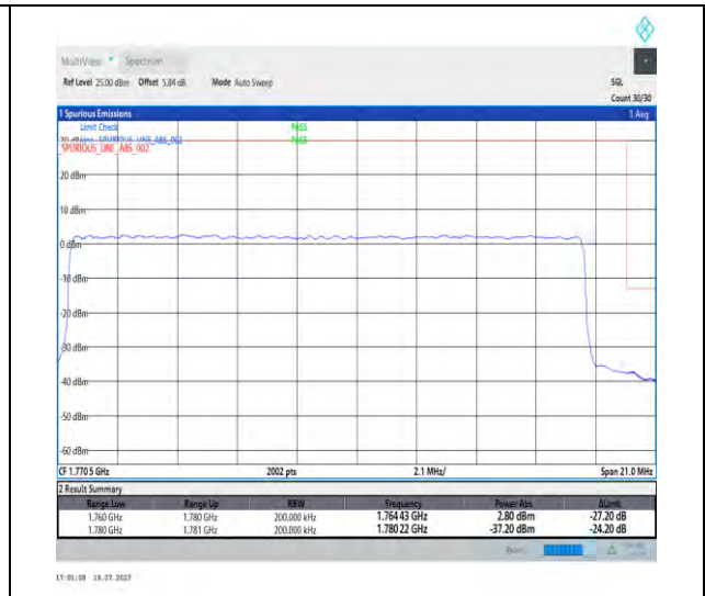
1-N66-PC3-15-20-H-3-DFT-PI2BPSK-Outer_Full-100@0-Ant3-1-seegraph-PASS-see graph
