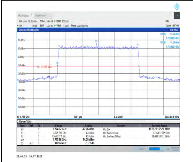
1-N66-PC3-15-40-M-1-DFT-QPSK-Outer_Full-216 @0-Ant3-38.612-40.160-≤40-PASS
