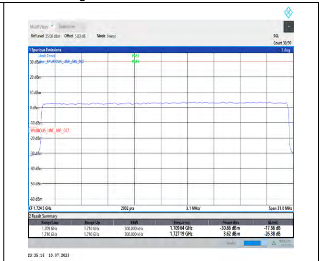
1-N66-PC3-15-30-L-3-DFT-PI2BPSK-Outer_Full-160@0-Ant3-1-seegraph-PASS-see graph
