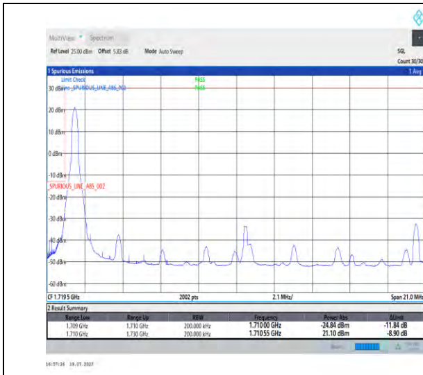
1-N66-PC3-15-20-L-1-DFT-PI2BPSK-Edge_1RB_Left-1@0-Ant3-1-seegraph-PASS-see graph
