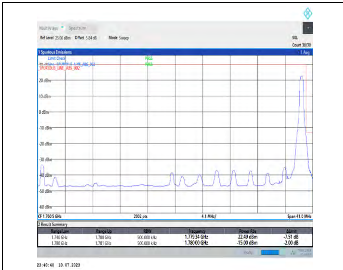
1-N66-PC3-15-40-H-2-DFT-PI2BPSK-Edge_1RB_Right-t-1@215-Ant3-1-seegraph-PASS-see graph
