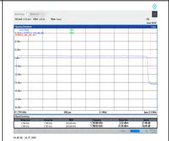
1-N66-PC3-15-20-H-6-CP-QPSK-Outer_Full-106@0-Ant3-1-seegraph-PASS-see graph
