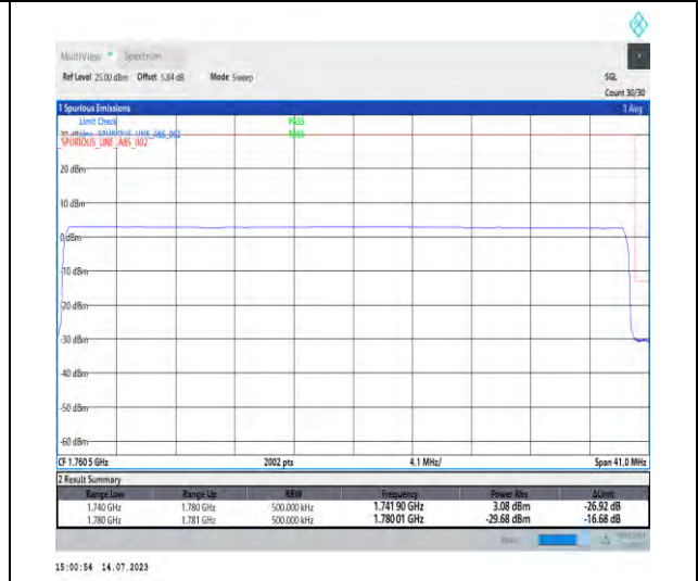
1-N66-PC3-15-40-H-6-CP-QPSK-Outer_Full-216@0-Ant3-1-seegraph-PASS-see graph
