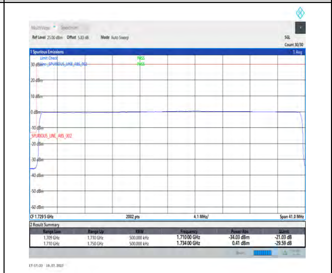
1-N66-PC3-15-40-L-6-CP-QPSK-Outer_Full-216@0-Ant3-1-seegraph-PASS-see graph
