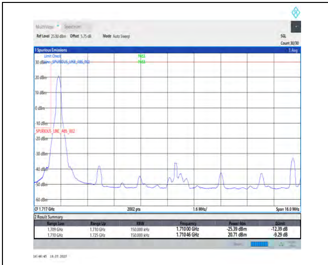
1-N66-PC3-15-15-L-1-DFT-PI2BPSK-Edge_1RB_Left-1@0-Ant3-1-seegraph-PASS-see graph
