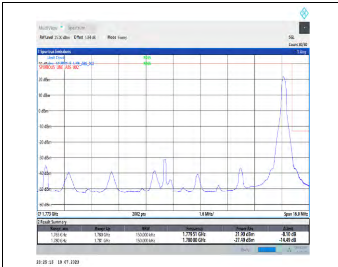
1-N66-PC3-15-15-H-2-DFT-PI2BPSK-Edge_1RB_Right-t-1@78-Ant3-1-seegraph-PASS-see graph
