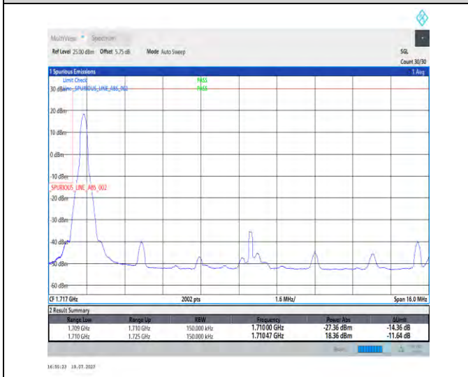
1-N66-PC3-15-15-L-4-CP-QPSK-Edge_1RB_Left-1@0-Ant3-1-seegraph-PASS-see graph
