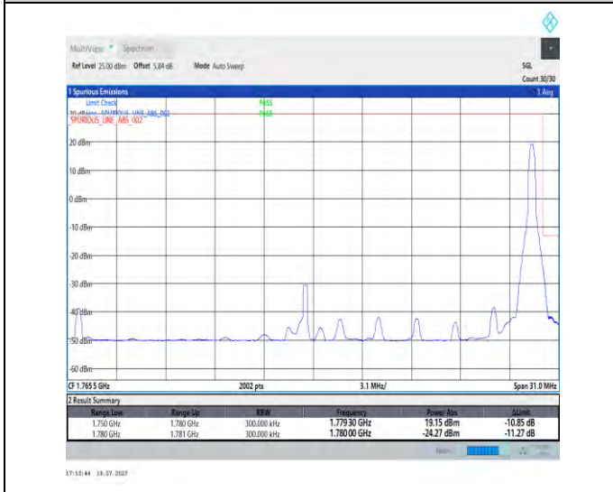
1-N66-PC3-15-30-H-5-CP-QPSK-Edge_1RB_Right-1@159-Ant3-1-seegraph-PASS-see graph
