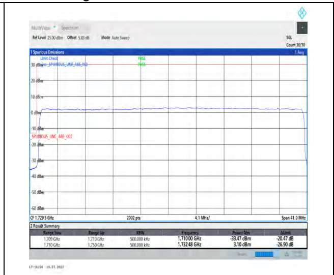
1-N66-PC3-15-40-L-3-DFT-PI2BPSK-Outer_Full-216@0-Ant3-1-seegraph-PASS-see graph
