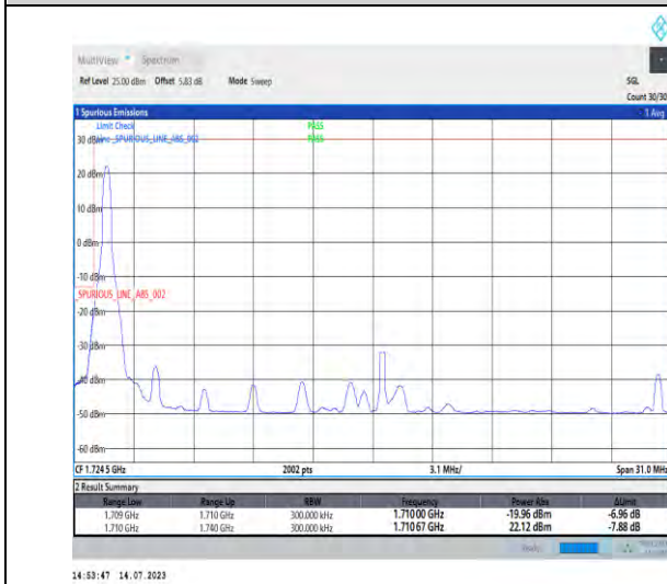
1-N66-PC3-15-30-L-4-CP-QPSK-Edge_1RB_Left-1@0-Ant3-1-seegraph-PASS-see graph
