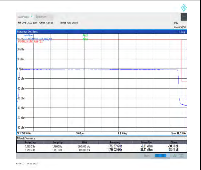
1-N66-PC3-15-30-H-6-CP-QPSK-Outer_Full-160@0-Ant3-1-seegraph-PASS-see graph
