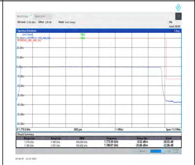
1-N66-PC3-15-10-H-6-CP-QPSK-Outer_Full-52@0-Ant3-1-seegraph-PASS-see graph
