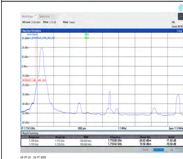
1-N66-PC3-15-10-L-4-CP-QPSK-Edge_1RB_Left-1@0-Ant3-1-seegraph-PASS-see graph
