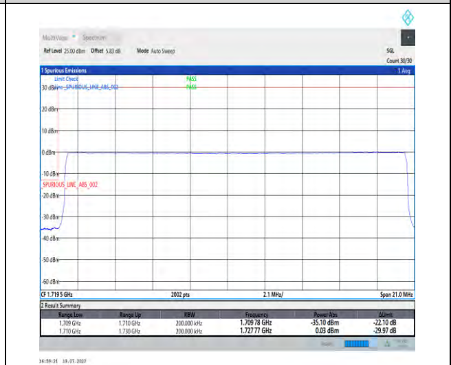
1-N66-PC3-15-20-L-6-CP-QPSK-Outer_Full-106@0-Ant3-1-seegraph-PASS-see graph
