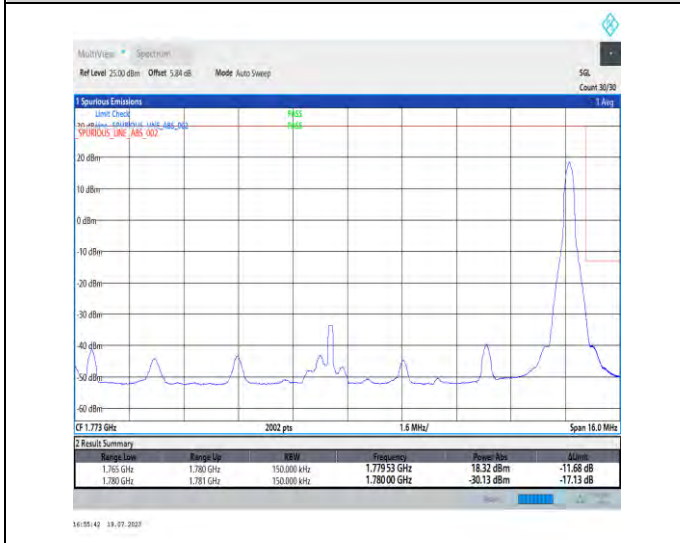
1-N66-PC3-15-15-H-5-CP-QPSK-Edge_1RB_Right-1@78-Ant3-1-seegraph-PASS-see graph
