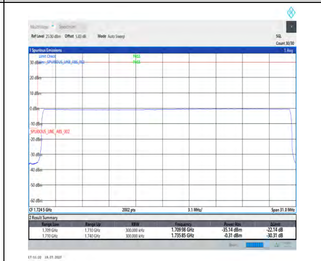
1-N66-PC3-15-30-L-6-CP-QPSK-Outer_Full-160@0-Ant3-1-seegraph-PASS-see graph
