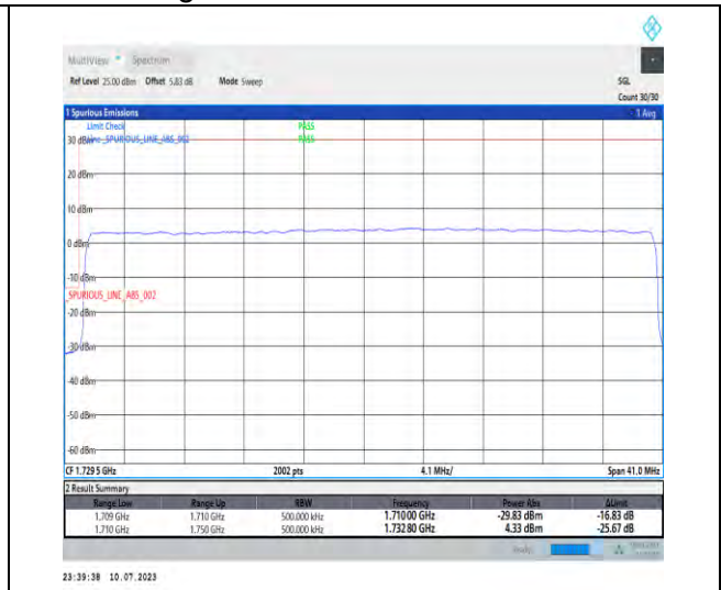
1-N66-PC3-15-40-L-3-DFT-PI2BPSK-Outer_Full-216@0-Ant3-1-seegraph-PASS-see graph
