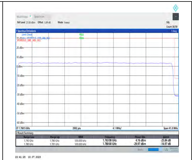
1-N66-PC3-15-40-H-3-DFT-PI2BPSK-Outer_Full-2-16@0-Ant3-1-seegraph-PASS-see graph
