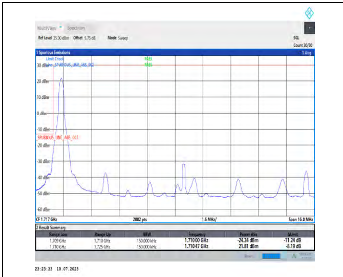
1-N66-PC3-15-15-L-1-DFT-PI2BPSK-Edge_1RB_Left-1@0-Ant3-1-seegraph-PASS-see graph
