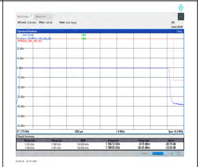
1-N66-PC3-15-15-H-6-CP-QPSK-Outer_Full-79@0-Ant3-1-seegraph-PASS-see graph
