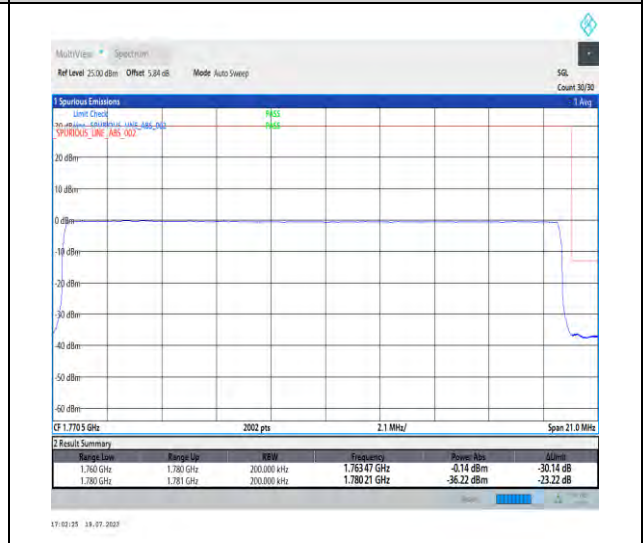
1-N66-PC3-15-20-H-6-CP-QPSK-Outer_Full-106@0-Ant3-1-seegraph-PASS-see graph
