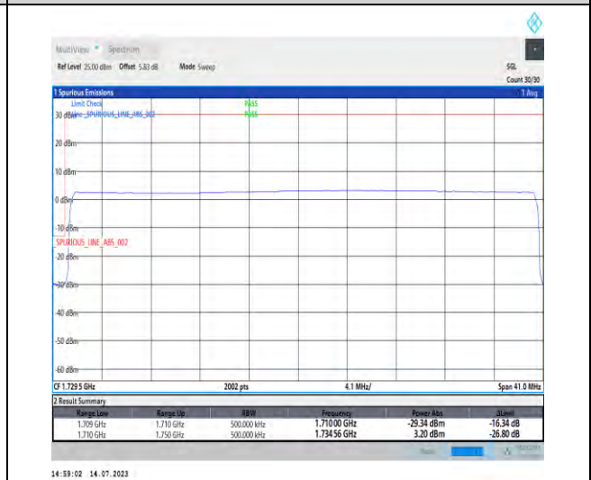
1-N66-PC3-15-40-L-6-CP-QPSK-Outer_Full-216@0-Ant3-1-seegraph-PASS-see graph
