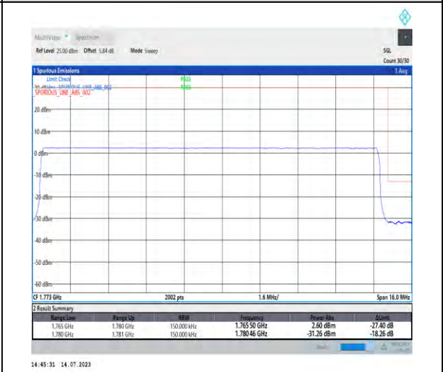
1-N66-PC3-15-15-H-6-CP-QPSK-Outer_Full-79@0-Ant3-1-seegraph-PASS-see graph
