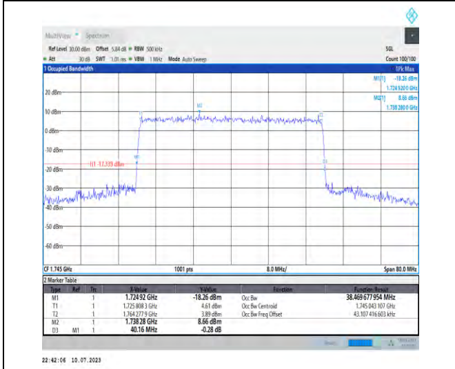
1-N66-PC3-15-40-M-9-CP-256QAM-Outer_Full-216 @0-Ant3-38.47-40.160-≤40-PASS
