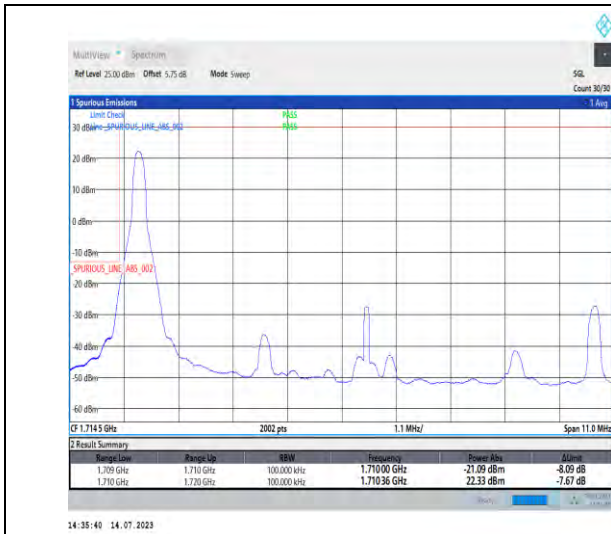
1-N66-PC3-15-10-L-1-DFT-PI2BPSK-Edge_1RB_Left-1@0-Ant3-1-seegraph-PASS-see graph
