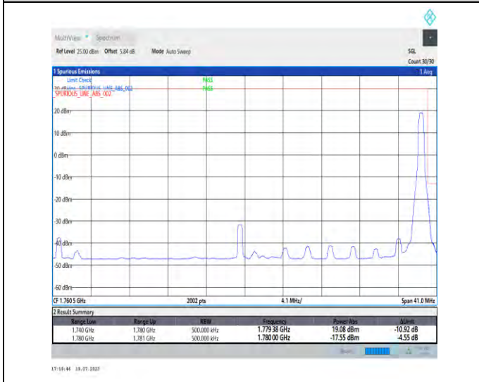
1-N66-PC3-15-40-H-5-CP-QPSK-Edge_1RB_Right-1@215-Ant3-1-seegraph-PASS-see graph
