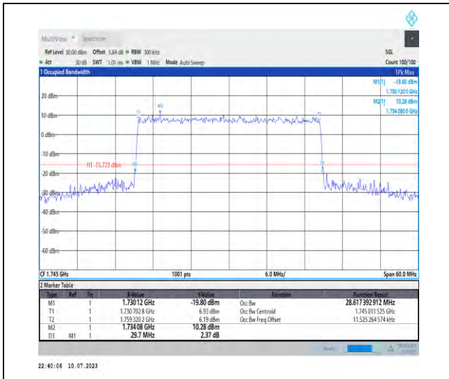
1-N66-PC3-15-30-M-8-CP-64QAM-Outer_Full-160 @0-Ant3-28.617-29.700-≤30-PASS
