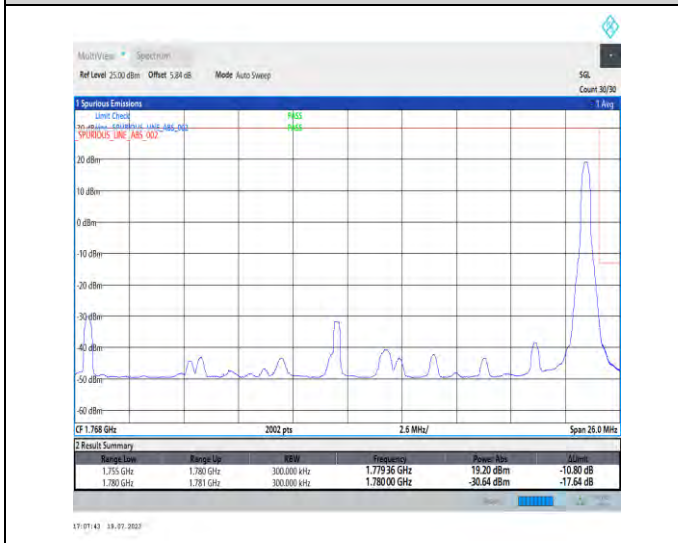
1-N66-PC3-15-25-H-5-CP-QPSK-Edge_1RB_Right-1@132-Ant3-1-seegraph-PASS-see graph
