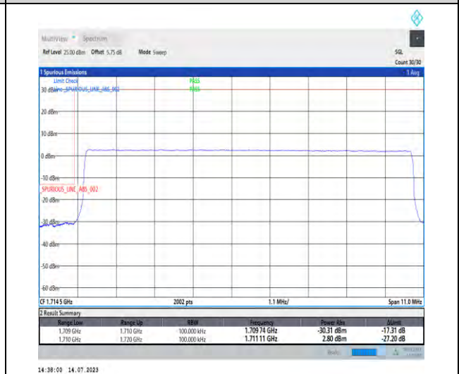
1-N66-PC3-15-10-L-6-CP-QPSK-Outer_Full-52@0-Ant3-1-seegraph-PASS-see graph
