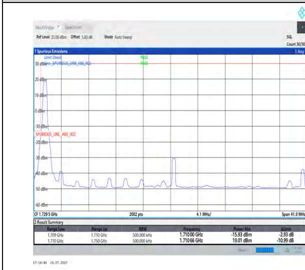
1-N66-PC3-15-40-L-4-CP-QPSK-Edge_1RB_Left-1@0-Ant3-1-seegraph-PASS-see graph
