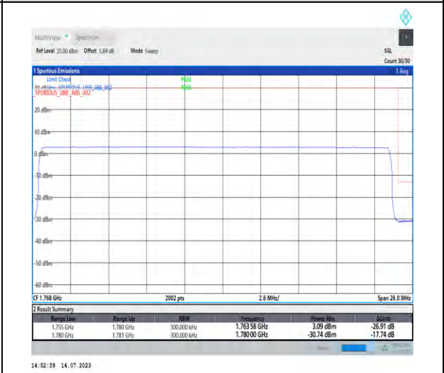
1-N66-PC3-15-25-H-6-CP-QPSK-Outer_Full-133@0-Ant3-1-seegraph-PASS-see graph
