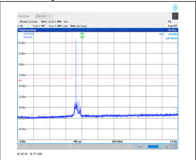
1-N66-PC3-15-40-M-1-DFT-PI2BPSK-Inner_1RB_Lef t-1@1-1000-3000-Ant3-2991.50--44.68--13-PASS
