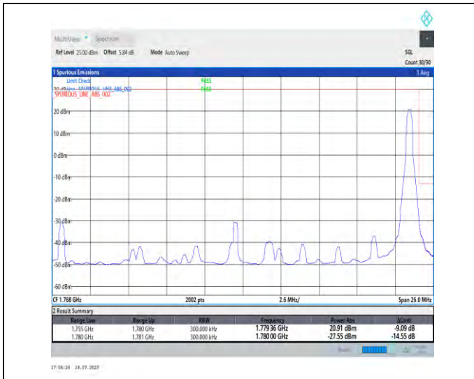
1-N66-PC3-15-25-H-2-DFT-PI2BPSK-Edge_1RB_Right-t-1@132-Ant3-1-seegraph-PASS-see graph
