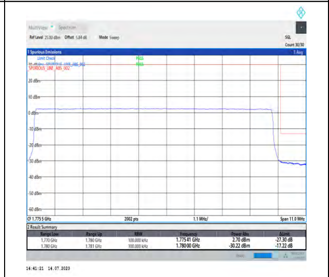
1-N66-PC3-15-10-H-6-CP-QPSK-Outer_Full-52@0-Ant3-1-seegraph-PASS-see graph
