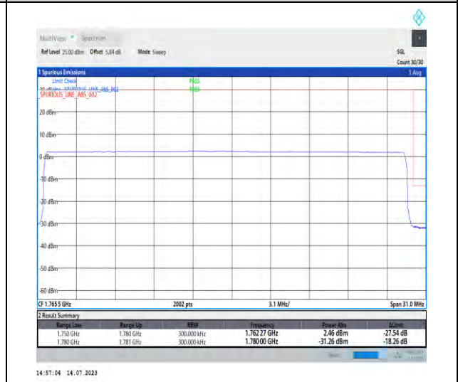
1-N66-PC3-15-30-H-6-CP-QPSK-Outer_Full-160@0-Ant3-1-seegraph-PASS-see graph
