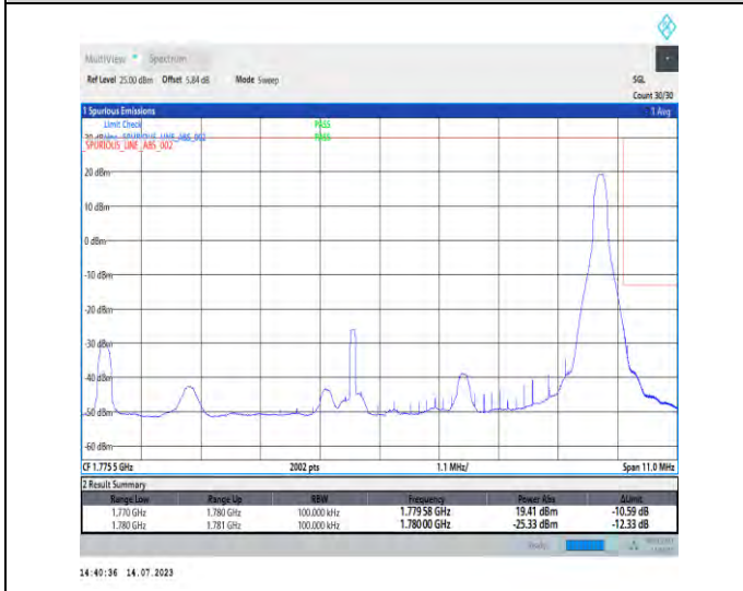
1-N66-PC3-15-10-H-5-CP-QPSK-Edge_1RB_Right-1@51-Ant3-1-seegraph-PASS-see graph
