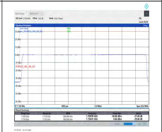
1-N66-PC3-15-25-L-6-CP-QPSK-Outer_Full-133@0-Ant3-1-seegraph-PASS-see graph
