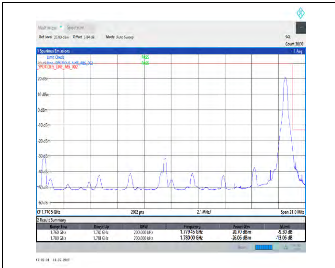
1-N66-PC3-15-20-H-2-DFT-PI2BPSK-Edge_1RB_Right-t-1@105-Ant3-1-seegraph-PASS-see graph
