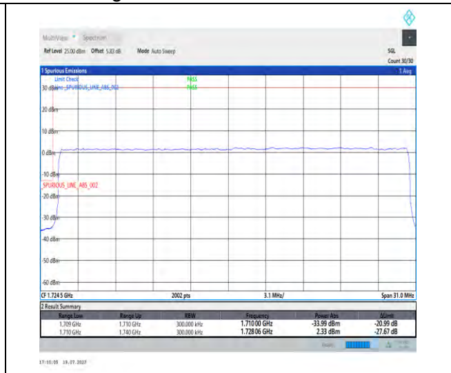
1-N66-PC3-15-30-L-3-DFT-PI2BPSK-Outer_Full-160@0-Ant3-1-seegraph-PASS-see graph
