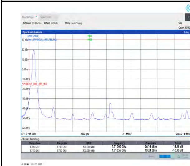
1-N66-PC3-15-20-L-4-CP-QPSK-Edge_1RB_Left-1@0-Ant3-1-seegraph-PASS-see graph
