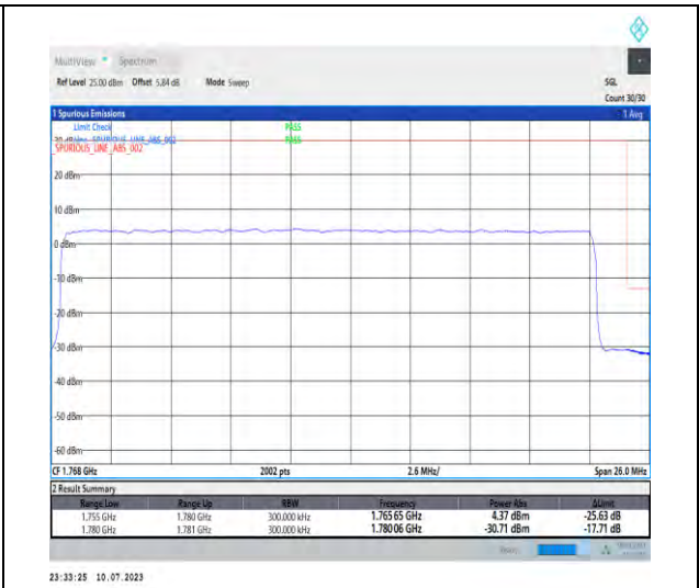
1-N66-PC3-15-25-H-3-DFT-PI2BPSK-Outer_Full-128@0-Ant3-1-seegraph-PASS-see graph
