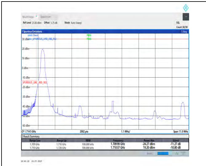
1-N66-PC3-15-10-L-1-DFT-PI2BPSK-Edge_1RB_Left-1@0-Ant3-1-seegraph-PASS-see graph
