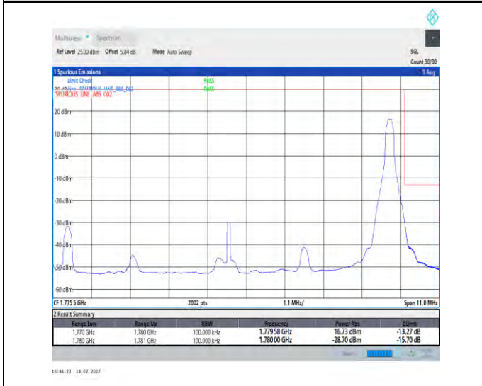
1-N66-PC3-15-10-H-5-CP-QPSK-Edge_1RB_Right-1@51-Ant3-1-seegraph-PASS-see graph
