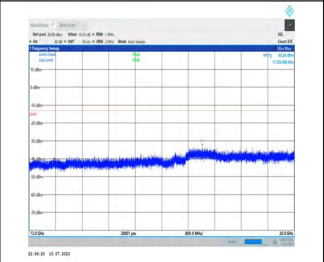
1-N66-PC3-15-40-M-1-DFT-PI2BPSK-Inner_1RB_Lef t-1@1-12000-20000-Ant3-17222.80--33.24--13-PASS
