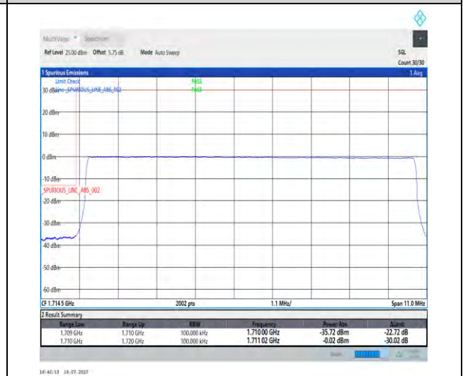
1-N66-PC3-15-10-L-6-CP-QPSK-Outer_Full-52@0-Ant3-1-seegraph-PASS-see graph
