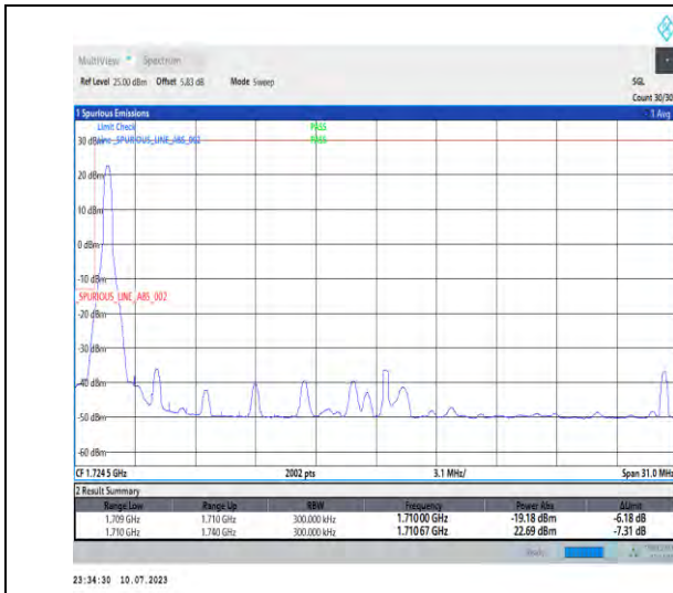
1-N66-PC3-15-30-L-1-DFT-PI2BPSK-Edge_1RB_Left-1@0-Ant3-1-seegraph-PASS-see graph
