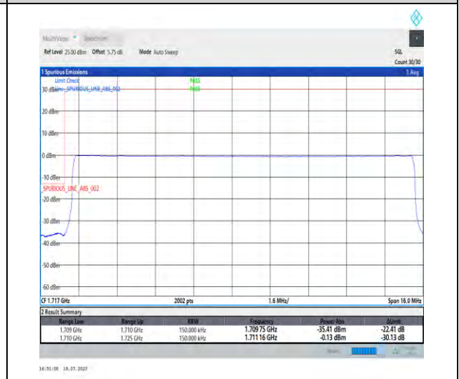
1-N66-PC3-15-15-L-6-CP-QPSK-Outer_Full-79@0-Ant3-1-seegraph-PASS-see graph
