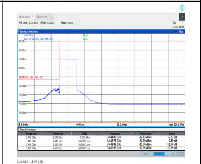
1-N77-3450-3550-PC1.5-30-20-L-6-CP-QPSK-Outer_Full-51@0-Ant3-1--PASS-see graph
