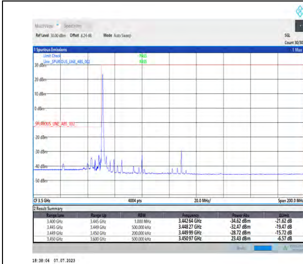
1-N77-3450-3550-PC1.5-30-60-L-1-DFT-PI2BPSK-Edge_1RB_Left-1@0-Ant3-1--PASS-see graph
