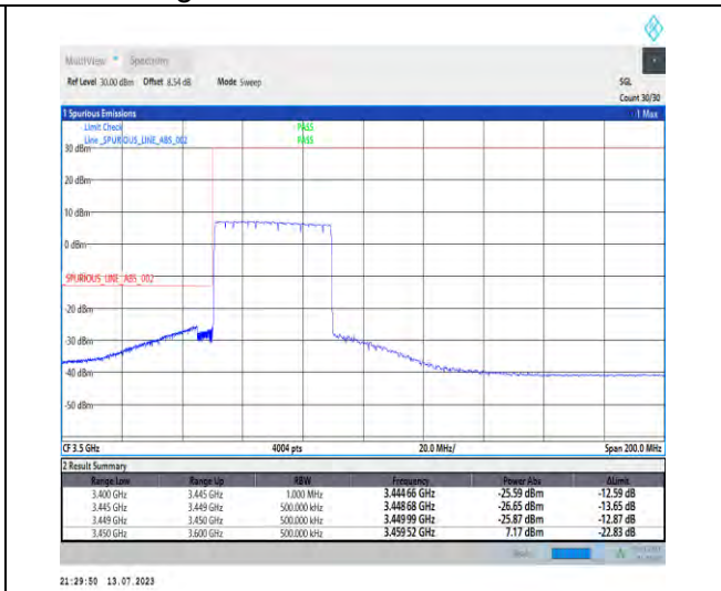
1-N77-3450-3550-PC1.5-30-40-L-3-DFT-PI2BPSK-Outer_Full-100@0-Ant3-1--PASS-see graph
