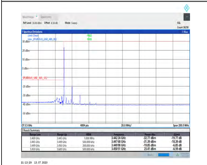
1-N77-3450-3550-PC1.5-30-20-L-4-CP-QPSK-Edge_1RB_Left-1@0-Ant3-1--PASS-see graph
