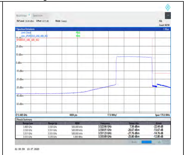
1-N77-3450-3550-PC1.5-30-40-H-3-DFT-PI2BPSK-Outer_Full-100@0-Ant3-1--PASS-see graph
