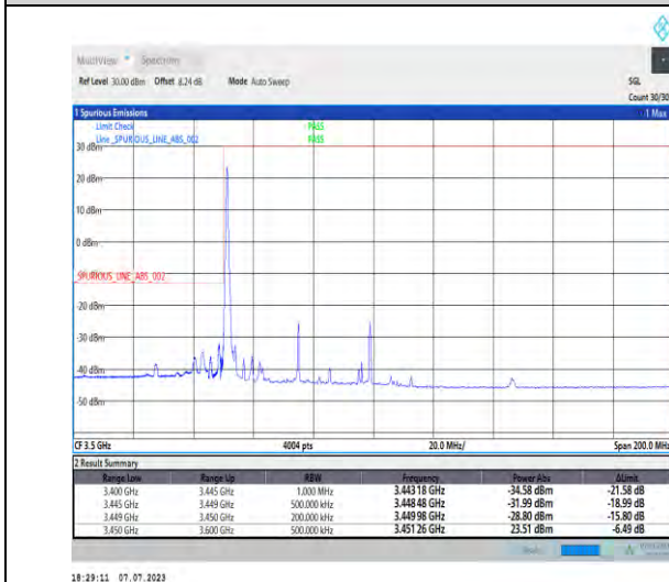
1-N77-3450-3550-PC1.5-30-50-L-4-CP-QPSK-Edge_1RB_Left-1@0-Ant3-1--PASS-see graph
