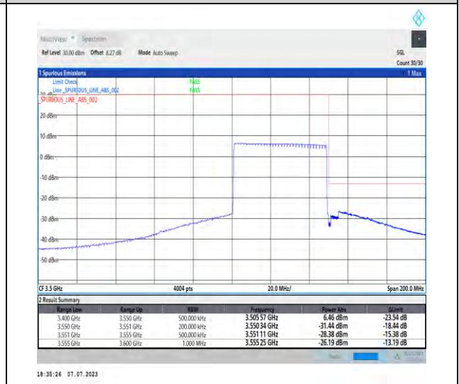
1-N77-3450-3550-PC1.5-30-50-H-6-CP-QPSK-Outer_Full-133@0-Ant3-1--PASS-see graph
