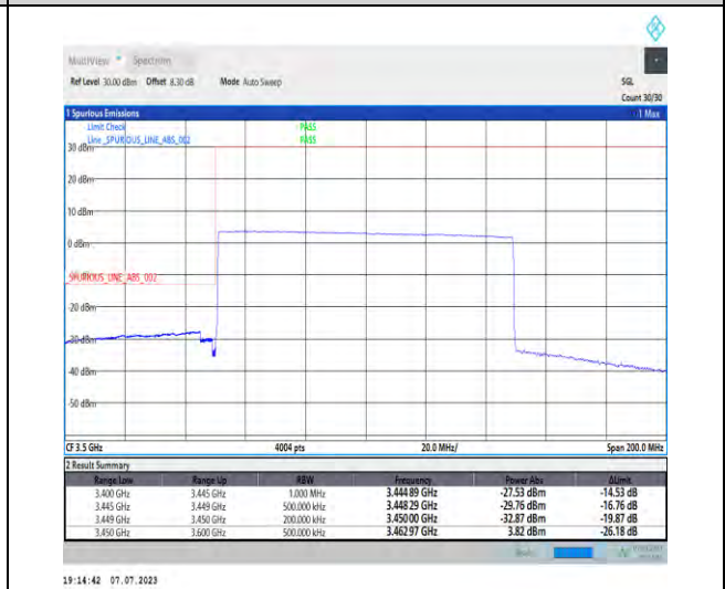
1-N77-3450-3550-PC1.5-30-100-L-6-CP-QPSK-Outer_Full-273@0-Ant3-1--PASS-see graph
