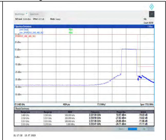
1-N77-3450-3550-PC1.5-30-20-H-3-DFT-PI2BPSK-Outer_Full-50@0-Ant3-1--PASS-see graph
