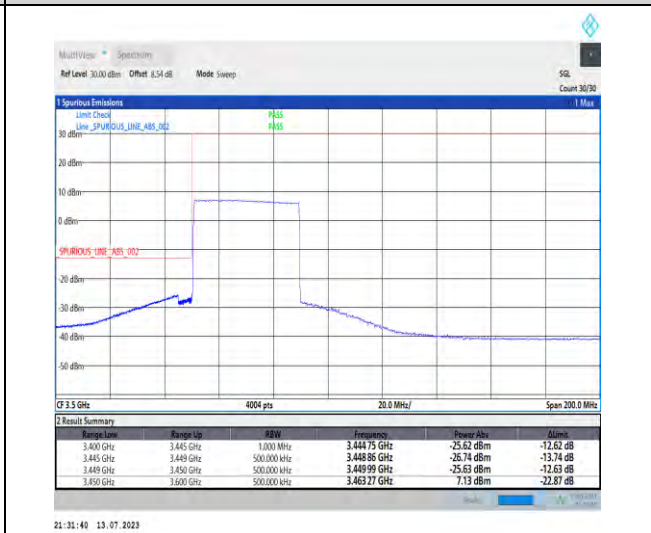
1-N77-3450-3550-PC1.5-30-40-L-6-CP-QPSK-Outer_Full-100@0-Ant3-1--PASS-see graph
