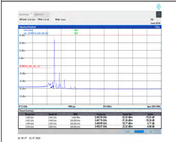
1-N77-3450-3550-PC1.5-30-15-L-4-CP-QPSK-Edge_1RB_Left-1@0-Ant3-1--PASS-see graph
