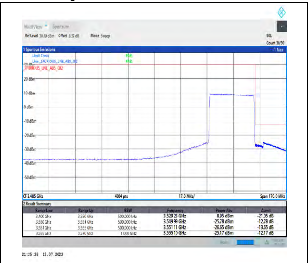
1-N77-3450-3550-PC1.5-30-30-H-3-DFT-PI2BPSK-Outer_Full-75@0-Ant3-1--PASS-see graph
