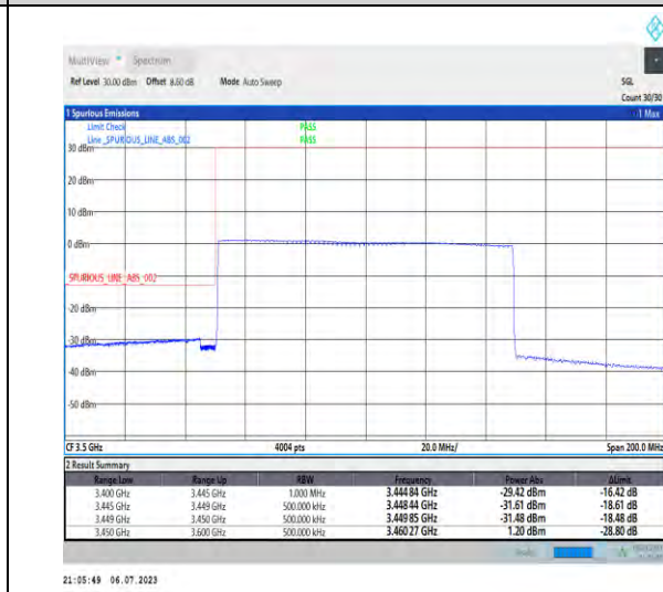
1-N77-3450-3550-PC1.5-30-100-L-4-CP-QPSK-Edge _1RB_Left-1@0-Ant3-1--PASS-see graph 1-N77-3450-3550-PC1.5-30-100-L-6-CP-QPSK-Out er_Full-273@0-Ant3-1--PASS-see graph
