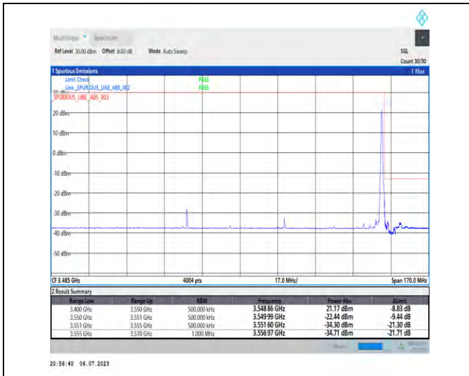
1-N77-3450-3550-PC1.5-30-90-H-2-DFT-PI2BPSK-Edge_1RB_Right-1@244-Ant3-1--PASS-see graph
