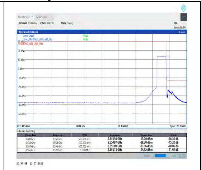
1-N77-3450-3550-PC1.5-30-10-H-3-DFT-PI2BPSK-Outer_Full-24@0-Ant3-1--PASS-see graph
