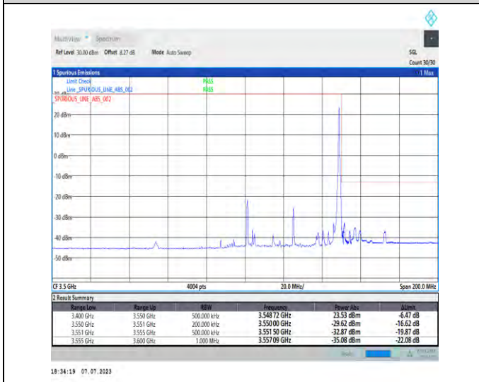
1-N77-3450-3550-PC1.5-30-50-H-5-CP-QPSK-Edge_1RB_Right-1@132-Ant3-1--PASS-see graph
