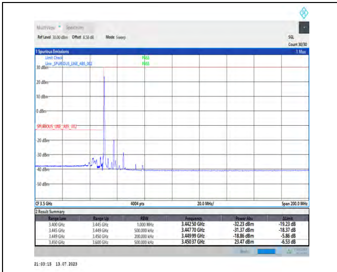
1-N77-3450-3550-PC1.5-30-15-L-1-DFT-PI2BPSK-Edge_1RB_Left-1@0-Ant3-1--PASS-see graph
