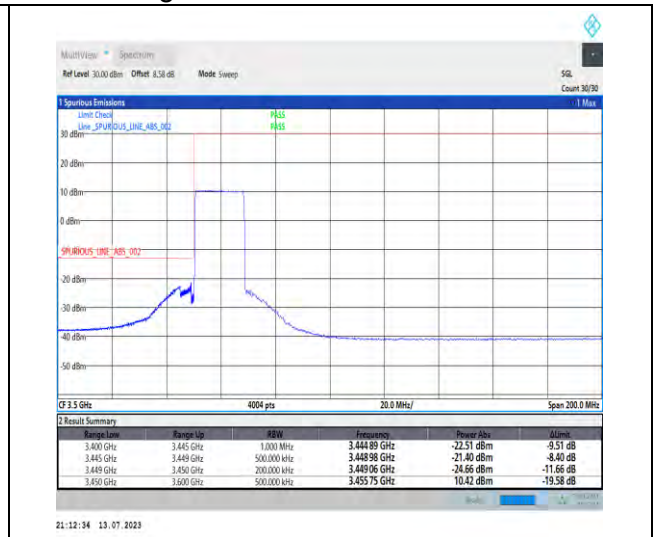
1-N77-3450-3550-PC1.5-30-20-L-3-DFT-PI2BPSK-Outer_Full-50@0-Ant3-1--PASS-see graph
