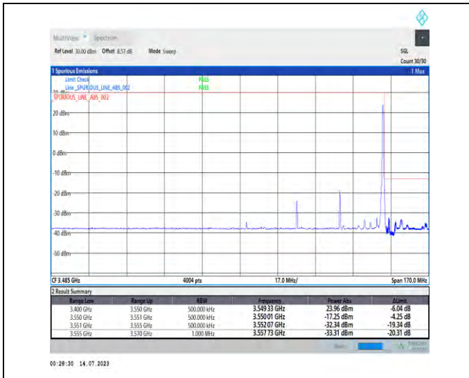
1-N77-3450-3550-PC1.5-30-40-H-2-DFT-PI2BPSK-Edge_1RB_Right-1@105-Ant3-1--PASS-see graph
