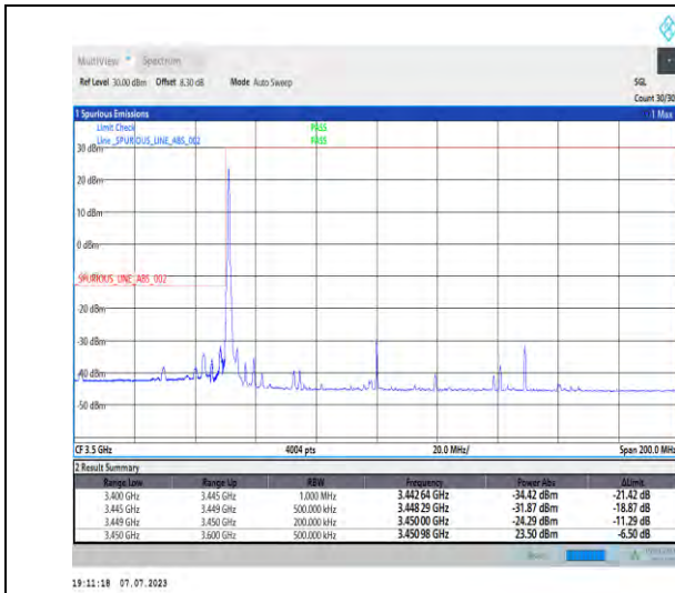
1-N77-3450-3550-PC1.5-30-100-L-1-DFT-PI2BPSK-E dge_1RB_Left-1@0-Ant3-1--PASS-see graph
