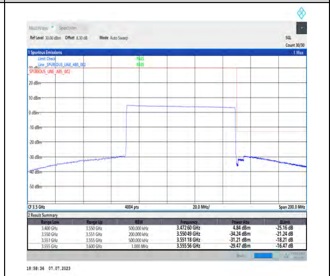
1-N77-3450-3550-PC1.5-30-80-H-6-CP-QPSK-Outer_Full-217@0-Ant3-1--PASS-see graph
