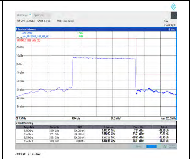
1-N77-3450-3550-PC1.5-30-80-H-3-DFT-PI2BPSK-Outer_Full-100@0-Ant3-1--PASS-see graph
