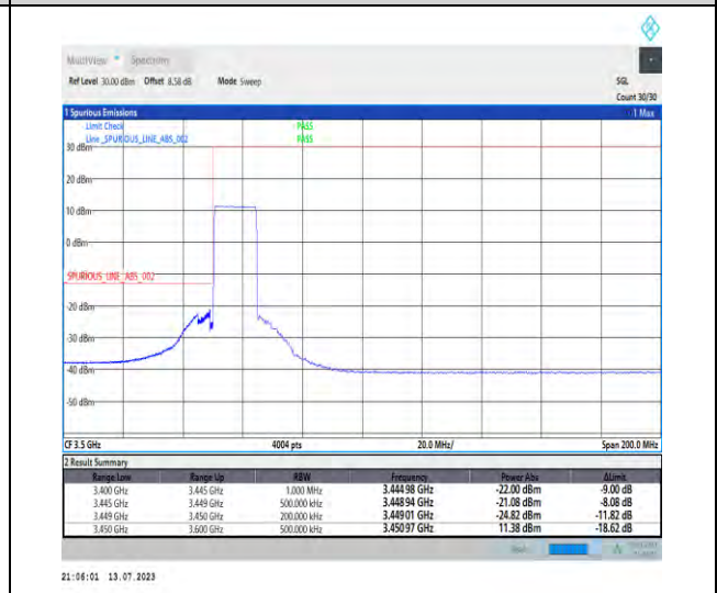
1-N77-3450-3550-PC1.5-30-15-L-6-CP-QPSK-Outer_Full-38@0-Ant3-1--PASS-see graph
