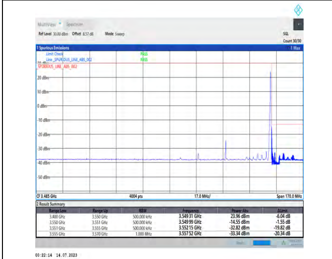
1-N77-3450-3550-PC1.5-30-30-H-5-CP-QPSK-Edge_1RB_Right-1@77-Ant3-1--PASS-see graph
