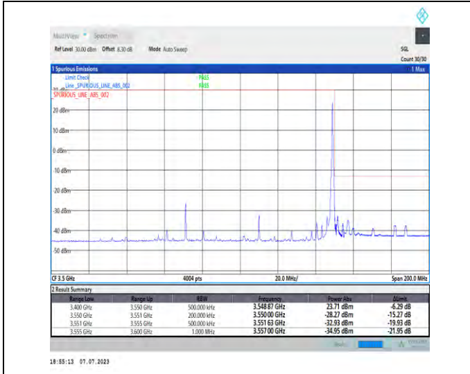
1-N77-3450-3550-PC1.5-30-80-H-2-DFT-PI2BPSK-Edge_1RB_Right-1@216-Ant3-1--PASS-see graph
