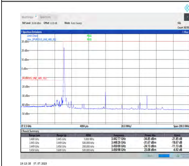
1-N77-3450-3550-PC1.5-30-100-L-4-CP-QPSK-Edge _1RB_Left-1@0-Ant3-1--PASS-see graph
