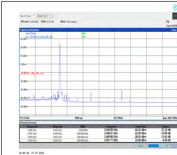
1-N77-3450-3550-PC1.5-30-80-L-1-DFT-PI2BPSK-Edge_1RB_Left-1@0-Ant3-1--PASS-see graph
