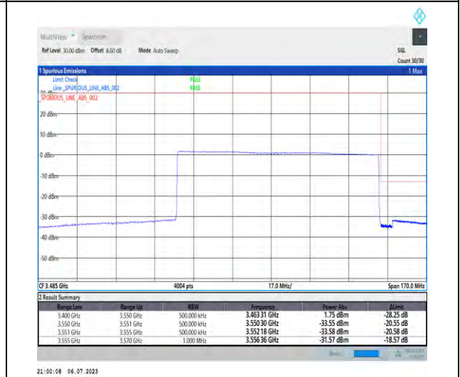
1-N77-3450-3550-PC1.5-30-90-H-6-CP-QPSK-Outer_Full-245@0-Ant3-1--PASS-see graph
