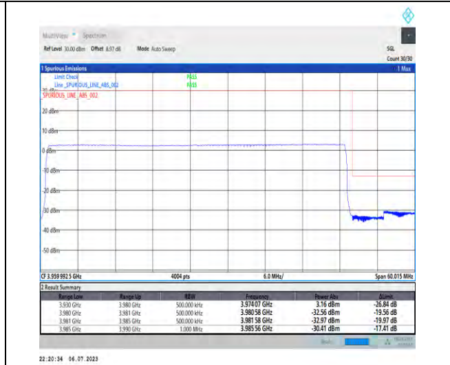
1-N77-3700-3980-PC1-30-50-H-6-CP-QPSK-Outer _Full-133@0-Ant3-1--PASS-see graph
