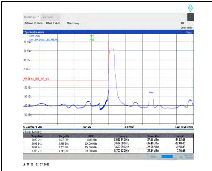
1-N77-3700-3980-PC1.5-30-10-L-4-CP-QPSK-Edge_1 RB_Left-1@0-Ant3-1--PASS-see graph
