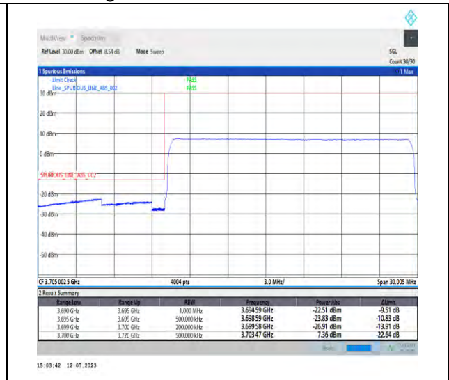
1-N77-3700-3980-PC1.5-30-20-L-6-CP-QPSK-Out er_Full-51@0-Ant3-1--PASS-see graph
