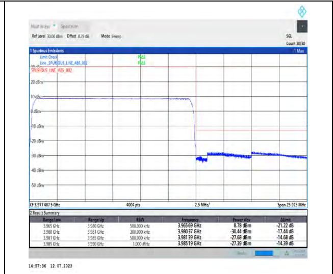
1-N77-3700-3980-PC1.5-30-15-H-6-CP-QPSK-Out_er_Full-38@0-Ant3-1--PASS-see graph
