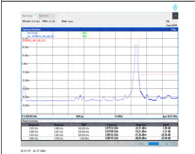
1-N77-3700-3980-PC1.5-30-30-H-2-DFT-PI2BPSK-Ed ge_1RB_Right-1@77-Ant3-1--PASS-see graph
