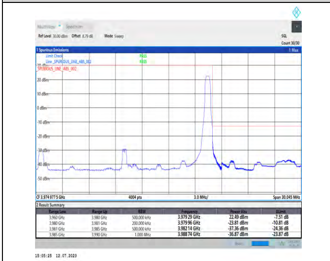
1-N77-3700-3980-PC1.5-30-20-H-2-DFT-PI2BPSK-Ed ge_1RB_Right-1@50-Ant3-1--PASS-see graph
