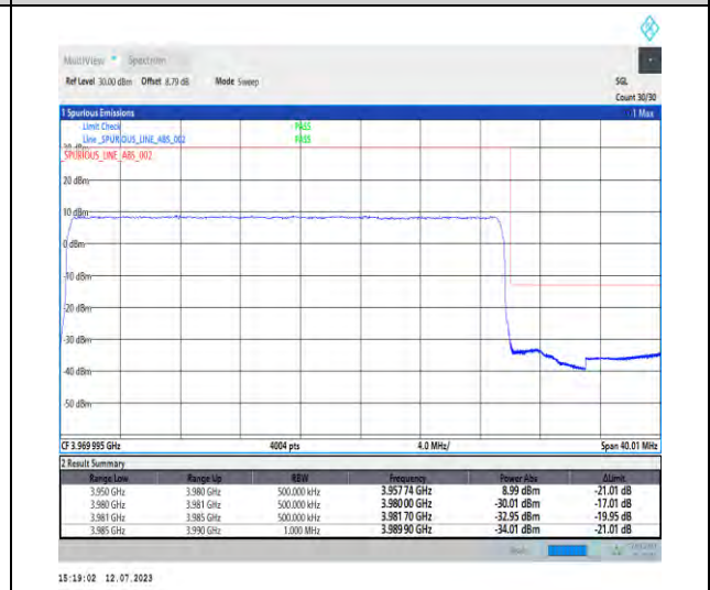
1-N77-3700-3980-PC1.5-30-30-H-3-DFT-PI2BPSK -Outer_Full-75@0-Ant3-1--PASS-see graph
