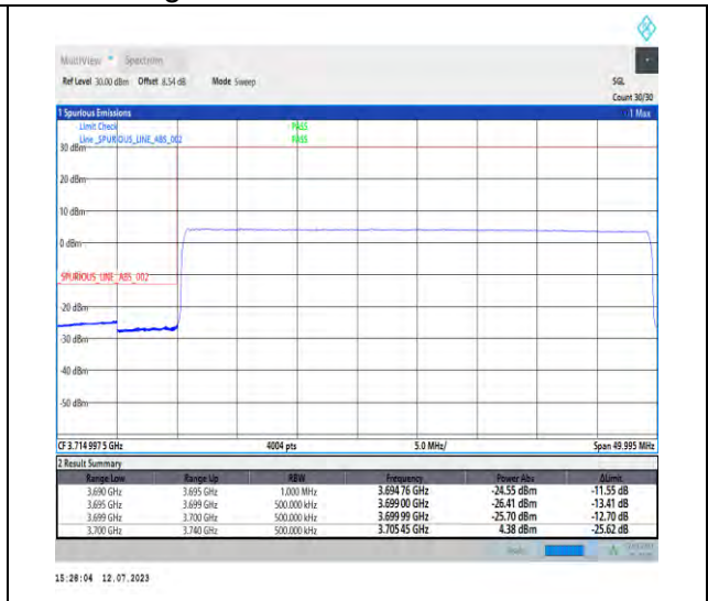
1-N77-3700-3980-PC1.5-30-40-L-6-CP-QPSK-Out er_Full-100@0-Ant3-1--PASS-see graph
