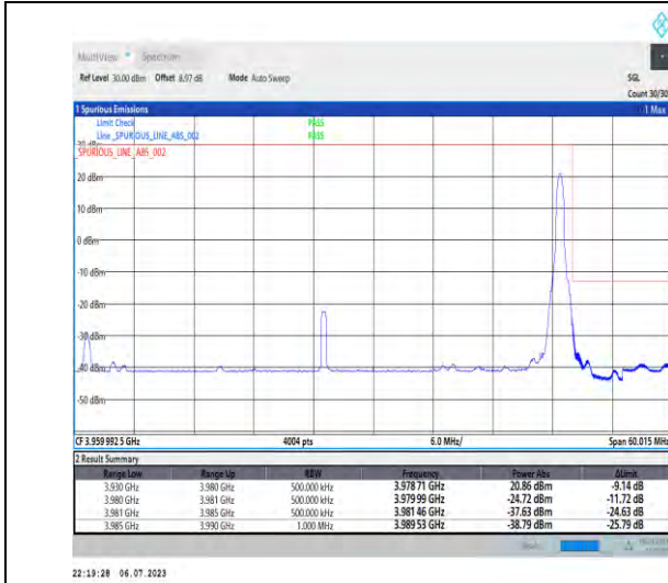
1-N77-3700-3980-PC1-30-50-H-5-CP-QPSK-Edge_1 RB_Right-1@132-Ant3-1--PASS-see graph
