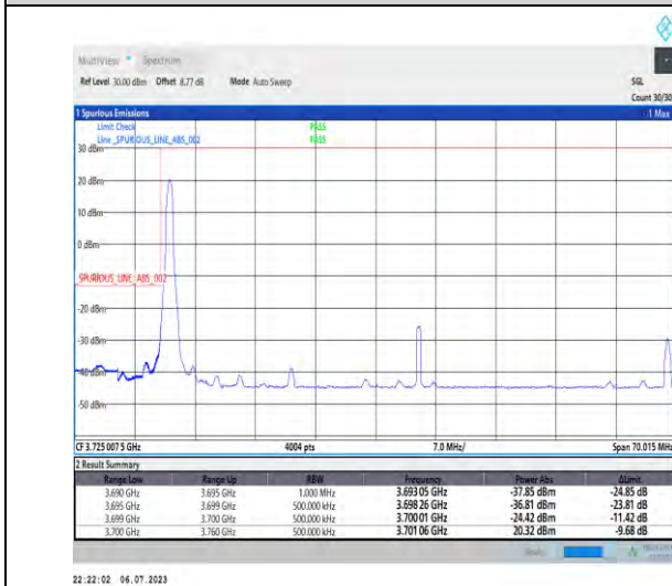
1-N77-3700-3980-PC1-30-60-L-1-DFT-PI2BPSK-Edg e_1RB_Left-1@0-Ant3-1--PASS-see graph
