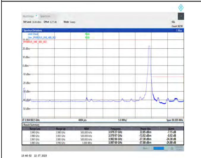
1-N77-3700-3980-PC1.5-30-40-H-2-DFT-PI2BPSK-Ed ge_1RB_Right-1@105-Ant3-1--PASS-see graph
