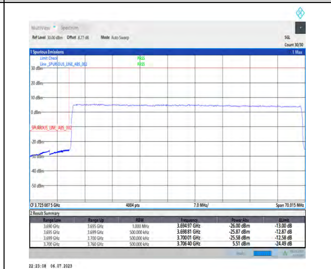
1-N77-3700-3980-PC1-30-60-L-3-DFT-PI2BPSK-O uter_Full-162@0-Ant3-1--PASS-see graph
