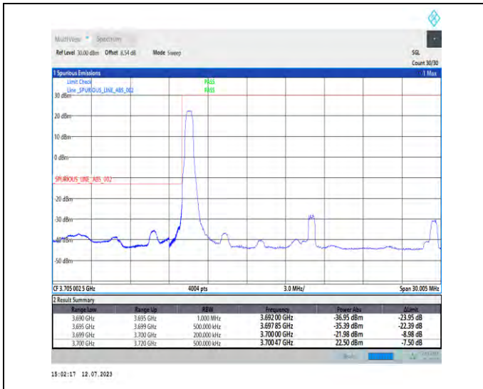
1-N77-3700-3980-PC1.5-30-20-L-4-CP-QPSK-Edge_1 RB_Left-1@0-Ant3-1--PASS-see graph
