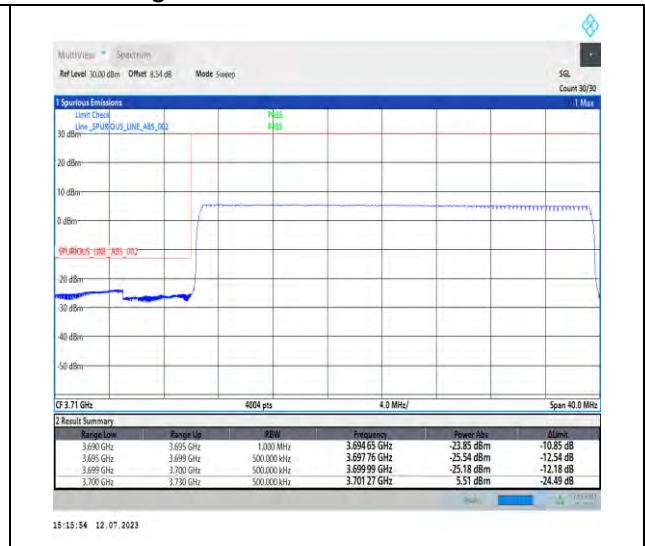
1-N77-3700-3980-PC1.5-30-30-L-6-CP-QPSK-Out er_Full-75@0-Ant3-1--PASS-see graph
