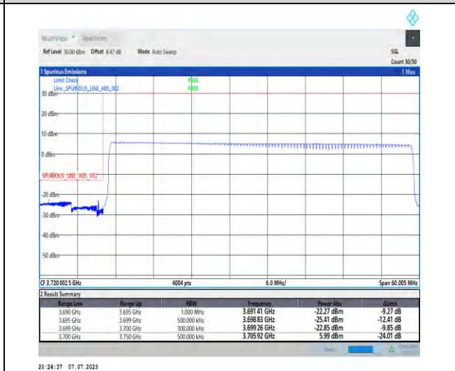
1-N77-3700-3980-PC1.5-30-50-L-6-CP-QPSK-Outer_Full-133@0-Ant3-1--PASS-see graph
