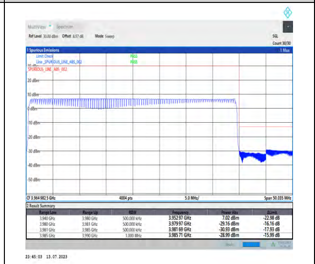
1-N77-3700-3980-PC1.5-30-40-H-6-CP-QPSK-Outer_Full-100@0-Ant3-1--PASS-see graph
