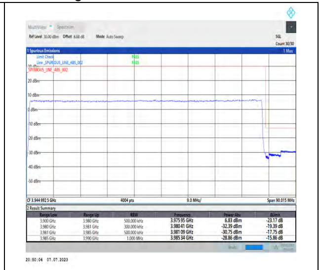
1-N77-3700-3980-PC1.5-30-80-H-3-DFT-PI2BPSK-Outer_Full-100@0-Ant3-1--PASS-see graph
