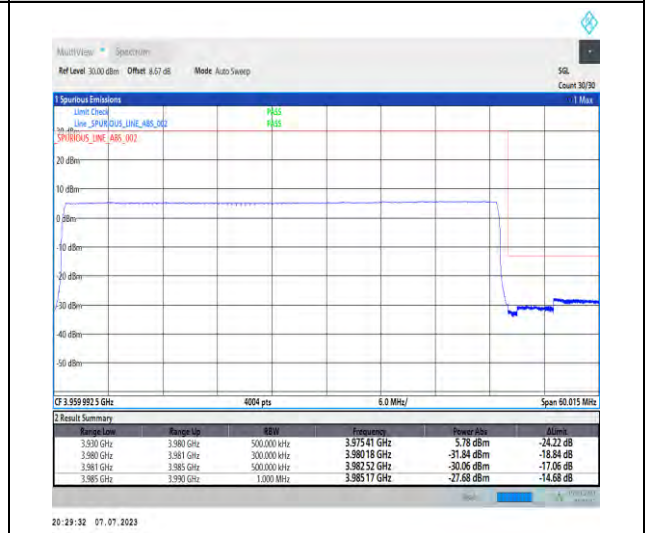
1-N77-3700-3980-PC1.5-30-50-H-6-CP-QPSK-Outer_Full-133@0-Ant3-1--PASS-see graph
