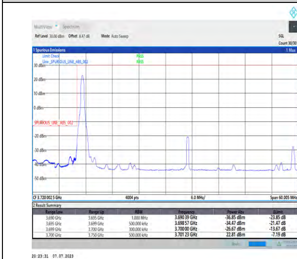
1-N77-3700-3980-PC1.5-30-50-L-4-CP-QPSK-Edge_1RB_Left-1@0-Ant3-1--PASS-see graph
