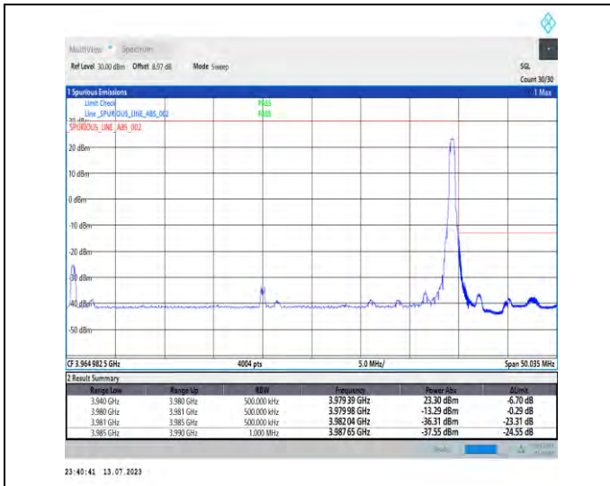
1-N77-3700-3980-PC1.5-30-40-H-2-DFT-PI2BPSK-Edge_1RB_Right-1@105-Ant3-1--PASS-see graph
