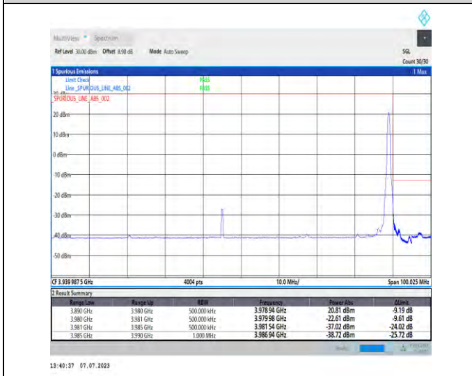
1-N77-3700-3980-PC1-30-90-H-2-DFT-PI2BPSK-Edge_1RB_Right-1@244-Ant3-1--PASS-see graph
