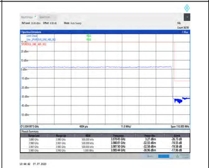
1-N77-3700-3980-PC1-30-100-H-3-DFT-PI2BPSK-Outer_Full-270@0-Ant3-1--PASS-see graph
