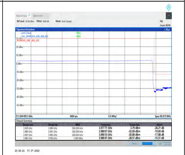
1-N77-3700-3980-PC1.5-30-80-H-6-CP-QPSK-Outer_Full-217@0-Ant3-1--PASS-see graph
