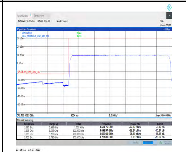
1-N77-3700-3980-PC1.5-30-20-L-6-CP-QPSK-Outer_Full-51@0-Ant3-1--PASS-see graph
