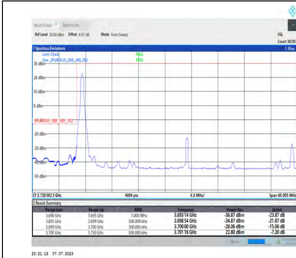
1-N77-3700-3980-PC1.5-30-50-L-1-DFT-PI2BPSK-Edge_1RB_Left-1@0-Ant3-1--PASS-see graph
