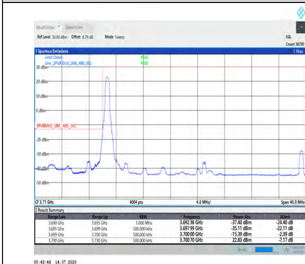
1-N77-3700-3980-PC1.5-30-30-L-4-CP-QPSK-Edge_1RB_Left-1@0-Ant3-1-PASS-see graph
