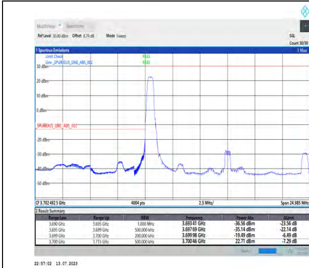
1-N77-3700-3980-PC1.5-30-15-L-1-DFT-PI2BPSK-Edge_1RB_Left-1@0-Ant3-1-PASS-see graph
