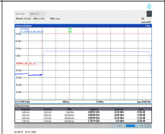
1-N77-3700-3980-PC1.5-30-40-L-6-CP-QPSK-Outer_Full-100@0-Ant3-1--PASS-see graph
