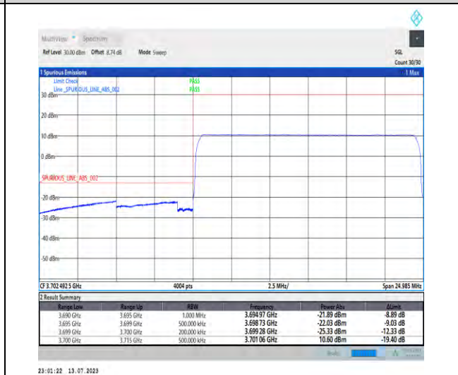
1-N77-3700-3980-PC1.5-30-15-L-6-CP-QPSK-Outer_Full-38@0-Ant3-1-PASS-see graph
