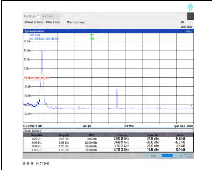
1-N77-3700-3980-PC1-30-90-L-4-CP-QPSK-Edge_1R_B_Left-1@0-Ant3-1--PASS-see graph
