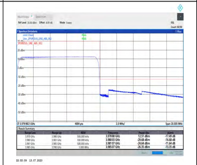
1-N77-3700-3980-PC1.5-30-10-H-6-CP-QPSK-Outer_Full-24@0-Ant3-1--PASS-see graph
