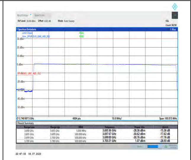
1-N77-3700-3980-PC1-30-90-L-6-CP-QPSK-Outer_Full-245@0-Ant3-1--PASS-see graph
