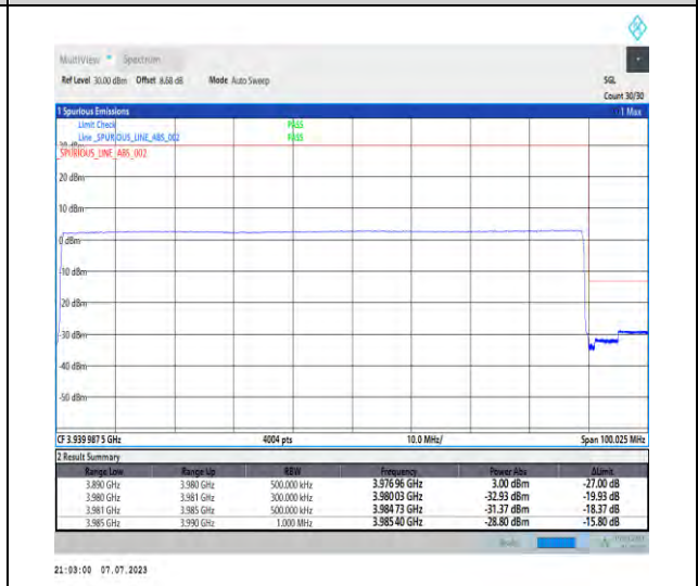
1-N77-3700-3980-PC1.5-30-90-H-6-CP-QPSK-Outer_Full-245@0-Ant3-1--PASS-see graph
