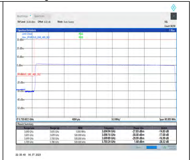
1-N77-3700-3980-PC1-30-80-L-6-CP-QPSK-Outer_Full-217@0-Ant3-1--PASS-see graph
