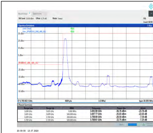
1-N77-3700-3980-PC1.5-30-20-L-1-DFT-PI2BPSK-Edge_1RB_Left-1@0-Ant3-1--PASS-see graph
