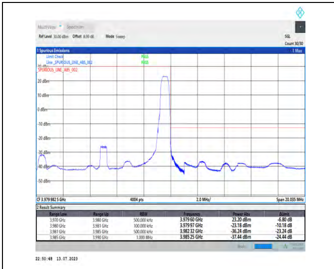
1-N77-3700-3980-PC1.5-30-10-H-2-DFT-PI2BPSK-Edge_1RB_Right-1@23-Ant3-1--PASS-see graph
