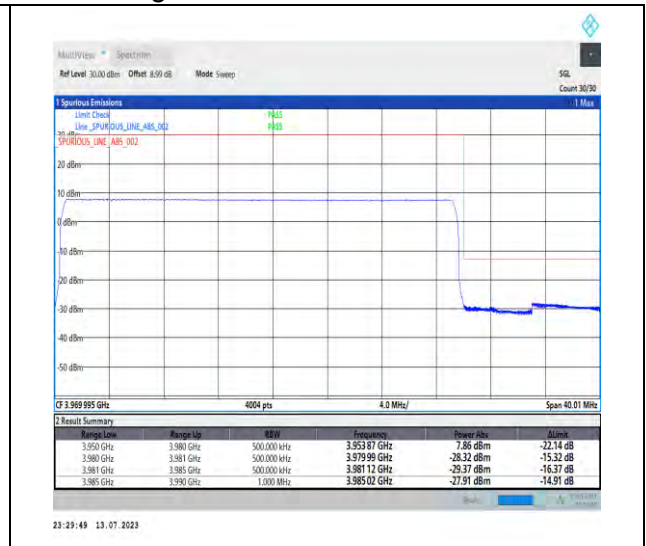
1-N77-3700-3980-PC1.5-30-30-H-3-DFT-PI2BPSK-Outer_Full-75@0-Ant3-1--PASS-see graph
