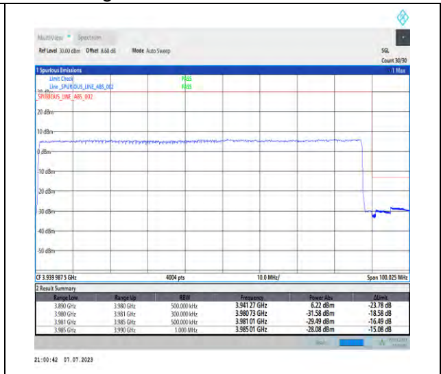
1-N77-3700-3980-PC1.5-30-90-H-3-DFT-PI2BPSK-Outer_Full-240@0-Ant3-1--PASS-see graph
