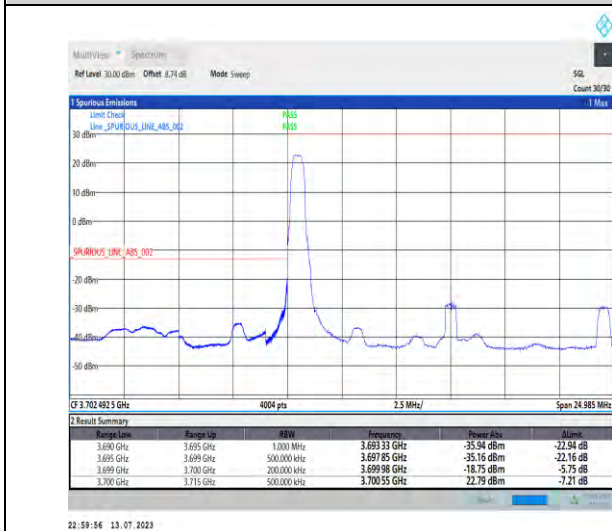
1-N77-3700-3980-PC1.5-30-15-L-4-CP-QPSK-Edge_1RB_Left-1@0-Ant3-1-PASS-see graph
