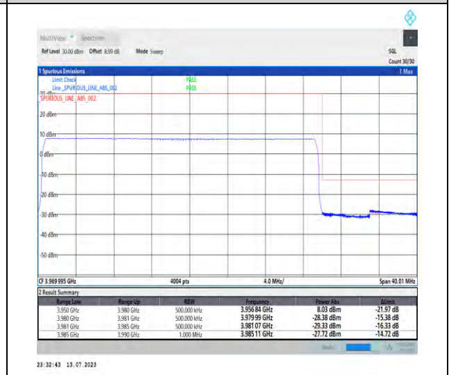
1-N77-3700-3980-PC1.5-30-30-H-6-CP-QPSK-Outer_Full-75@0-Ant3-1--PASS-see graph
