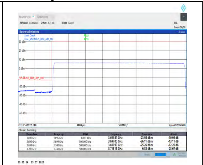
1-N77-3700-3980-PC1.5-30-40-L-3-DFT-PI2BPSK-Outer_Full-100@0-Ant3-1--PASS-see graph
