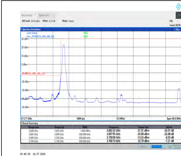
1-N77-3700-3980-PC1.5-30-30-L-1-DFT-PI2BPSK-Edge_1RB_Left-1@0-Ant3-1-PASS-see graph
