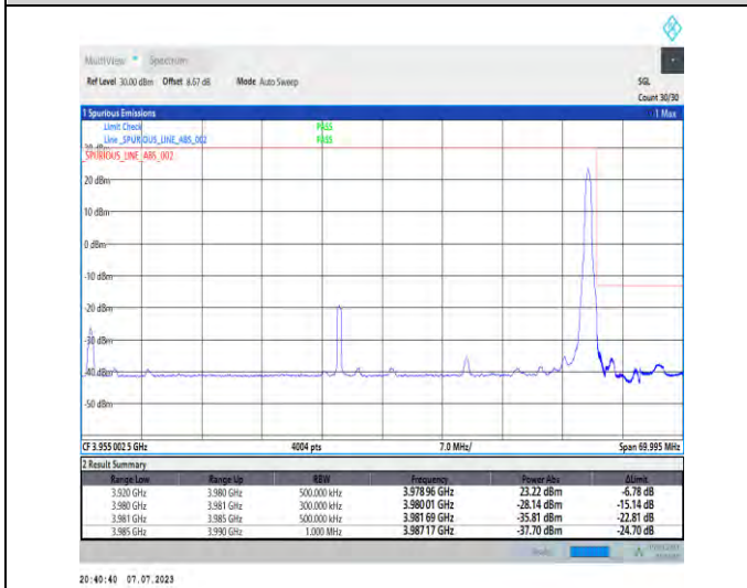
1-N77-3700-3980-PC1.5-30-60-H-5-CP-QPSK-Edge_1RB_Right-1@161-Ant3-1--PASS-see graph
