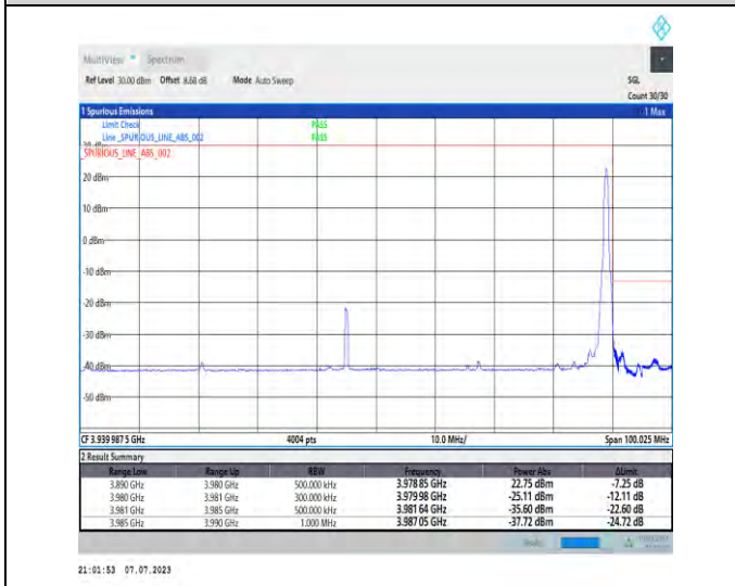
1-N77-3700-3980-PC1.5-30-90-H-5-CP-QPSK-Edge_1RB_Right-1@244-Ant3-1--PASS-see graph
