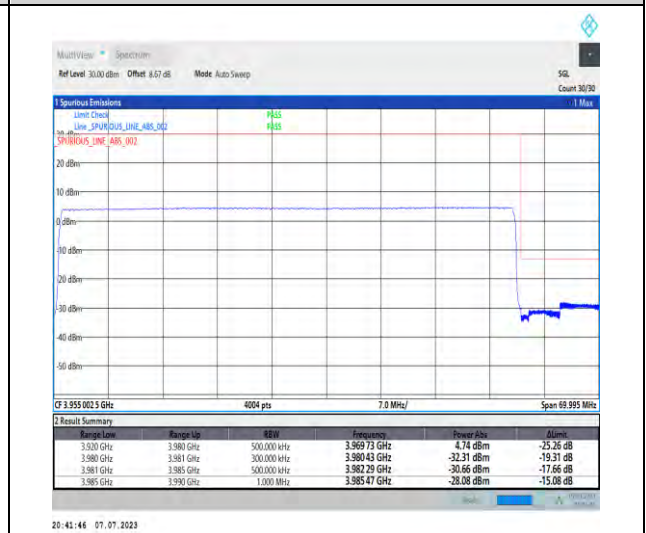
1-N77-3700-3980-PC1.5-30-60-H-6-CP-QPSK-Outer_Full-162@0-Ant3-1--PASS-see graph
