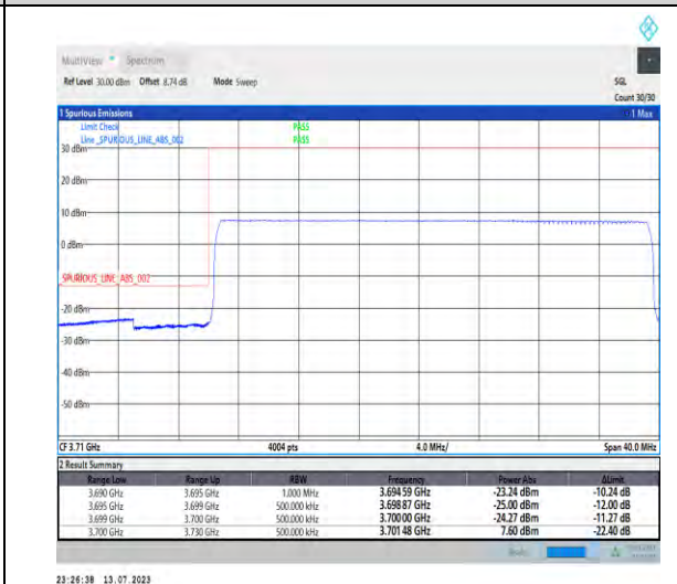
1-N77-3700-3980-PC1.5-30-30-L-6-CP-QPSK-Outer_Full-75@0-Ant3-1-PASS-see graph
