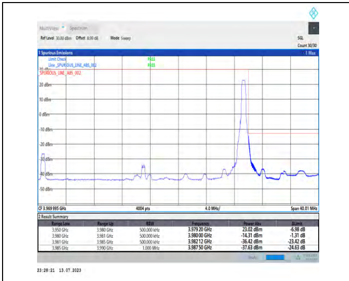
1-N77-3700-3980-PC1.5-30-30-H-2-DFT-PI2BPSK-Edge_1RB_Right-1@77-Ant3-1--PASS-see graph
