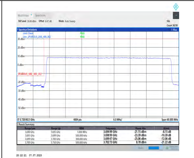
1-N77-3700-3980-PC1.5-30-50-L-3-DFT-PI2BPSK-Outer_Full-128@0-Ant3-1--PASS-see graph
