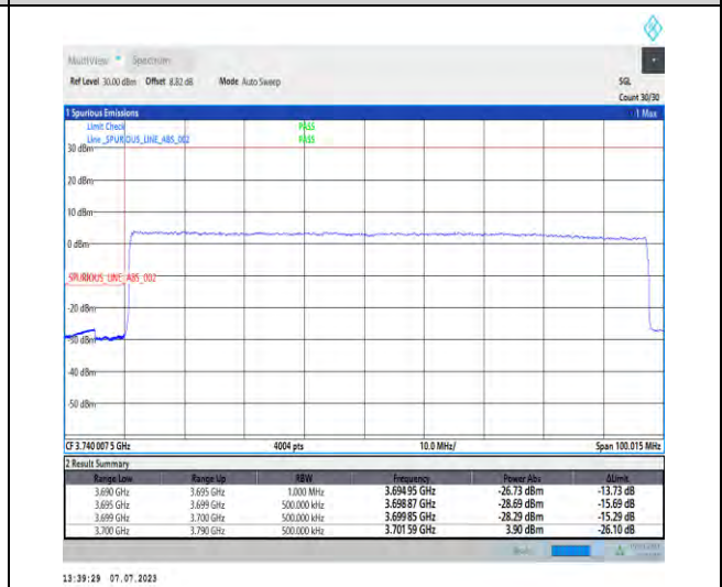
1-N77-3700-3980-PC1-30-90-L-3-DFT-PI2BPSK-Outer_Full-240@0-Ant3-1--PASS-see graph
