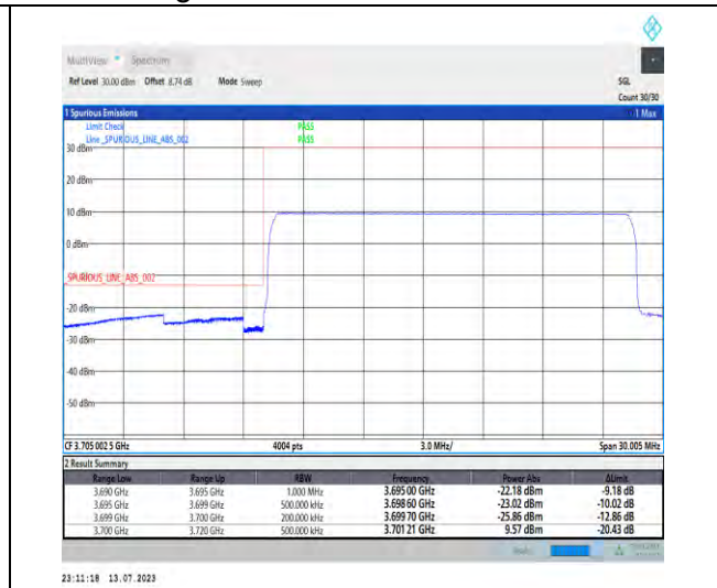
1-N77-3700-3980-PC1.5-30-20-L-3-DFT-PI2BPSK-Outer_Full-50@0-Ant3-1--PASS-see graph
