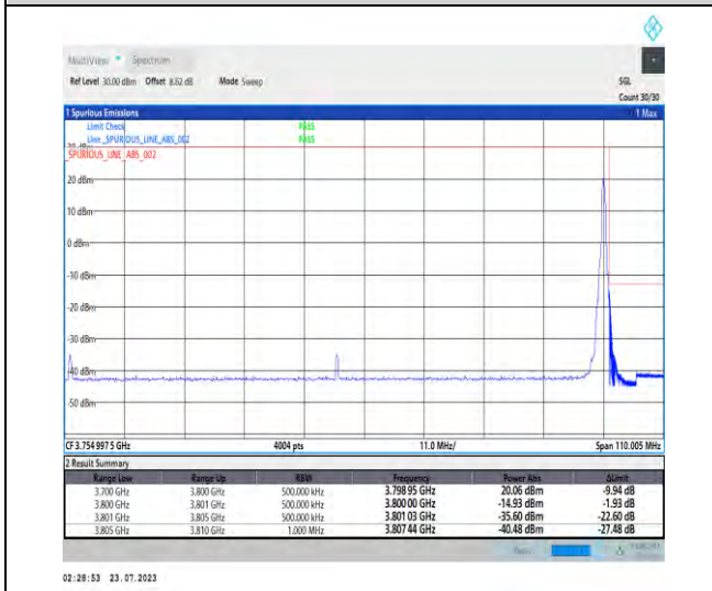
1-N77-3700-3980-PC1-30-100-H-2-DFT-PI2BPSK-Outer_Full-1@0-Ant3-1--PASS-see graph
