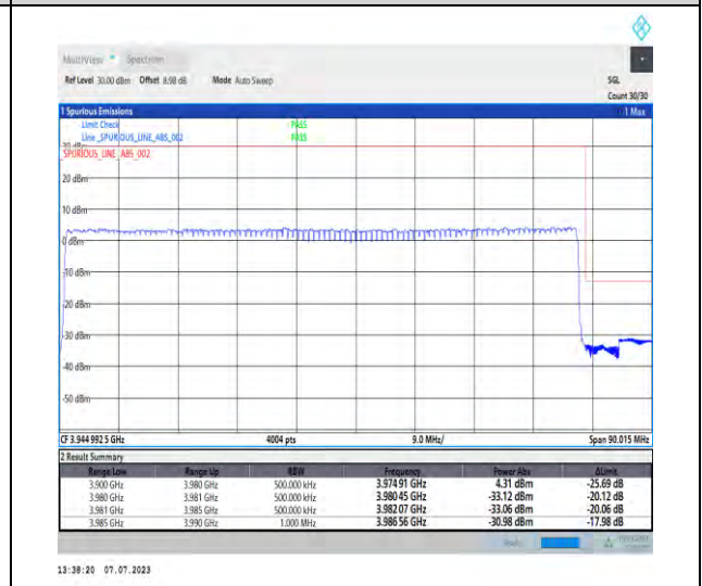
1-N77-3700-3980-PC1-30-80-H-3-DFT-PI2BPSK-Outer_Full-100@0-Ant3-1--PASS-see graph
