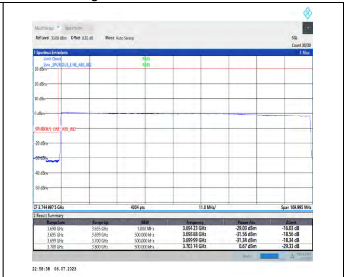
1-N77-3700-3980-PC1-30-100-L-6-CP-QPSK-Outer_Full-273@0-Ant3-1--PASS-see graph
