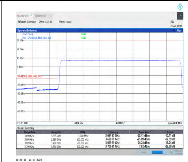
1-N77-3700-3980-PC1.5-30-30-L-3-DFT-PI2BPSK-Outer_Full-75@0-Ant3-1-PASS-see graph
