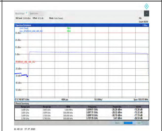
1-N77-3700-3980-PC1.5-30-90-L-6-CP-QPSK-Outer_Full-245@0-Ant3-1--PASS-see graph
