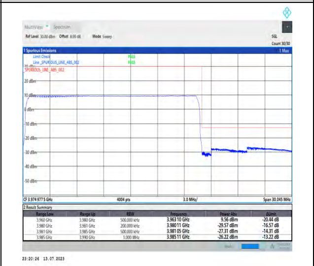
1-N77-3700-3980-PC1.5-30-20-H-6-CP-QPSK-Outer_Full-51@0-Ant3-1--PASS-see graph
