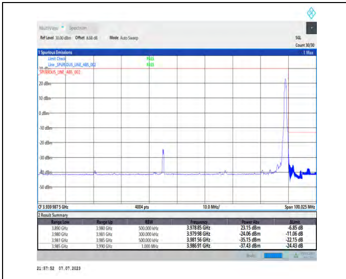
1-N77-3700-3980-PC1.5-30-90-H-2-DFT-PI2BPSK-Edge_1RB_Right-1@244-Ant3-1--PASS-see graph
