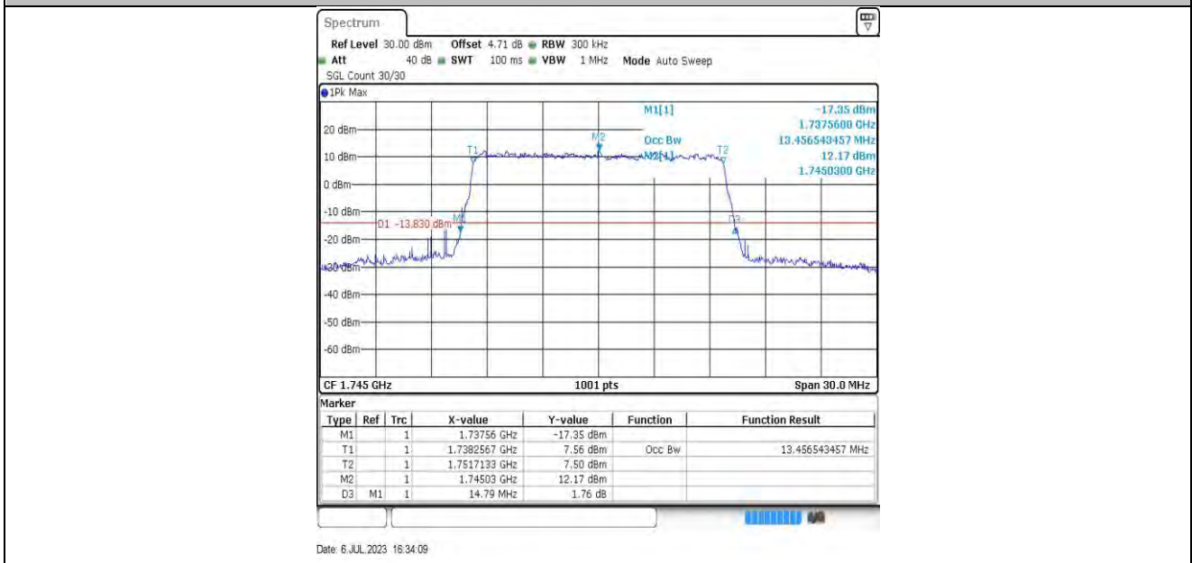
15MHz-132322 64QAM
