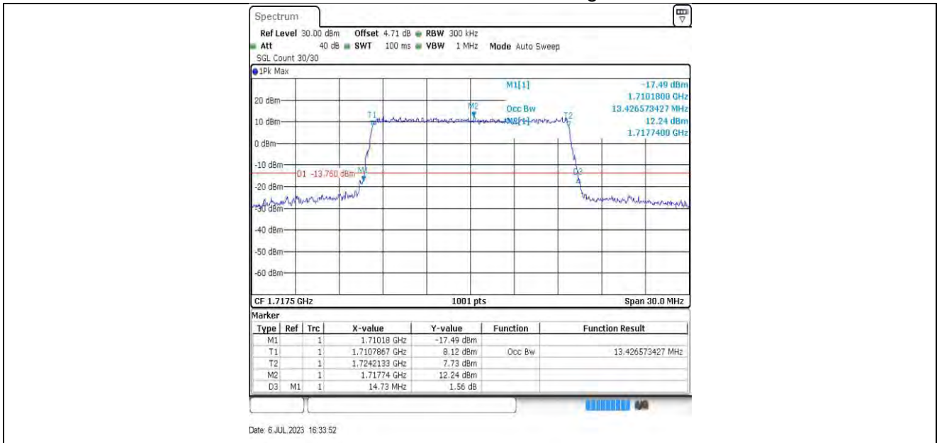
15MHz-132047 64QAM
