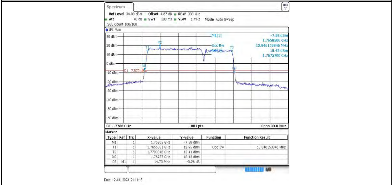
10MHz-5MHz-132572-132644 16QAM-16QAM
