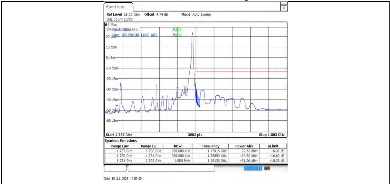
15MHz-5MHz_QPSK@QPSK-QPSK@QPSK_132549-132642_0RB#0@75RB#0-1RB#24@25RB#0
