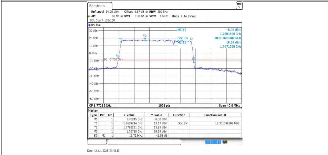
15MHz-5MHz-132549-132642 16QAM-16QAM
