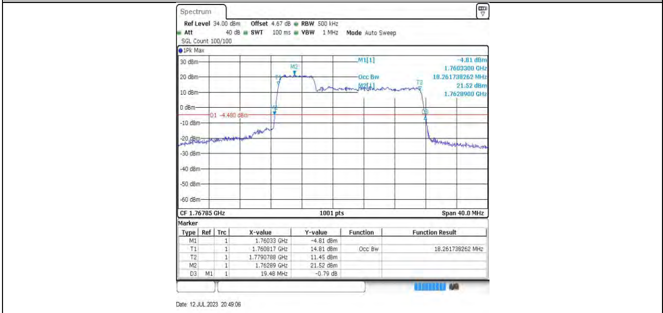
5MHz-15MHz-132504-132597 16QAM-16QAM
