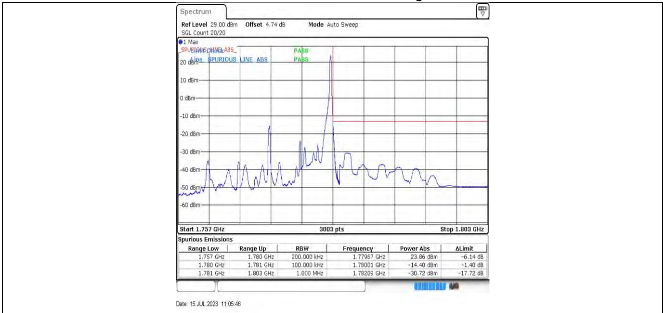
5MHz-5MHz_QPSK@QPSK-QPSK@QPSK_132599-132647_0RB#0@25RB#0-1RB#24@25RB#0
