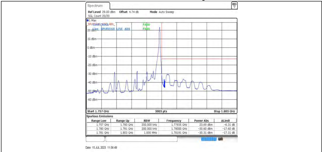
10MHz-5MHz_QPSK@QPSK-QPSK@QPSK_132572-132644_0RB#0@50RB#0-1RB#24@25RB#0
