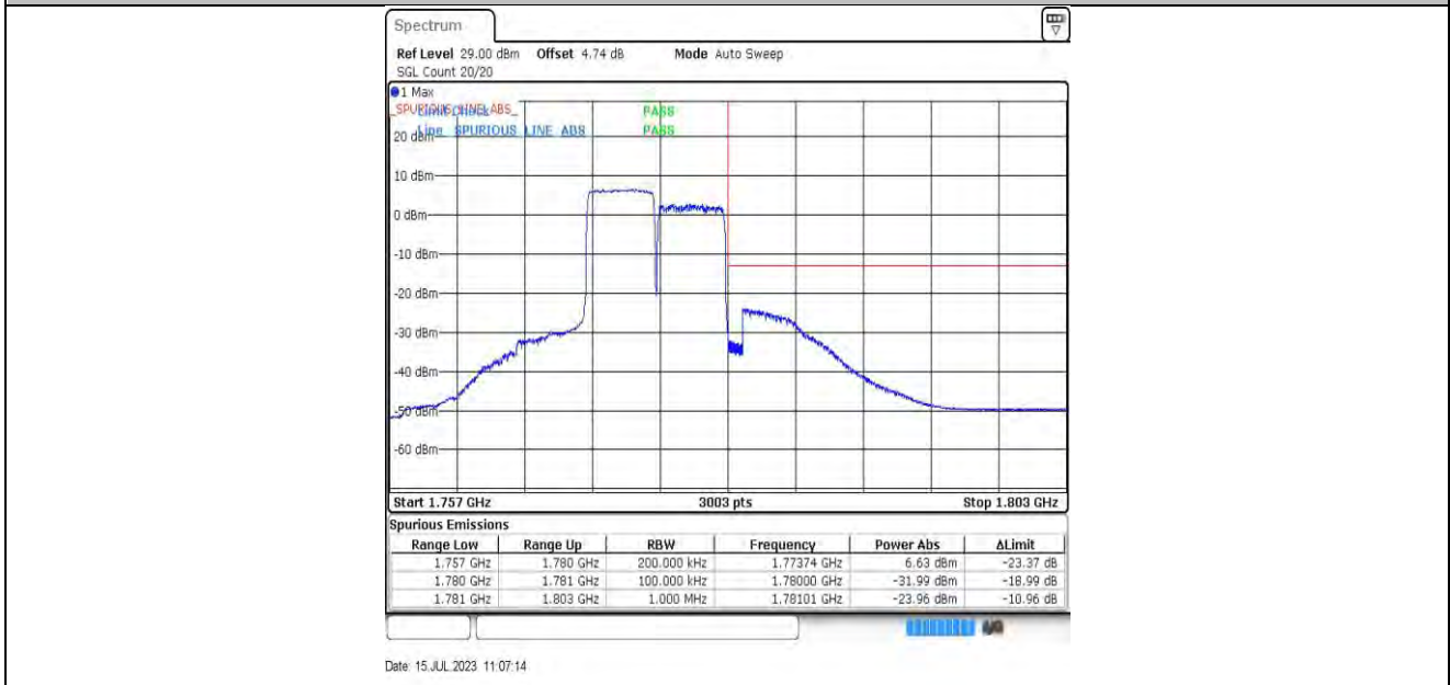
5MHz-5MHz_QPSK@QPSK-QPSK@QPSK_132599-132647_25RB#0@25RB#0-25RB#0@25RB#0
