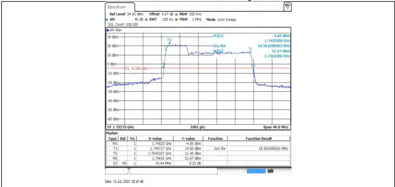
5MHz-15MHz-132353-132446 16QAM-16QAM
