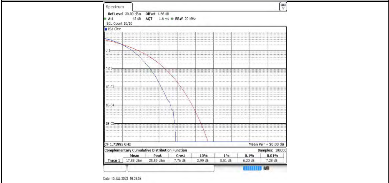
10MHz-10MHz-132022-132121 256QAM-256QAM
