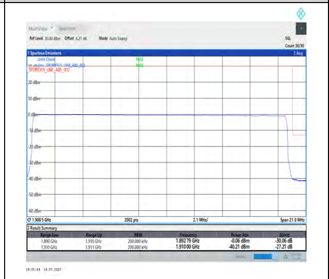
1-N2-PC3-15-20-H-6-CP-QPSK-Outer_Full-106@0-Ant3-1-seegraph-PASS-see graph
