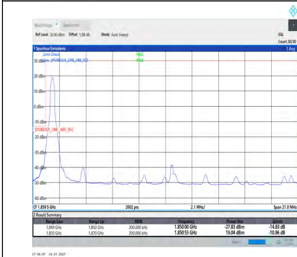
1-N2-PC3-15-20-L-4-CP-QPSK-Edge_1RB_Left-1@0-Ant3-1-seegraph-PASS-see graph
