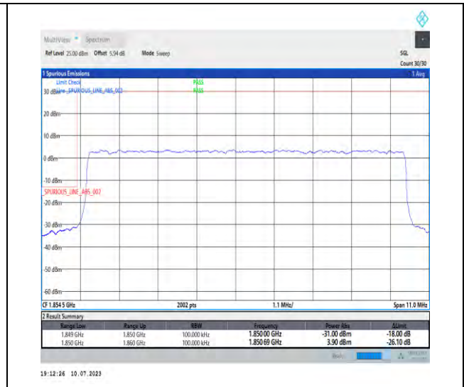
1-N2-PC3-15-10-L-3-DFT-PI2BPSK-Outer_Full-50 @0-Ant3-1-seegraph-PASS-see graph
