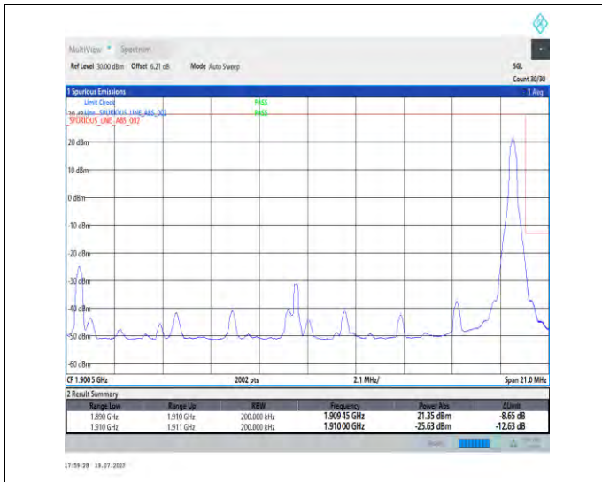
1-N2-PC3-15-20-H-2-DFT-PI2BPSK-Edge_1RB_Right-1@105-Ant3-1-seegraph-PASS-see graph
