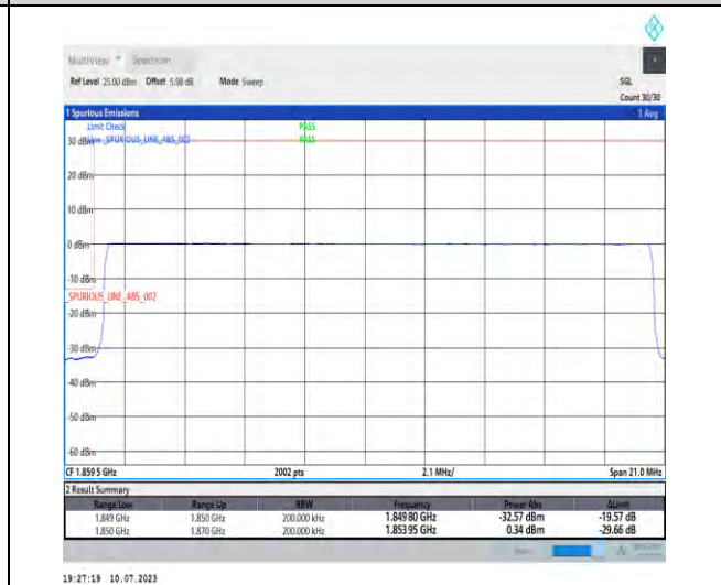
1-N2-PC3-15-20-L-6-CP-QPSK-Outer_Full-106@0-Ant3-1-seegraph-PASS-see graph
