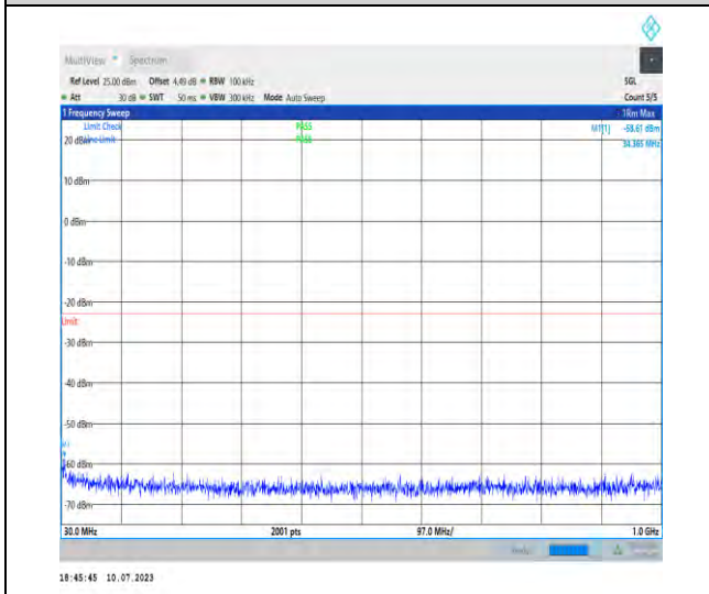
1-N2-PC3-15-20-H-1-DFT-PI2BPSK-Inner_1RB_Lef t-1@1-30-1000-Ant3-34.37--58.61--23-PASS
