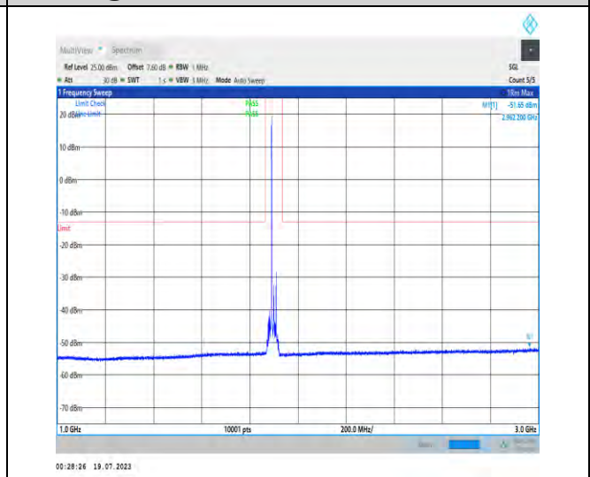
1-N2-PC3-15-20-H-1-DFT-PI2BPSK-Inner_1RB_Left -1@1-1000-3000-Ant3-2962.2--51.65--13-PASS
