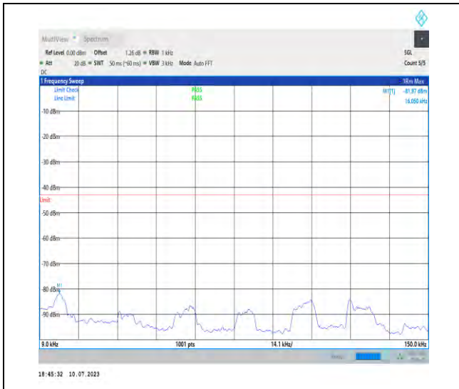
1-N2-PC3-15-20-H-1-DFT-PI2BPSK-Inner_1RB_Lef t-1@1-0.009-0.15-Ant3-0.02--81.97--43-PASS
