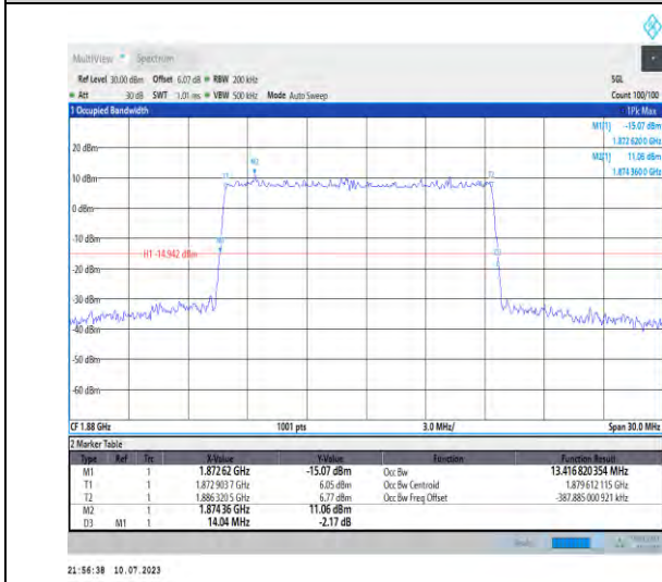
1-N2-PC3-15-15-M-5-DFT-256QAM-Outer_Full-75@0-Ant3-13.417-14.040-≤15-PASS
