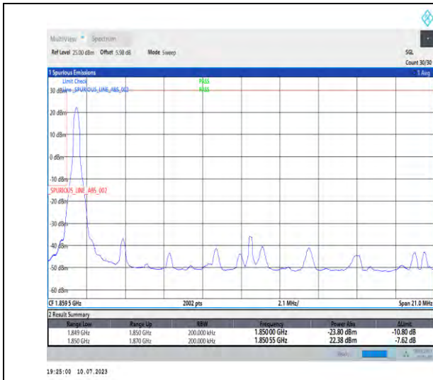
1-N2-PC3-15-20-L-1-DFT-PI2BPSK-Edge_1RB_Left-1@0-Ant3-1-seegraph-PASS-see graph
