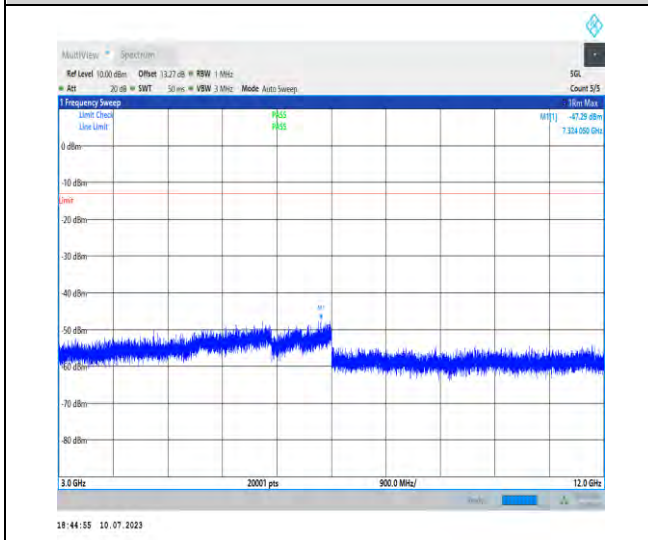
1-N2-PC3-15-20-M-1-DFT-PI2BPSK-Inner_1RB_Lef t-1@1-3000-12000-Ant3-7324.05--47.29--13-PASS
