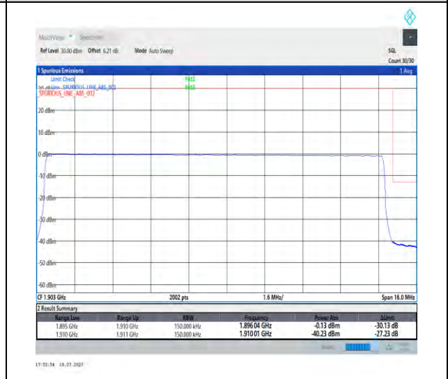
1-N2-PC3-15-15-H-6-CP-QPSK-Outer_Full-79@0-Ant3-1-seegraph-PASS-see graph
