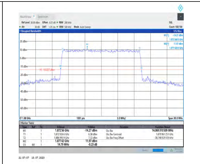
1-N2-PC3-15-15-M-8-CP-64QAM-Outer_Full-79@0- Ant3-14.069-14.790-≤15-PASS
