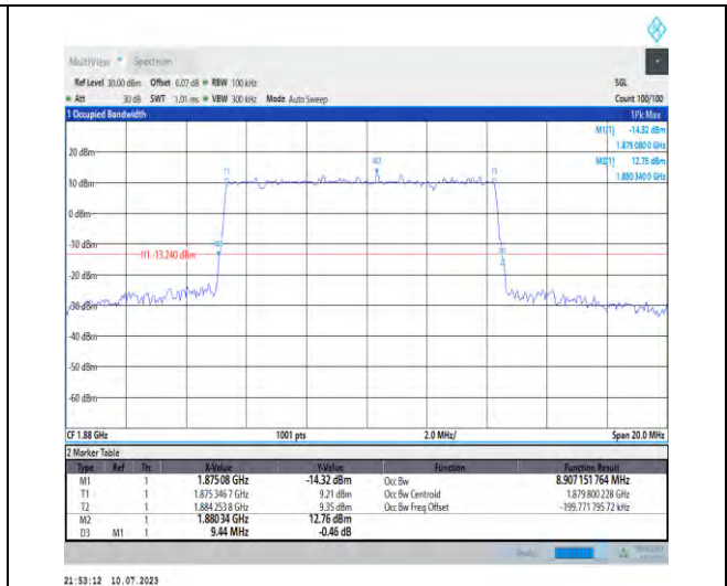
1-N2-PC3-15-10-M-1-DFT-QPSK-Outer_Full-50@0-Ant3-8.907-9.440-≤10-PASS
