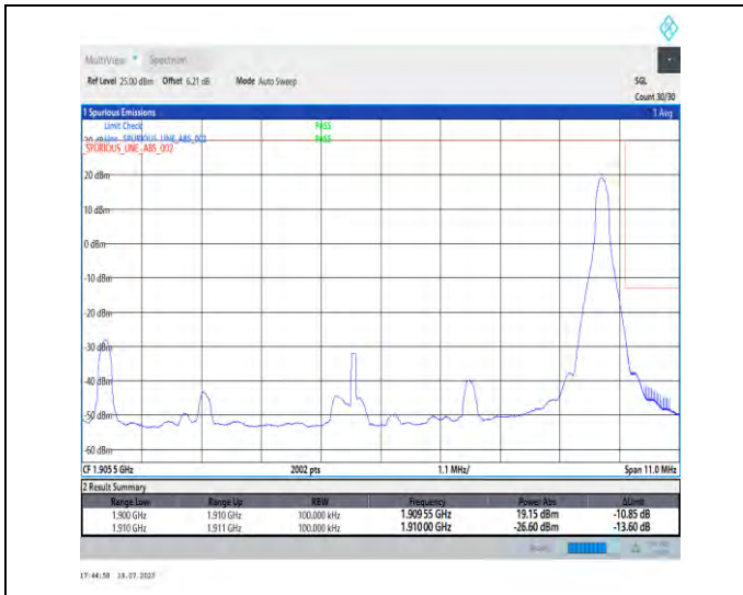
1-N2-PC3-15-10-H-2-DFT-PI2BPSK-Edge_1RB_Right-1@51-Ant3-1-seegraph-PASS-see graph
