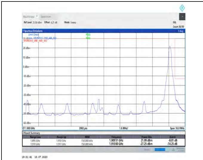
1-N2-PC3-15-15-H-2-DFT-PI2BPSK-Edge_1RB_Right-1@78-Ant3-1-seegraph-PASS-see graph
