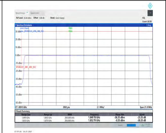
1-N2-PC3-15-20-L-6-CP-QPSK-Outer_Full-106@0-Ant3-1-seegraph-PASS-see graph
