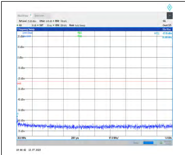
1-N2-PC3-15-20-M-1-DFT-PI2BPSK-Inner_1RB_Lef t-1@1-30-1000-Ant3-33.40--57.05--23-PASS
