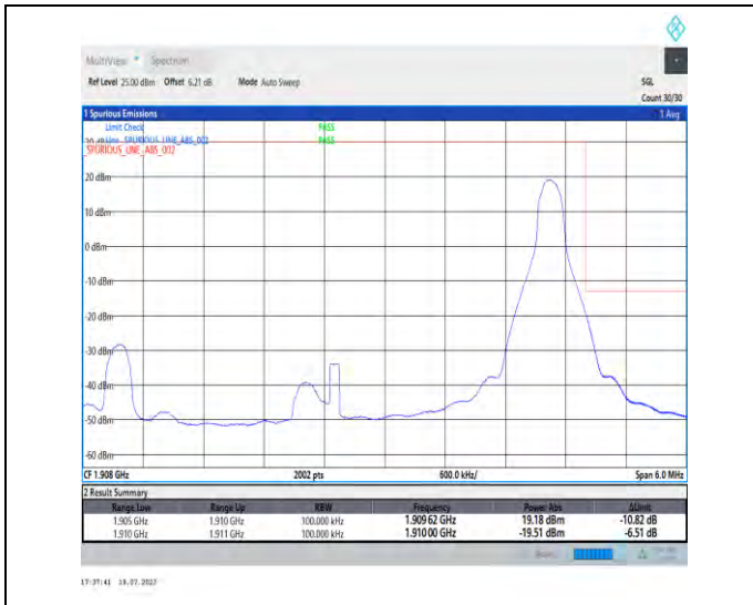
1-N2-PC3-15-5-H-2-DFT-PI2BPSK-Edge_1RB_Right-1 @24-Ant3-1-seegraph-PASS-see graph
