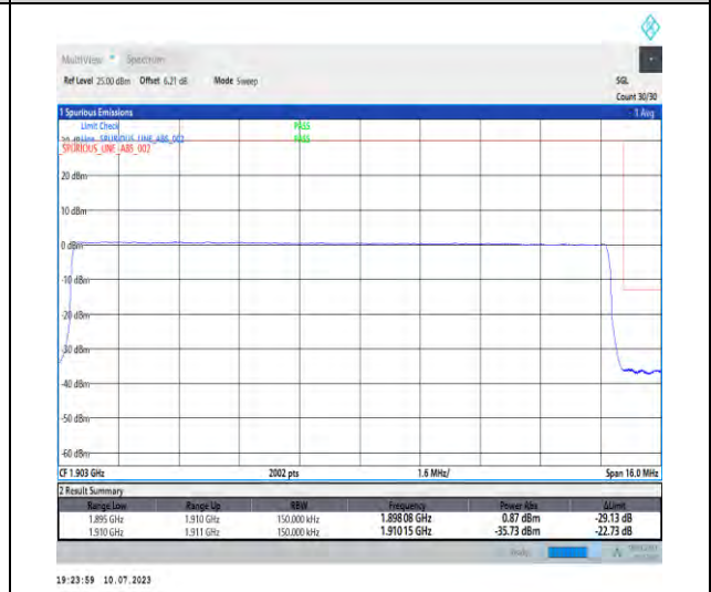
1-N2-PC3-15-15-H-6-CP-QPSK-Outer_Full-79@0-Ant3-1-seegraph-PASS-see graph
