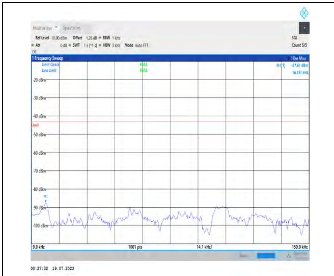
1-N2-PC3-15-20-H-1-DFT-PI2BPSK-Inner_1RB_Left -1@1-0.009-0.15-Ant3-16.191--87.61--43-PASS
