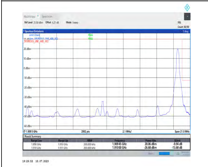
1-N2-PC3-15-20-H-5-CP-QPSK-Edge_1RB_Right-1@105-Ant3-1-seegraph-PASS-see graph
