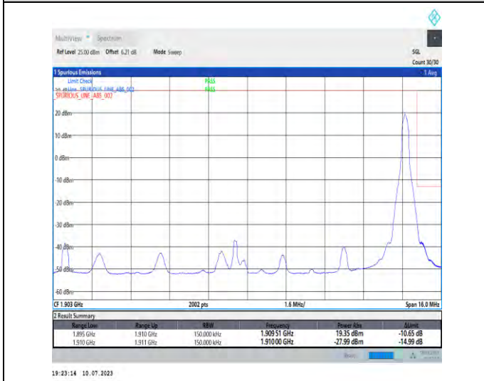
1-N2-PC3-15-15-H-5-CP-QPSK-Edge_1RB_Right-1@78-Ant3-1-seegraph-PASS-see graph
