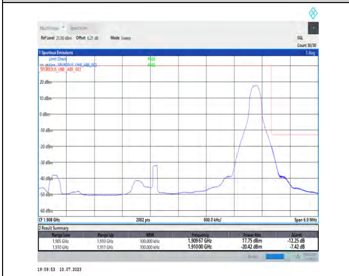
1-N2-PC3-15-5-H-5-CP-QPSK-Edge_1RB_Right-1@24 4-Ant3-1-seegraph-PASS-see graph
