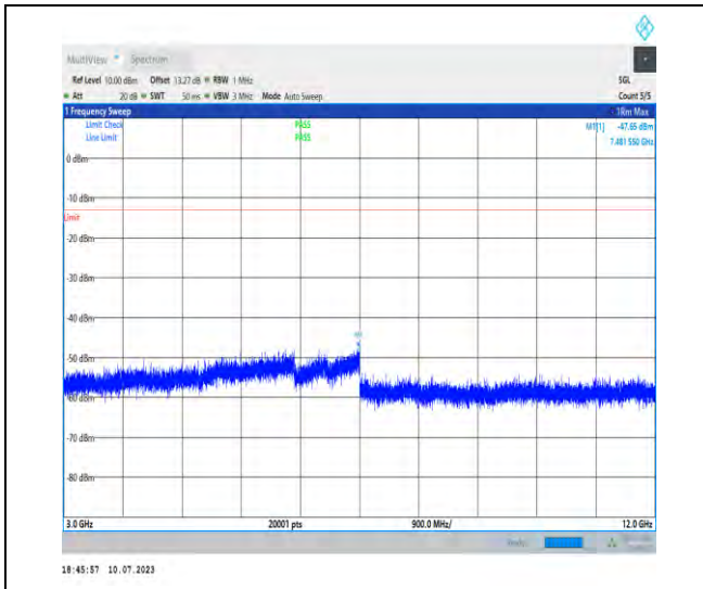
1-N2-PC3-15-20-H-1-DFT-PI2BPSK-Inner_1RB_Lef t-1@1-3000-12000-Ant3-7481.55--47.65--13-PASS
