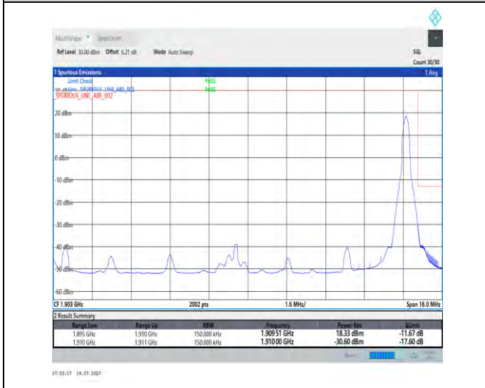
1-N2-PC3-15-15-H-5-CP-QPSK-Edge_1RB_Right-1@78-Ant3-1-seegraph-PASS-see graph
