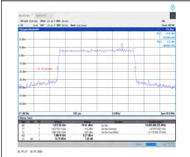
1-N2-PC3-15-15-M-9-CP-256QAM-Outer_Full-79@0 -Ant3-14.095-14.790-≤15-PASS
