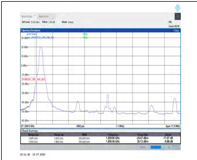
1-N2-PC3-15-10-L-1-DFT-PI2BPSK-Edge_1RB_Left-1 @0-Ant3-1-seegraph-PASS-see graph
