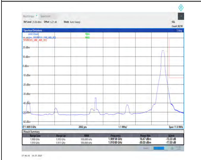
1-N2-PC3-15-10-H-5-CP-QPSK-Edge_1RB_Right-1@51-Ant3-1-seegraph-PASS-see graph
