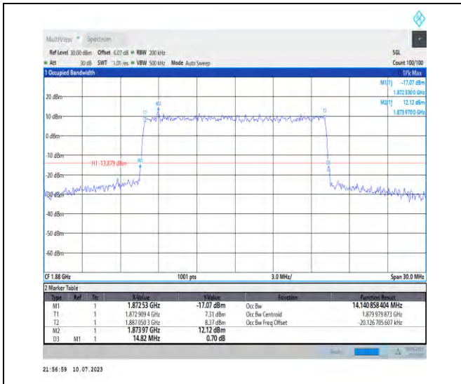
1-N2-PC3-15-15-M-7-CP-16QAM-Outer_Full-79@0- Ant3-14.141-14.820-≤15-PASS
