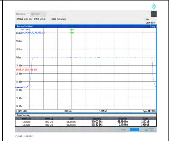
1-N2-PC3-15-10-L-6-CP-QPSK-Outer_Full-52@0-A nt3-1-seegraph-PASS-see graph
