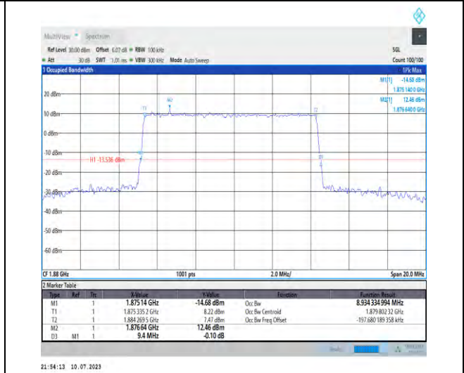
1-N2-PC3-15-10-M-3-DFT-16QAM-Outer_Full-50@0-Ant3-8.934-9.400-≤10-PASS
