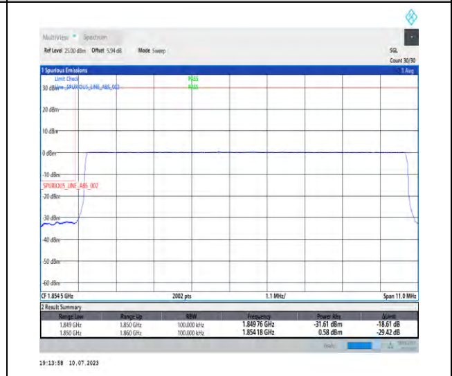
1-N2-PC3-15-10-L-6-CP-QPSK-Outer_Full-52@0-Ant3-1-seegraph-PASS-see graph
