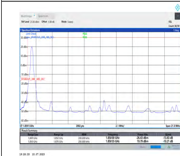
1-N2-PC3-15-20-L-4-CP-QPSK-Edge_1RB_Left-1@0-Ant3-1-seegraph-PASS-see graph
