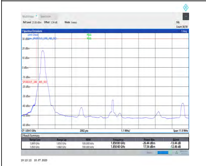
1-N2-PC3-15-10-L-4-CP-QPSK-Edge_1RB_Left-1@0 -Ant3-1-seegraph-PASS-see graph
