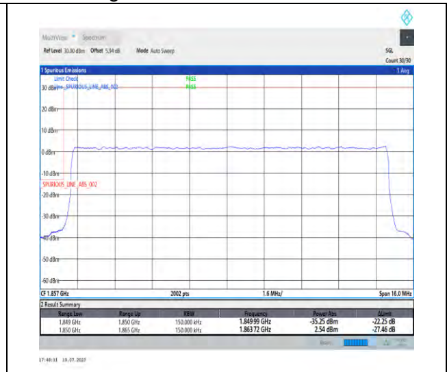
1-N2-PC3-15-15-L-3-DFT-PI2BPSK-Outer_Full-75 @0-Ant3-1-seegraph-PASS-see graph
