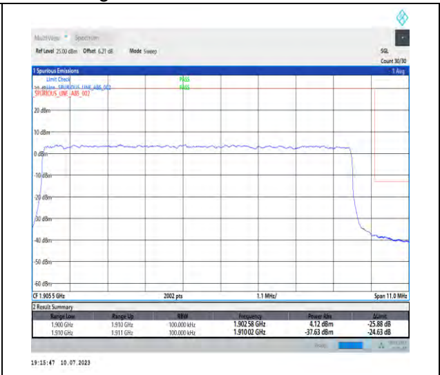
1-N2-PC3-15-10-H-3-DFT-PI2BPSK-Outer_Full-50@0-Ant3-1-seegraph-PASS-see graph
