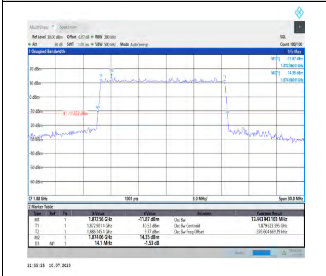
1-N2-PC3-15-15-M-1-DFT-QPSK-Outer_Full-75@0- Ant3-13.444-14.100-≤15-PASS
