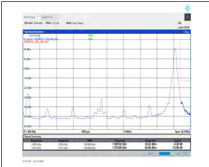
1-N2-PC3-15-15-H-2-DFT-PI2BPSK-Edge_1RB_Right-1@78-Ant3-1-seegraph-PASS-see graph
