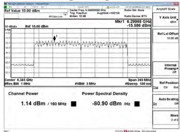
Channel Power+PSD_802.11be160_802.11be160 6345MHz
