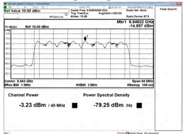
Channel Power+PSD_802.11be40_802.11be40 6845MHz
