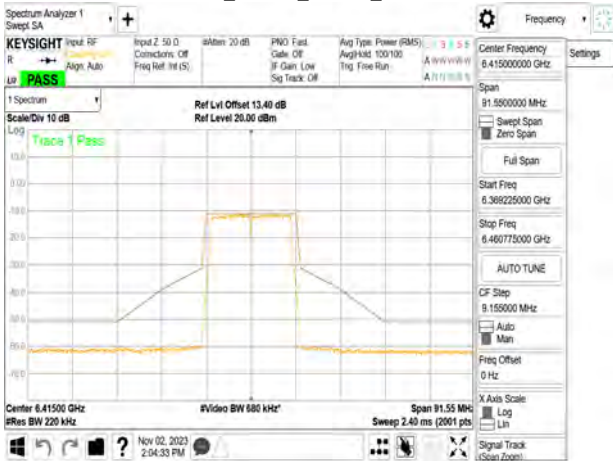
802.11a_20MHz_Chain0_6415MHz
