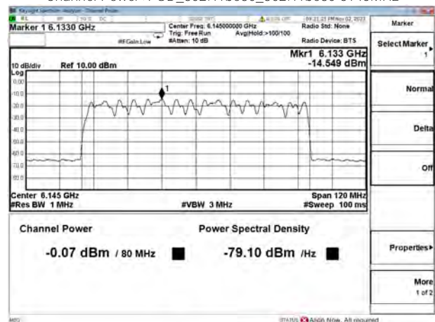
Channel Power+PSD_802.11be80_802.11be80 6145MHz
