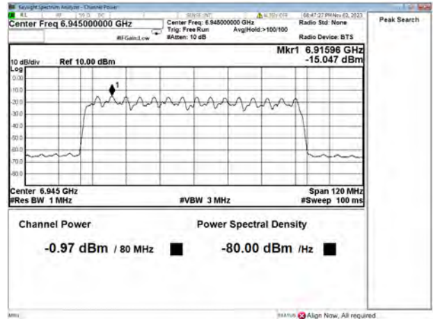
Channel Power+PSD_802.11ac80_802.11ac80 6945MHz
