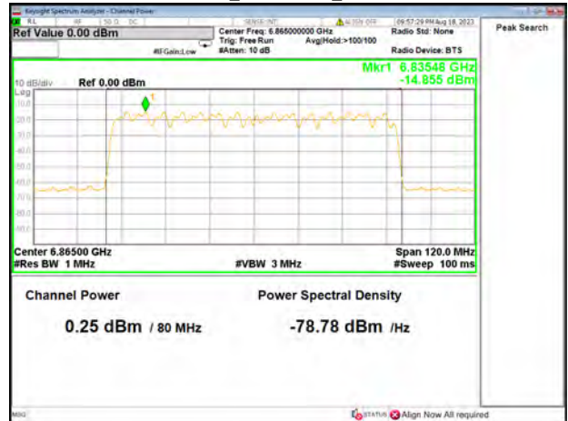
Channel Power+PSD_802.11ac80_802.11ac80 6865MHz
