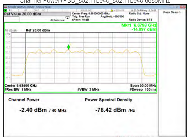
Channel Power+PSD_802.11be40_802.11be40 6685MHz
