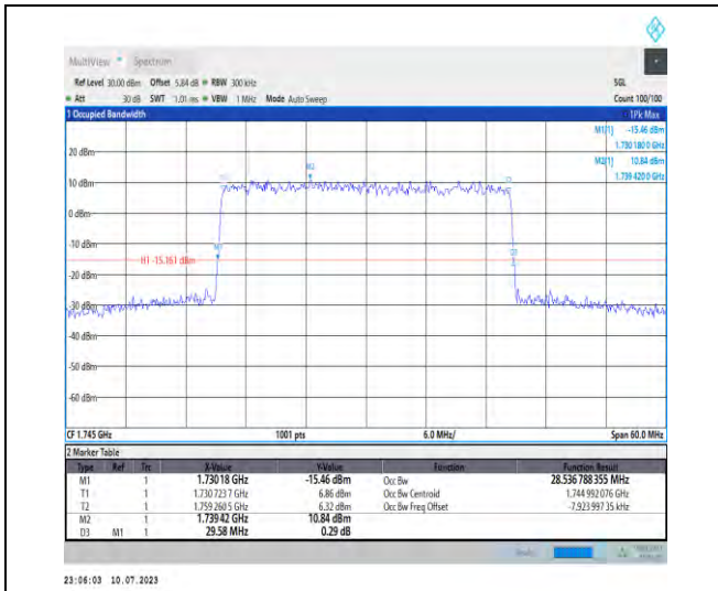
1-N66-PC3-15-30-M-4-DFT-64QAM-Outer_Full-160 @0-Ant3-28.537-29.580-≤30-PASS
