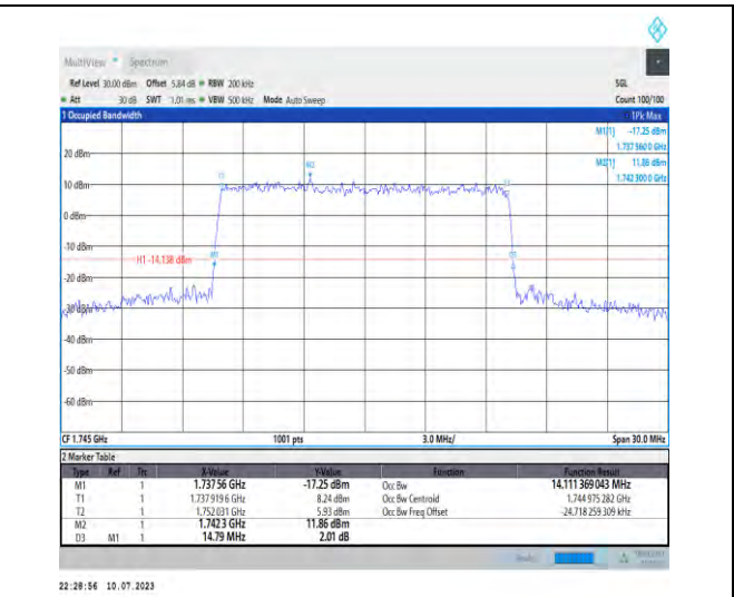
1-N66-PC3-15-15-M-8-CP-64QAM-Outer_Full-79@0 -Ant3-14.111-14.790-≤15-PASS
