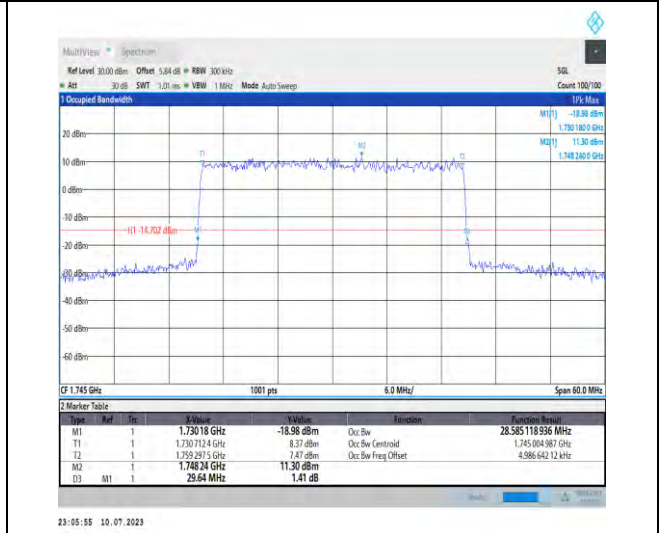
1-N66-PC3-15-30-M-3-DFT-16QAM-Outer_Full-160 @0-Ant3-28.585-29.640-≤30-PASS
