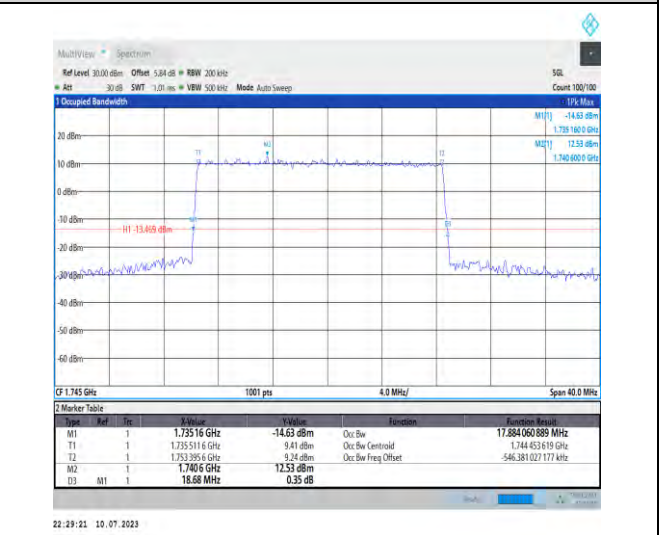
1-N66-PC3-15-20-M-1-DFT-QPSK-Outer_Full-100@0 -Ant3-17.884-18.680-≤20-PASS
