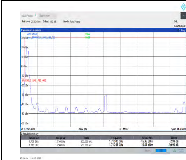
1-N66-PC3-15-40-L-4-CP-QPSK-Edge_1RB_Left-1@0-Ant3-1-seegraph-PASS-see graph
