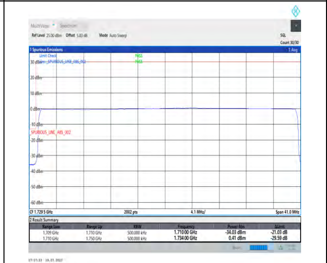
1-N66-PC3-15-40-L-6-CP-QPSK-Outer_Full-216@0-Ant3-1-seegraph-PASS-see graph
