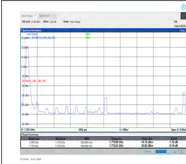
1-N66-PC3-15-40-L-1-DFT-PI2BPSK-Edge_1RB_Left-1@0-Ant3-1-seegraph-PASS-see graph
