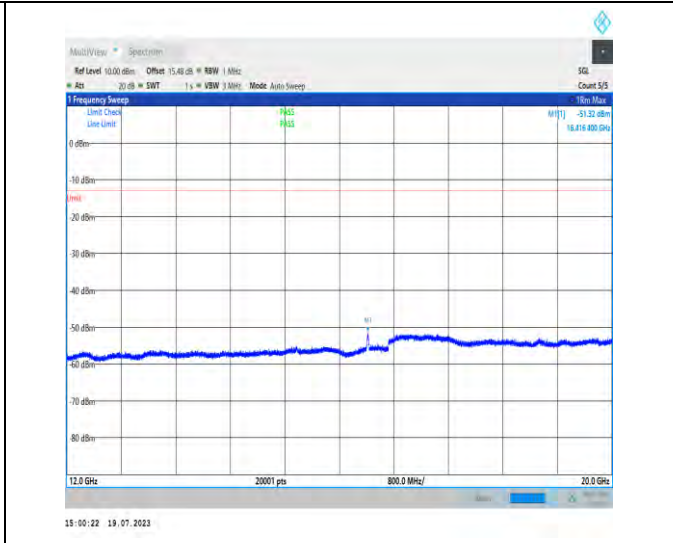
1-N66-PC3-15-40-H-1-DFT-PI2BPSK-Inner_1RB_Left -1@1-12000-20000-Ant3-16416.40--51.32--13-PASS
