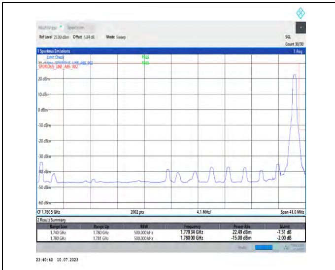
1-N66-PC3-15-40-H-2-DFT-PI2BPSK-Edge_1RB_Right-t-1@215-Ant3-1-seegraph-PASS-see graph
