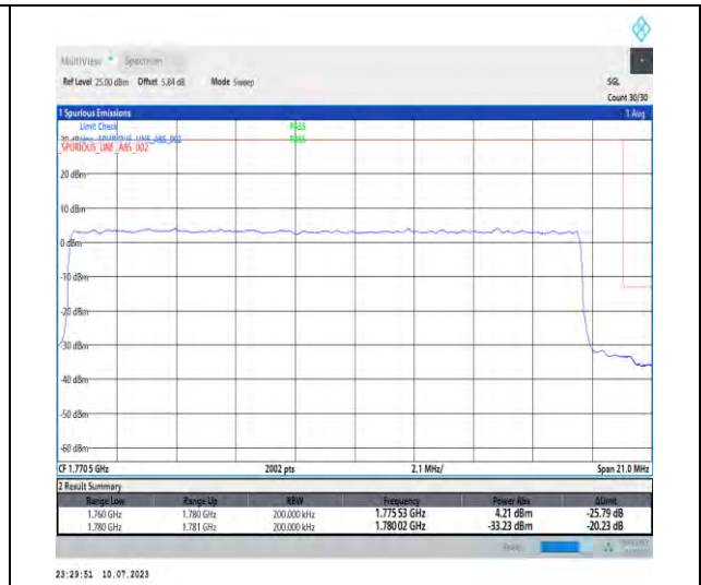
1-N66-PC3-15-20-H-3-DFT-PI2BPSK-Outer_Full-100@0-Ant3-1-seegraph-PASS-see graph
