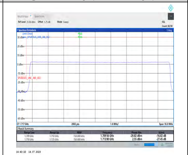
1-N66-PC3-15-15-L-6-CP-QPSK-Outer_Full-79@0-Ant3-1-seegraph-PASS-see graph
