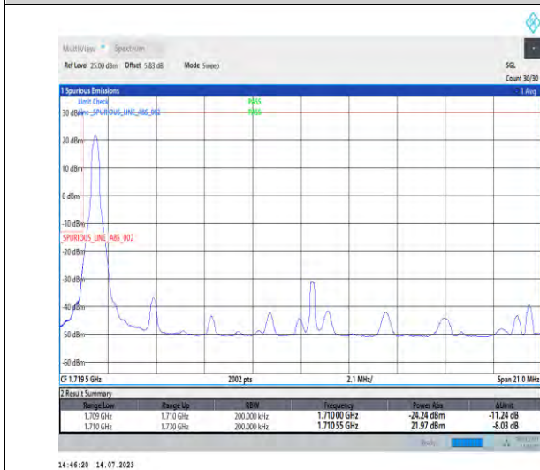
1-N66-PC3-15-20-L-4-CP-QPSK-Edge_1RB_Left-1@0-Ant3-1-seegraph-PASS-see graph
