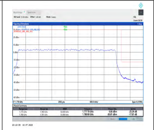
1-N66-PC3-15-5-H-3-DFT-PI2BPSK-Outer_Full-25@0-Ant3-1-seegraph-PASS-see graph
