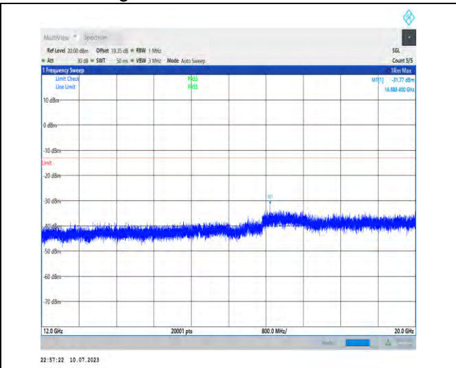
1-N66-PC3-15-40-H-1-DFT-PI2BPSK-Inner_1RB_Lef t-1@1-12000-20000-Ant3-16888.40--31.77--13-PASS
