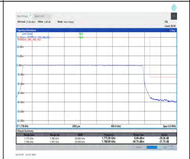
1-N66-PC3-15-5-H-6-CP-QPSK-Outer_Full-25@0-Ant3-1-seegraph-PASS-see graph
