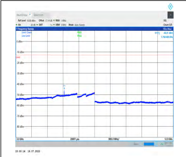
1-N66-PC3-15-40-H-1-DFT-PI2BPSK-Inner_1RB_L eft-1@1-3000-12000-Ant3-5768.4--45.01--13-PASS
