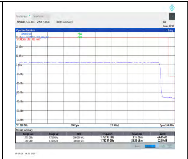
1-N66-PC3-15-25-H-3-DFT-PI2BPSK-Outer_Full-128@0-Ant3-1-seegraph-PASS-see graph
