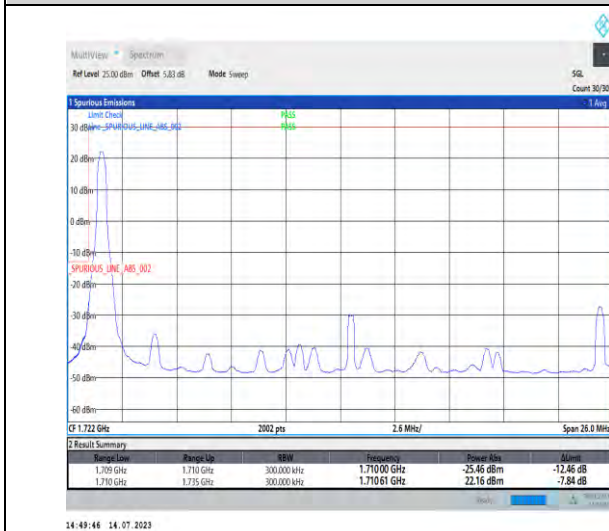
1-N66-PC3-15-25-L-4-CP-QPSK-Edge_1RB_Left-1@0-Ant3-1-seegraph-PASS-see graph
