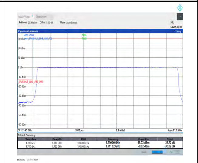
1-N66-PC3-15-10-L-6-CP-QPSK-Outer_Full-52@0-Ant3-1-seegraph-PASS-see graph
