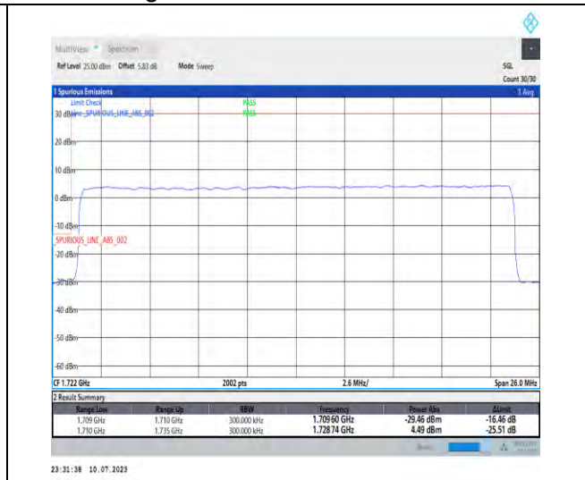
1-N66-PC3-15-25-L-3-DFT-PI2BPSK-Outer_Full-128@0-Ant3-1-seegraph-PASS-see graph
