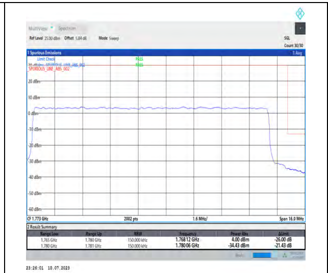
1-N66-PC3-15-15-H-3-DFT-PI2BPSK-Outer_Full-75@0-Ant3-1-seegraph-PASS-see graph
