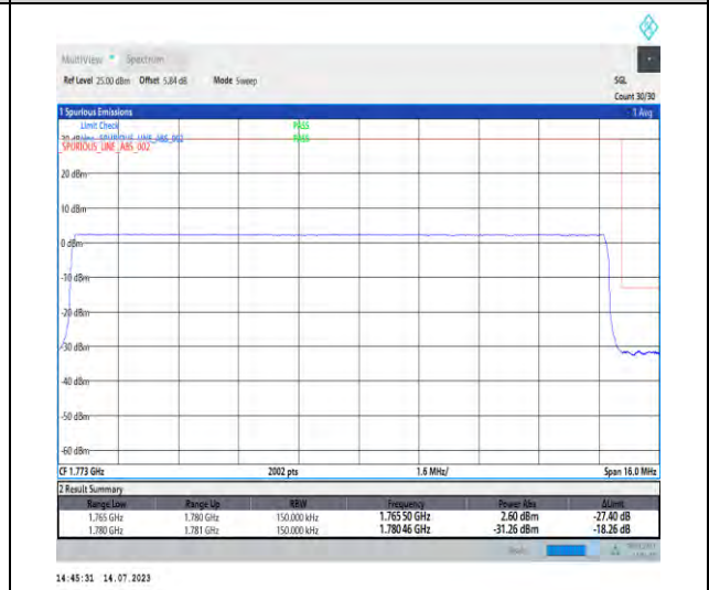
1-N66-PC3-15-15-H-6-CP-QPSK-Outer_Full-79@0-Ant3-1-seegraph-PASS-see graph
