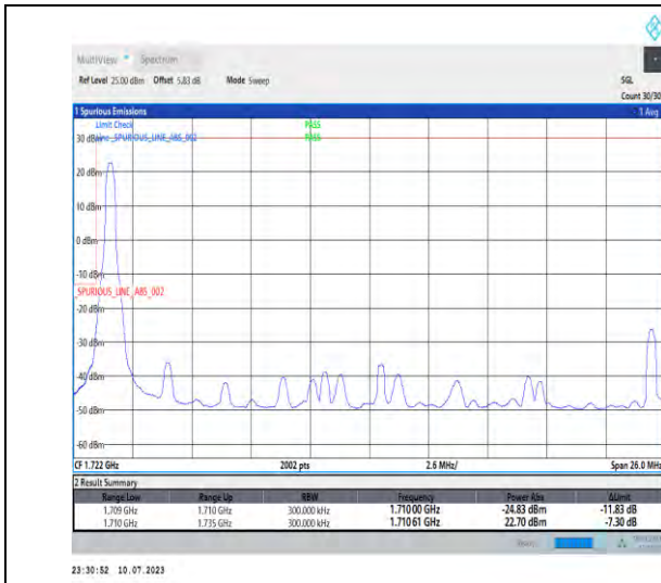
1-N66-PC3-15-25-L-1-DFT-PI2BPSK-Edge_1RB_Left-1@0-Ant3-1-seegraph-PASS-see graph
