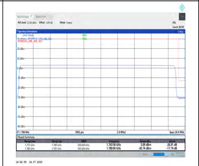
1-N66-PC3-15-25-H-6-CP-QPSK-Outer_Full-133@0-Ant3-1-seegraph-PASS-see graph
