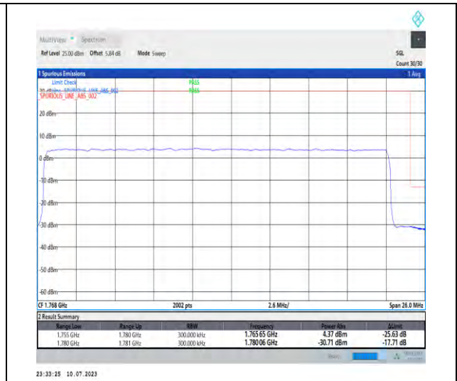
1-N66-PC3-15-25-H-3-DFT-PI2BPSK-Outer_Full-128@0-Ant3-1-seegraph-PASS-see graph
