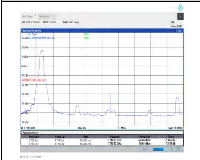
1-N66-PC3-15-10-L-4-CP-QPSK-Edge_1RB_Left-1@0-Ant3-1-seegraph-PASS-see graph
