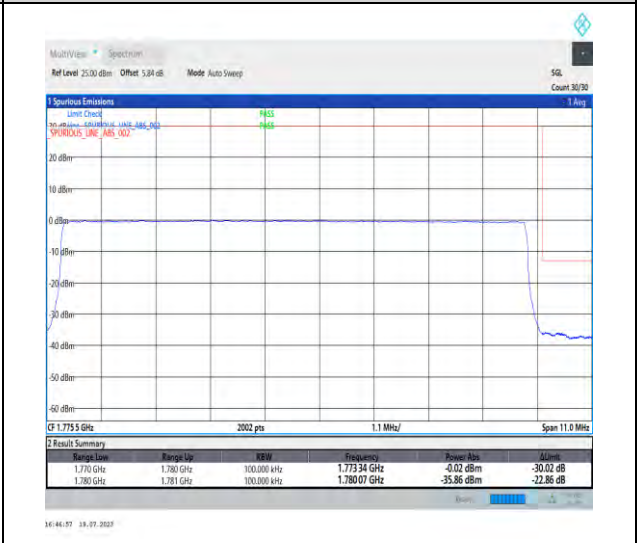
1-N66-PC3-15-10-H-6-CP-QPSK-Outer_Full-52@0-Ant3-1-seegraph-PASS-see graph
