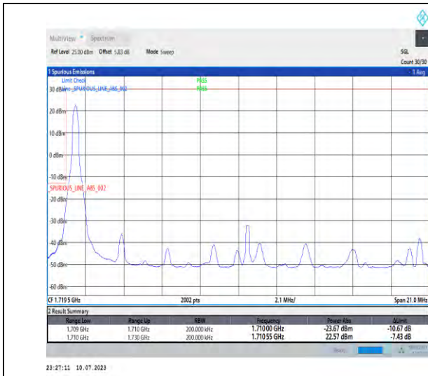
1-N66-PC3-15-20-L-1-DFT-PI2BPSK-Edge_1RB_Left-1@0-Ant3-1-seegraph-PASS-see graph
