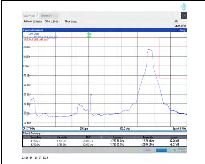
1-N66-PC3-15-5-H-2-DFT-PI2BPSK-Edge_1RB_Right-1@24-Ant3-1-seegraph-PASS-see graph
