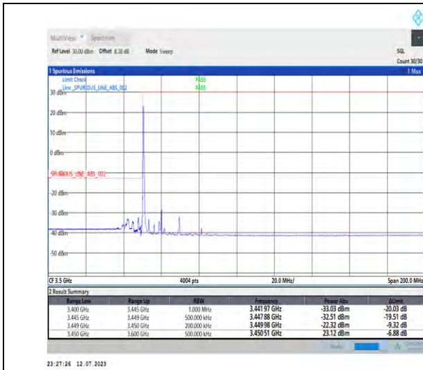
1-N77-3450-3550-PC1.5-30-20-L-1-DFT-PI2BPSK-Edge_1RB_Left-1@0-Ant3-1--PASS-see graph
