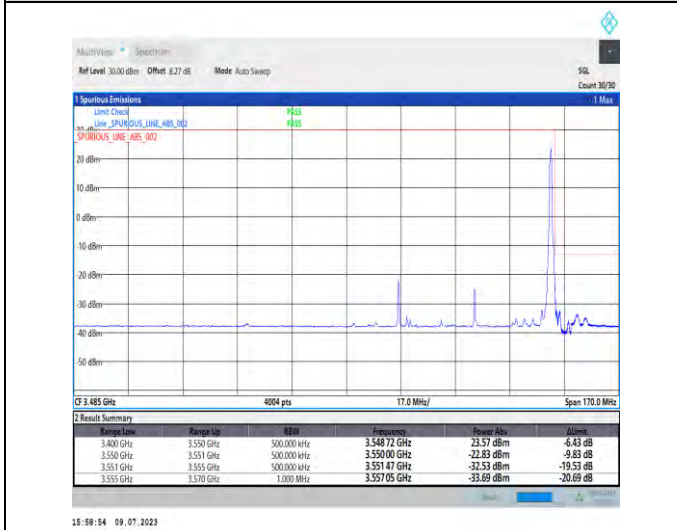
1-N77-3450-3550-PC1.5-30-50-H-5-CP-QPSK-Edge_1RB_Right-1@132-Ant3-1--PASS-see graph
