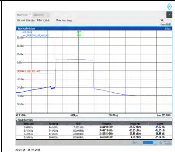
1-N77-3450-3550-PC1.5-30-50-L-6-CP-QPSK-Outer_Full-133@0-Ant3-1--PASS-see graph
