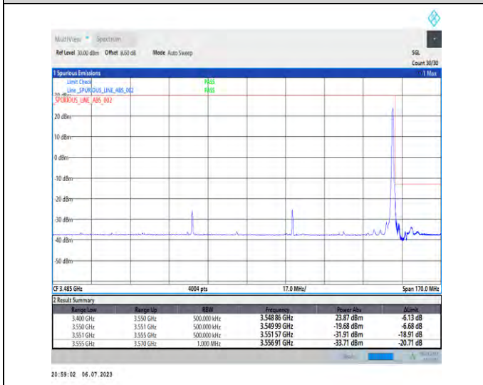
1-N77-3450-3550-PC1.5-30-90-H-5-CP-QPSK-Edge_1RB_Right-1@244-Ant3-1--PASS-see graph
