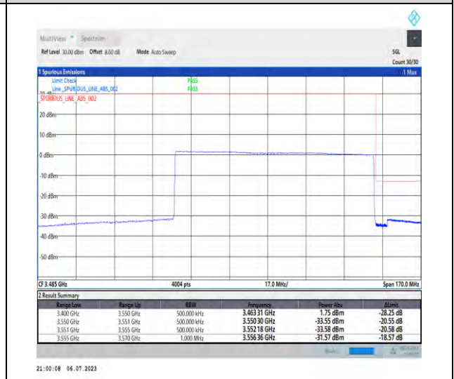
1-N77-3450-3550-PC1.5-30-90-H-6-CP-QPSK-Outer_Full-245@0-Ant3-1--PASS-see graph
