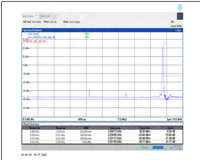
1-N77-3450-3550-PC1.5-30-80-H-2-DFT-PI2BPSK-Edge_1RB_Right-1@216-Ant3-1--PASS-see graph
