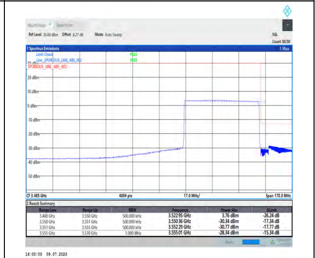
1-N77-3450-3550-PC1.5-30-50-H-6-CP-QPSK-Outer_Full-133@0-Ant3-1--PASS-see graph
