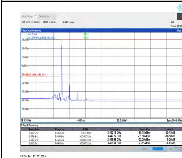
1-N77-3450-3550-PC1.5-30-20-L-4-CP-QPSK-Edge_1RB_Left-1@0-Ant3-1--PASS-see graph
