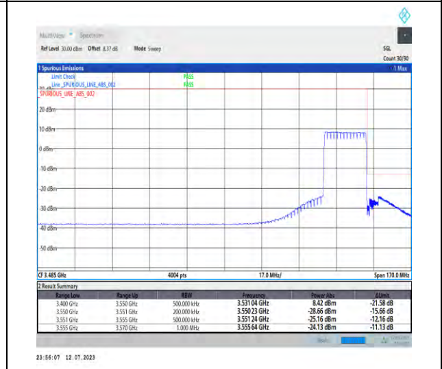
1-N77-3450-3550-PC1.5-30-20-H-6-CP-QPSK-Outer_Full-51@0-Ant3-1--PASS-see graph
