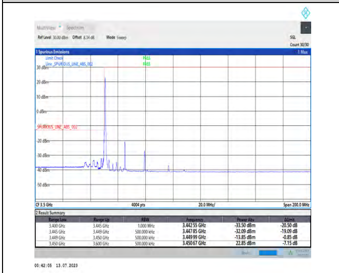
1-N77-3450-3550-PC1.5-30-30-L-4-CP-QPSK-Edge_1RB_Left-1@0-Ant3-1--PASS-see graph
