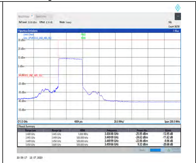
1-N77-3450-3550-PC1.5-30-30-L-3-DFT-PI2BPSK-Outer_Full-75@0-Ant3-1--PASS-see graph
