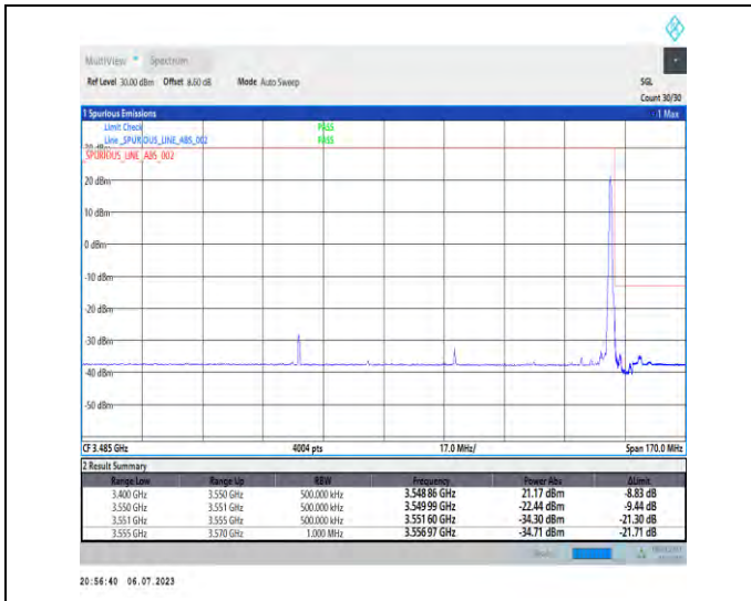
1-N77-3450-3550-PC1.5-30-90-H-2-DFT-PI2BPSK-Edge_1RB_Right-1@244-Ant3-1--PASS-see graph
