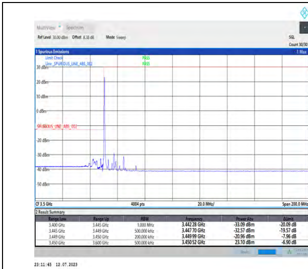
1-N77-3450-3550-PC1.5-30-15-L-1-DFT-PI2BPSK-Edge_1RB_Left-1@0-Ant3-1--PASS-see graph
