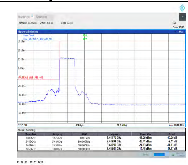
1-N77-3450-3550-PC1.5-30-20-L-3-DFT-PI2BPSK-Outer_Full-50@0-Ant3-1--PASS-see graph
