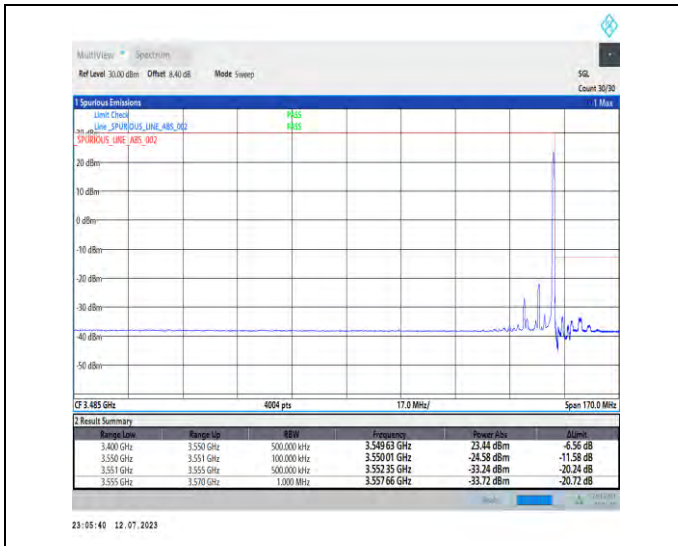
1-N77-3450-3550-PC1.5-30-10-H-2-DFT-PI2BPSK-Edge_1RB_Right-1@23-Ant3-1--PASS-see graph
