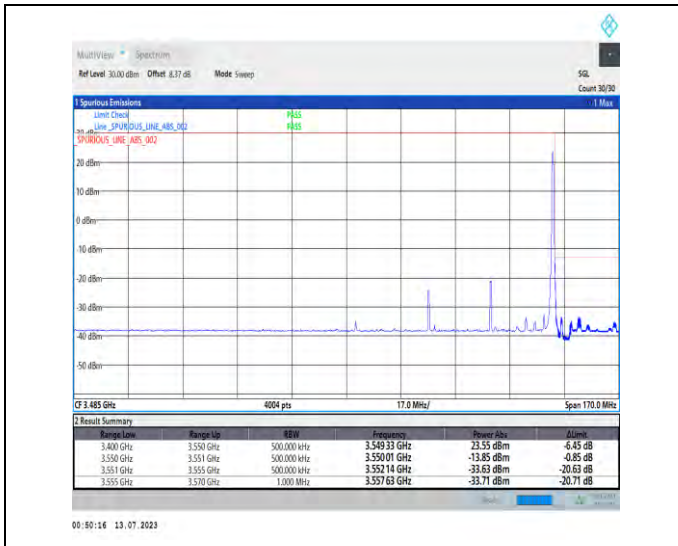
1-N77-3450-3550-PC1.5-30-40-H-2-DFT-PI2BPSK-Edge_1RB_Right-1@105-Ant3-1--PASS-see graph
