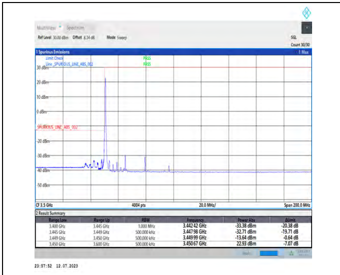
1-N77-3450-3550-PC1.5-30-30-L-1-DFT-PI2BPSK-Edge_1RB_Left-1@0-Ant3-1--PASS-see graph
