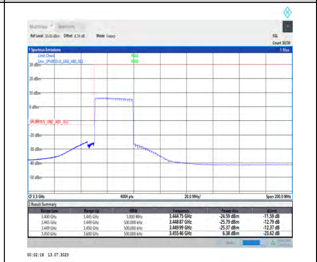
1-N77-3450-3550-PC1.5-30-30-L-6-CP-QPSK-Outer_Full-75@0-Ant3-1--PASS-see graph
