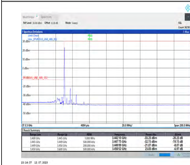
1-N77-3450-3550-PC1.5-30-15-L-4-CP-QPSK-Edge_1RB_Left-1@0-Ant3-1--PASS-see graph
