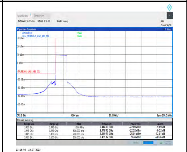
1-N77-3450-3550-PC1.5-30-15-L-6-CP-QPSK-Outer_Full-38@0-Ant3-1--PASS-see graph
