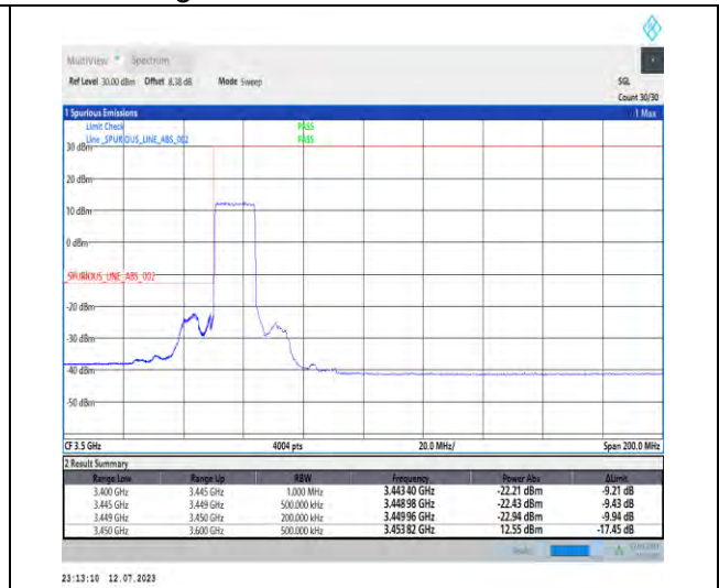
1-N77-3450-3550-PC1.5-30-15-L-3-DFT-PI2BPSK-Outer_Full-36@0-Ant3-1--PASS-see graph
