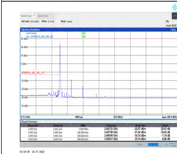
1-N77-3450-3550-PC1.5-30-30-L-4-CP-QPSK-Edge_1RB_Left-1@0-Ant3-1--PASS-see graph
