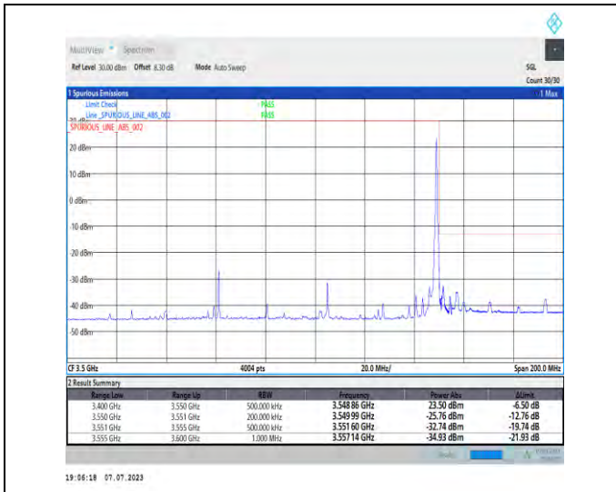
1-N77-3450-3550-PC1.5-30-90-H-2-DFT-PI2BPSK-Edge_1RB_Right-1@244-Ant3-1--PASS-see graph
