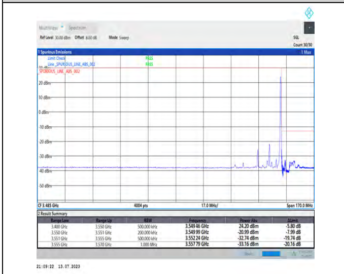
1-N77-3450-3550-PC1.5-30-15-H-5-CP-QPSK-Edge_1RB_Right-1@37-Ant3-1--PASS-see graph
