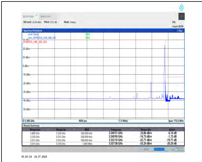
1-N77-3450-3550-PC1.5-30-30-H-2-DFT-PI2BPSK-Edge_1RB_Right-1@77-Ant3-1--PASS-see graph
