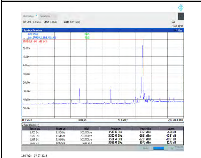
1-N77-3450-3550-PC1.5-30-80-H-5-CP-QPSK-Edge_1RB_Right-1@216-Ant3-1--PASS-see graph
