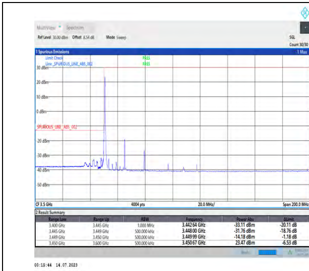
1-N77-3450-3550-PC1.5-30-30-L-1-DFT-PI2BPSK-Edge_1RB_Left-1@0-Ant3-1--PASS-see graph
