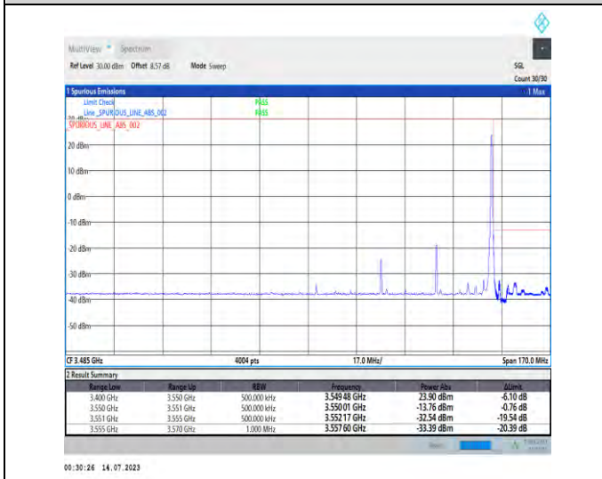
1-N77-3450-3550-PC1.5-30-40-H-5-CP-QPSK-Edge_1RB_Right-1@105-Ant3-1--PASS-see graph
