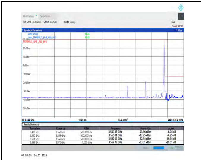
1-N77-3450-3550-PC1.5-30-40-H-2-DFT-PI2BPSK-Edge_1RB_Right-1@105-Ant3-1--PASS-see graph
