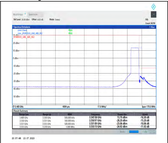
1-N77-3450-3550-PC1.5-30-10-H-3-DFT-PI2BPSK-Outer_Full-24@0-Ant3-1--PASS-see graph
