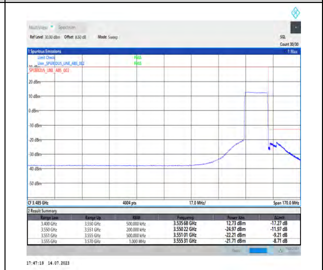
1-N77-3450-3550-PC1.5-30-15-H-6-CP-QPSK-Outer_Full-38@0-Ant3-1--PASS-see graph
