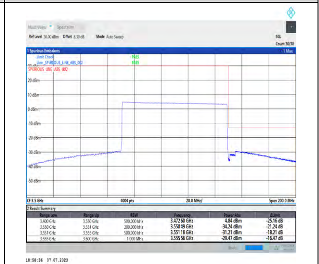
1-N77-3450-3550-PC1.5-30-80-H-6-CP-QPSK-Outer_Full-217@0-Ant3-1--PASS-see graph
