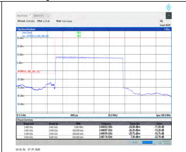
1-N77-3450-3550-PC1.5-30-90-L-3-DFT-PI2BPSK-Outer_Full-240@0-Ant3-1--PASS-see graph
