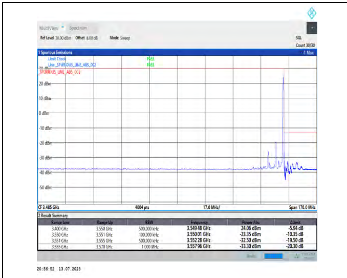
1-N77-3450-3550-PC1.5-30-10-H-2-DFT-PI2BPSK-Edge_1RB_Right-1@23-Ant3-1--PASS-see graph
