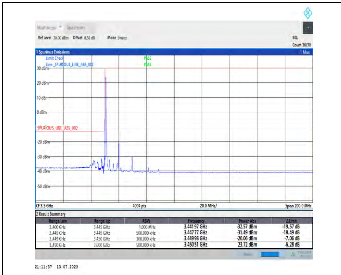
1-N77-3450-3550-PC1.5-30-20-L-1-DFT-PI2BPSK-Edge_1RB_Left-1@0-Ant3-1--PASS-see graph
