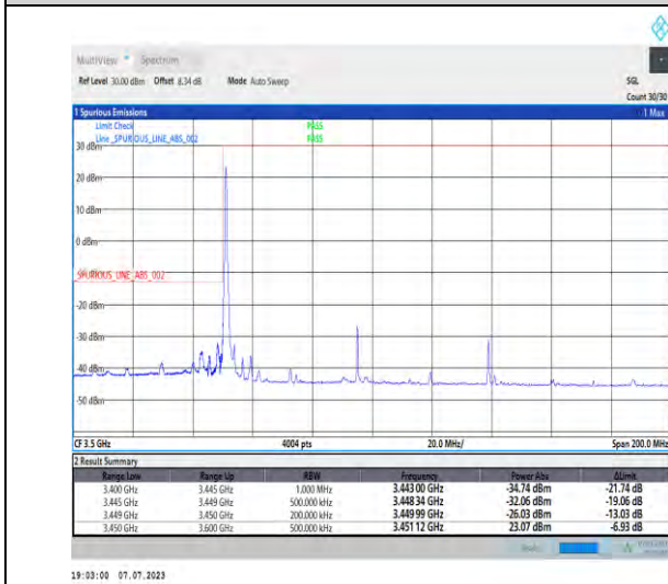
1-N77-3450-3550-PC1.5-30-90-L-4-CP-QPSK-Edge_1RB_Left-1@0-Ant3-1--PASS-see graph
