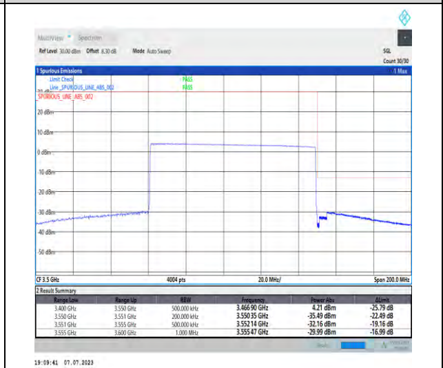
1-N77-3450-3550-PC1.5-30-90-H-6-CP-QPSK-Outer_Full-245@0-Ant3-1--PASS-see graph
