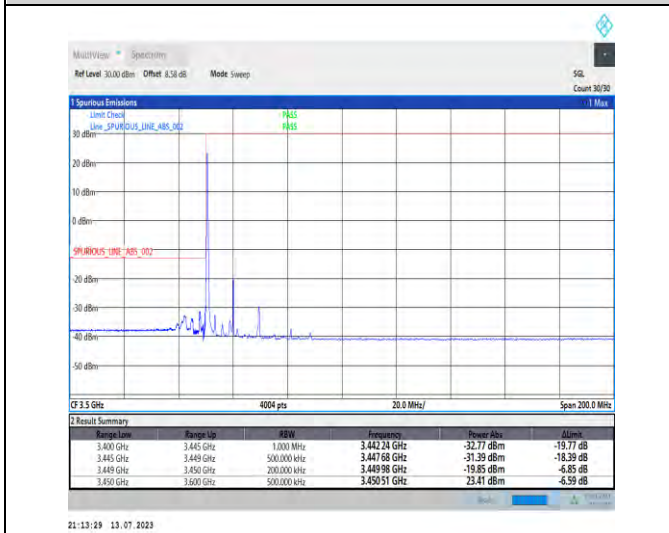
1-N77-3450-3550-PC1.5-30-20-L-4-CP-QPSK-Edge_1RB_Left-1@0-Ant3-1--PASS-see graph
