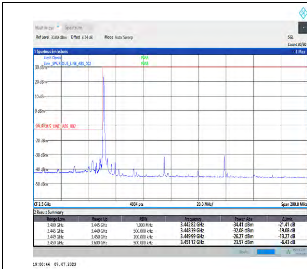
1-N77-3450-3550-PC1.5-30-90-L-1-DFT-PI2BPSK-Edge_1RB_Left-1@0-Ant3-1--PASS-see graph
