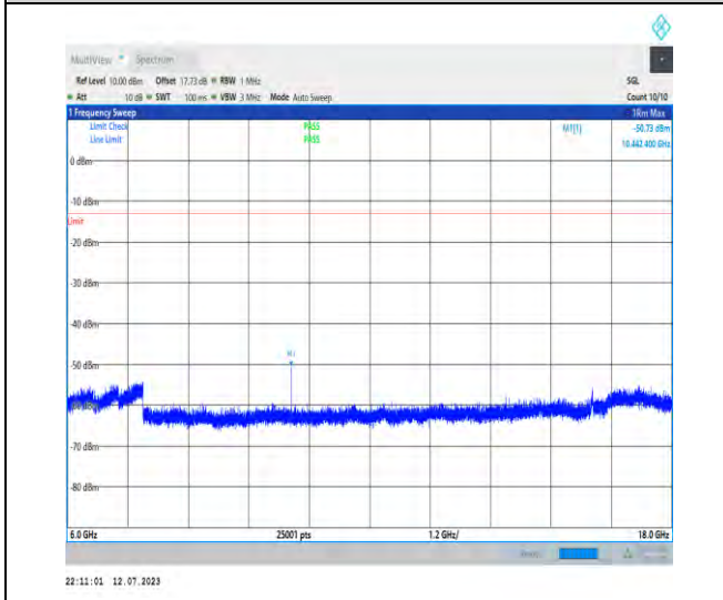
1-N77-3450-3550-PC1.5-30-100-M-1-DFT-PI2BPSK -Inner_1RB_Left-1@1-6000-18000-Ant3-10442.40-- 50.73--13-PASS
