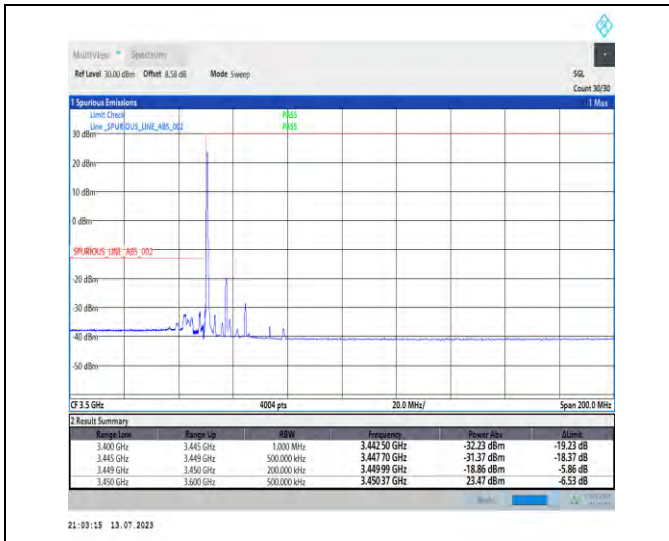
1-N77-3450-3550-PC1.5-30-15-L-1-DFT-PI2BPSK-Edge_1RB_Left-1@0-Ant3-1-PASS-see graph
