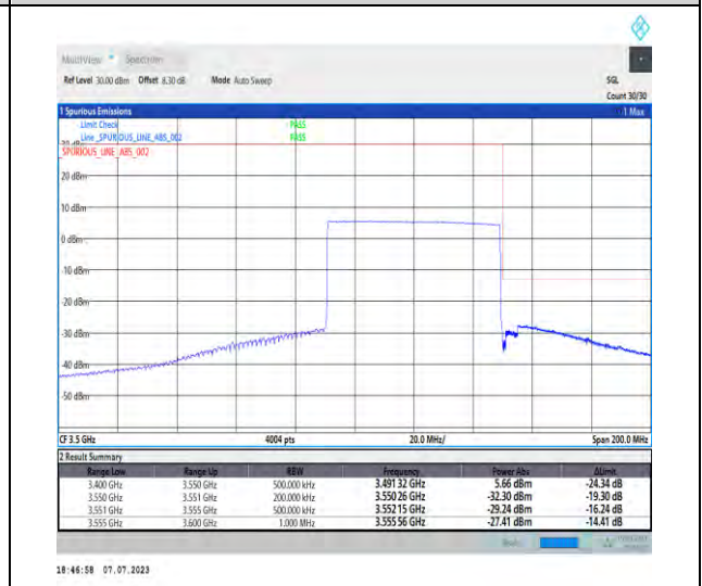
1-N77-3450-3550-PC1.5-30-60-H-6-CP-QPSK-Outer_Full-162@0-Ant3-1--PASS-see graph
