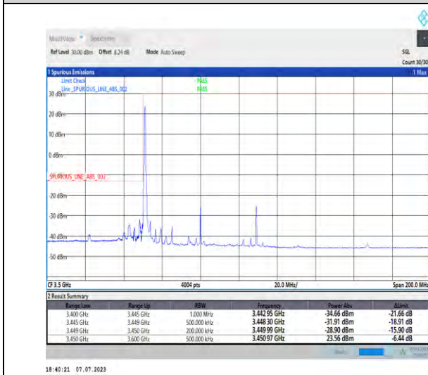
1-N77-3450-3550-PC1.5-30-60-L-4-CP-QPSK-Edge_1RB_Left-1@0-Ant3-1--PASS-see graph
