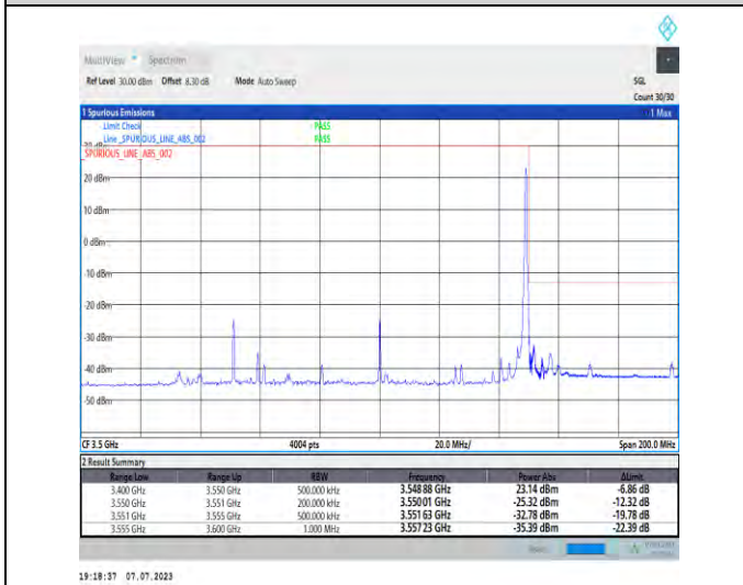
1-N77-3450-3550-PC1.5-30-100-H-5-CP-QPSK-Edge_ 1RB_Right-1@272-Ant3-1--PASS-see graph
