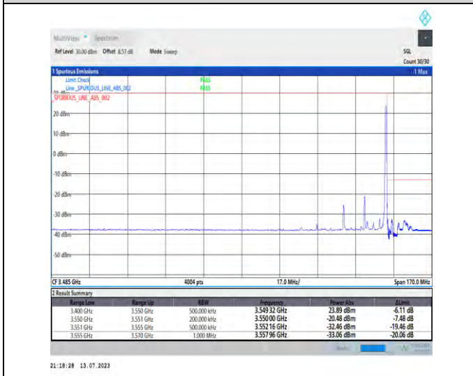
1-N77-3450-3550-PC1.5-30-20-H-5-CP-QPSK-Edge_1RB_Right-1@50-Ant3-1--PASS-see graph
