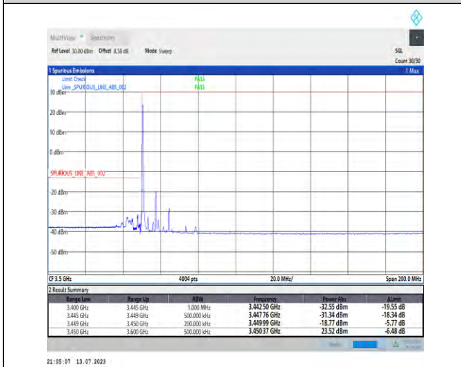
1-N77-3450-3550-PC1.5-30-15-L-4-CP-QPSK-Edge_1RB_Left-1@0-Ant3-1-PASS-see graph
