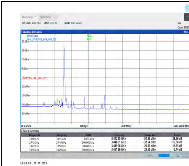
1-N77-3450-3550-PC1.5-30-50-L-1-DFT-PI2BPSK-Edge_1RB_Left-1@0-Ant3-1--PASS-see graph
