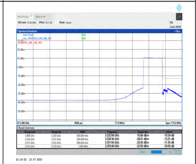
1-N77-3450-3550-PC1.5-30-20-H-6-CP-QPSK-Outer_Full-51@0-Ant3-1--PASS-see graph
