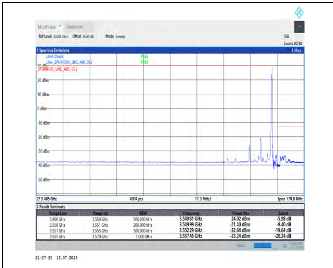
1-N77-3450-3550-PC1.5-30-15-H-2-DFT-PI2BPSK-Edge_1RB_Right-1@37-Ant3-1--PASS-see graph
