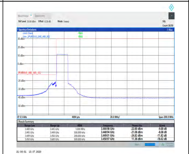
1-N77-3450-3550-PC1.5-30-15-L-6-CP-QPSK-Outer_Full-38@0-Ant3-1-PASS-see graph
