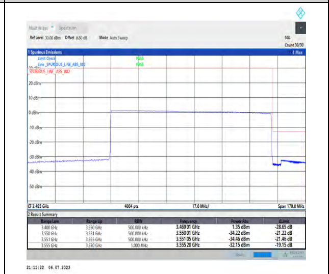
1-N77-3450-3550-PC1.5-30-100-H-6-CP-QPSK-O uter_Full-273@0-Ant3-1--PASS-see graph
