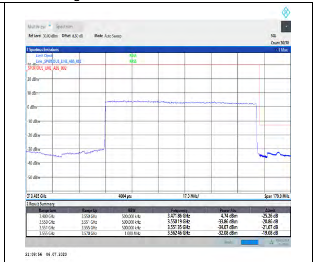
1-N77-3450-3550-PC1.5-30-100-H-3-DFT-PI2BPS K-Outer_Full-270@0-Ant3-1--PASS-see graph
