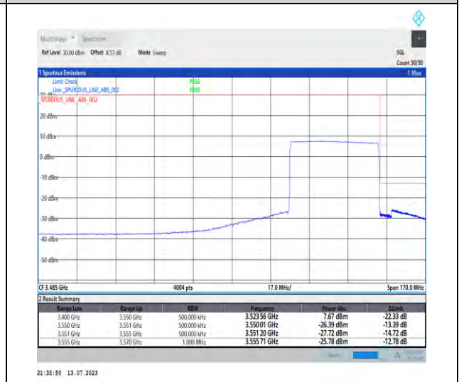
1-N77-3450-3550-PC1.5-30-40-H-6-CP-QPSK-Outer_Full-100@0-Ant3-1--PASS-see graph
