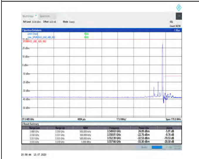
1-N77-3450-3550-PC1.5-30-10-H-5-CP-QPSK-Edge_1RB_Right-1@23-Ant3-1--PASS-see graph
