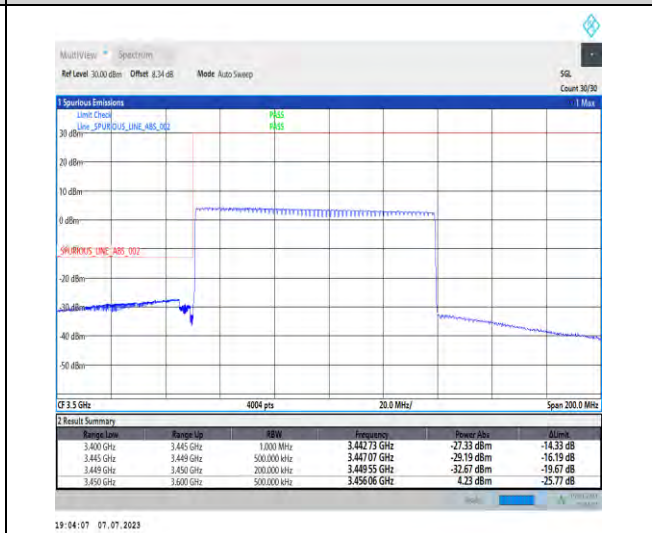
1-N77-3450-3550-PC1.5-30-90-L-6-CP-QPSK-Outer_Full-245@0-Ant3-1--PASS-see graph
