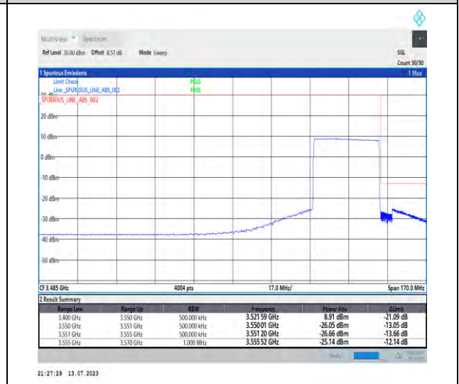
1-N77-3450-3550-PC1.5-30-30-H-6-CP-QPSK-Outer_Full-75@0-Ant3-1--PASS-see graph
