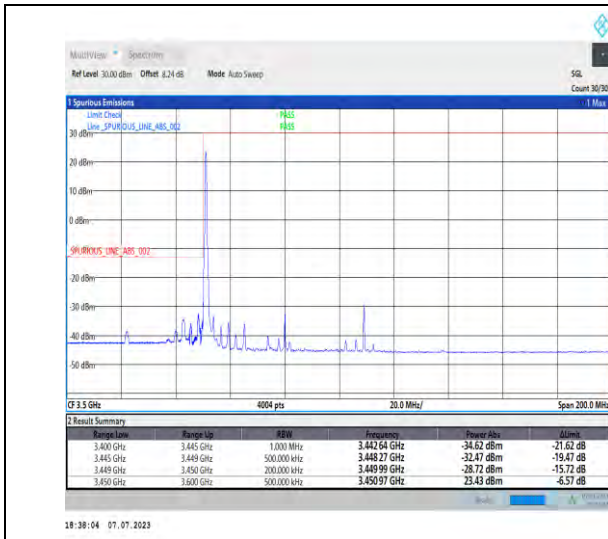
1-N77-3450-3550-PC1.5-30-60-L-1-DFT-PI2BPSK-Edge_1RB_Left-1@0-Ant3-1--PASS-see graph
