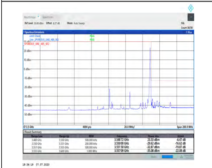
1-N77-3450-3550-PC1.5-30-50-H-5-CP-QPSK-Edge_1RB_Right-1@132-Ant3-1--PASS-see graph
