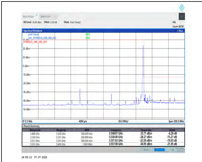
1-N77-3450-3550-PC1.5-30-80-H-2-DFT-PI2BPSK-Edge_1RB_Right-1@216-Ant3-1--PASS-see graph
