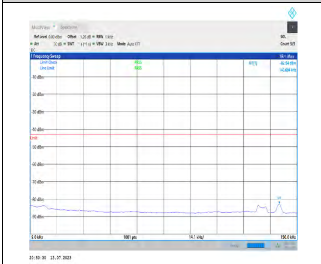
1-N77-3450-3550-PC1.5-30-100-H-1-DFT-QPSK-Edge_1RB_Left-1@0-0.009-0.30-Ant3-0.14--82.84--43-PASS
