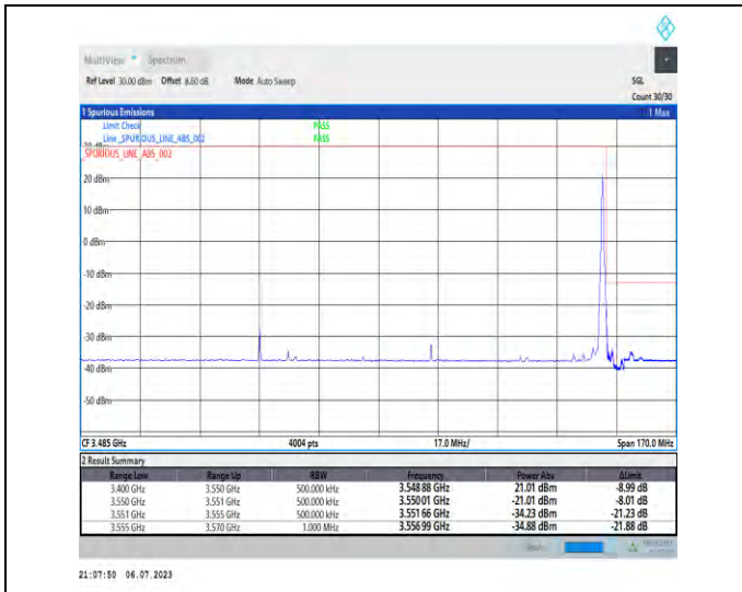
1-N77-3450-3550-PC1.5-30-100-H-2-DFT-PI2BPSK-E dge_1RB_Right-1@272-Ant3-1--PASS-see graph
