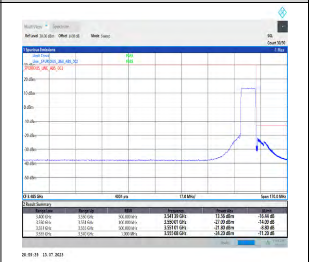
1-N77-3450-3550-PC1.5-30-10-H-6-CP-QPSK-Outer_Full-24@0-Ant3-1--PASS-see graph
