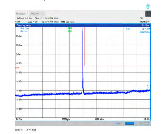
1-N77-3450-3550-PC1.5-30-100-M-1-DFT-PI2BPSK -Inner_1RB_Left-1@1-1000-6000-Ant3-5918.50--38.1 4--13-PASS
