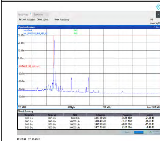
1-N77-3450-3550-PC1.5-30-50-L-4-CP-QPSK-Edge_1RB_Left-1@0-Ant3-1--PASS-see graph
