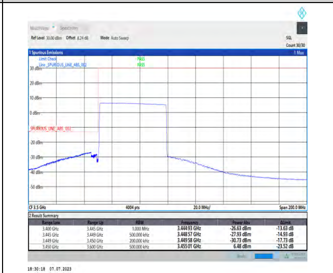
1-N77-3450-3550-PC1.5-30-50-L-6-CP-QPSK-Outer_Full-133@0-Ant3-1--PASS-see graph
