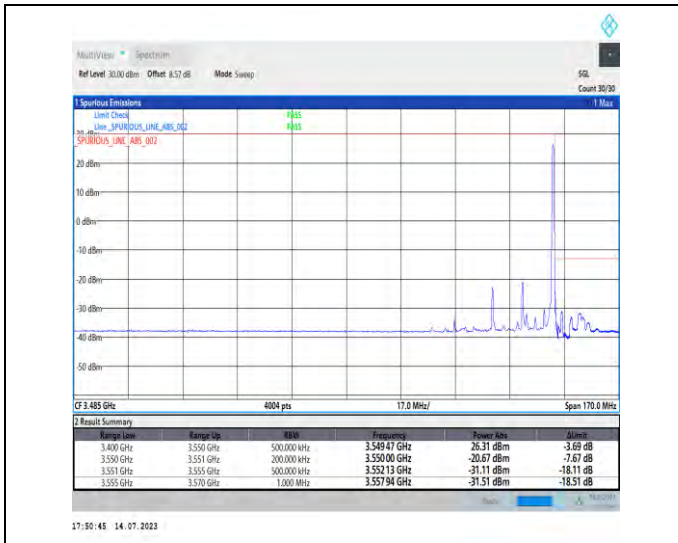
1-N77-3450-3550-PC1.5-30-20-H-2-DFT-PI2BPSK-Edge_1RB_Right-1@50-Ant3-1--PASS-see graph
