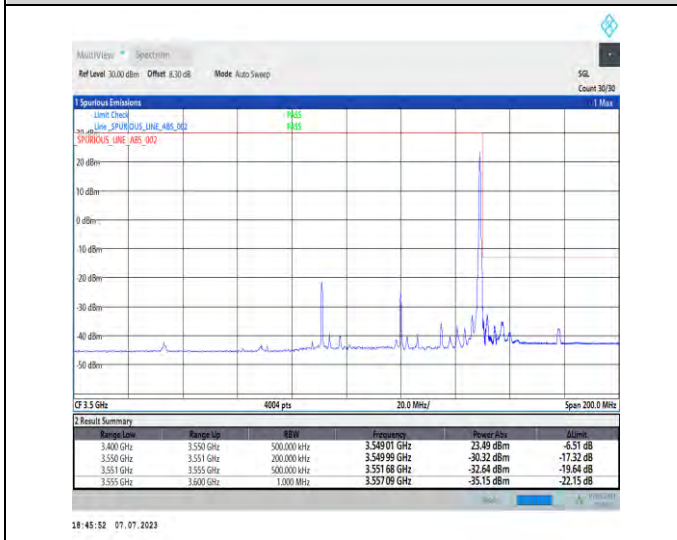
1-N77-3450-3550-PC1.5-30-60-H-5-CP-QPSK-Edge_1RB_Right-1@161-Ant3-1--PASS-see graph
