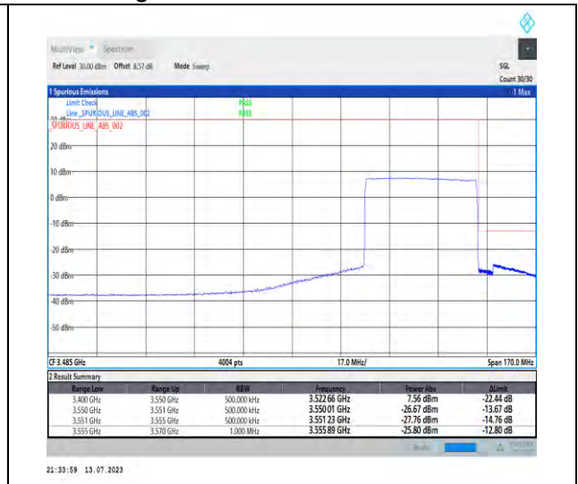
1-N77-3450-3550-PC1.5-30-40-H-3-DFT-PI2BPSK-Outer_Full-100@0-Ant3-1--PASS-see graph
