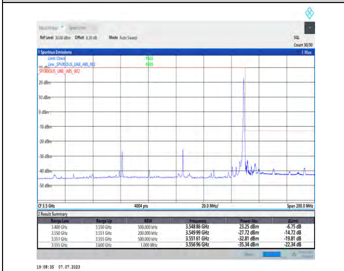
1-N77-3450-3550-PC1.5-30-90-H-5-CP-QPSK-Edge_1RB_Right-1@244-Ant3-1--PASS-see graph
