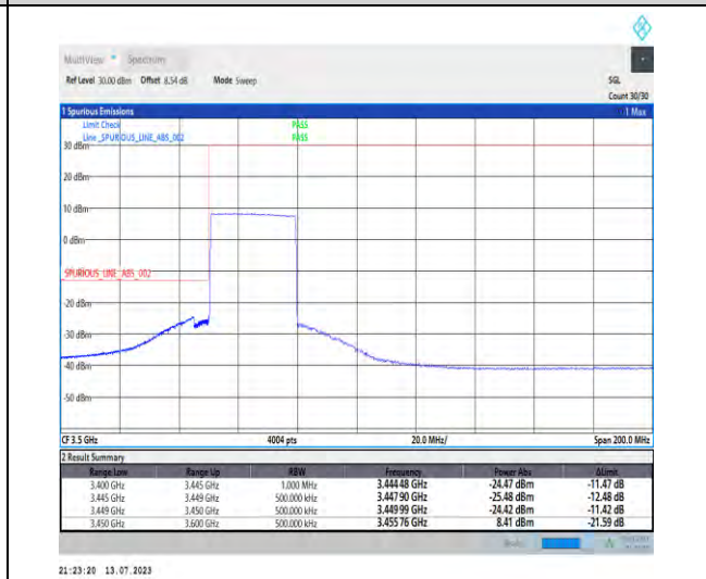
1-N77-3450-3550-PC1.5-30-30-L-6-CP-QPSK-Outer_Full-75@0-Ant3-1--PASS-see graph
