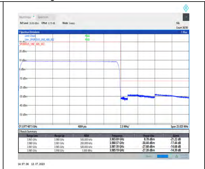
1-N77-3700-3980-PC1.5-30-15-H-6-CP-QPSK-Out_er_Full-38@0-Ant3-1--PASS-see graph
