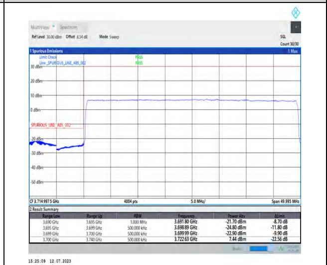
1-N77-3700-3980-PC1.5-30-40-L-3-DFT-PI2BPSK-Outer_Full-100@0-Ant3-1--PASS-see graph
