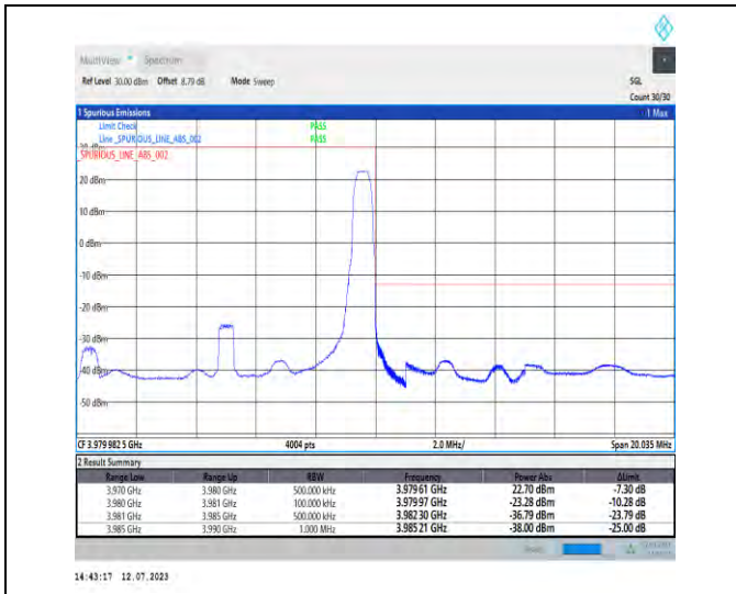
1-N77-3700-3980-PC1.5-30-10-H-5-CP-QPSK-Edge_1RB_Right-1@23-Ant3-1--PASS-see graph
