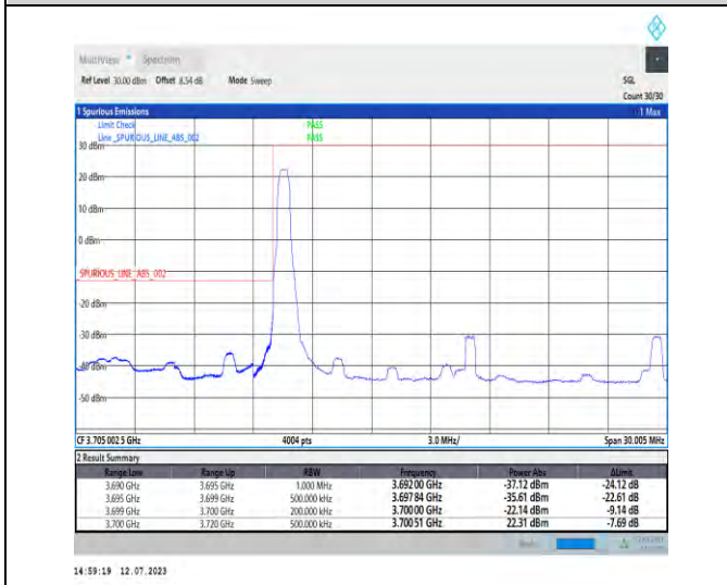
1-N77-3700-3980-PC1.5-30-20-L-1-DFT-PI2BPSK-Edge_1RB_Left-1@0-Ant3-1--PASS-see graph
