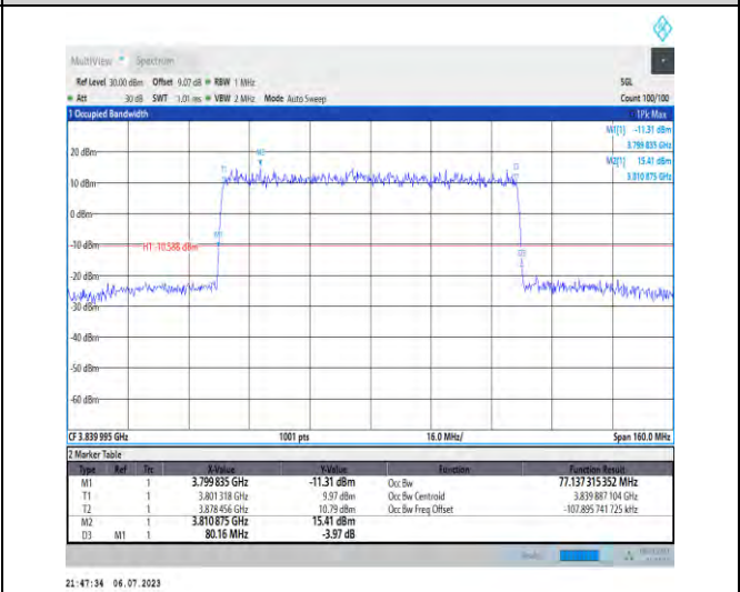
1-N77-3700-3980-PC1.5-30-80-M-4-DFT-64QAM-O uter_Full-100@0-Ant3-77.137-80.160-≤80-PASS
