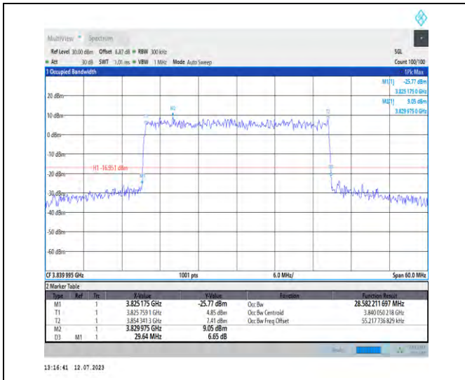
1-N77-3700-3980-PC1.5-30-30-M-9-CP-256QAM-Ou ter_Full-75@0-Ant3-28.582-29.640-<30-PASS
