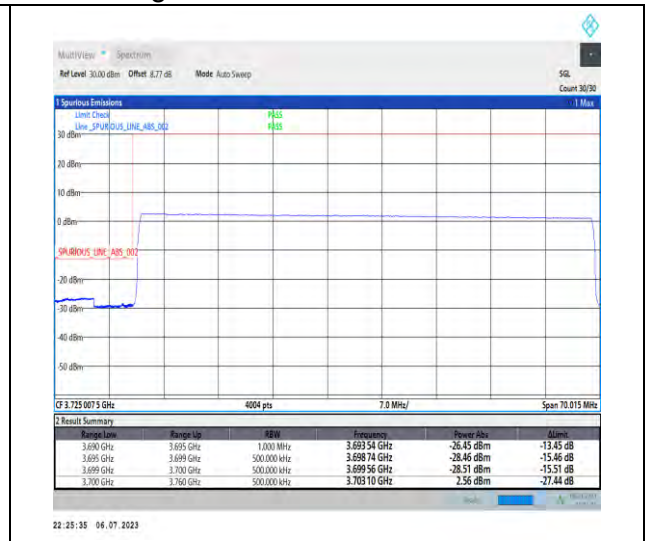
1-N77-3700-3980-PC1-30-60-L-6-CP-QPSK-Outer _Full-162@0-Ant3-1--PASS-see graph
