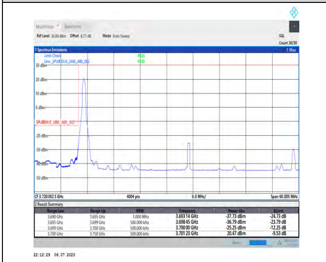
1-N77-3700-3980-PC1-30-50-L-1-DFT-PI2BPSK-Edge_1RB_Left-1@0-Ant3-1--PASS-see graph
