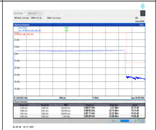
1-N77-3700-3980-PC1-30-60-H-3-DFT-PI2BPSK- Outer_Full-162@0-Ant3-1--PASS-see graph
