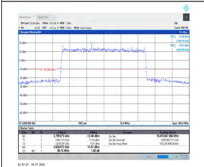
1-N77-3700-3980-PC1.5-30-80-M-3-DFT-16QAM-O uter_Full-100@0-Ant3-76.976-80.160-≤80-PASS
