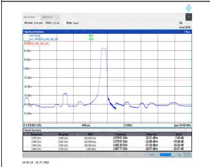
1-N77-3700-3980-PC1.5-30-10-H-2-DFT-PI2BPSK-Ed ge_1RB_Right-1@23-Ant3-1--PASS-see graph
