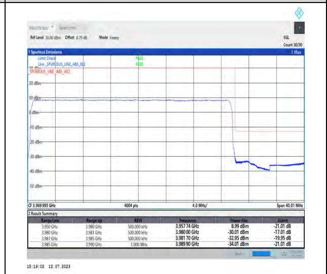
1-N77-3700-3980-PC1.5-30-30-H-3-DFT-PI2BPSK -Outer_Full-75@0-Ant3-1--PASS-see graph
