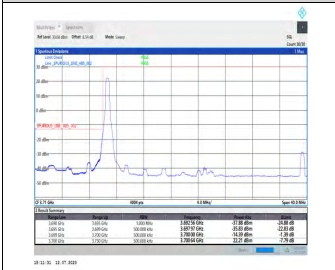
1-N77-3700-3980-PC1.5-30-30-L-1-DFT-PI2BPSK-Edge_1RB_Left-1@0-Ant3-1--PASS-see graph
