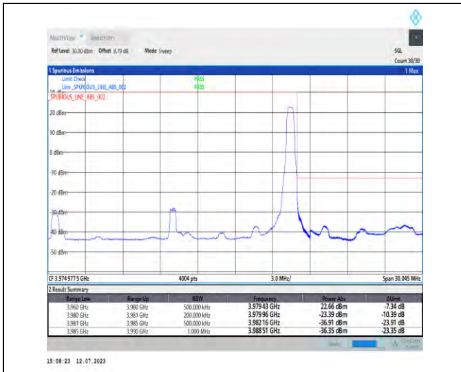
1-N77-3700-3980-PC1.5-30-20-H-5-CP-QPSK-Edge_1RB_Right-1@50-Ant3-1--PASS-see graph
