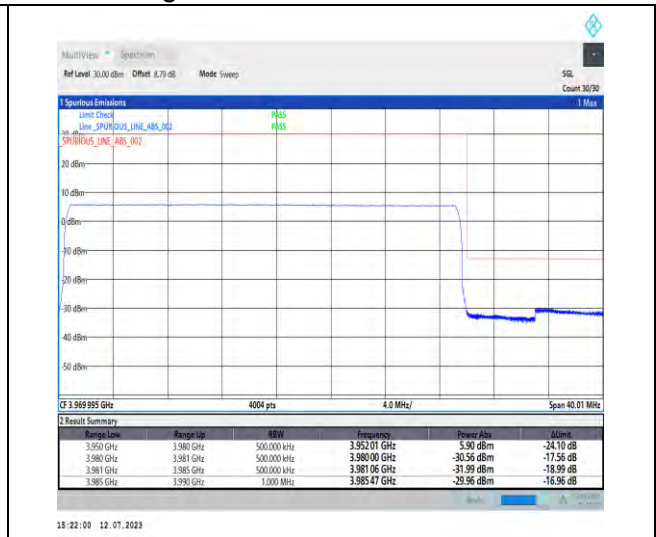
1-N77-3700-3980-PC1.5-30-30-H-6-CP-QPSK-Outer_Full-75@0-Ant3-1--PASS-see graph
