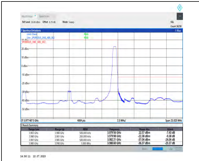
1-N77-3700-3980-PC1.5-30-15-H-5-CP-QPSK-Edge_1RB_Right-1@37-Ant3-1--PASS-see graph
