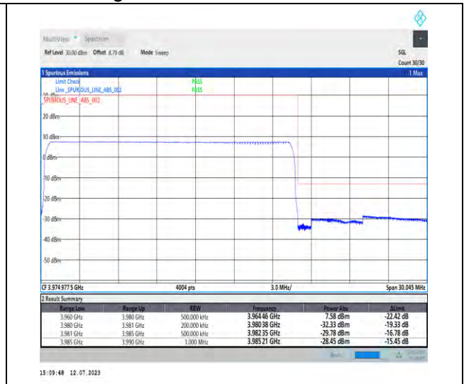
1-N77-3700-3980-PC1.5-30-20-H-6-CP-QPSK-Out_er_Full-51@0-Ant3-1--PASS-see graph
