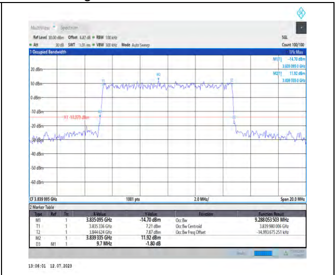
1-N77-3700-3980-PC1.5-30-10-M-6-CP-QPSK-Outer_Full-24@0-Ant3-9.288-9.700-≤10-PASS
