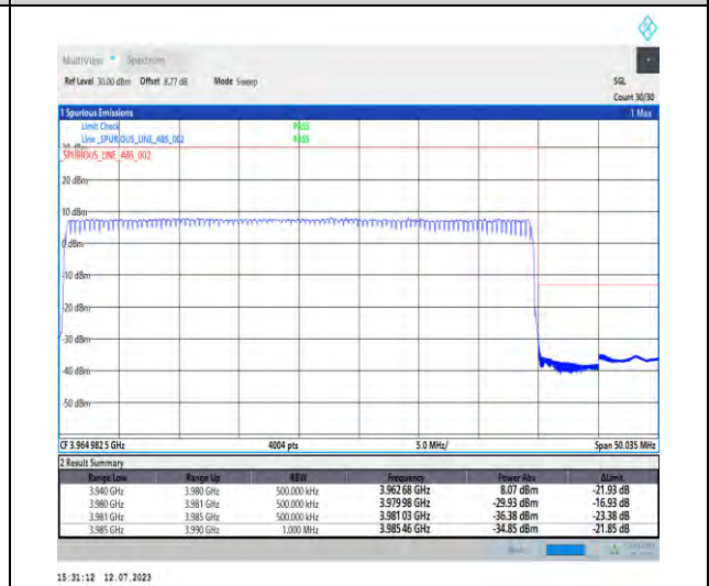
1-N77-3700-3980-PC1.5-30-40-H-3-DFT-PI2BPSK -Outer_Full-100@0-Ant3-1--PASS-see graph
