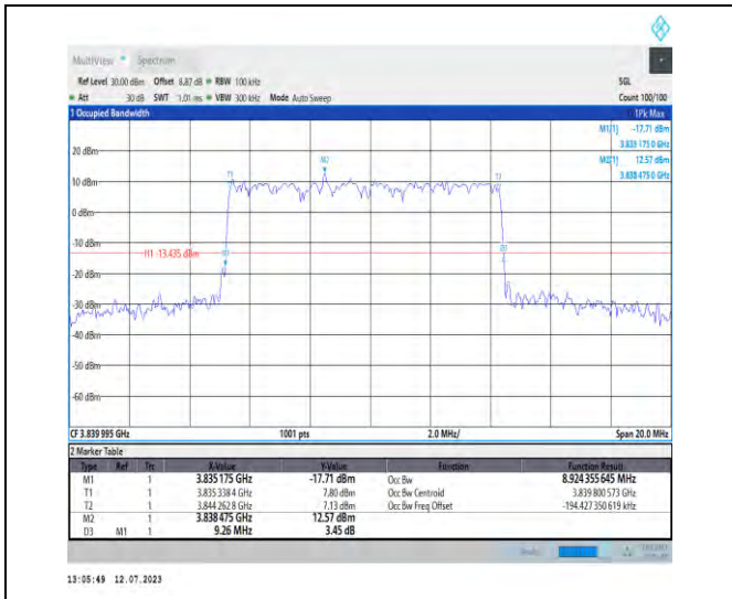
1-N77-3700-3980-PC1.5-30-10-M-5-DFT-256QAM-Outer_Full-24@0-Ant3-8.924-9.260-≤10-PASS
