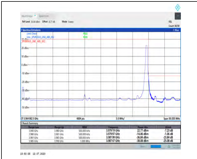
1-N77-3700-3980-PC1.5-30-40-H-5-CP-QPSK-Edge_1RB_Right-1@105-Ant3-1--PASS-see graph
