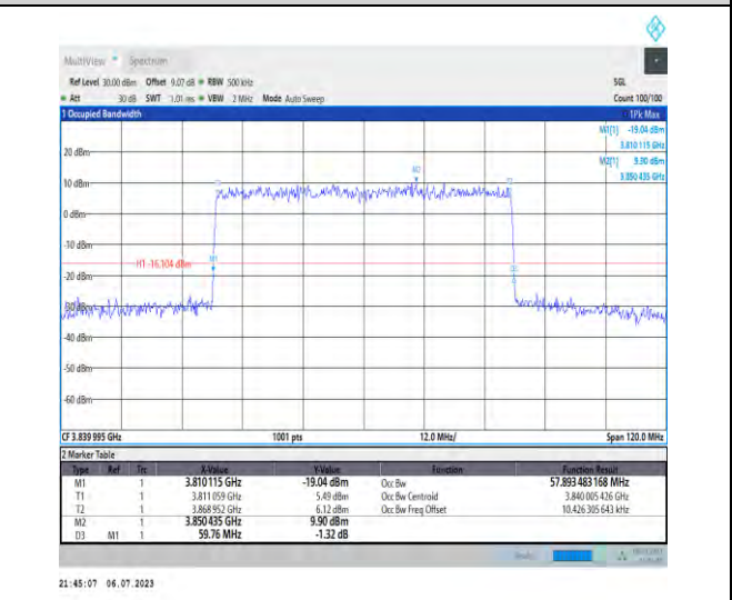
1-N77-3700-3980-PC1.5-30-60-M-5-DFT-256QAM-Outer_Full-162@0-Ant3-57.893-59.760-≤60-PASS
