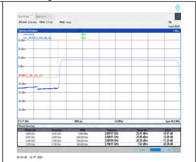
1-N77-3700-3980-PC1.5-30-30-L-3-DFT-PI2BPSK-Outer_Full-75@0-Ant3-1--PASS-see graph
