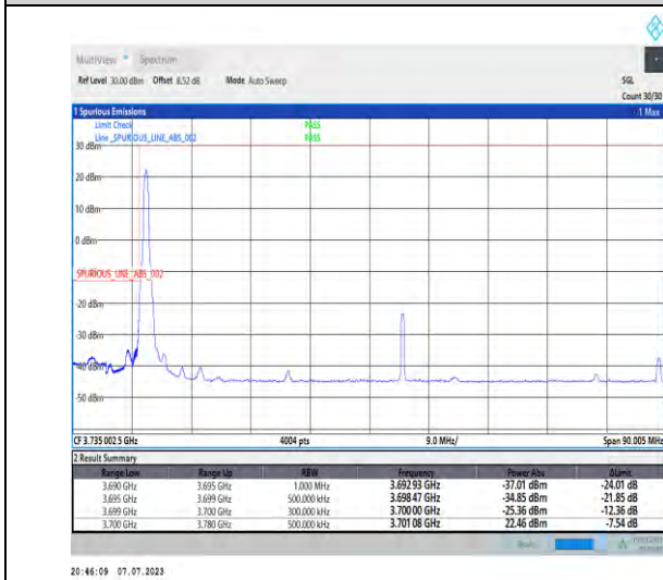
1-N77-3700-3980-PC1.5-30-80-L-4-CP-QPSK-Edge_1RB_Left-1@0-Ant3-1--PASS-see graph
