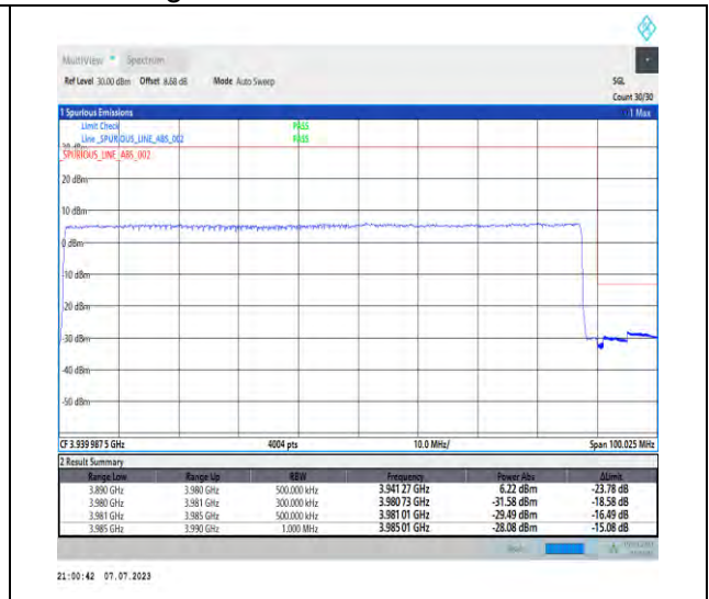
1-N77-3700-3980-PC1.5-30-90-H-3-DFT-PI2BPSK-Outer_Full-240@0-Ant3-1--PASS-see graph
