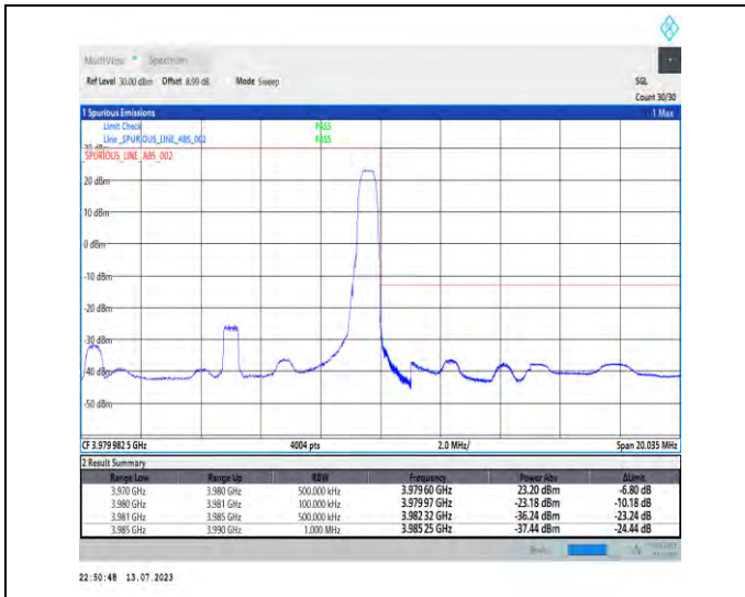
1-N77-3700-3980-PC1.5-30-10-H-2-DFT-PI2BPSK-Edge_1RB_Right-1@23-Ant3-1--PASS-see graph
