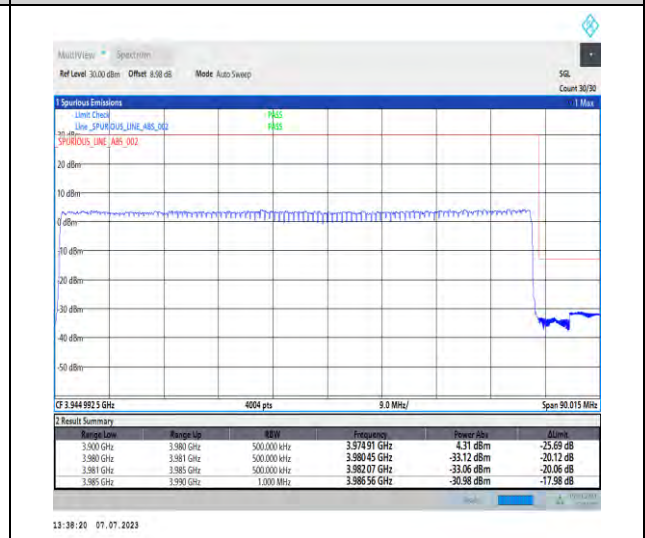
1-N77-3700-3980-PC1-30-80-H-3-DFT-PI2BPSK-Outer_Full-100@0-Ant3-1--PASS-see graph
