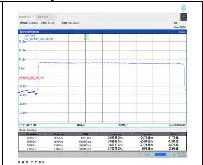
1-N77-3700-3980-PC1.5-30-80-L-3-DFT-PI2BPSK-Outer_Full-100@0-Ant3-1--PASS-see graph
