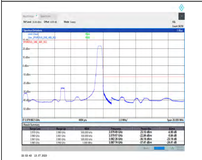
1-N77-3700-3980-PC1.5-30-10-H-5-CP-QPSK-Edge_1RB_Right-1@23-Ant3-1--PASS-see graph
