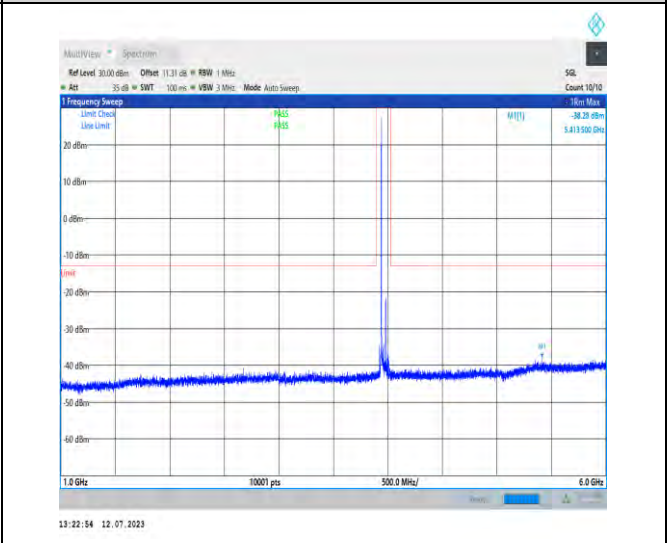
1-N77-3700-3980-PC1.5-30-100-H-1-DFT-PI2BPSK- Inner_1RB_Left-1@1-1000-6000-Ant3-5413.50--38.2 8--13-PASS
