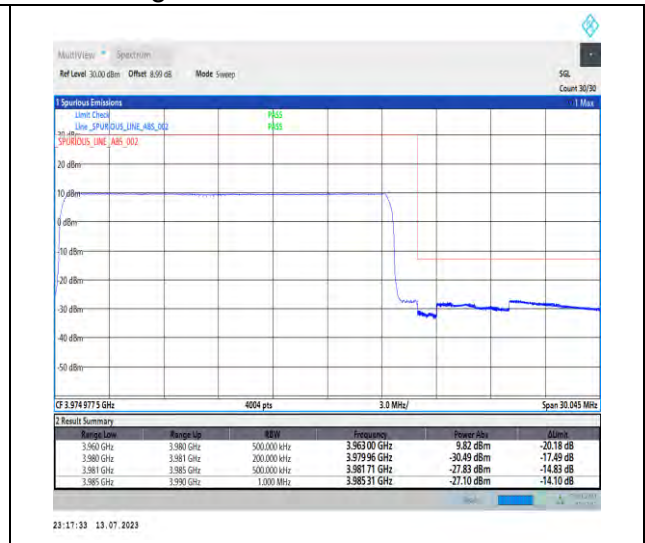
1-N77-3700-3980-PC1.5-30-20-H-3-DFT-PI2BPSK-Outer_Full-50@0-Ant3-1--PASS-see graph
