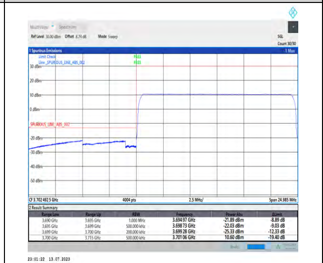
1-N77-3700-3980-PC1.5-30-15-L-6-CP-QPSK-Outer_Full-38@0-Ant3-1--PASS-see graph
