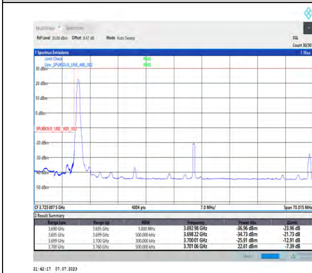
1-N77-3700-3980-PC1.5-30-60-L-4-CP-QPSK-Edge_1RB_Left-1@0-Ant3-1--PASS-see graph
