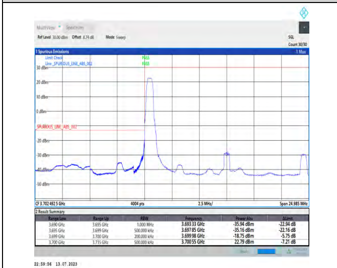
1-N77-3700-3980-PC1.5-30-15-L-4-CP-QPSK-Edge_1RB_Left-1@0-Ant3-1--PASS-see graph
