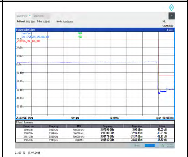
1-N77-3700-3980-PC1.5-30-90-H-6-CP-QPSK-Outer_Full-245@0-Ant3-1--PASS-see graph
