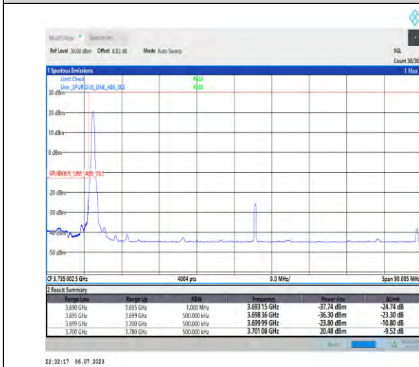
1-N77-3700-3980-PC1-30-80-L-1-DFT-PI2BPSK-Edg e_1RB_Left-1@0-Ant3-1--PASS-see graph
