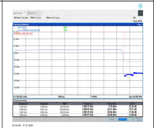
1-N77-3700-3980-PC1.5-30-60-H-6-CP-QPSK-Outer_Full-162@0-Ant3-1--PASS-see graph
