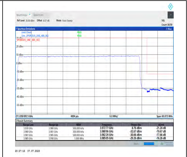
1-N77-3700-3980-PC1.5-30-50-H-3-DFT-PI2BPSK-Outer_Full-128@0-Ant3-1--PASS-see graph
