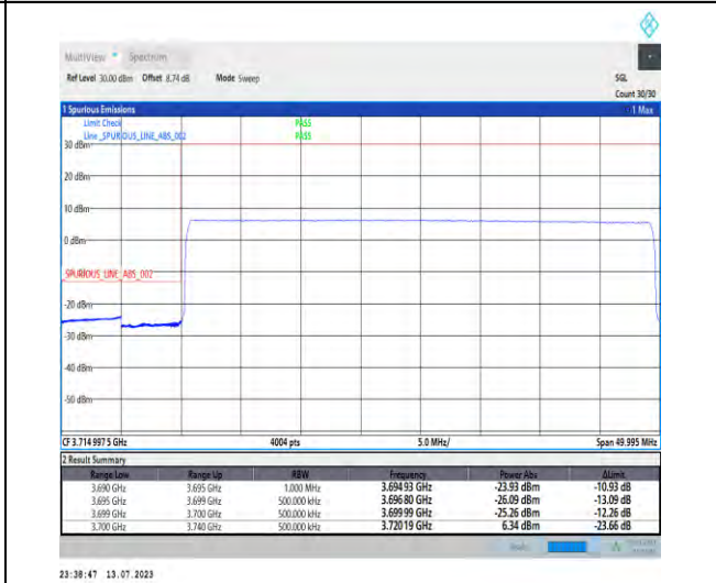
1-N77-3700-3980-PC1.5-30-40-L-6-CP-QPSK-Outer_Full-100@0-Ant3-1--PASS-see graph
