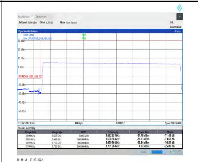
1-N77-3700-3980-PC1.5-30-60-L-6-CP-QPSK-Outer_Full-162@0-Ant3-1--PASS-see graph
