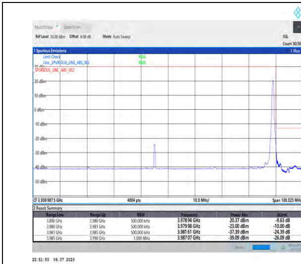
1-N77-3700-3980-PC1-30-90-H-5-CP-QPSK-Edge_1 RB_Right-1@244-Ant3-1--PASS-see graph
