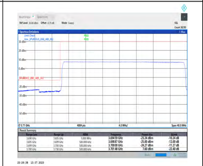
1-N77-3700-3980-PC1.5-30-30-L-6-CP-QPSK-Outer_Full-75@0-Ant3-1--PASS-see graph
