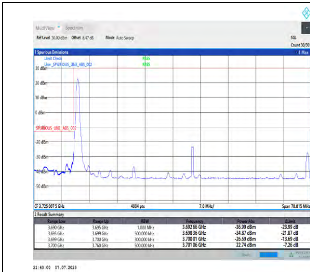
1-N77-3700-3980-PC1.5-30-60-L-1-DFT-PI2BPSK-Edge_1RB_Left-1@0-Ant3-1--PASS-see graph
