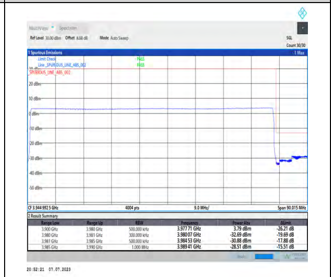
1-N77-3700-3980-PC1.5-30-80-H-6-CP-QPSK-Outer_Full-217@0-Ant3-1--PASS-see graph
