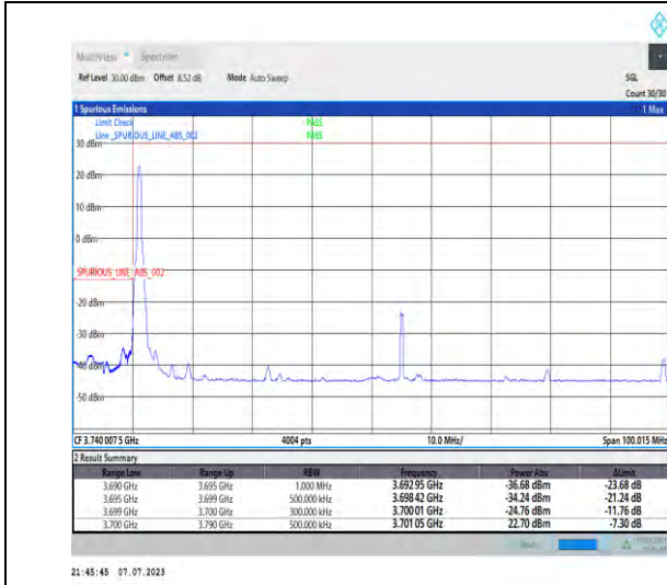
1-N77-3700-3980-PC1.5-30-90-L-1-DFT-PI2BPSK-Edge_1RB_Left-1@0-Ant3-1--PASS-see graph
