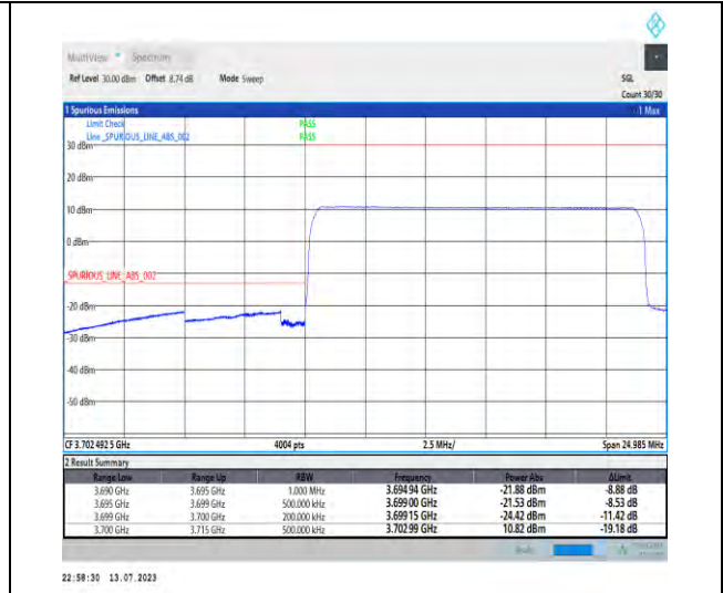
1-N77-3700-3980-PC1.5-30-15-L-3-DFT-PI2BPSK-Outer_Full-36@0-Ant3-1--PASS-see graph
