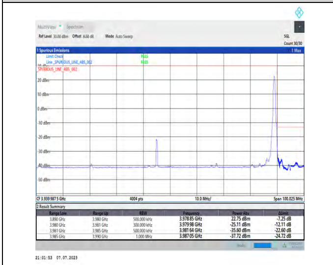
1-N77-3700-3980-PC1.5-30-90-H-5-CP-QPSK-Edge_1RB_Right-1@244-Ant3-1--PASS-see graph
