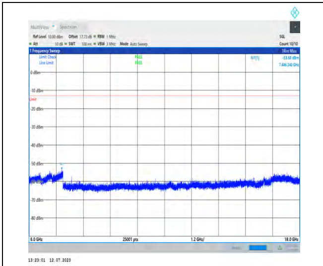
1-N77-3700-3980-PC1.5-30-100-H-1-DFT-PI2BPSK -Inner_1RB_Left-1@1-6000-18000-Ant3-7446.24--5 3.68--13-PASS
