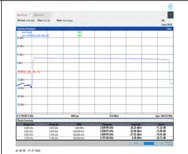
1-N77-3700-3980-PC1.5-30-90-L-3-DFT-PI2BPSK-Outer_Full-240@0-Ant3-1--PASS-see graph
