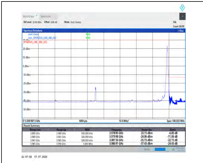
1-N77-3700-3980-PC1.5-30-90-H-2-DFT-PI2BPSK-Edge_1RB_Right-1@244-Ant3-1--PASS-see graph
