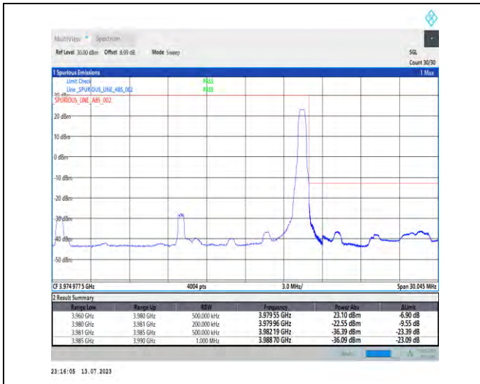
1-N77-3700-3980-PC1.5-30-20-H-2-DFT-PI2BPSK-Edge_1RB_Right-1@50-Ant3-1--PASS-see graph
