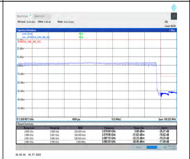
1-N77-3700-3980-PC1-30-90-H-3-DFT-PI2BPSK-Outer_Full-240@0-Ant3-1--PASS-see graph
