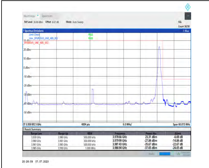
1-N77-3700-3980-PC1.5-30-50-H-2-DFT-PI2BPSK-Edge_1RB_Right-1@132-Ant3-1--PASS-see graph
