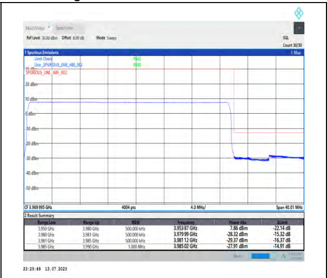
1-N77-3700-3980-PC1.5-30-30-H-3-DFT-PI2BPSK-Outer_Full-75@0-Ant3-1--PASS-see graph
