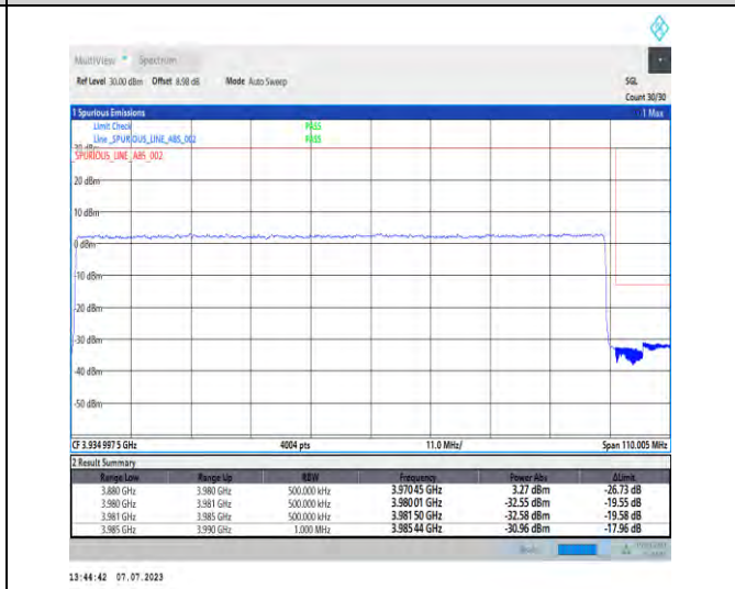
1-N77-3700-3980-PC1-30-100-H-3-DFT-PI2BPSK-Outer_Full-270@0-Ant3-1--PASS-see graph
