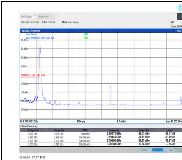
1-N77-3700-3980-PC1.5-30-80-L-1-DFT-PI2BPSK-Edge_1RB_Left-1@0-Ant3-1--PASS-see graph
