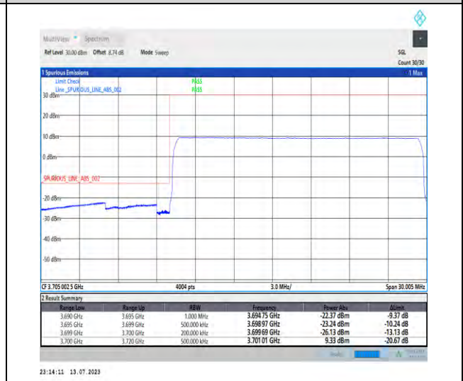
1-N77-3700-3980-PC1.5-30-20-L-6-CP-QPSK-Outer_Full-51@0-Ant3-1--PASS-see graph
