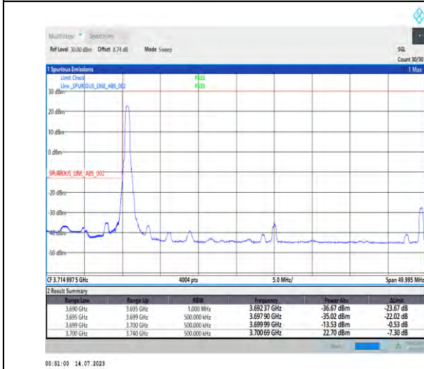
1-N77-3700-3980-PC1.5-30-40-L-4-CP-QPSK-Edge_1RB_Left-1@0-Ant3-1--PASS-see graph
