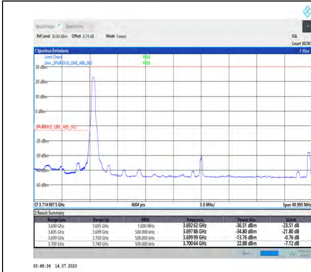
1-N77-3700-3980-PC1.5-30-40-L-1-DFT-PI2BPSK-Edge_1RB_Left-1@0-Ant3-1--PASS-see graph
