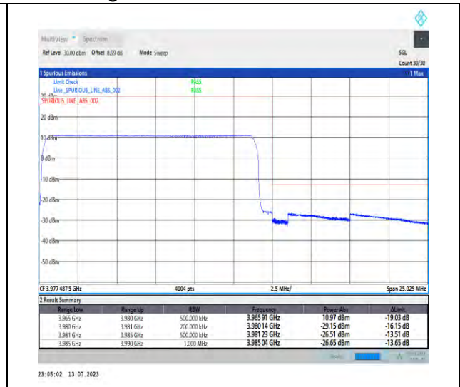
1-N77-3700-3980-PC1.5-30-15-H-3-DFT-PI2BPSK-Outer_Full-36@0-Ant3-1--PASS-see graph
