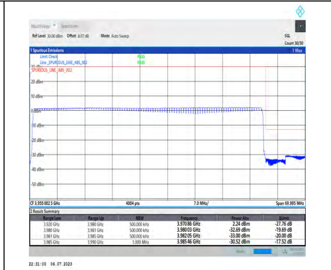
1-N77-3700-3980-PC1-30-60-H-6-CP-QPSK-Outer _Full-162@0-Ant3-1--PASS-see graph
