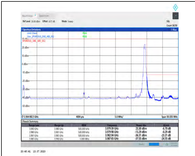
1-N77-3700-3980-PC1.5-30-40-H-2-DFT-PI2BPSK-Edge_1RB_Right-1@105-Ant3-1--PASS-see graph
