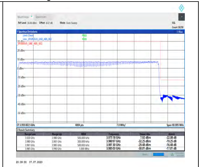
1-N77-3700-3980-PC1.5-30-60-H-3-DFT-PI2BPSK-Outer_Full-162@0-Ant3-1--PASS-see graph
