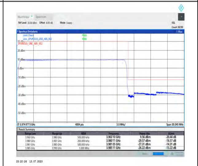
1-N77-3700-3980-PC1.5-30-20-H-6-CP-QPSK-Outer_Full-51@0-Ant3-1--PASS-see graph
