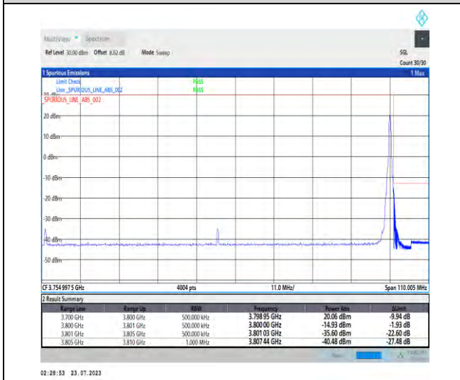
1-N77-3700-3980-PC1-30-100-H-2-DFT-PI2BPSK-Outer_Full-1@0-Ant3-1--PASS-see graph
