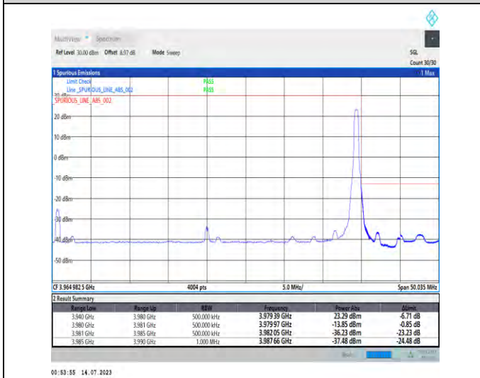
1-N77-3700-3980-PC1.5-30-40-H-5-CP-QPSK-Edge_1RB_Right-1@105-Ant3-1--PASS-see graph
