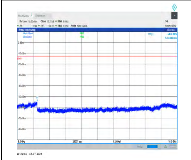
1-N77-3700-3980-PC1.5-30-100-M-1-DFT-PI2BPSK -Inner_1RB_Left-1@1-6000-18000-Ant3-7496.64--5 4.36--13-PASS
