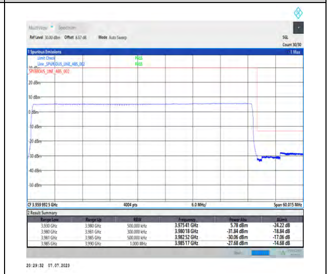
1-N77-3700-3980-PC1.5-30-50-H-6-CP-QPSK-Outer_Full-133@0-Ant3-1--PASS-see graph
