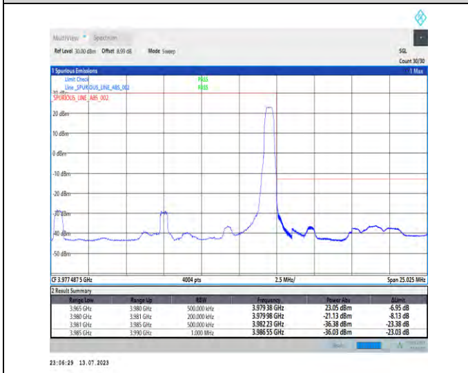
1-N77-3700-3980-PC1.5-30-15-H-5-CP-QPSK-Edge_1RB_Right-1@37-Ant3-1--PASS-see graph
