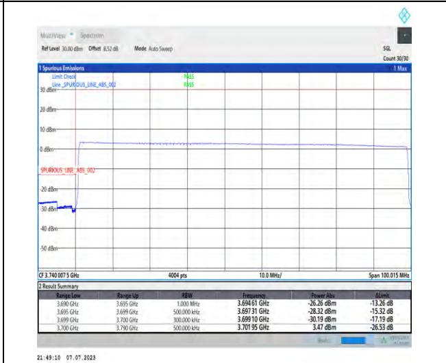
1-N77-3700-3980-PC1.5-30-90-L-6-CP-QPSK-Outer_Full-245@0-Ant3-1--PASS-see graph
