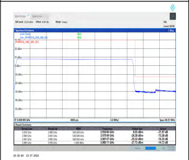
1-N77-3700-3980-PC1.5-30-30-H-6-CP-QPSK-Outer_Full-75@0-Ant3-1--PASS-see graph
