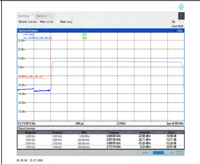
1-N77-3700-3980-PC1.5-30-40-L-3-DFT-PI2BPSK-Outer_Full-100@0-Ant3-1--PASS-see graph
