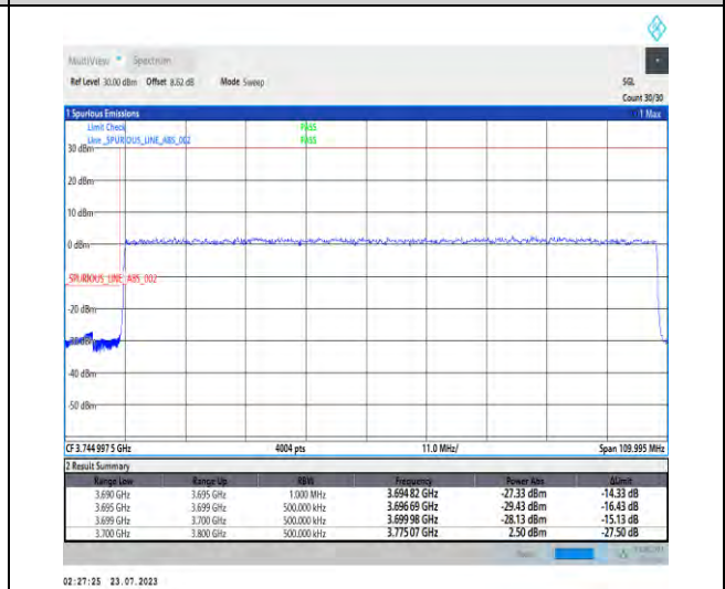
1-N77-3700-3980-PC1-30-100-L-3-DFT-PI2BPSK- Outer_Full-270@0-Ant3-1--PASS-see graph
