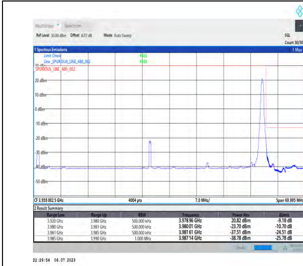
1-N77-3700-3980-PC1-30-60-H-5-CP-QPSK-Edge_1 RB_Right-1@161-Ant3-1--PASS-see graph
