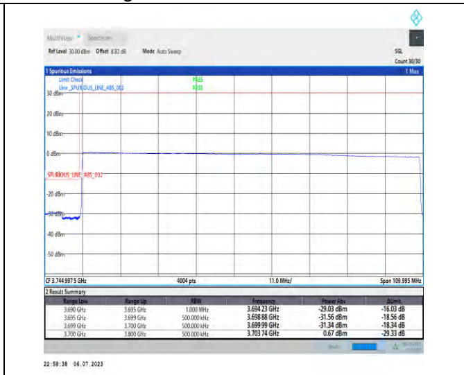
1-N77-3700-3980-PC1-30-100-L-6-CP-QPSK-Outer_Full-273@0-Ant3-1--PASS-see graph
