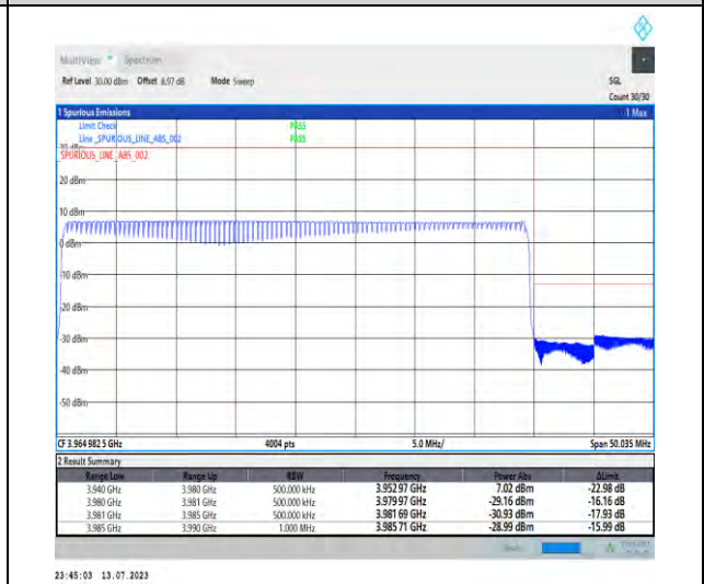
1-N77-3700-3980-PC1.5-30-40-H-6-CP-QPSK-Outer_Full-100@0-Ant3-1--PASS-see graph
