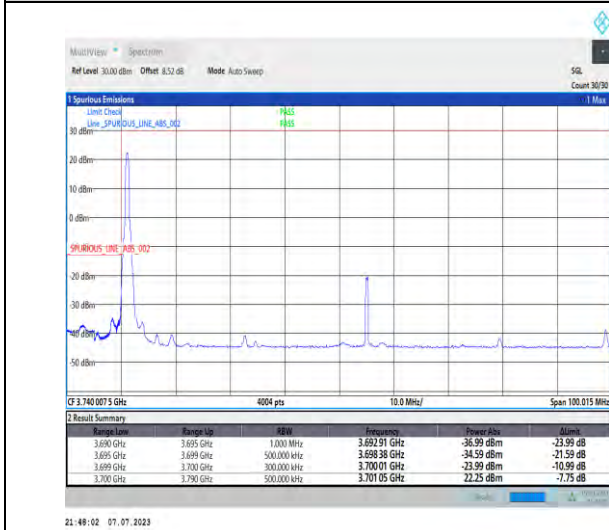
1-N77-3700-3980-PC1.5-30-90-L-4-CP-QPSK-Edge_1RB_Left-1@0-Ant3-1--PASS-see graph
