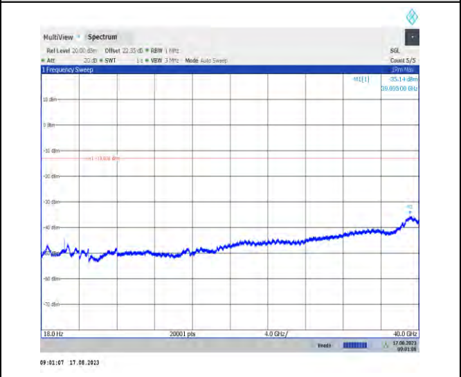
1-N77-3700-3980-PC1.5-30-100-M-1-DFT-PI2BPSK-I nner_1RB_Left-1@1-18000-40000-Ant3-18000.00--5 7.10--13-PASS
