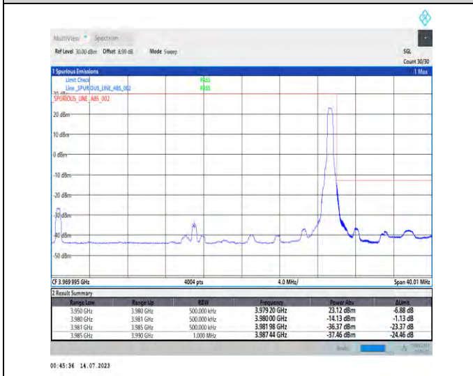
1-N77-3700-3980-PC1.5-30-30-H-5-CP-QPSK-Edge_1RB_Right-1@77-Ant3-1--PASS-see graph
