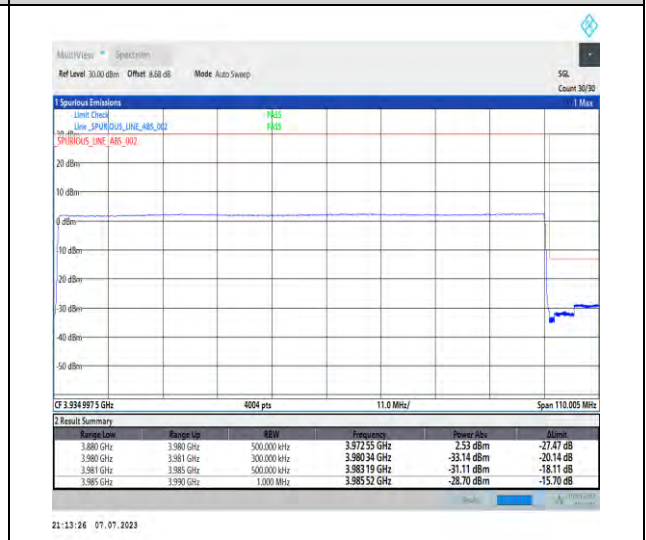
1-N77-3700-3980-PC1.5-30-100-H-6-CP-QPSK-O uter_Full-273@0-Ant3-1--PASS-see graph
