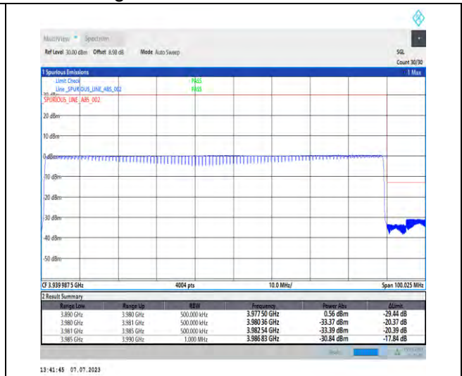
1-N77-3700-3980-PC1-30-90-H-6-CP-QPSK-Outer _Full-245@0-Ant3-1--PASS-see graph
