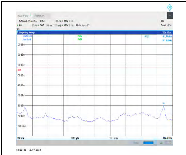
1-N77-3700-3980-PC1.5-30-100-H-1-DFT-PI2BPSK -Inner_1RB_Left-1@1-0.009-0.30-Ant3-0.14--81.39-- -43-PASS
