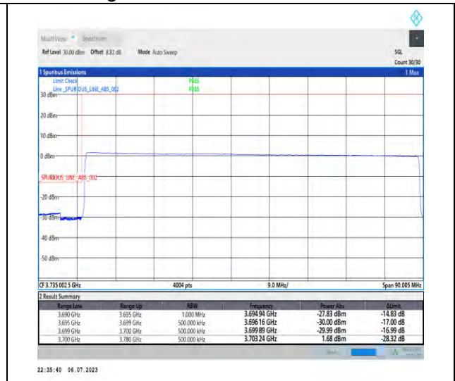
1-N77-3700-3980-PC1-30-80-L-6-CP-QPSK-Outer_Full-217@0-Ant3-1--PASS-see graph
