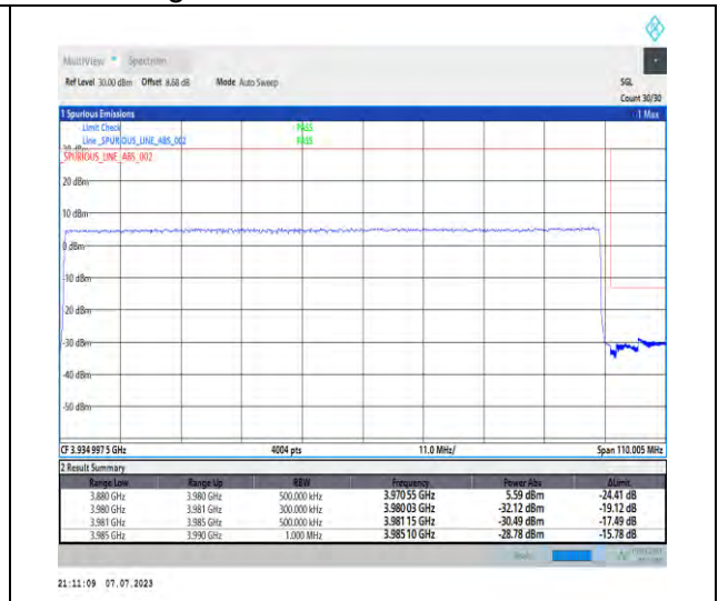
1-N77-3700-3980-PC1.5-30-100-H-3-DFT-PI2BPS K-Outer_Full-270@0-Ant3-1--PASS-see graph
