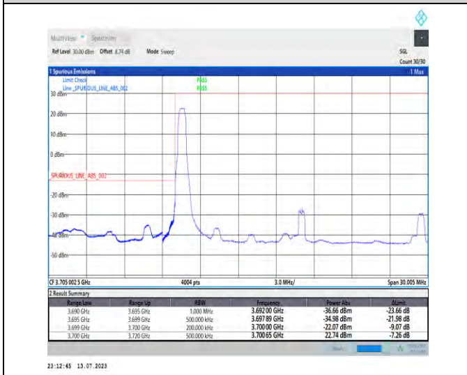
1-N77-3700-3980-PC1.5-30-20-L-4-CP-QPSK-Edge_1RB_Left-1@0-Ant3-1--PASS-see graph
