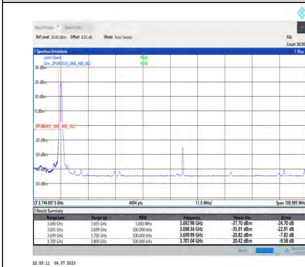
1-N77-3700-3980-PC1-30-100-L-1-DFT-PI2BPSK-Ed ge_1RB_Left-1@0-Ant3-1--PASS-see graph
