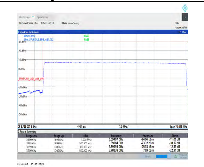
1-N77-3700-3980-PC1.5-30-60-L-3-DFT-PI2BPSK-Outer_Full-162@0-Ant3-1--PASS-see graph
