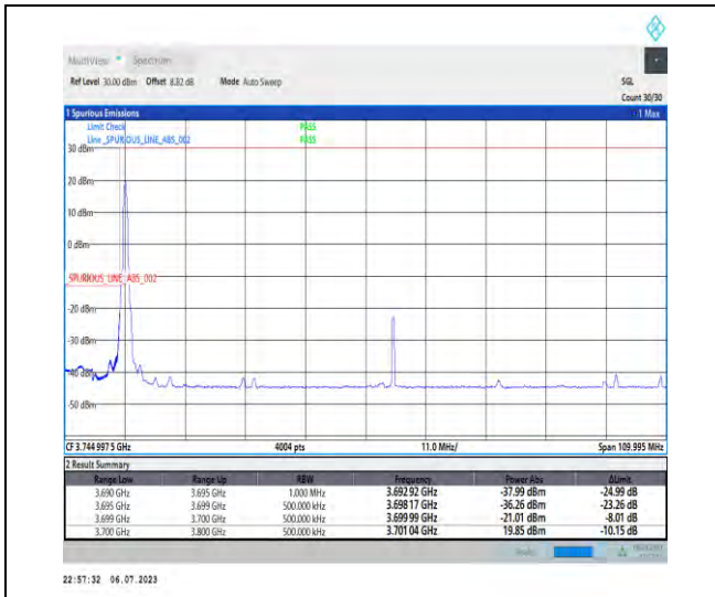
1-N77-3700-3980-PC1-30-100-L-4-CP-QPSK-Edge_1RB_Left-1@0-Ant3-1--PASS-see graph
