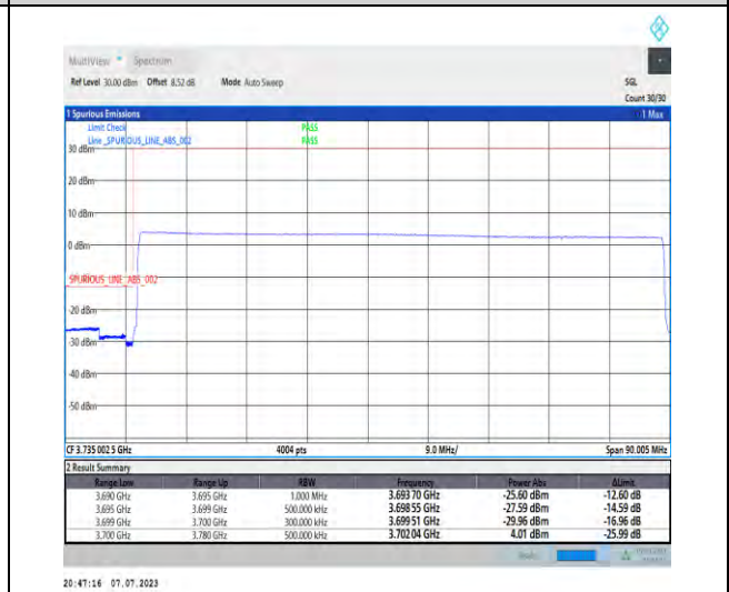
1-N77-3700-3980-PC1.5-30-80-L-6-CP-QPSK-Outer_Full-217@0-Ant3-1--PASS-see graph
