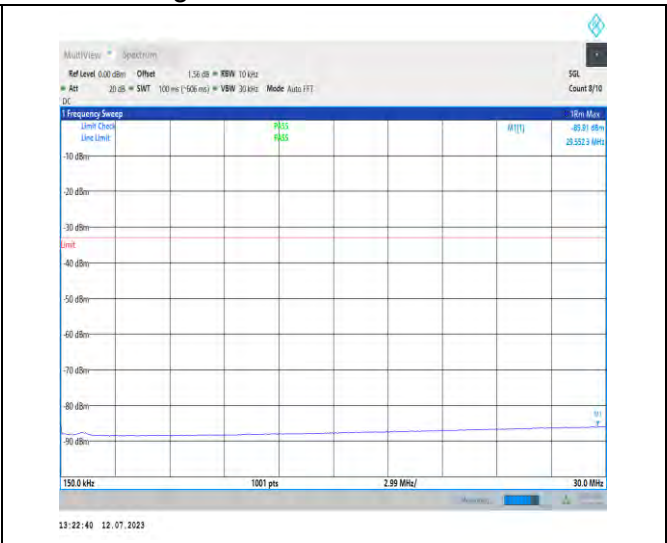
1-N77-3700-3980-PC1.5-30-100-H-1-DFT-PI2BPSK- Inner_1RB_Left-1@1-0.30-30-Ant3-29.55--85.91--33- PASS
