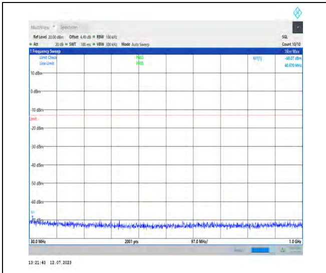
1-N77-3700-3980-PC1.5-30-100-M-1-DFT-PI2BPSK -Inner_1RB_Left-1@1-30-1000-Ant3-40.67--69.07-- 13-PASS
