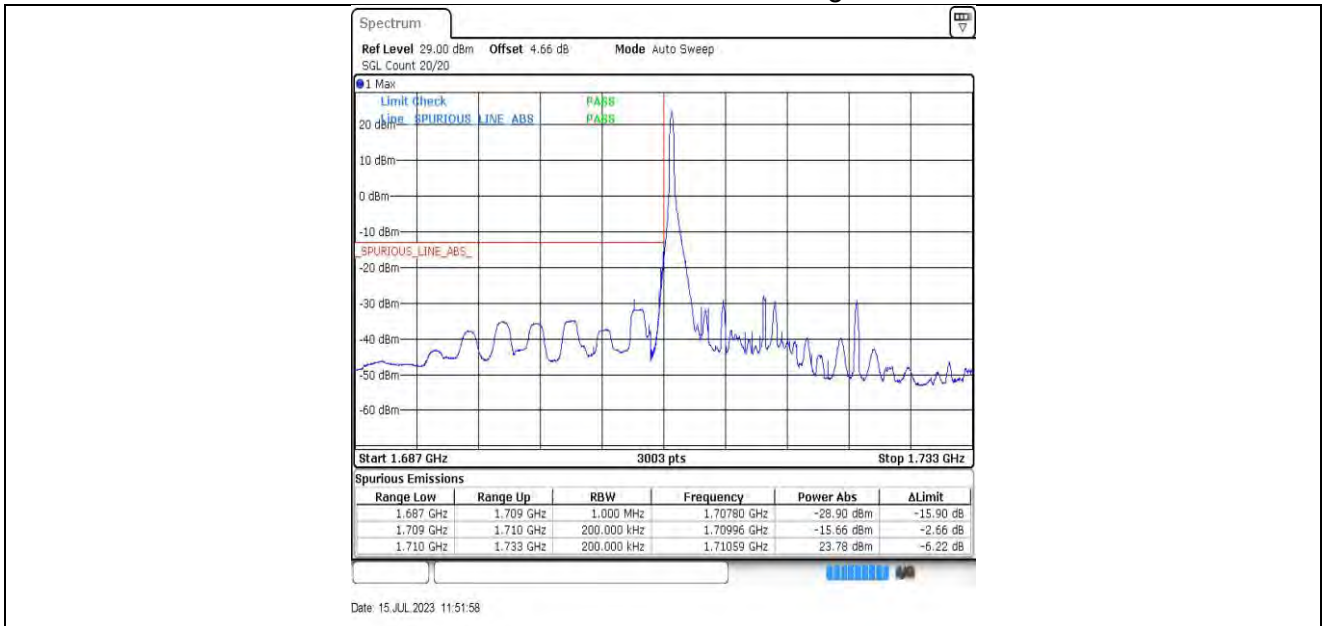
10MHz-5MHz_QPSK@QPSK-QPSK@QPSK_132022-132094_1RB#0@50RB#0-0RB#0@25RB#0
