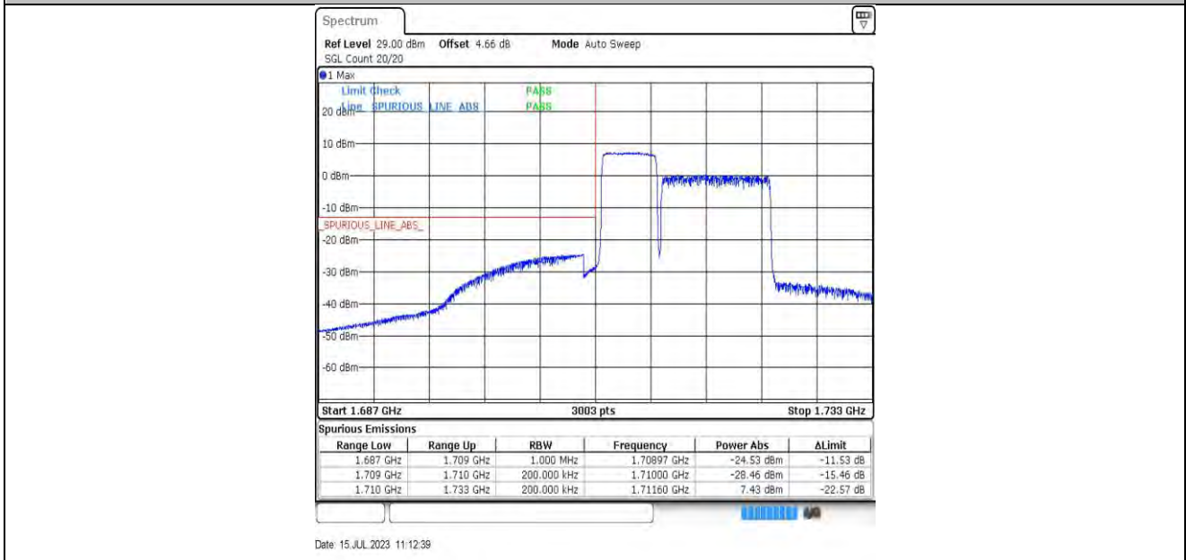
5MHz-10MHz_QPSK@QPSK-QPSK@QPSK_132000-132072_25RB#0@25RB#0-50RB#0@50RB#0
