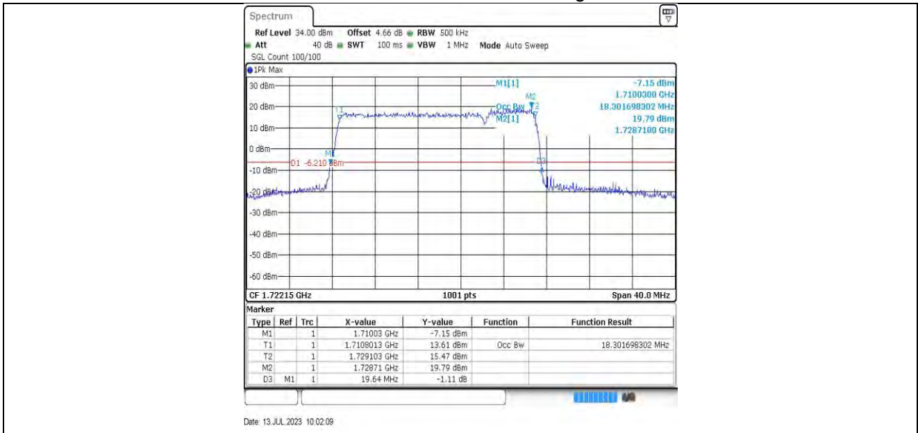
15MHz-5MHz-132047-132140 64QAM-64QAM
