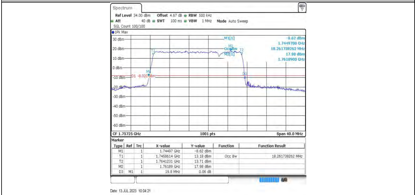
15MHz-5MHz-132398-132491 64QAM-64QAM
