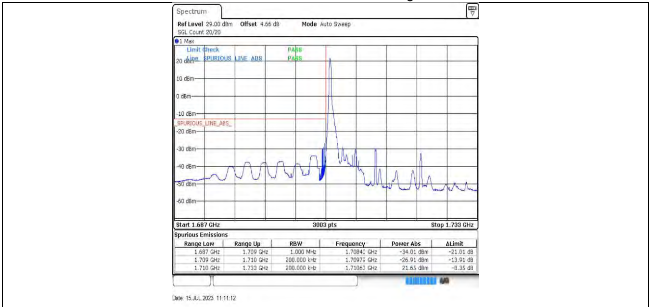
5MHz-10MHz_QPSK@QPSK-QPSK@QPSK_132000-132072_1RB#0@25RB#0-0RB#0@50RB#0
