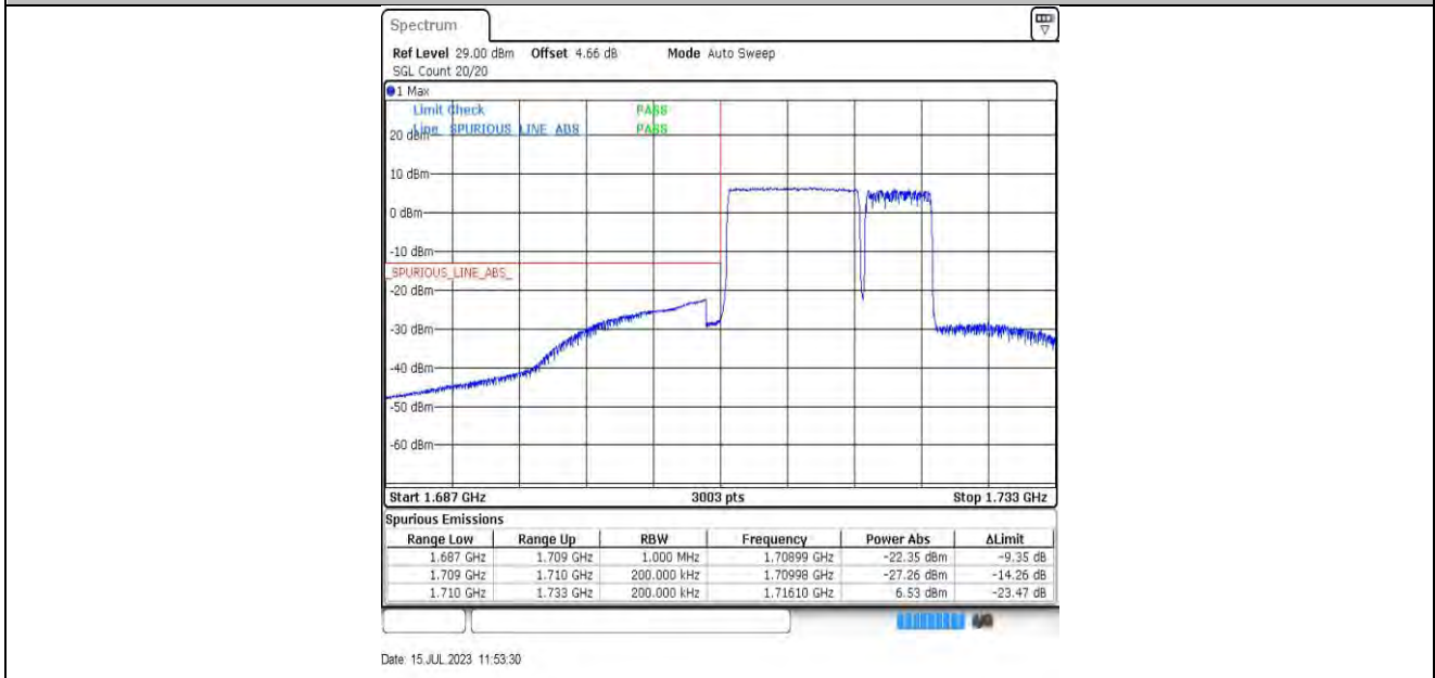
10MHz-5MHz_QPSK@QPSK-QPSK@QPSK_132022-132094_50RB#0@50RB#0-25RB#0@25RB#0
