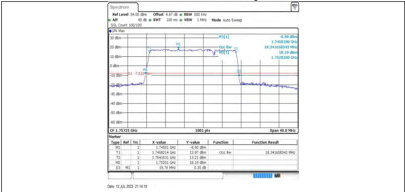
15MHz-5MHz-132398-132491 16QAM-16QAM
