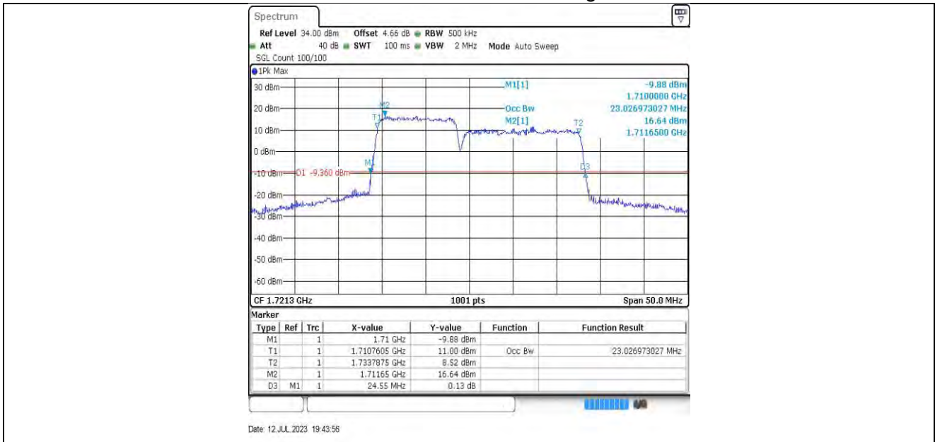
10MHz-15MHz-132025-132145 64QAM-64QAM
