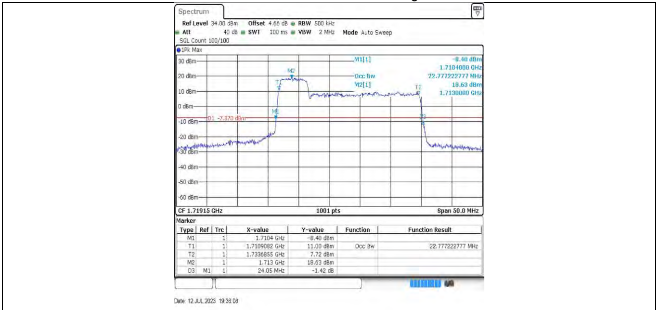
5MHz-20MHz-132005-132122 64QAM-64QAM
