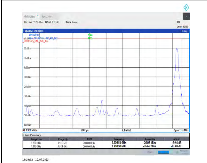
1-N2-PC3-15-20-H-5-CP-QPSK-Edge_1RB_Right-1@105-Ant3-1-seegraph-PASS-see graph
