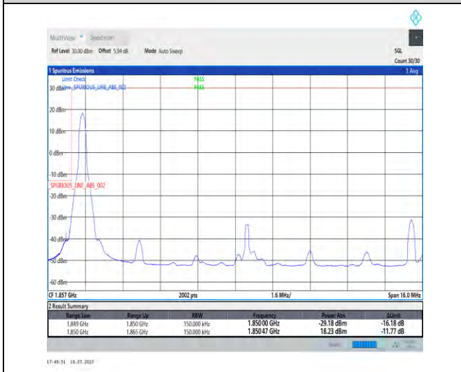
1-N2-PC3-15-15-L-4-CP-QPSK-Edge_1RB_Left-1@0 -Ant3-1-seegraph-PASS-see graph
