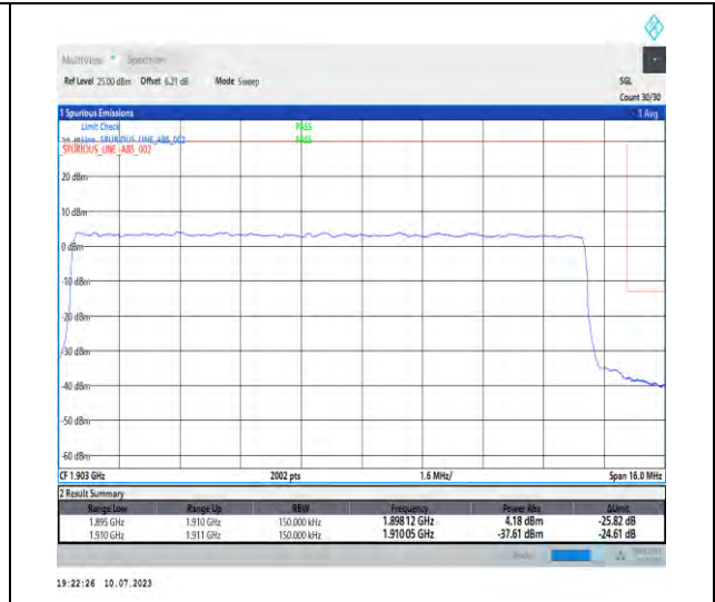
1-N2-PC3-15-15-H-3-DFT-PI2BPSK-Outer_Full-75@0-Ant3-1-seegraph-PASS-see graph
