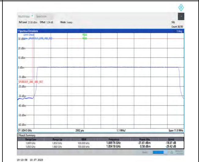
1-N2-PC3-15-10-L-6-CP-QPSK-Outer_Full-52@0-Ant3-1-seegraph-PASS-see graph
