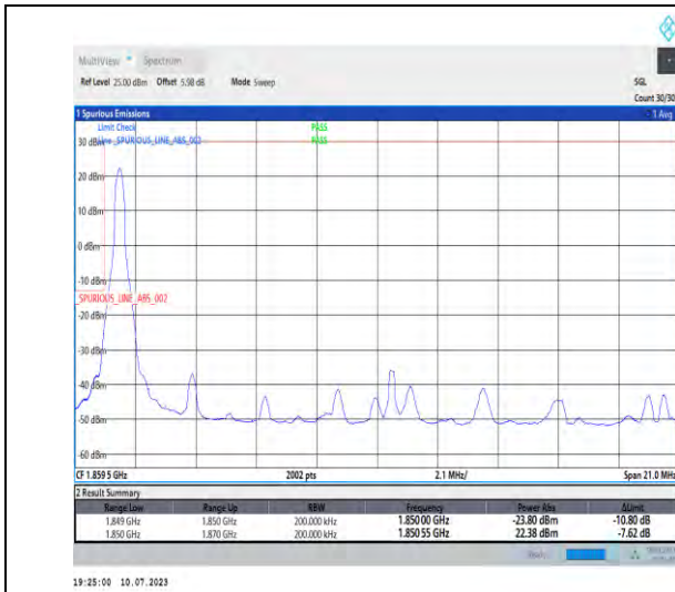
1-N2-PC3-15-20-L-1-DFT-PI2BPSK-Edge_1RB_Left-1@0-Ant3-1-seegraph-PASS-see graph
