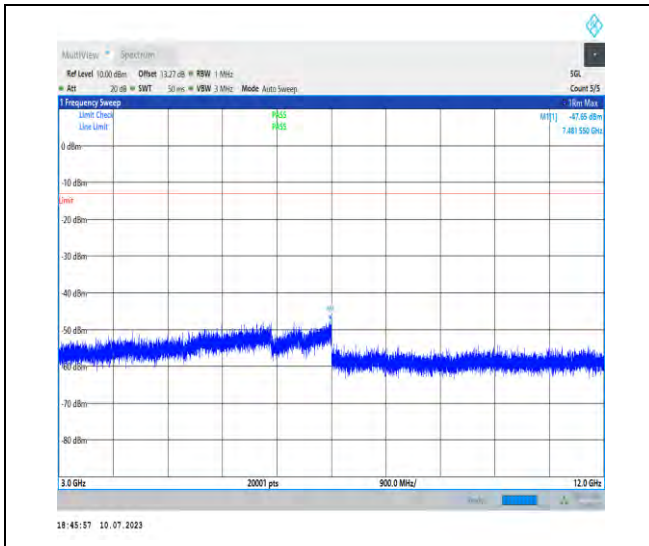
1-N2-PC3-15-20-H-1-DFT-PI2BPSK-Inner_1RB_Lef t-1@1-3000-12000-Ant3-7481.55--47.65--13-PASS
