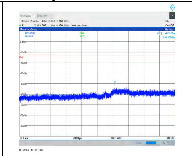
1-N2-PC3-15-20-H-1-DFT-PI2BPSK-Inner_1RB_Left- 1@1-12000-20000-Ant3-16907.60--41.79--13-PASS
