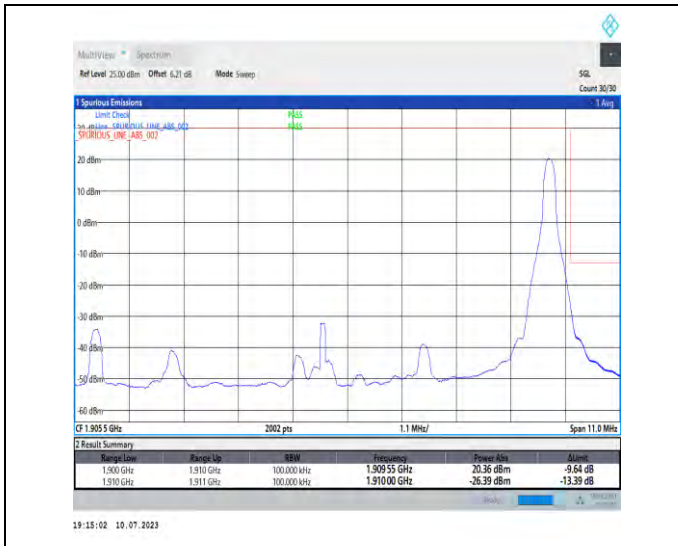
1-N2-PC3-15-10-H-2-DFT-PI2BPSK-Edge_1RB_Right-1@51-Ant3-1-seegraph-PASS-see graph
