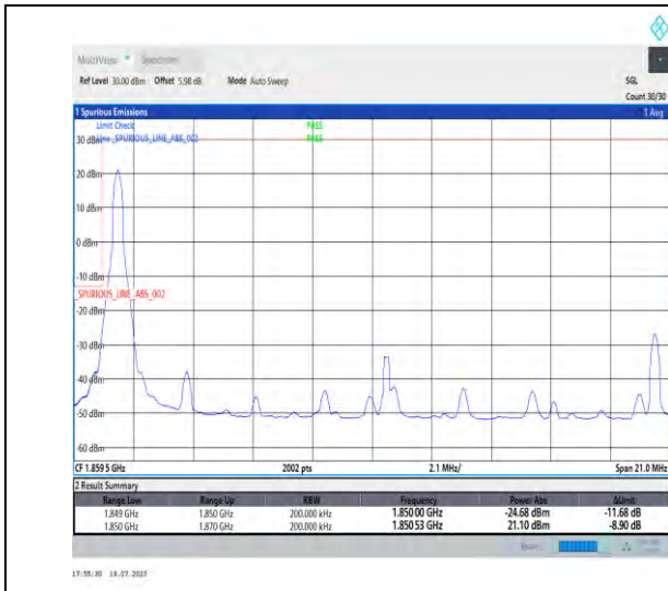
1-N2-PC3-15-20-L-1-DFT-PI2BPSK-Edge_1RB_Left-1@0-Ant3-1-seegraph-PASS-see graph
