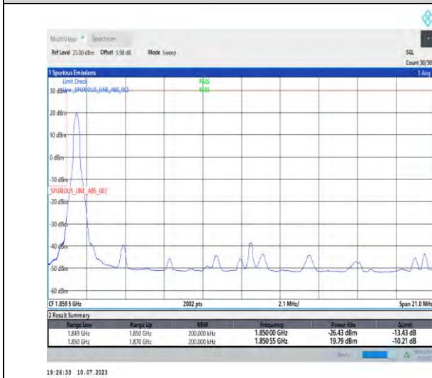
1-N2-PC3-15-20-L-4-CP-QPSK-Edge_1RB_Left-1@0-Ant3-1-seegraph-PASS-see graph
