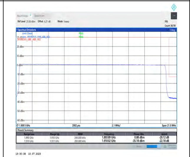
1-N2-PC3-15-20-H-6-CP-QPSK-Outer_Full-106@0-Ant3-1-seegraph-PASS-see graph
