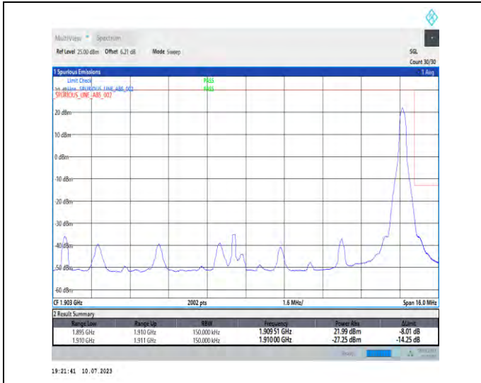
1-N2-PC3-15-15-H-2-DFT-PI2BPSK-Edge_1RB_Right-1@78-Ant3-1-seegraph-PASS-see graph
