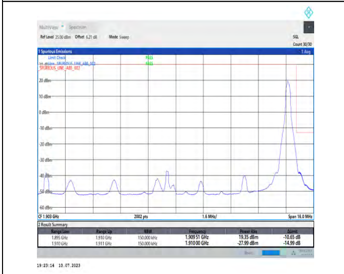
1-N2-PC3-15-15-H-5-CP-QPSK-Edge_1RB_Right-1@78-Ant3-1-seegraph-PASS-see graph
