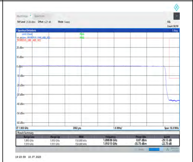
1-N2-PC3-15-15-H-6-CP-QPSK-Outer_Full-79@0-Ant3-1-seegraph-PASS-see graph
