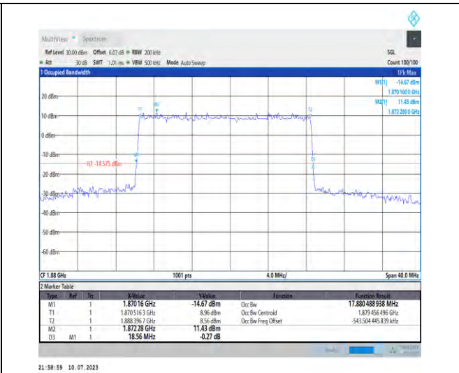
1-N2-PC3-15-20-M-3-DFT-16QAM-Outet_Full-100@ 0-Ant3-17.88-18.560-≤20-PASS
