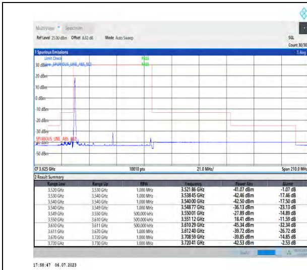
1-N48-PC3-30-60-L-1-DFT-PI2BPSK-Edge_1RB_Left -1@0-Ant3-1--PASS-see graph
