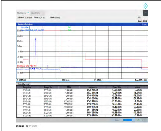
1-N48-PC3-30-40-L-4-CP-QPSK-Edge_1RB_Left-1@ 0-Ant3-1--PASS-see graph
