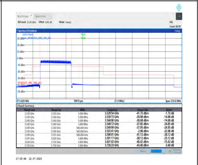
1-N48-PC3-30-40-L-6-CP-QPSK-Outer_Full-106@ 0-Ant3-1--PASS-see graph
