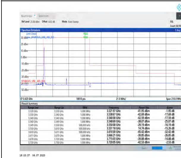
1-N48-PC3-30-60-L-4-CP-QPSK-Edge_1RB_Left-1@ 0-Ant3-1--PASS-see graph
