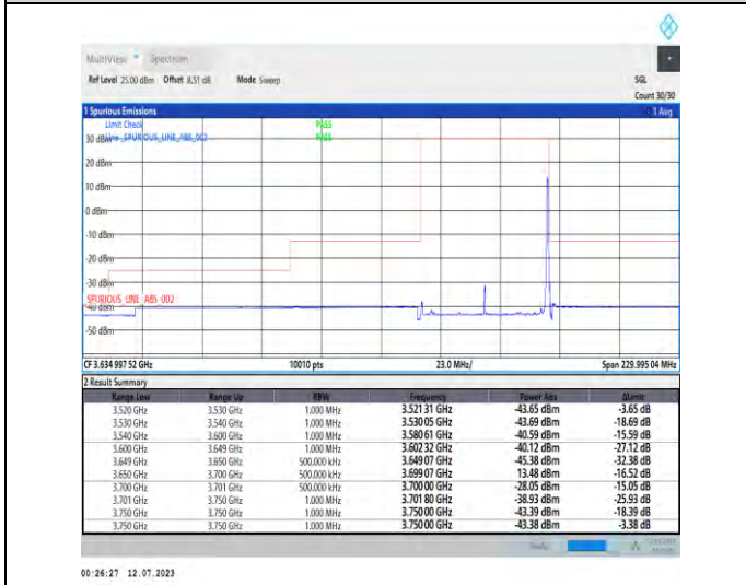
1-N48-PC3-30-50-H-5-CP-QPSK-Edge_1RB_Right-1 @132-Ant3-1--PASS-see graph
