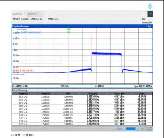
1-N48-PC3-30-50-H-6-CP-QPSK-Outer_Full-133 @0-Ant3-1--PASS-see graph
