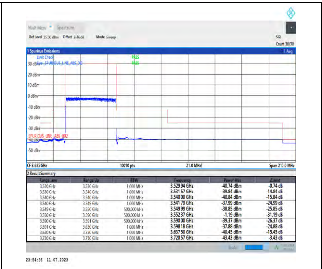
1-N48-PC3-30-40-L-3-DFT-PI2BPSK-Outer_Full-10 0@0-Ant3-1--PASS-see graph
