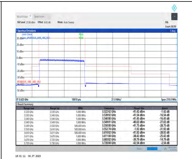
1-N48-PC3-30-60-L-3-DFT-PI2BPSK-Outer_Full-16 2@0-Ant3-1--PASS-see graph
