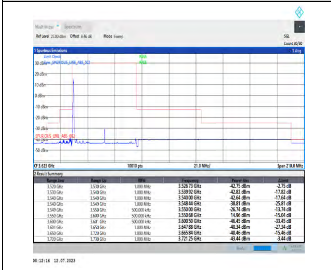
1-N48-PC3-30-50-L-4-CP-QPSK-Edge_1RB_Left-1@ 0-Ant3-1--PASS-see graph
