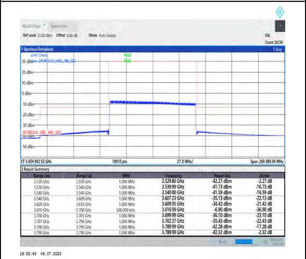
1-N48-PC3-30-90-H-6-CP-QPSK-Outer_Full-245 @0-Ant3-1--PASS-see graph
