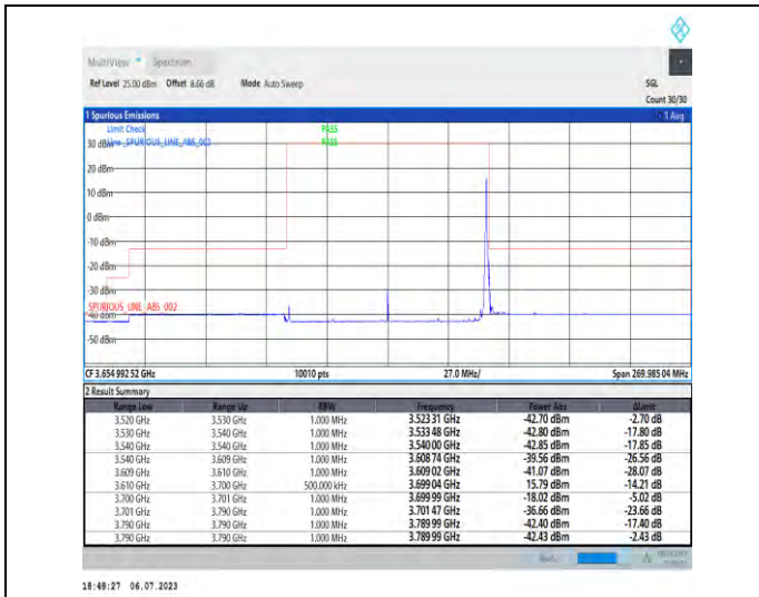
1-N48-PC3-30-90-H-2-DFT-PI2BPSK-Edge_1RB_Right t-1@244-Ant3-1--PASS-see graph
