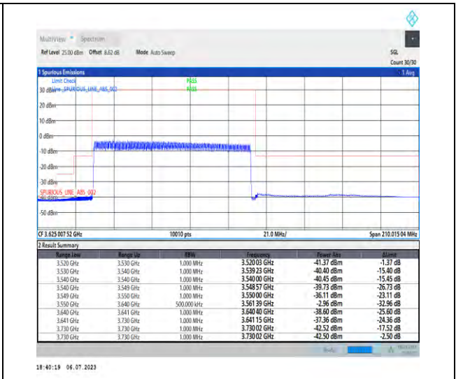
1-N48-PC3-30-90-L-3-DFT-PI2BPSK-Outer_Full-24 0@0-Ant3-1--PASS-see graph
