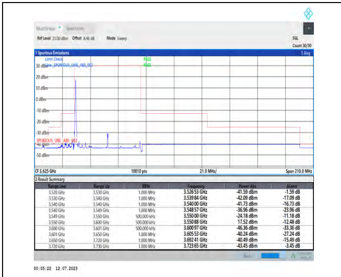
1-N48-PC3-30-50-L-1-DFT-PI2BPSK-Edge_1RB_Left -1@0-Ant3-1--PASS-see graph
