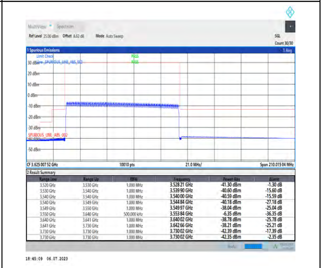
1-N48-PC3-30-90-L-6-CP-QPSK-Outer_Full-245@ 0-Ant3-1--PASS-see graph
