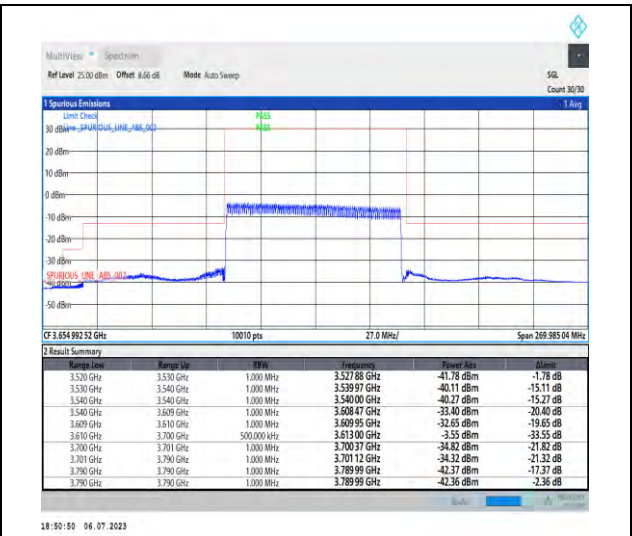
1-N48-PC3-30-90-H-3-DFT-PI2BPSK-Outer_Full-2 40@0-Ant3-1--PASS-see graph
