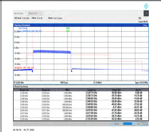
1-N48-PC3-30-60-L-6-CP-QPSK-Outer_Full-162@ 0-Ant3-1--PASS-see graph
