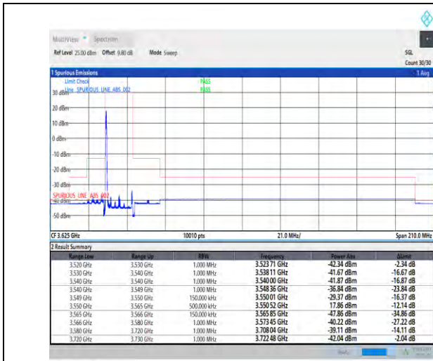
1-N48-PC3-30-15-L-1-DFT-PI2BPSK-Edge_1RB_Left-1@0-Ant3-1--PASS-see graph
