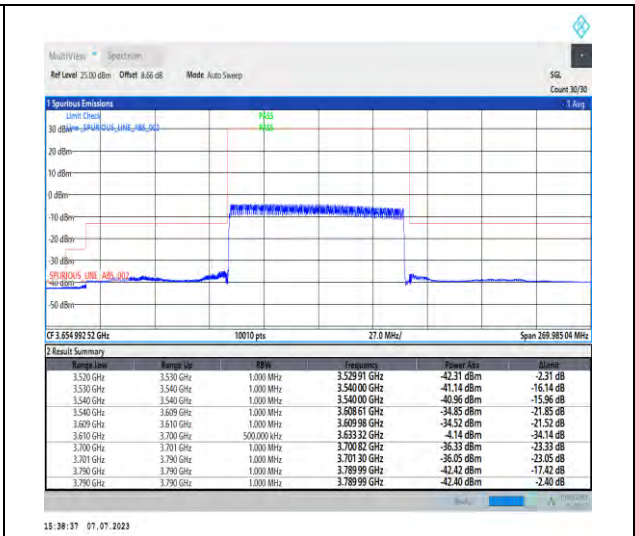
1-N48-PC3-30-90-H-3-DFT-PI2BPSK-Outer_Full-240@0-Ant3-1--PASS-see graph
