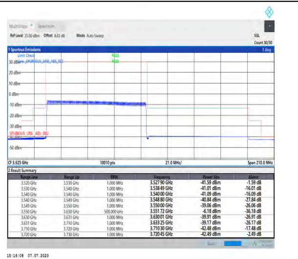
1-N48-PC3-30-80-L-6-CP-QPSK-Outer_Full-217@ 0-Ant3-1--PASS-see graph
