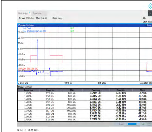
1-N48-PC3-30-20-L-4-CP-QPSK-Edge_1RB_Left-1@0-Ant3-1--PASS-see graph
