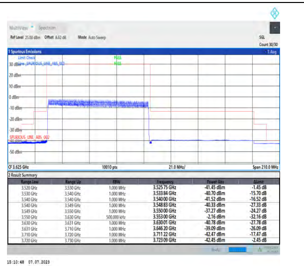
1-N48-PC3-30-80-L-3-DFT-PI2BPSK-Outer_Full-10 0@0-Ant3-1--PASS-see graph
