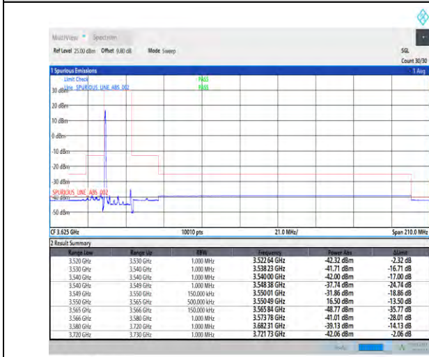
1-N48-PC3-30-15-L-1-DFT-PI2BPSK-Edge_1RB_Left-1@0-Ant3-1--PASS-see graph
