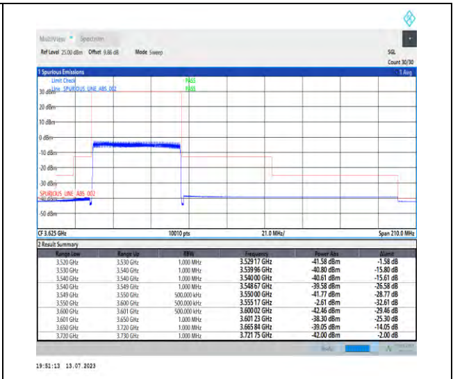
1-N48-PC3-30-50-L-3-DFT-PI2BPSK-Outer_Full-12 8@0-Ant3-1--PASS-see graph
