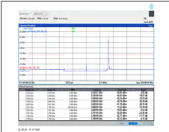
1-N48-PC3-30-90-H-2-DFT-PI2BPSK-Edge_1RB_Right-t-1@244-Ant3-1--PASS-see graph
