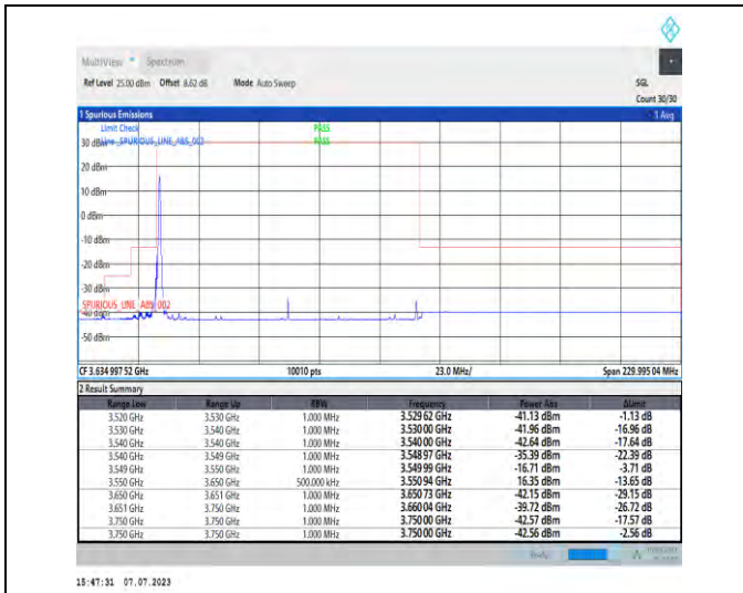
1-N48-PC3-30-100-L-1-DFT-PI2BPSK-Edge_1RB_Lef t-1@0-Ant3-1--PASS-see graph
