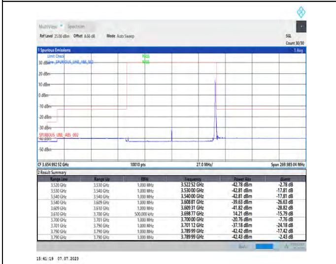
1-N48-PC3-30-90-H-5-CP-QPSK-Edge_1RB_Right-1@244-Ant3-1--PASS-see graph
