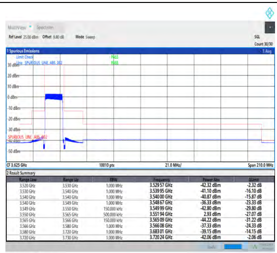
1-N48-PC3-30-15-L-3-DFT-PI2BPSK-Outer_Full-36@0Ant3-1--PASS-see graph
