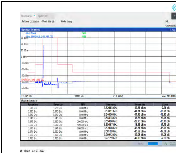
1-N48-PC3-30-20-L-1-DFT-PI2BPSK-Edge_1RB_Left-1@0-Ant3-1--PASS-see graph
