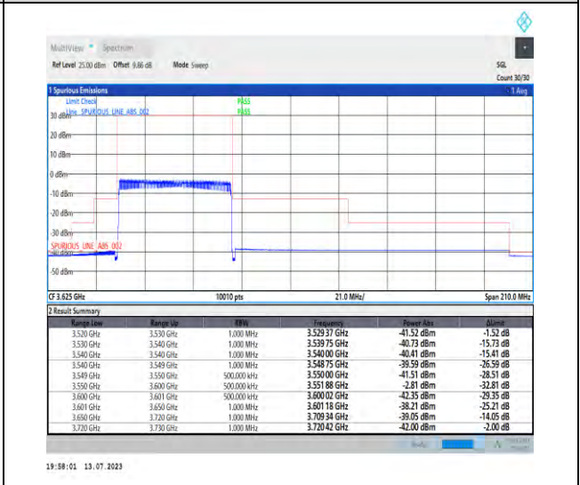
1-N48-PC3-30-50-L-6-CP-QPSK-Outer_Full-133@0 -Ant3-1--PASS-see graph
