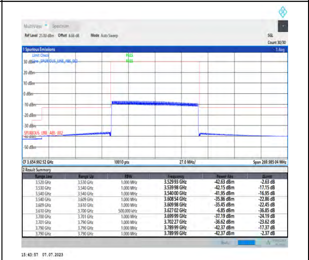
1-N48-PC3-30-90-H-6-CP-QPSK-Outer_Full-245@0-Ant3-1--PASS-see graph
