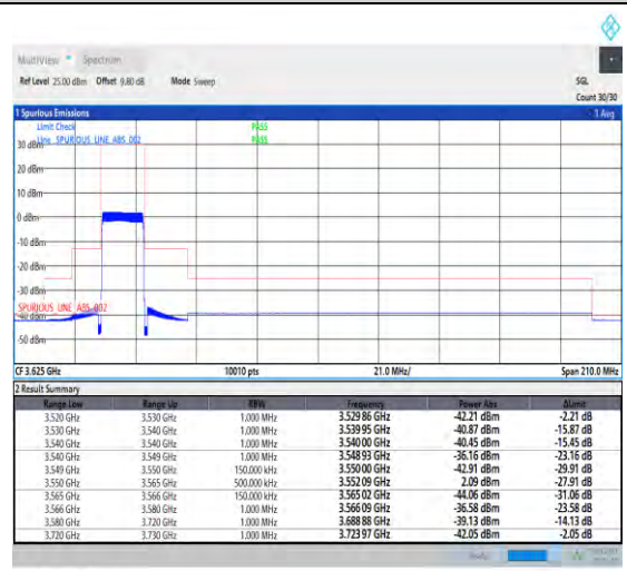
1-N48-PC3-30-15-L-3-DFT-PI2BPSK-Outer_Full-36@0Ant3-1--PASS-see graph
