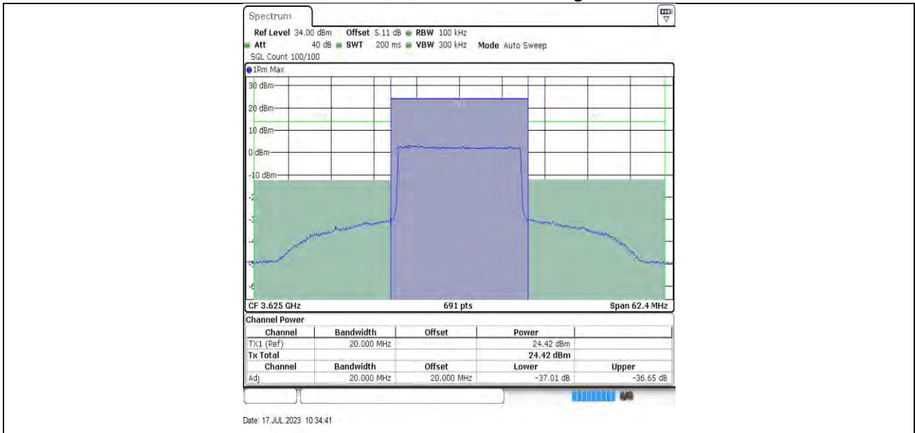
20MHz-55990
