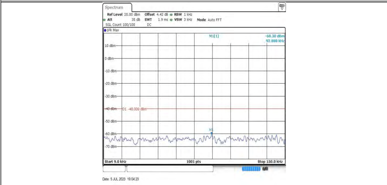
20MHz-55990
