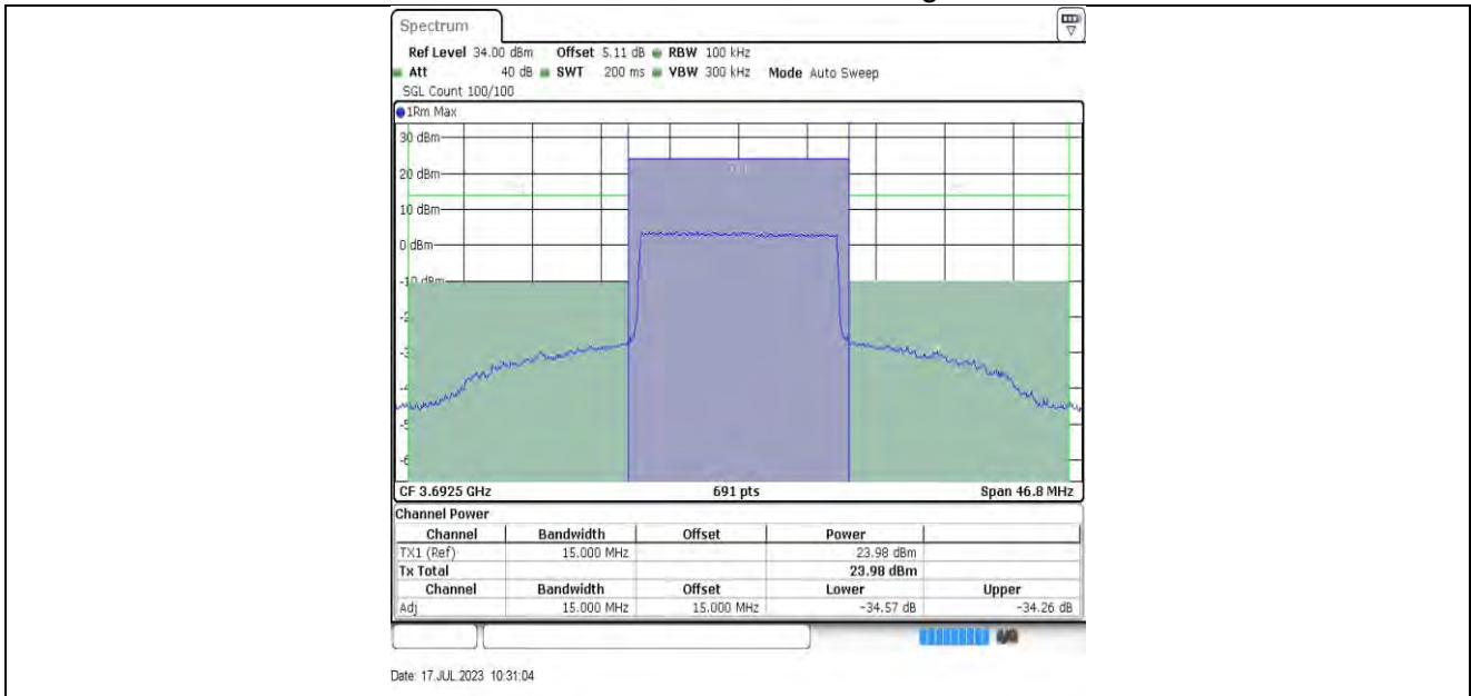
15MHz-56665
