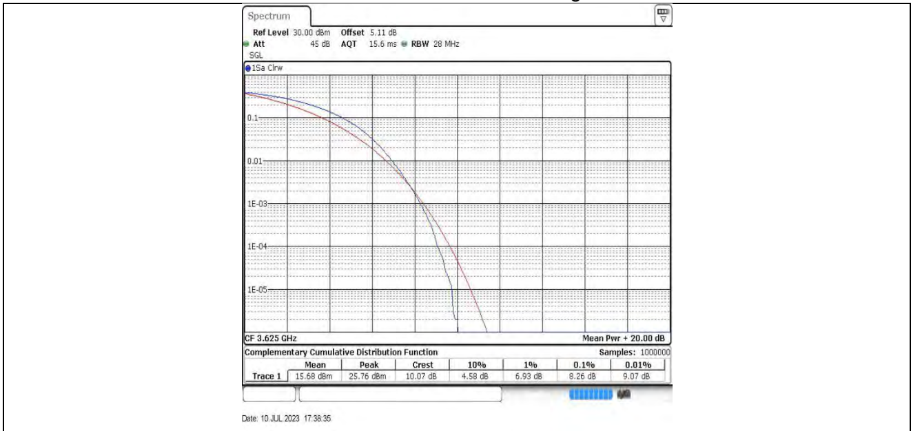
20MHz-55990 256QAM
