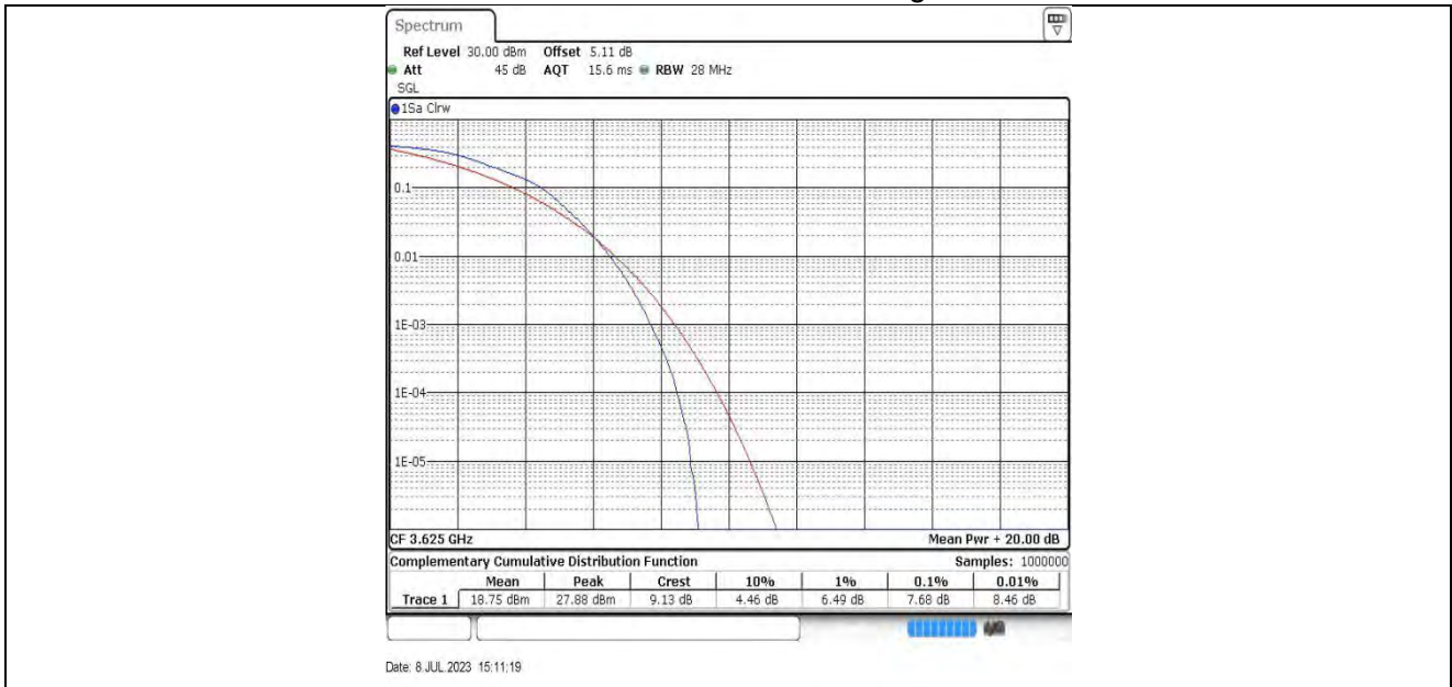
20MHz-55990 16QAM
