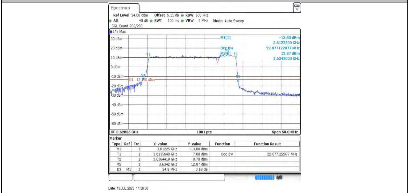
20MHz-5MHz-55965-56082 64QAM-64QAM
