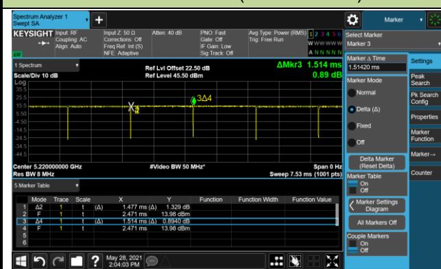
802.11ax-HE20 (T = 1.477ms)
