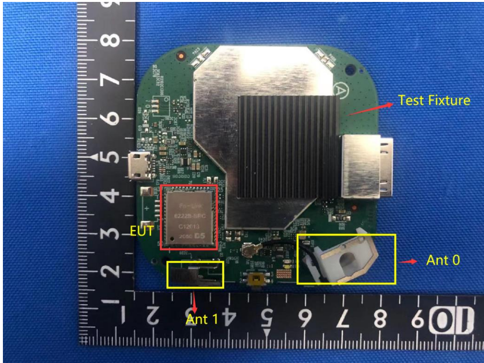
(1) Test Fixture & Module Photo
