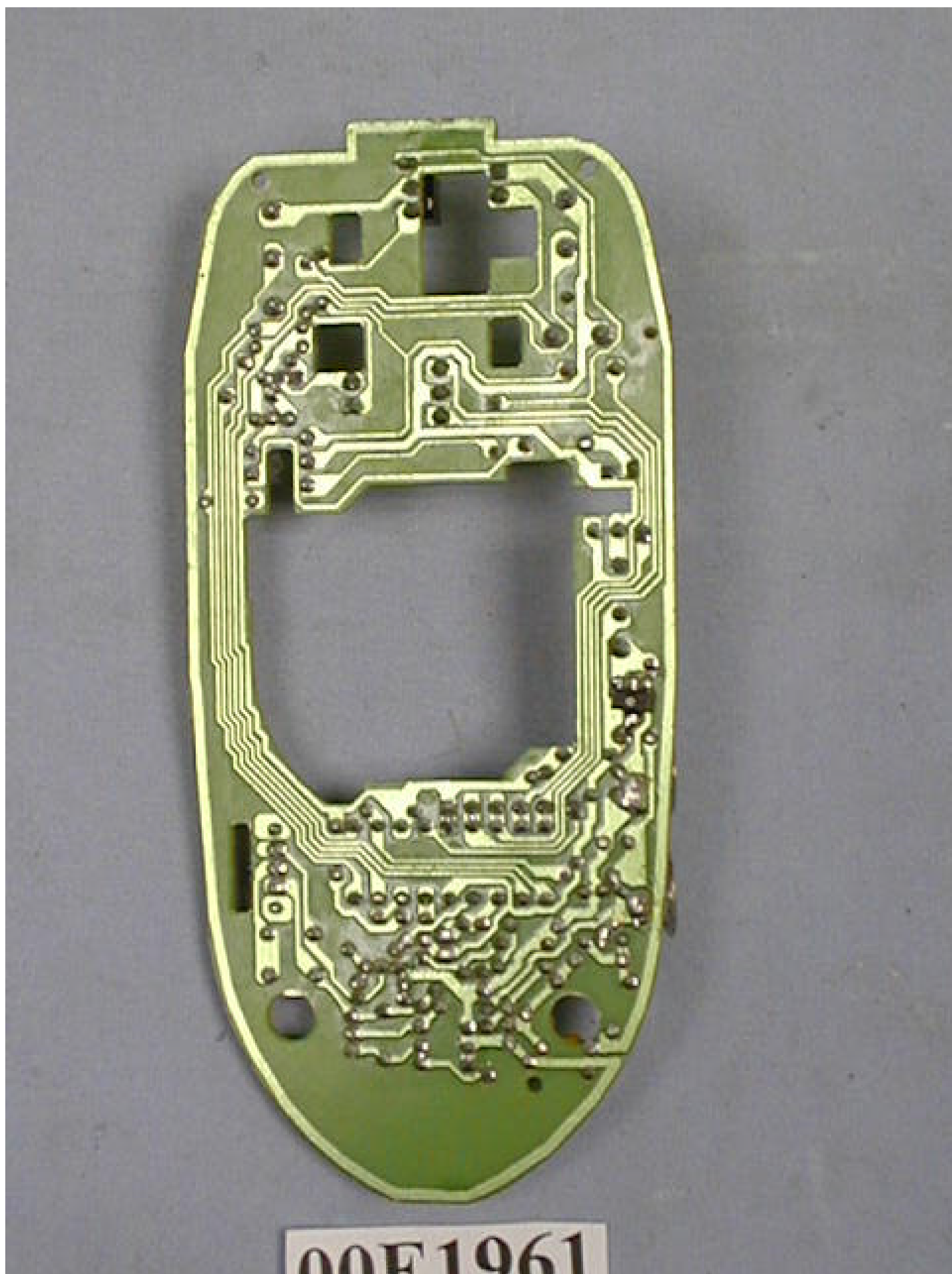
Photo # 2 RFW-23 Unit Partially Disassembled
